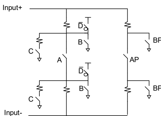
Figure 5. Programmable Input Buffer Logical Diagram
