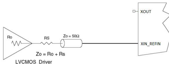
Figure 7. 1.2V LVC MOS Driver to XTAL Input Interface
