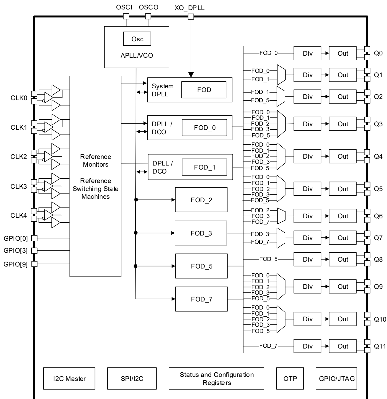
Figure 1. Block Diagram
