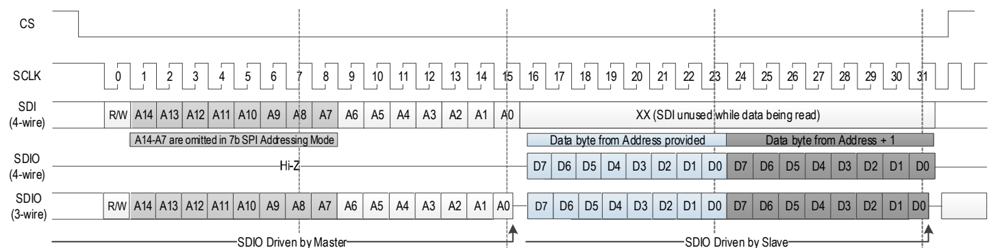
Figure 20. SPI Sequencing
