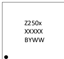
RH4Z250xBJ3GNM (12-DFN)
