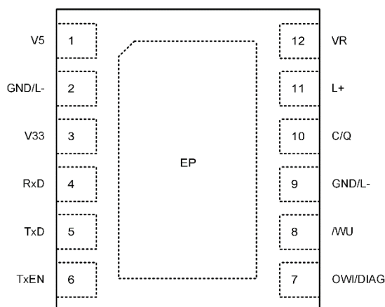
Figure 3. 12-DFN Pin Assignments (Top View)
