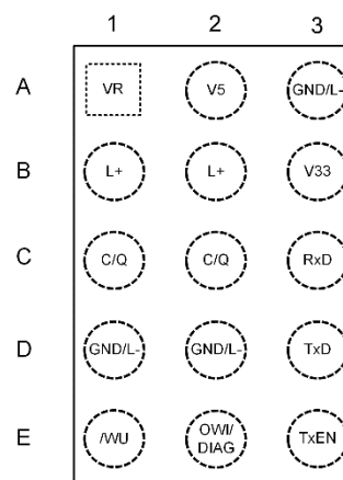
Figure 4. 15-WLCSP Pin Assignments (Top View)
