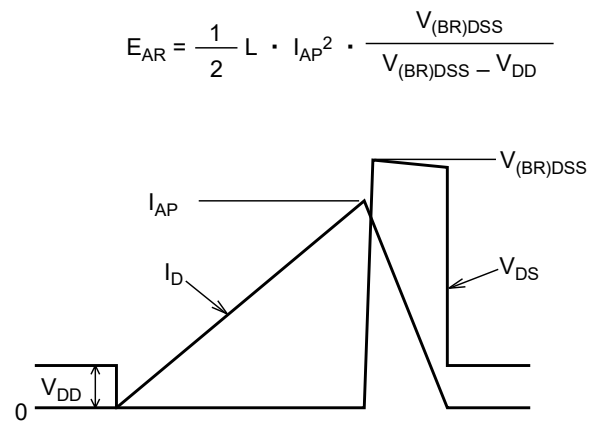
Avalanche Waveform
