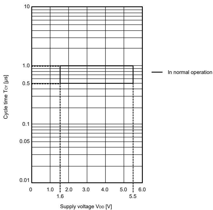
TCY vs VDD (LP (low-power main) mode)
