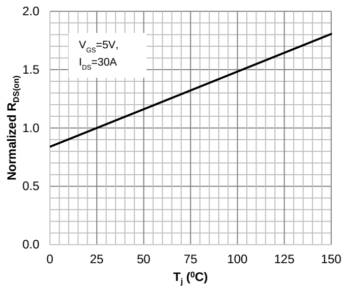
Figure 7. Normalized R_{DS(on)} , Parameter T_J
