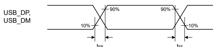
Figure 2.92 USB_DP, USB_DM output timing (full speed)
