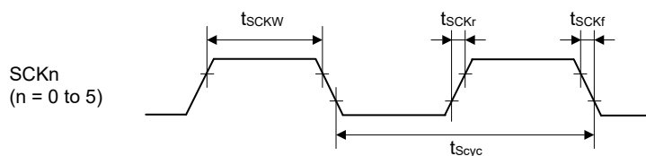
Figure 2.55 SCK clock input/output timing
