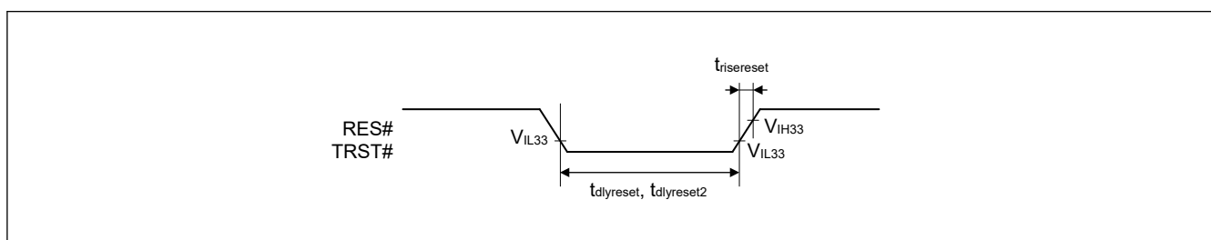
Figure 2.7 Reset input timing
