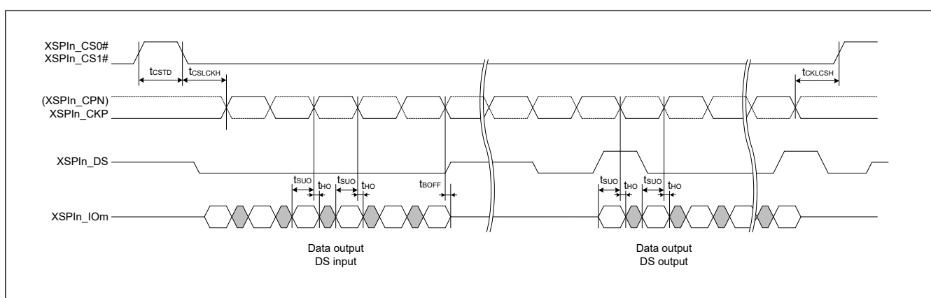
Figure 2.76 DDR transmit/receive timing (HyperRAM write)
