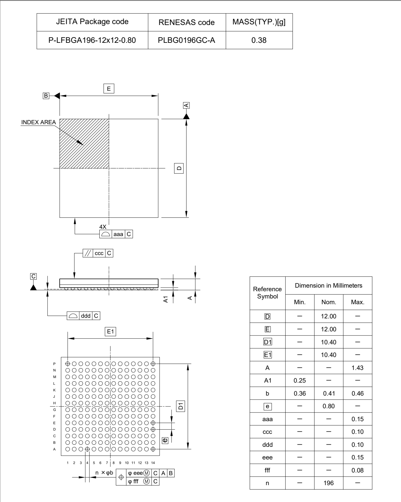
Figure A1.1 196-pin FBGA, 0.8mm pitch
