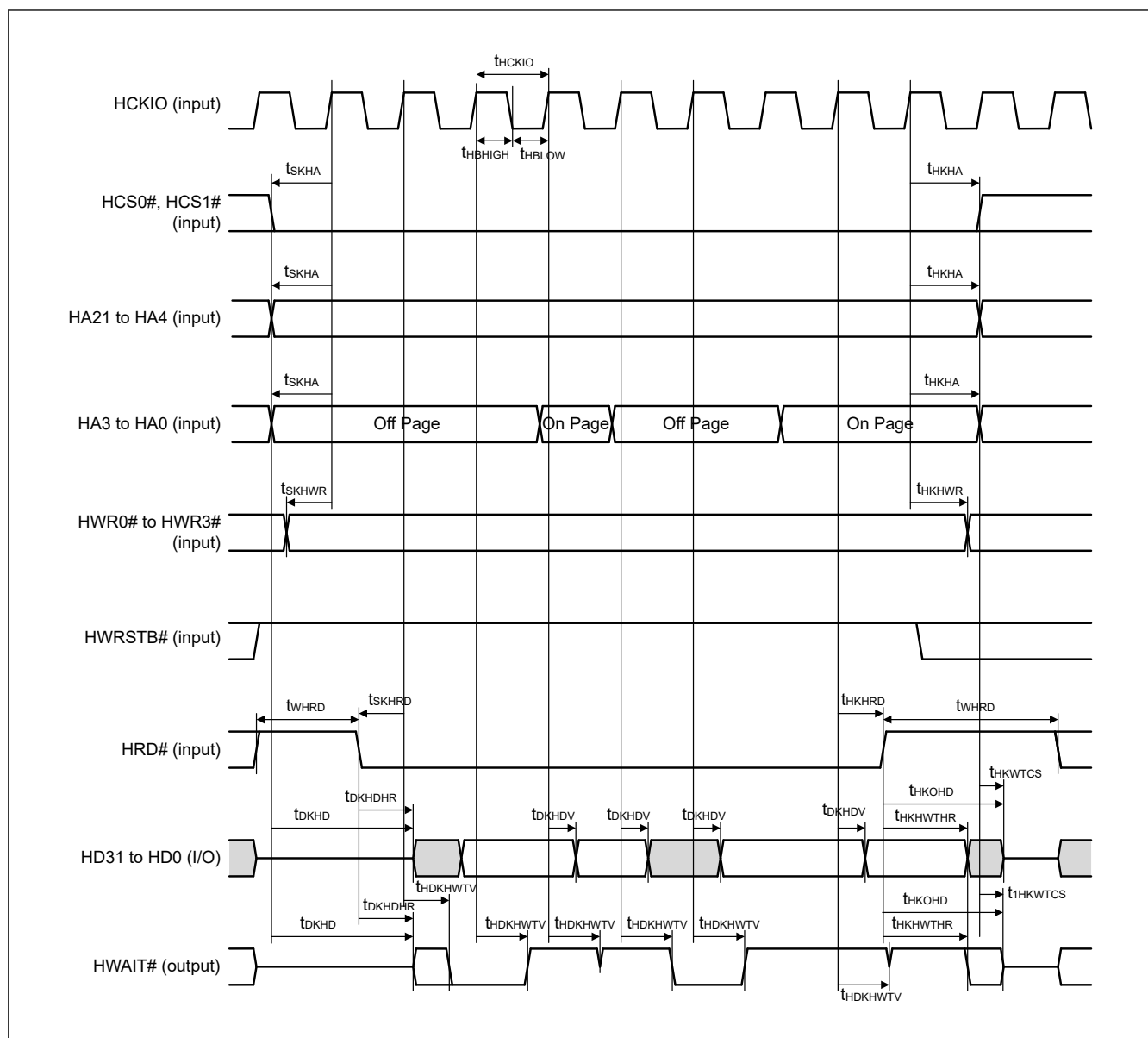
Figure 2.75 PHOSTIF page read timing (Synchronous SRAM interface mode)
