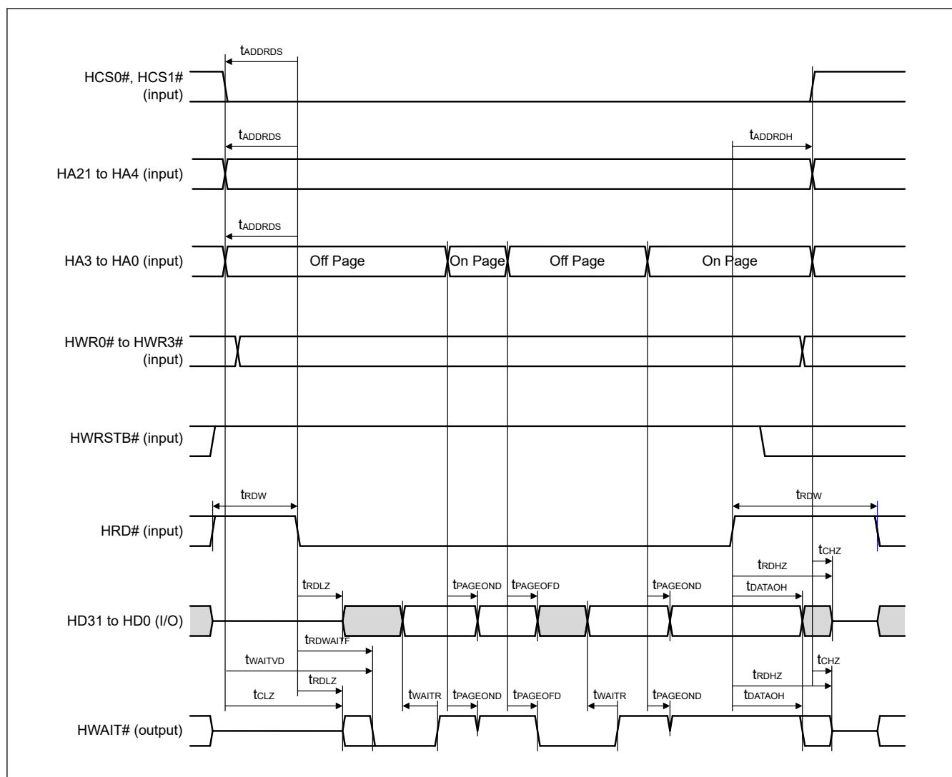
Figure 2.80 PHOSTIF page read timing (Asynchronous SRAM interface mode)
