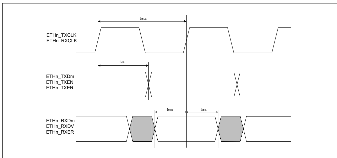
Figure 2.67 MII transmission and reception timing ( n = 0 to 4, m = 0 to 3)
