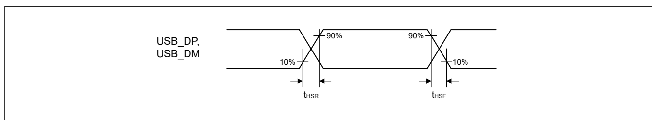
Figure 2.96 USB_DP, USB_DM output timing (high speed)
