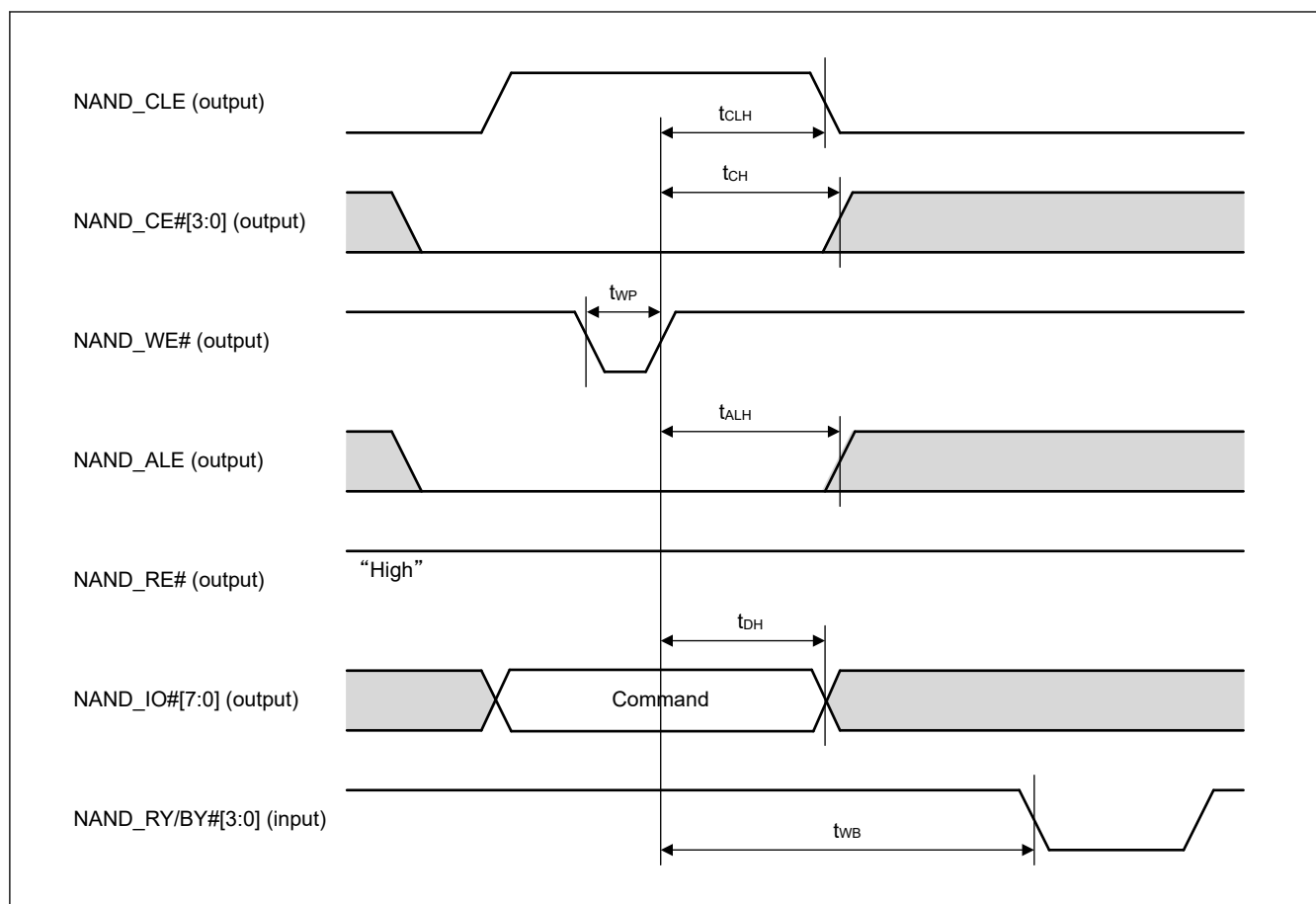
Figure 2.88 Command timing
