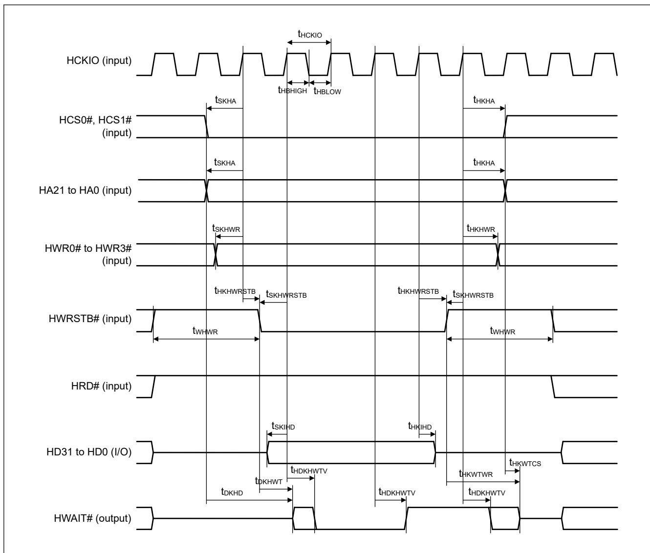
Figure 2.73 PHOSTIF write timing (Synchronous SRAM interface mode)
