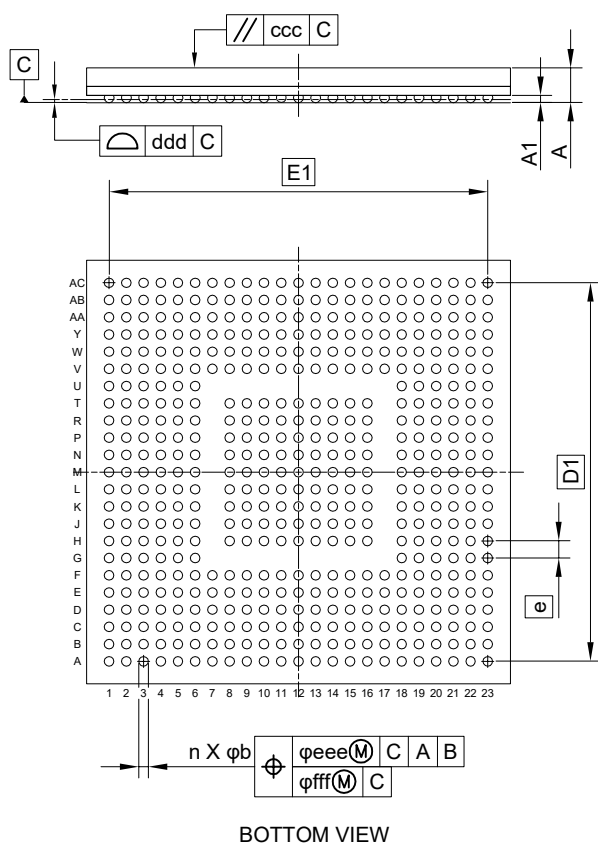
Figure A1.2 489-pin FBGA
