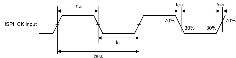
Figure 2.70 SHOSTIF clock timing
