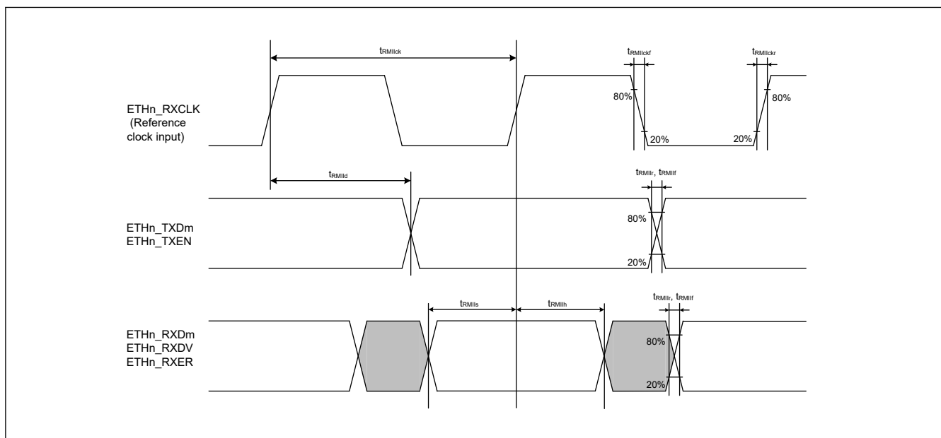
Figure 2.65 RMII transmission and reception timing (Reference clock input) (n = 0 to 4, m = 0 to 1)
