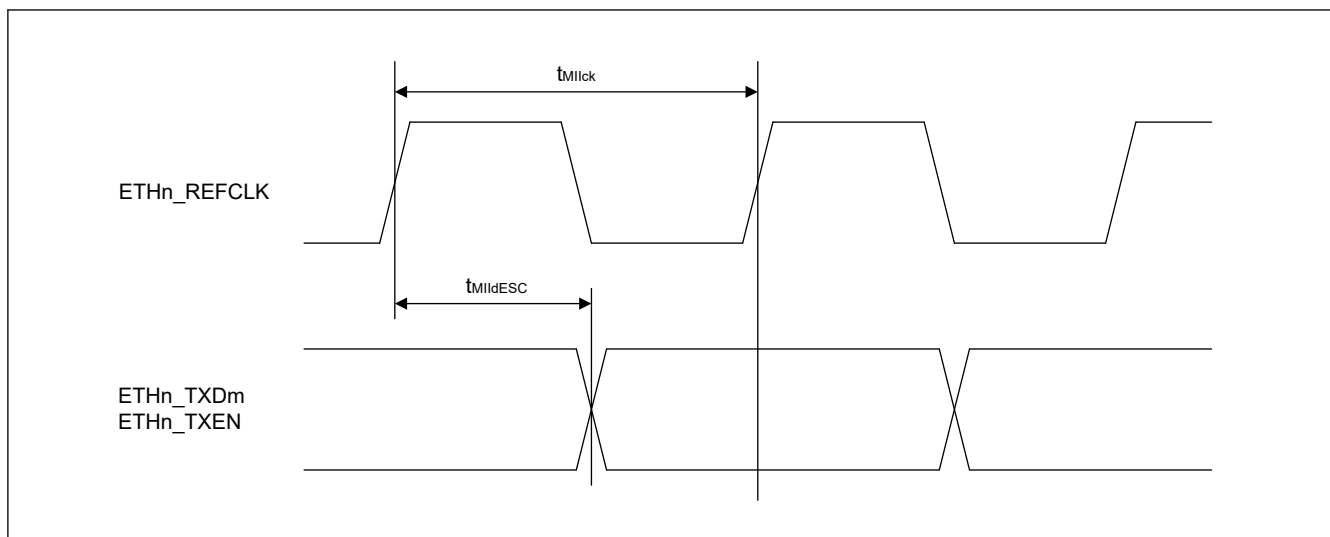
Figure 2.68 ESC MII transmission timing (Automatic TX shift disabled) ( n = 0 to 2 , m = 0 to 3 )
