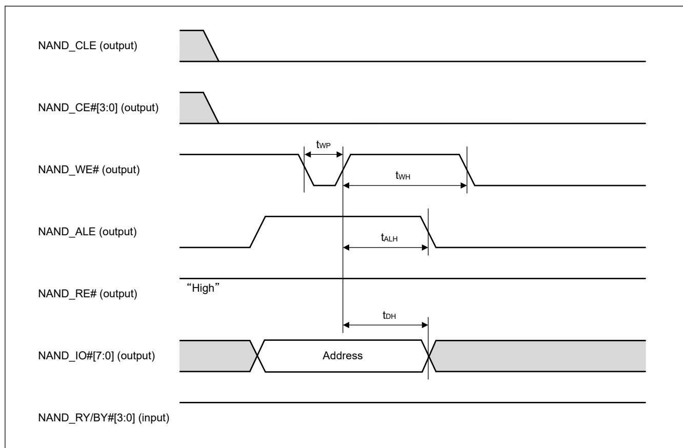
Figure 2.89 Address timing
