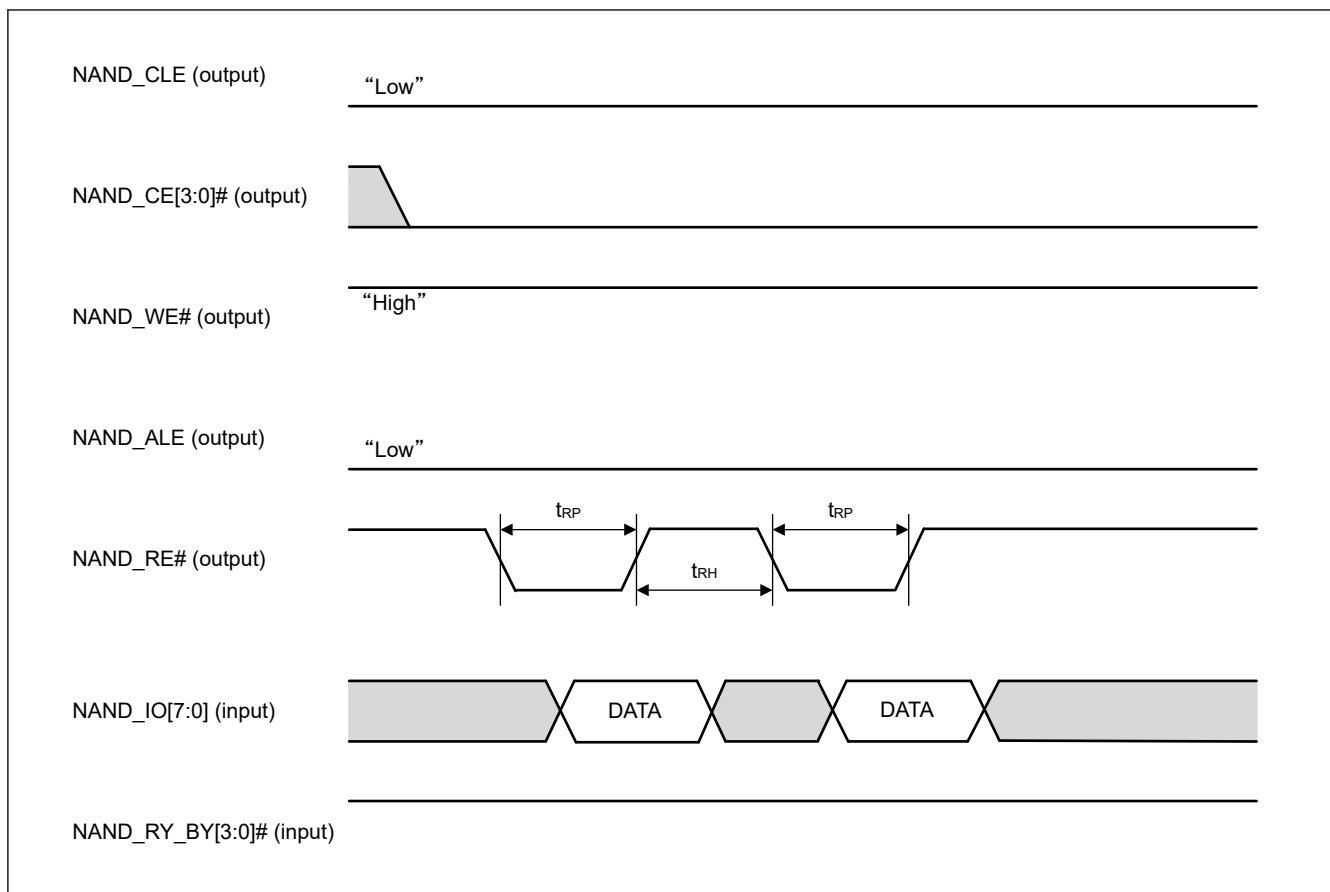
Figure 2.90 Data read timing
