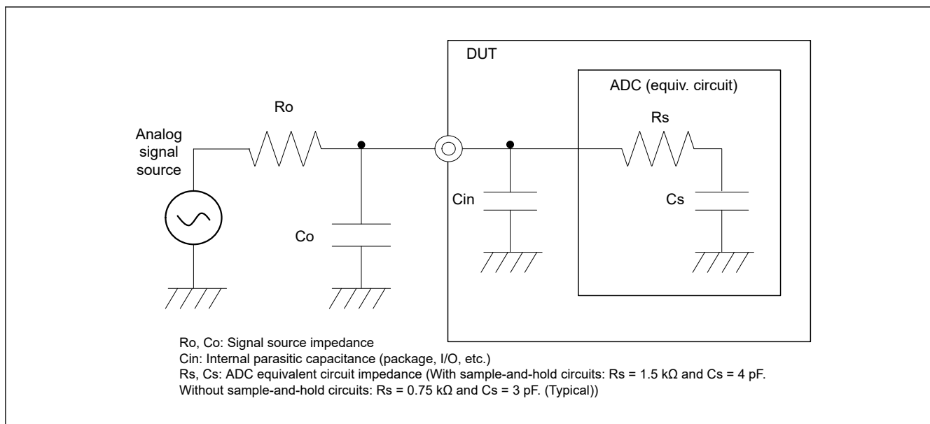
Figure 2.98 A/D converter equivalent circuit and peripheral configuration diagram
