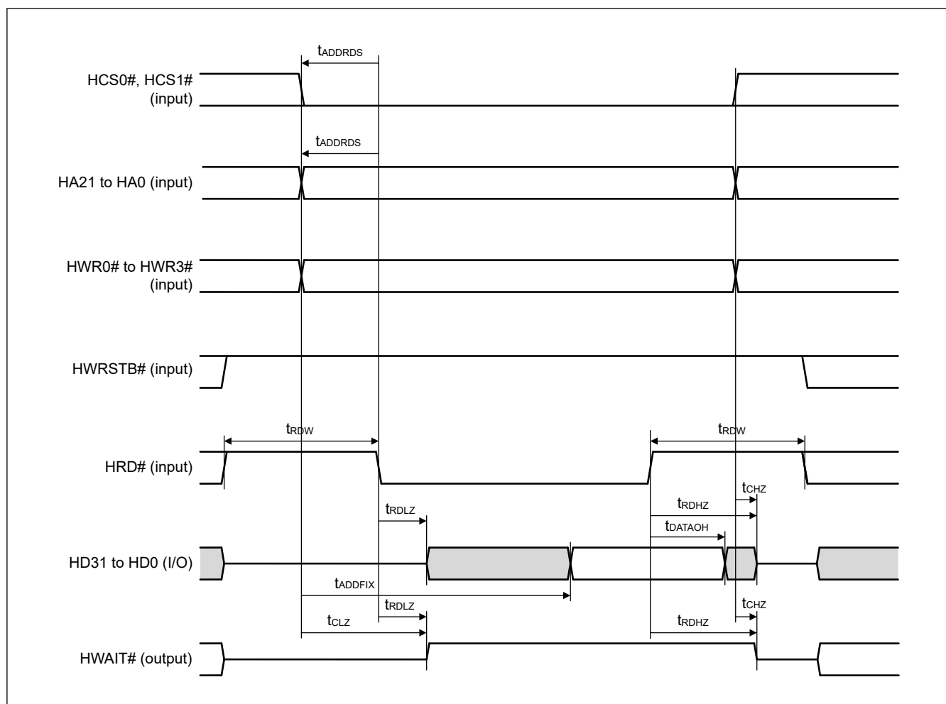
Figure 2.81 PHOSTIF register read timing (Asynchronous SRAM interface mode)
