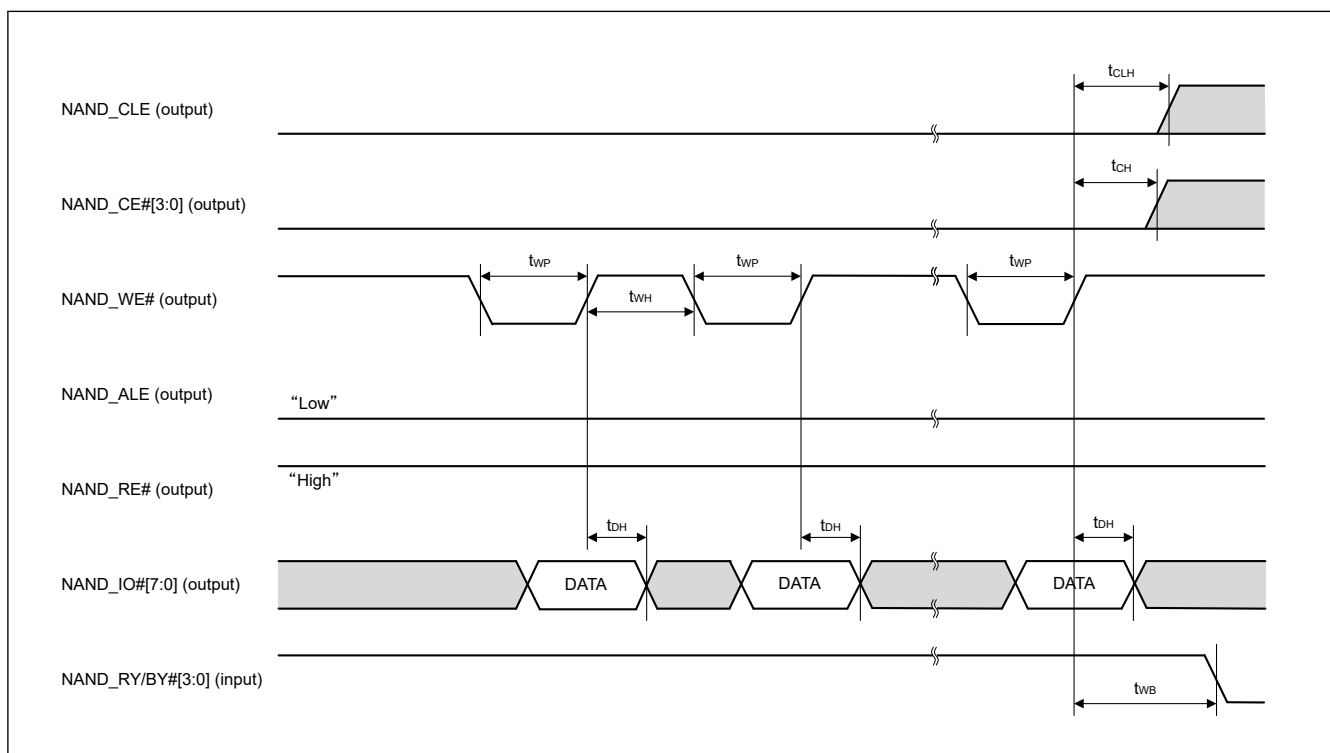
Figure 2.91 Data write timing
