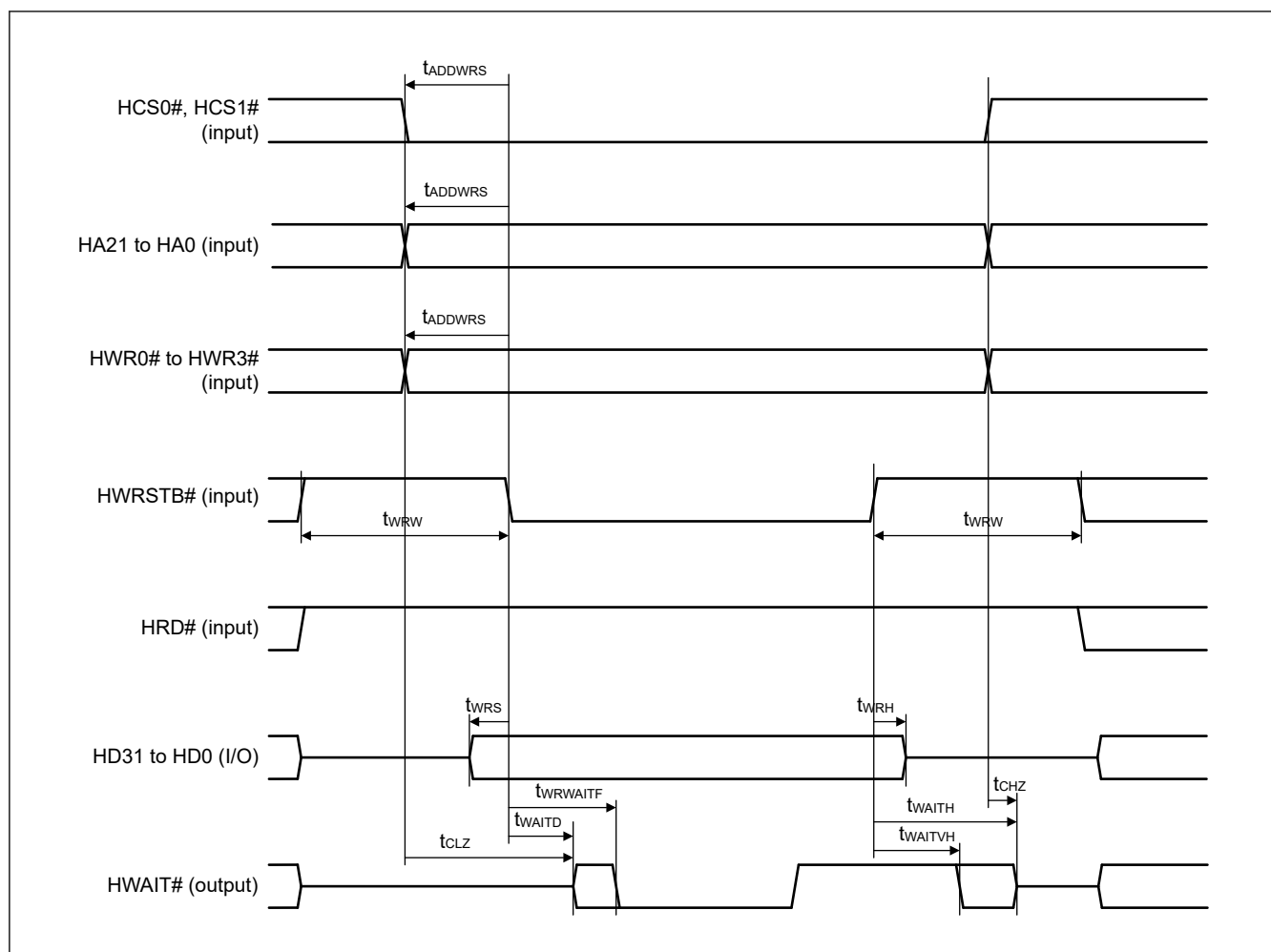
Figure 2.78 PHOSTIF write timing (Asynchronous SRAM interface mode)
