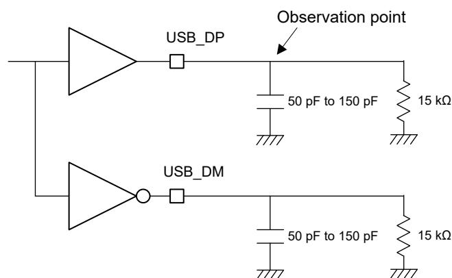
Figure 2.93 Measurement circuit (low-speed/host only)
