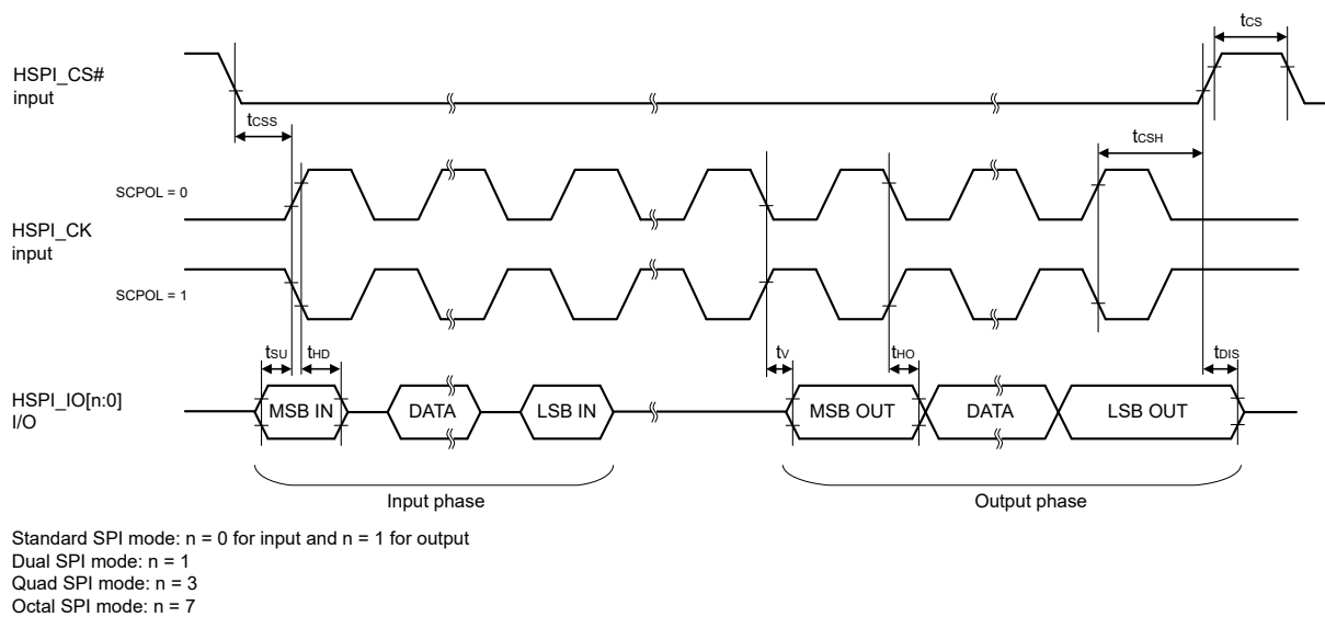
Figure 2.71 SHOSTIF timing (SCPH = 0)
