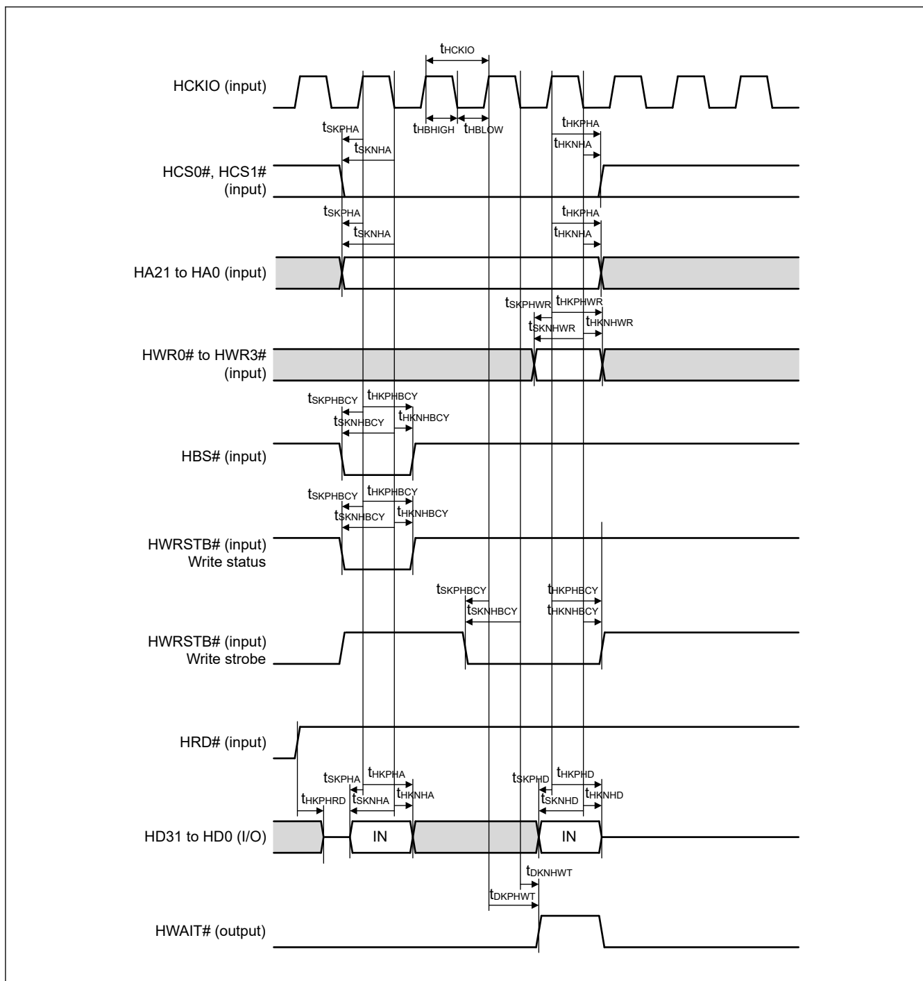
Figure 2.84 PHOSTIF write timing (Synchronous Burst SRAM Type transfer mode, Address/Data multiplexing)
