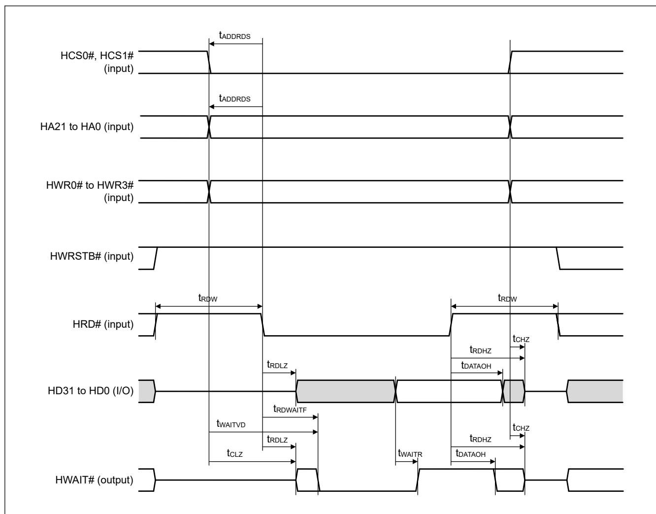
Figure 2.79 PHOSTIF read timing (Asynchronous SRAM interface mode)
