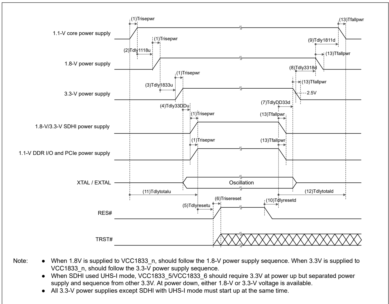
Figure 2.1 Power on/off sequence
