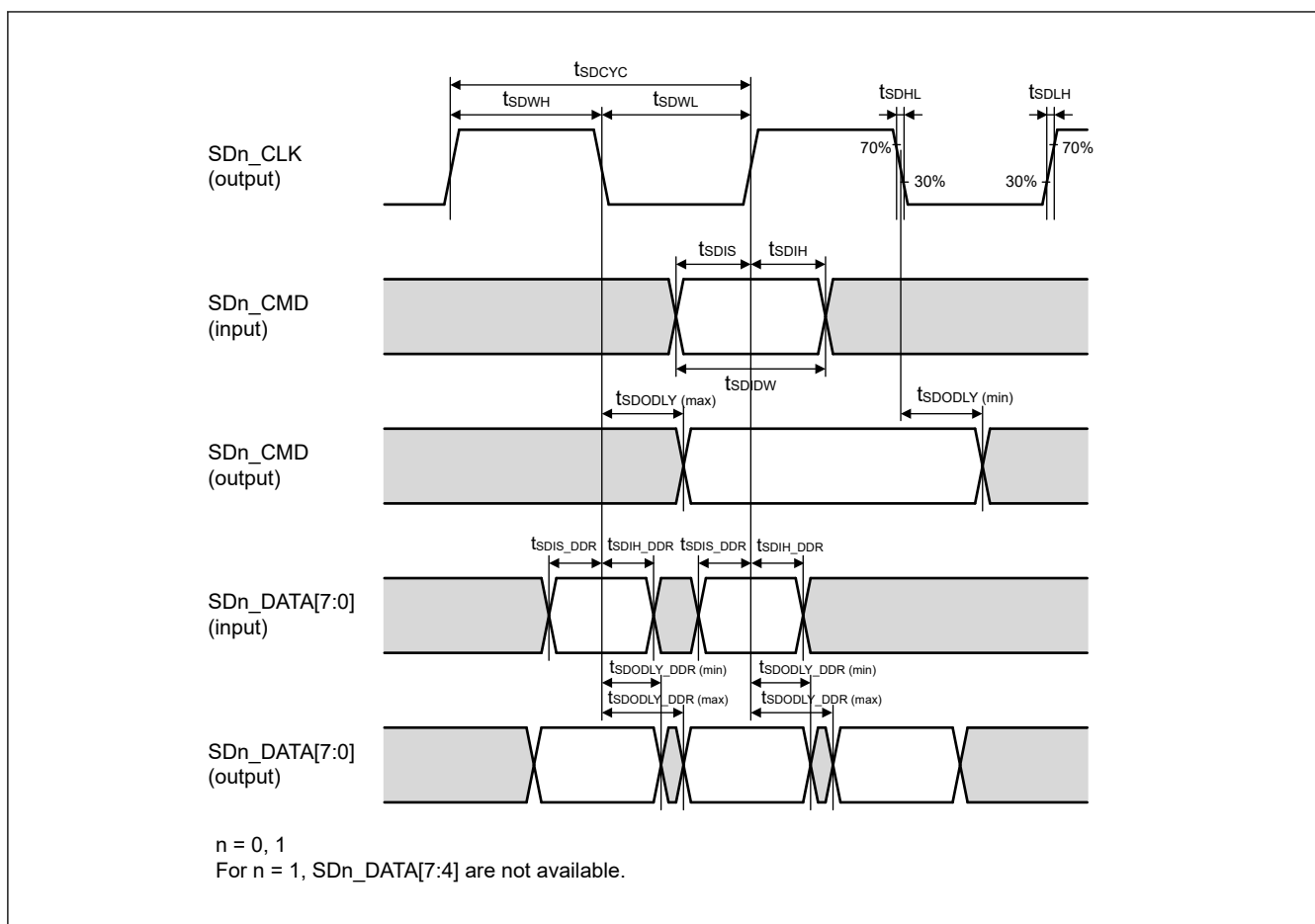
Figure 2.87 SDHI timing (DDR)
