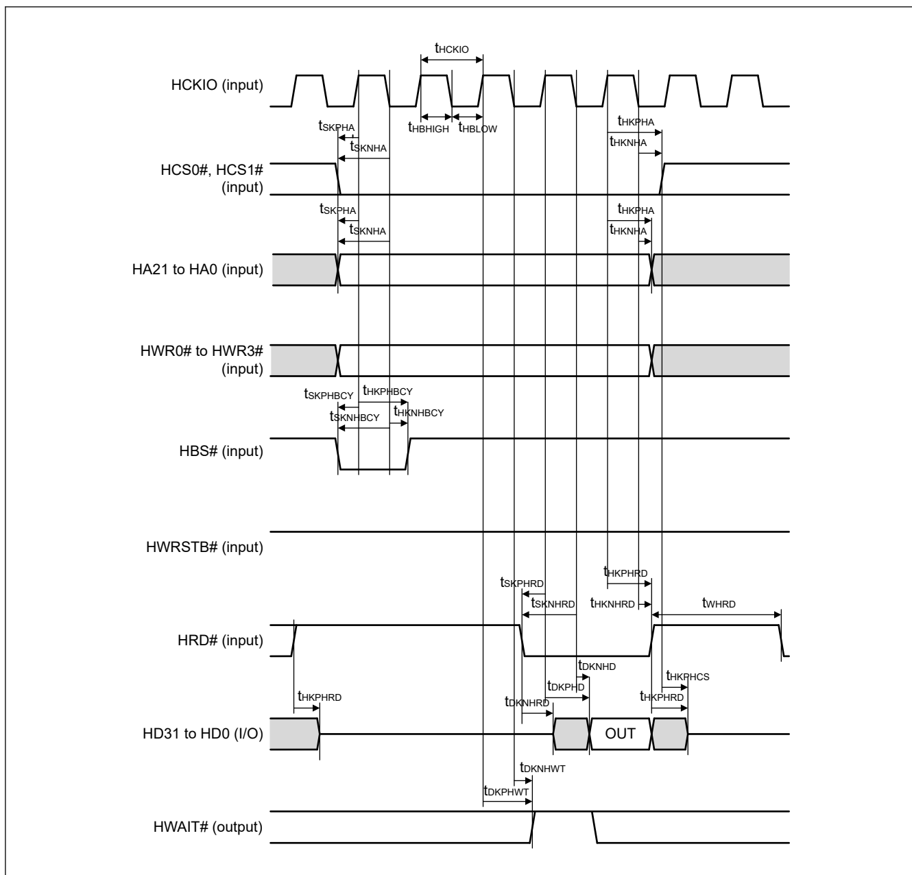
Figure 2.83 PHOSTIF read timing (Synchronous Burst SRAM Type transfer mode, Address/Data separation)
