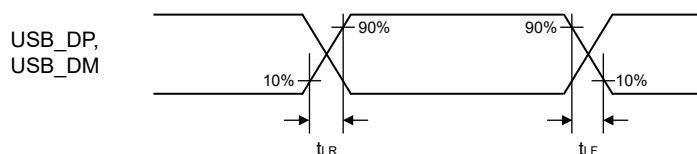
Figure 2.92 USB_DP, USB_DM output timing (low-speed/host only)
