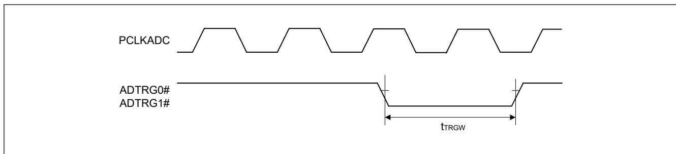
Figure 2.37 A/D converter trigger input timing (ADTRG0#, ADTRG1#)
