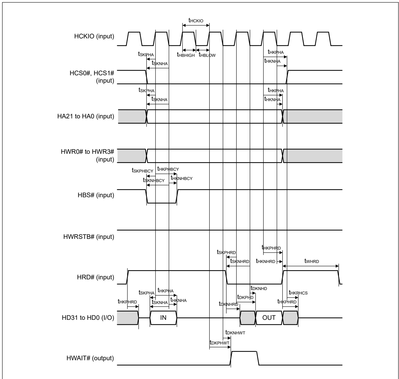
Figure 2.85 PHOSTIF read timing (Synchronous Burst SRAM Type transfer mode, Address/Data multiplexing)
