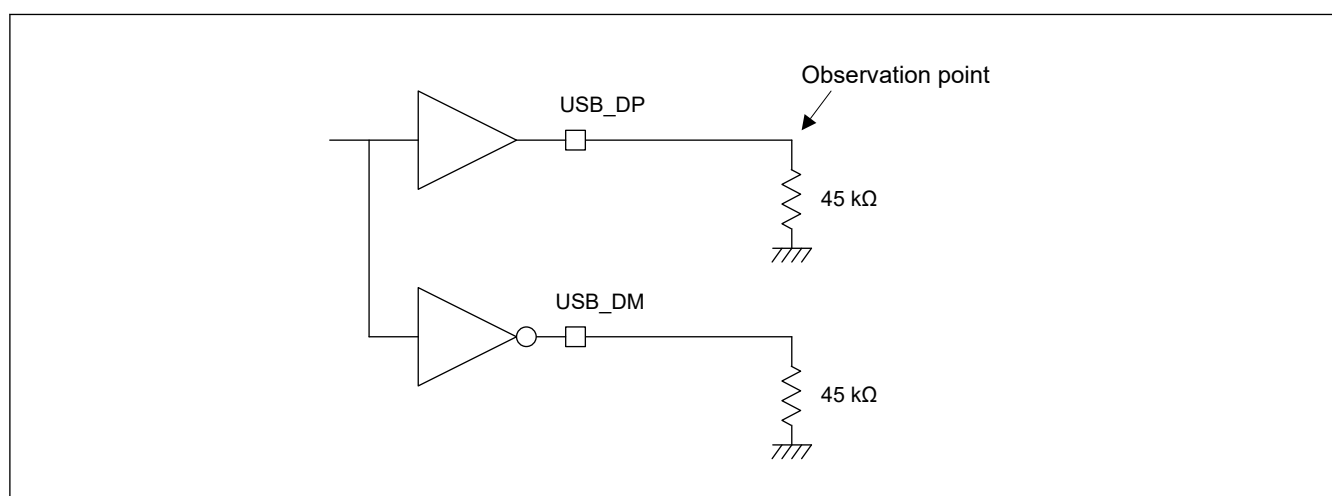
Figure 2.97 Measurement circuit (high speed)
