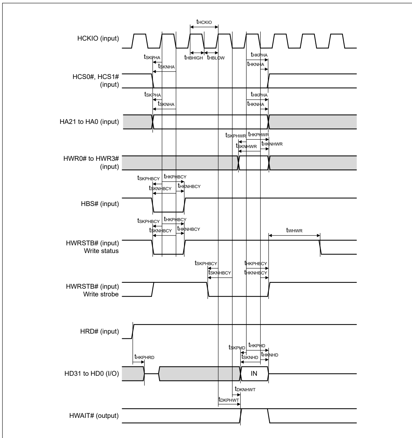
Figure 2.82 PHOSTIF write timing (Synchronous Burst SRAM Type transfer mode, Address/Data separation)
