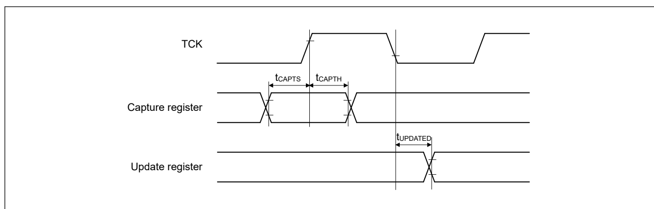
Figure 2.101 Boundary scan input/output timing
