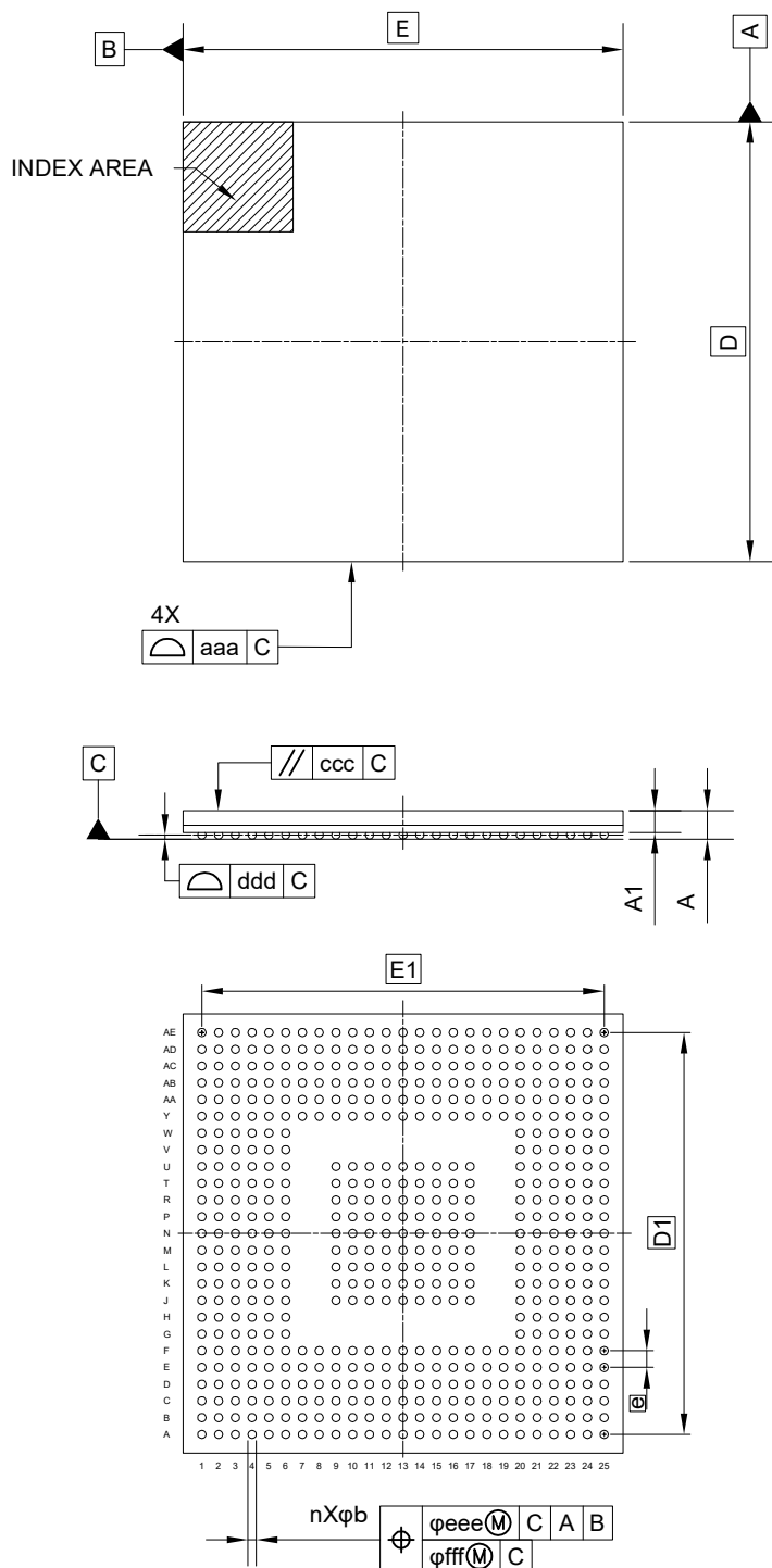
Figure A1.1 537-pin FBGA
