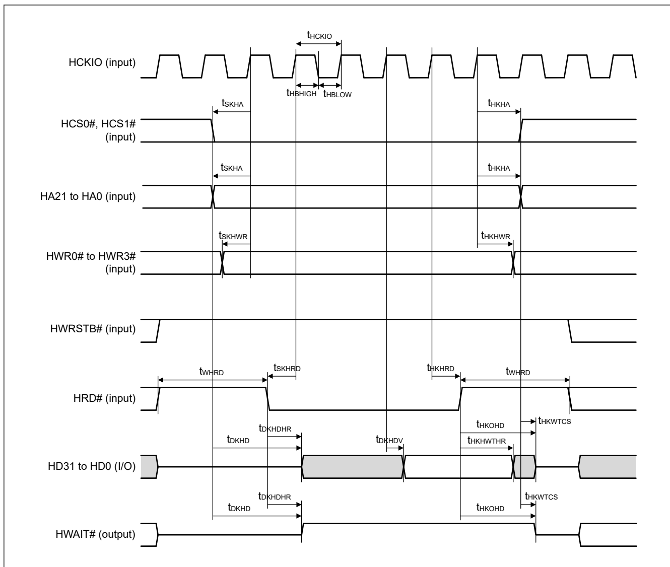
Figure 2.77 PHOSTIF page read timing (PHOSTIF register write) (Synchronous SRAM interface mode)
