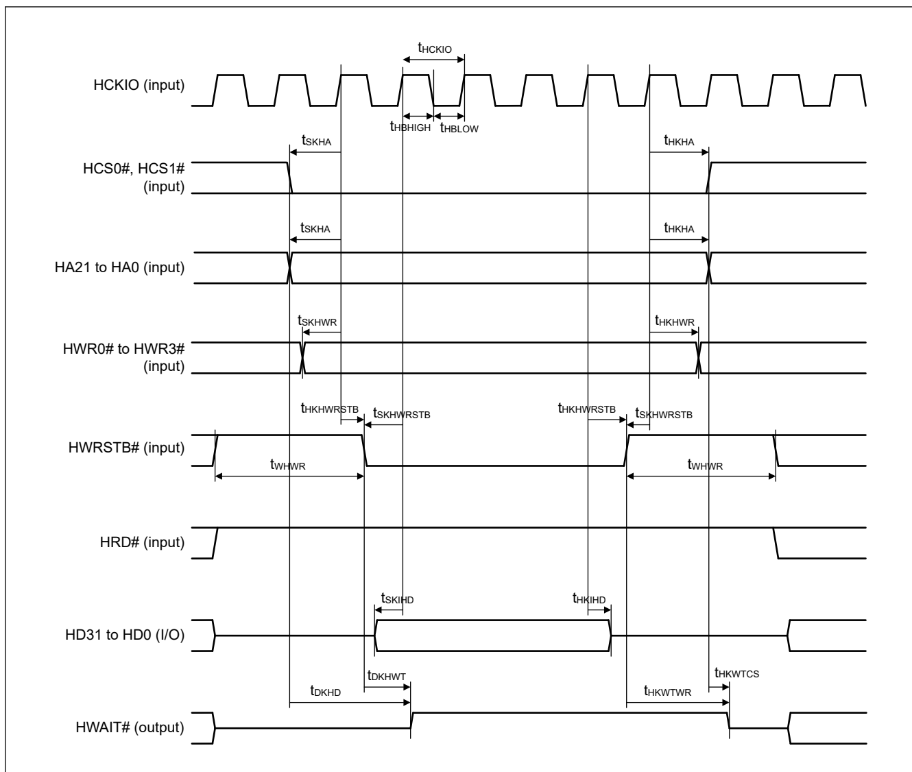
Figure 2.76 PHOSTIF page write timing (PHOSTIF register write) (Synchronous SRAM interface mode)
