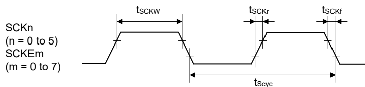
Figure 2.38 SCK clock input/output timing
