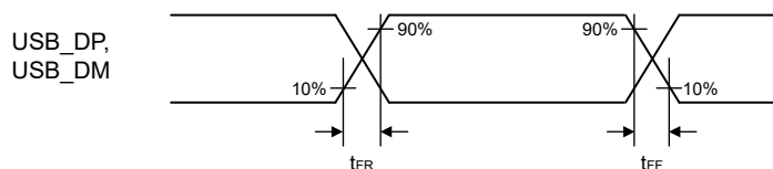
Figure 2.94 USB_DP, USB_DM output timing (full speed)
