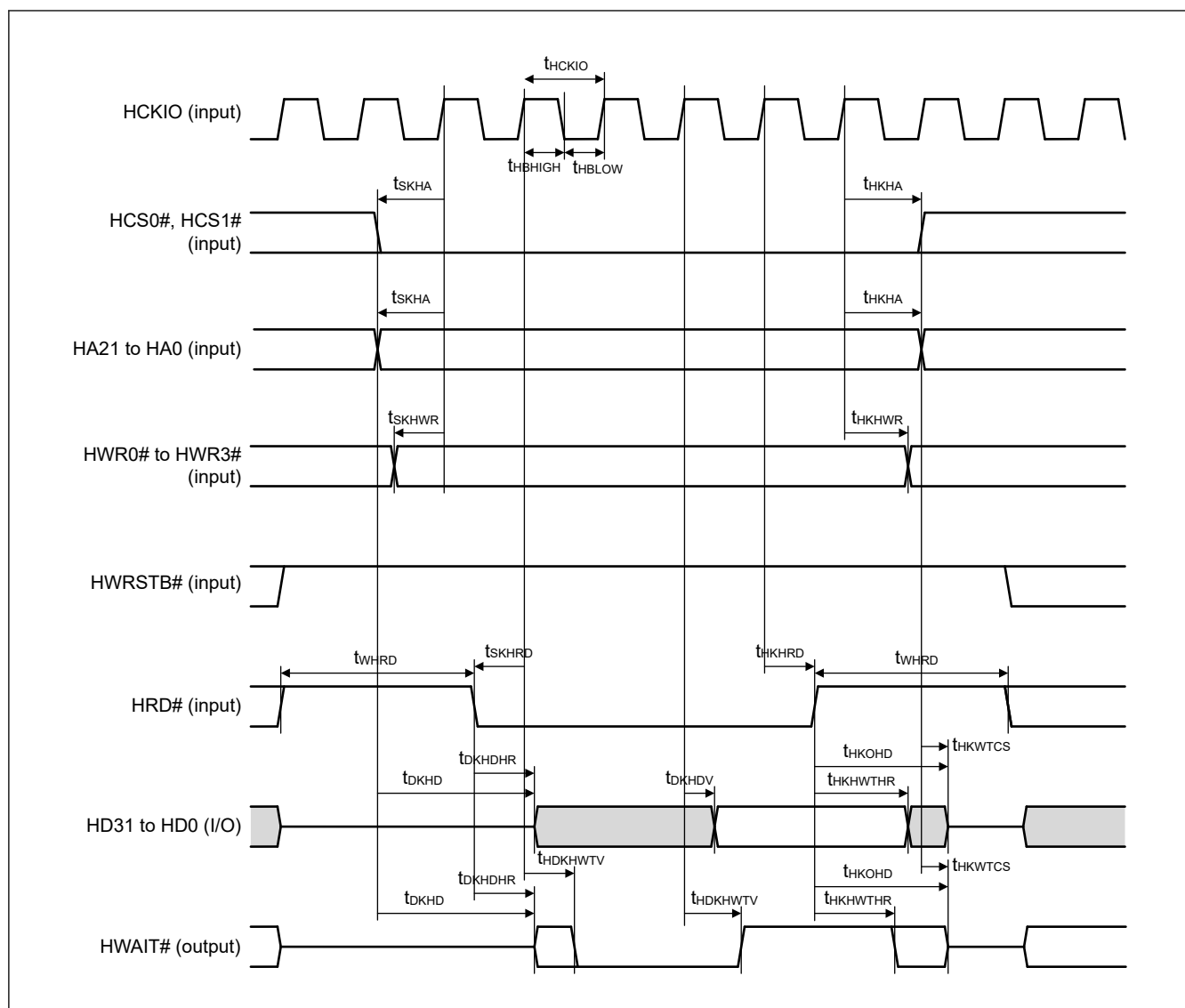
Figure 2.74 PHOSTIF read timing (Synchronous SRAM interface mode)
