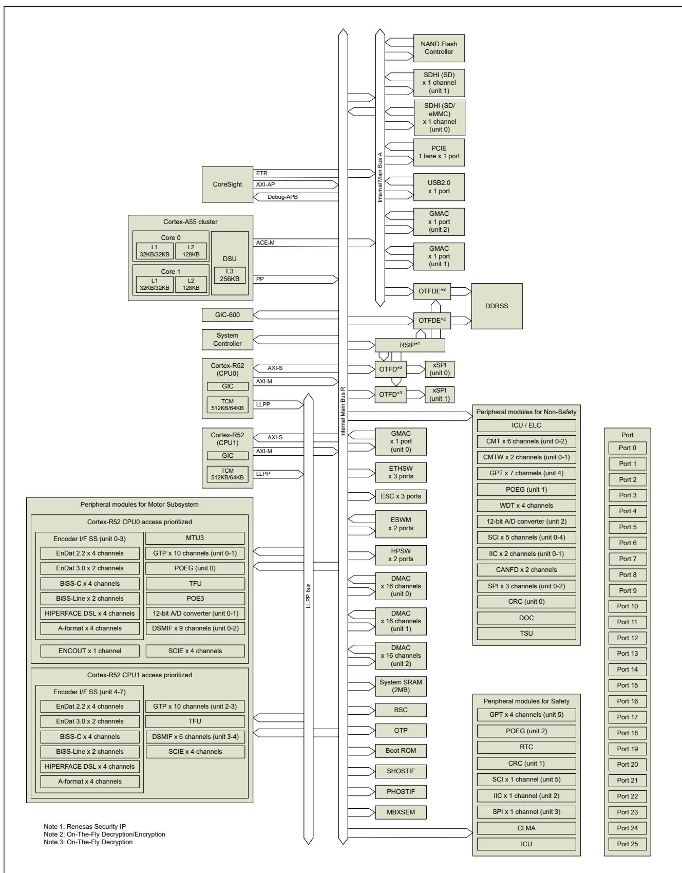
Figure 1.1 Block diagram
