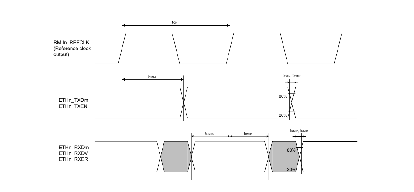
Figure 2.66 RMI transmission and reception timing (Reference clock output) ( n = 0 to 4, m = 0 to 1)
