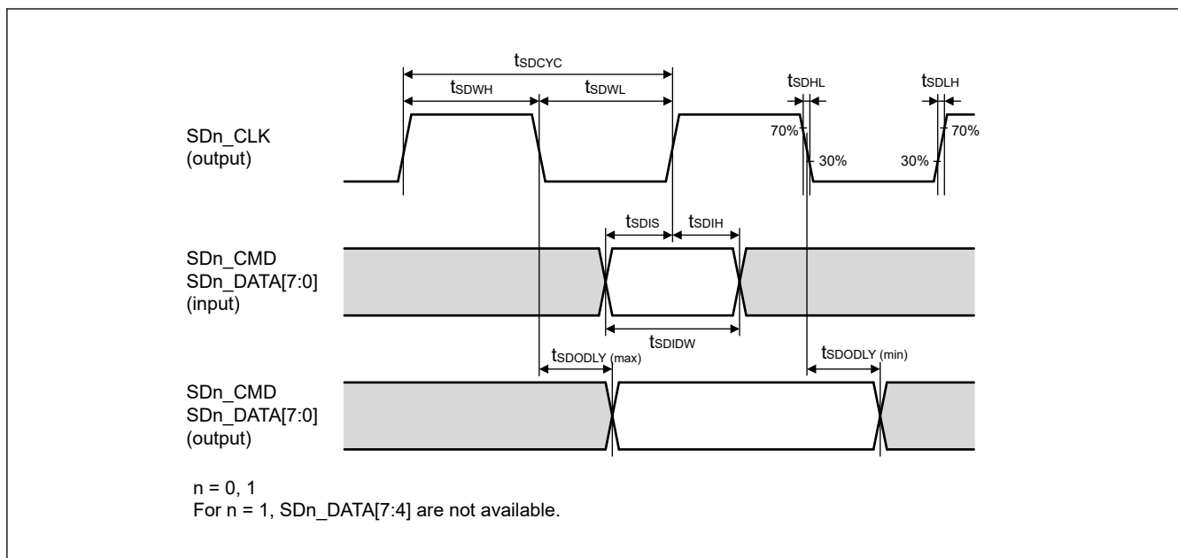
Figure 2.86 SDHI timing (SDR)
