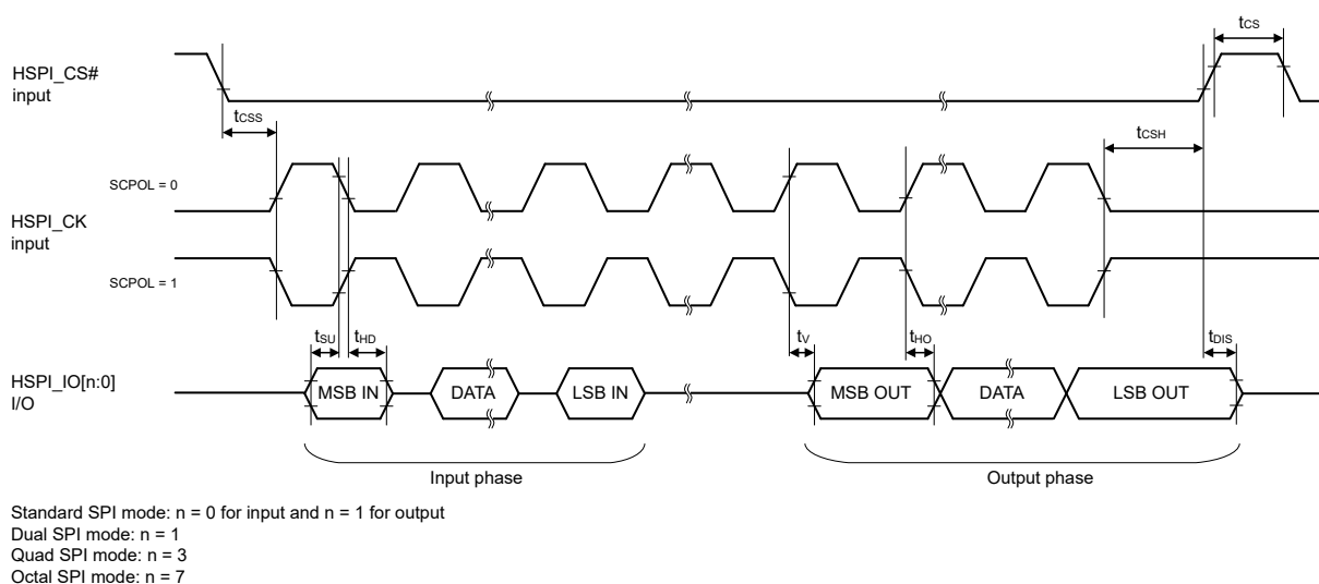
Figure 2.72 SHOSTIF timing (SCPH = 1)
