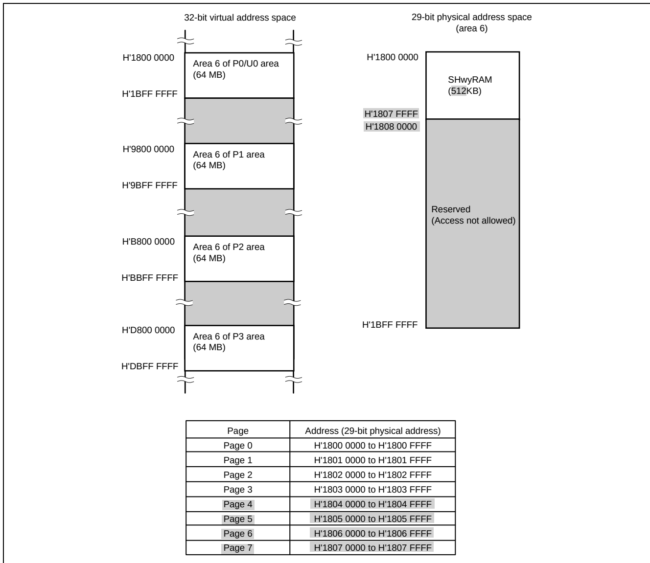
Figure 13.2 Address Space
