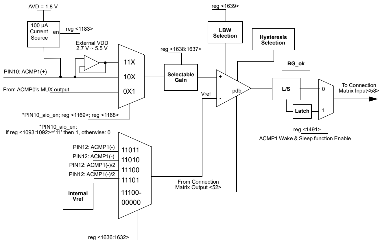
Figure 43. ACMP1 Block Diagram
