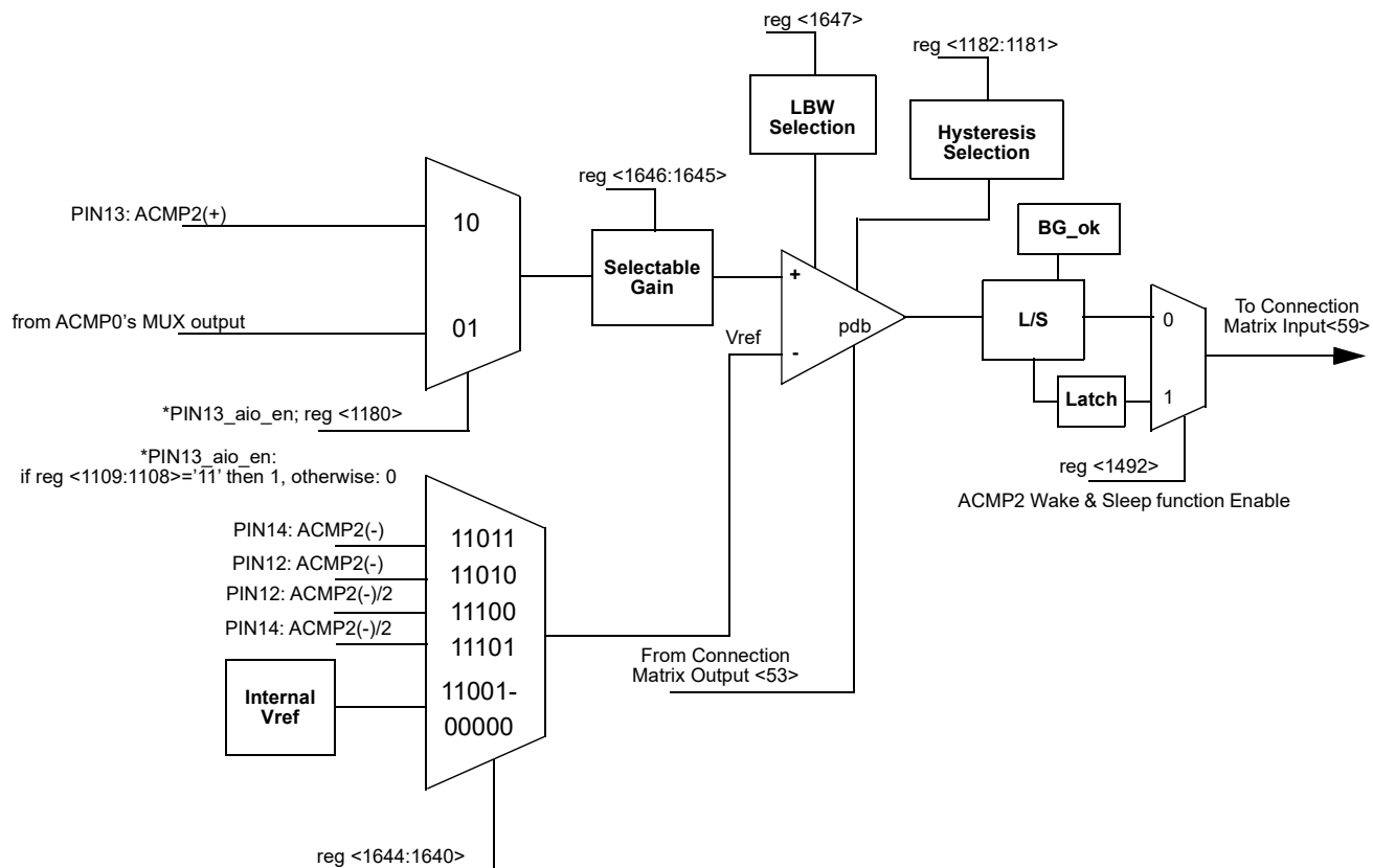
Figure 44. ACMP2 Block Diagram
