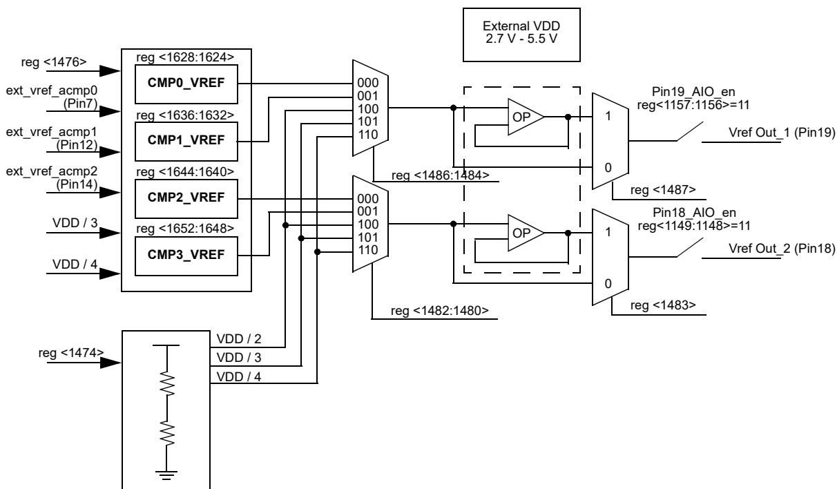
Figure 49. Voltage Reference Block Diagram
