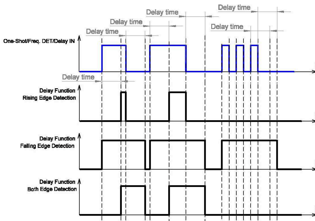
Figure 33. Delay Mode
