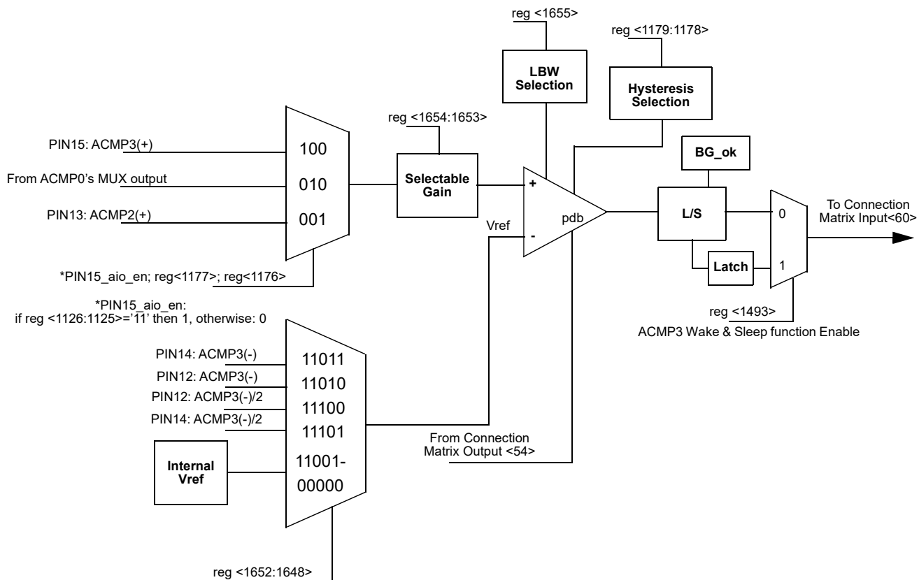
Figure 45. ACMP3 Block Diagram
