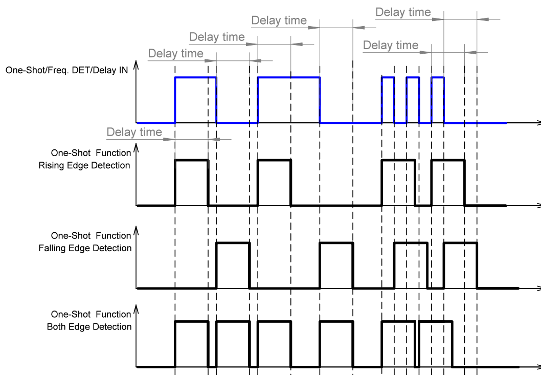
Figure 30. One-shot function
