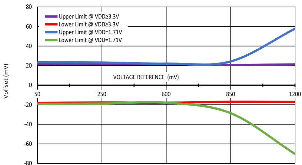
Figure 40. Typical Buffer Input Voltage Offset vs. Voltage Reference at T = (-40.... +85)°C, Buffer Bandwidth = 1 kHz, V hys = 0 mV, Gain = 1.
