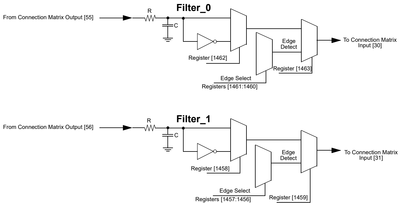
Figure 57. Deglitch Filter/Edge Detector
