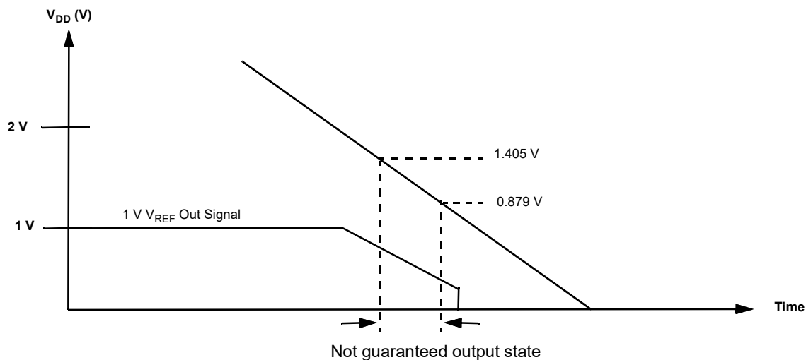
Figure 86. Power-Down
