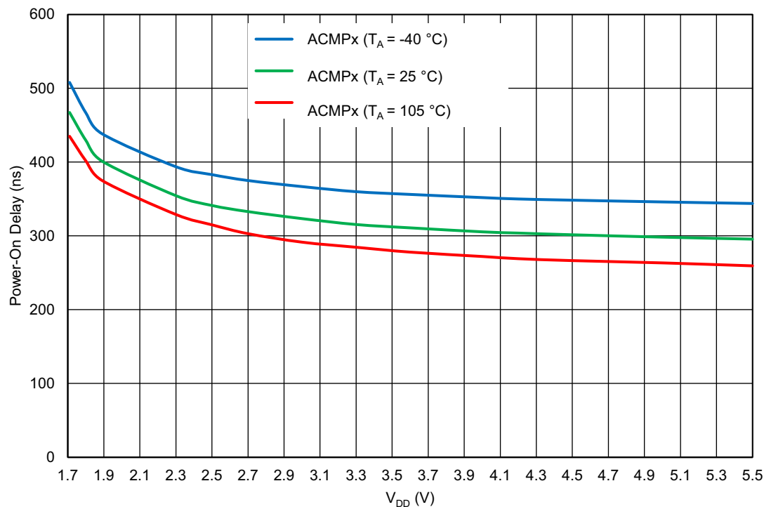
Figure 48. ACMPx Power-On Delay vs. V_{DD} , BG Delay – Any
