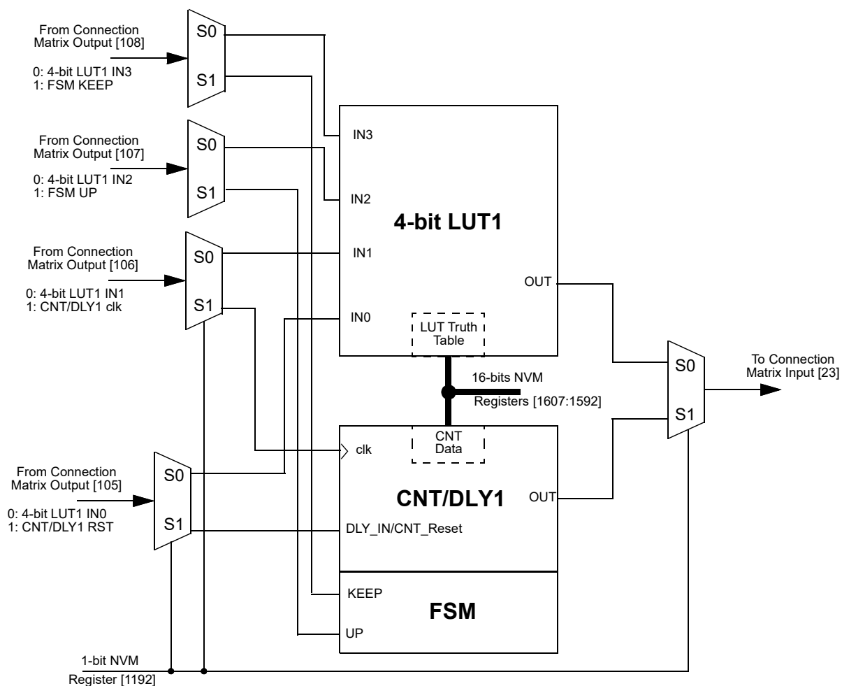
Figure 30. 4-bit LUT1 or CNT/DLY1
