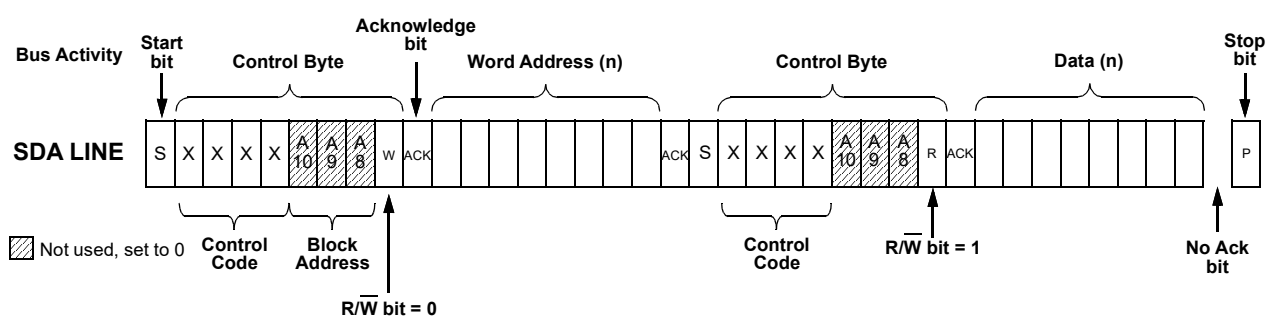
Figure 111. Random Read Command
