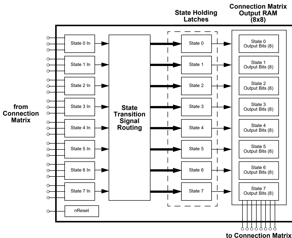
Figure 88. Asynchronous State Machine
