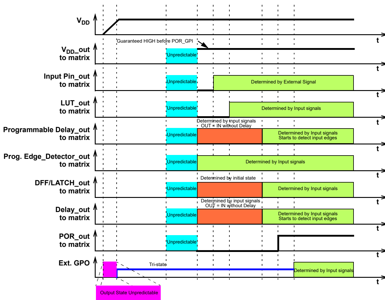
Figure 85. Internal Macrocell States during POR Sequence
