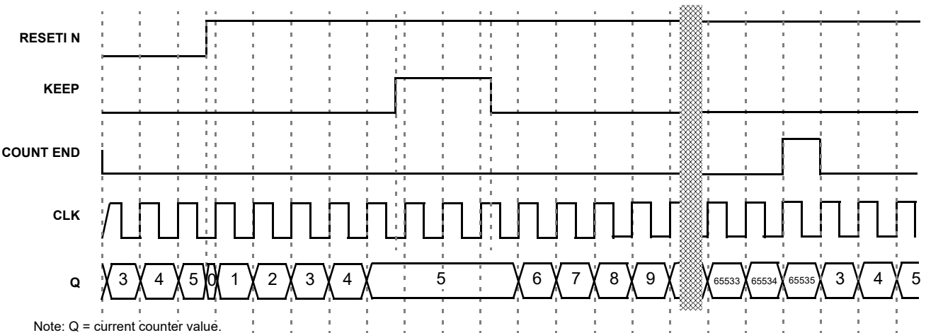
Figure 39. CNT/FSM Timing Diagram (Reset Rising Edge Mode, Oscillator is Forced On, UP = 1) for Counter Data = 3
