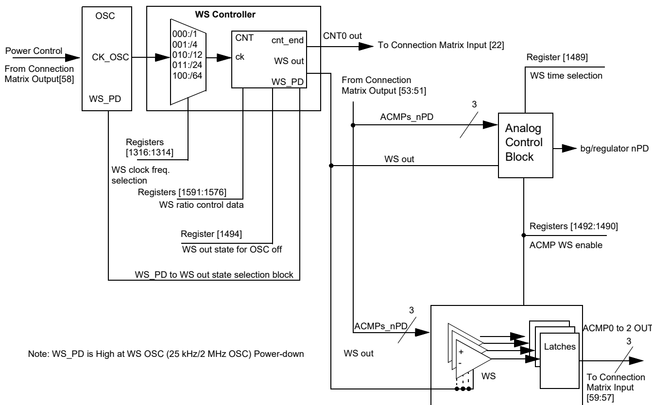
Figure 44. Wake/Sleep Controller
