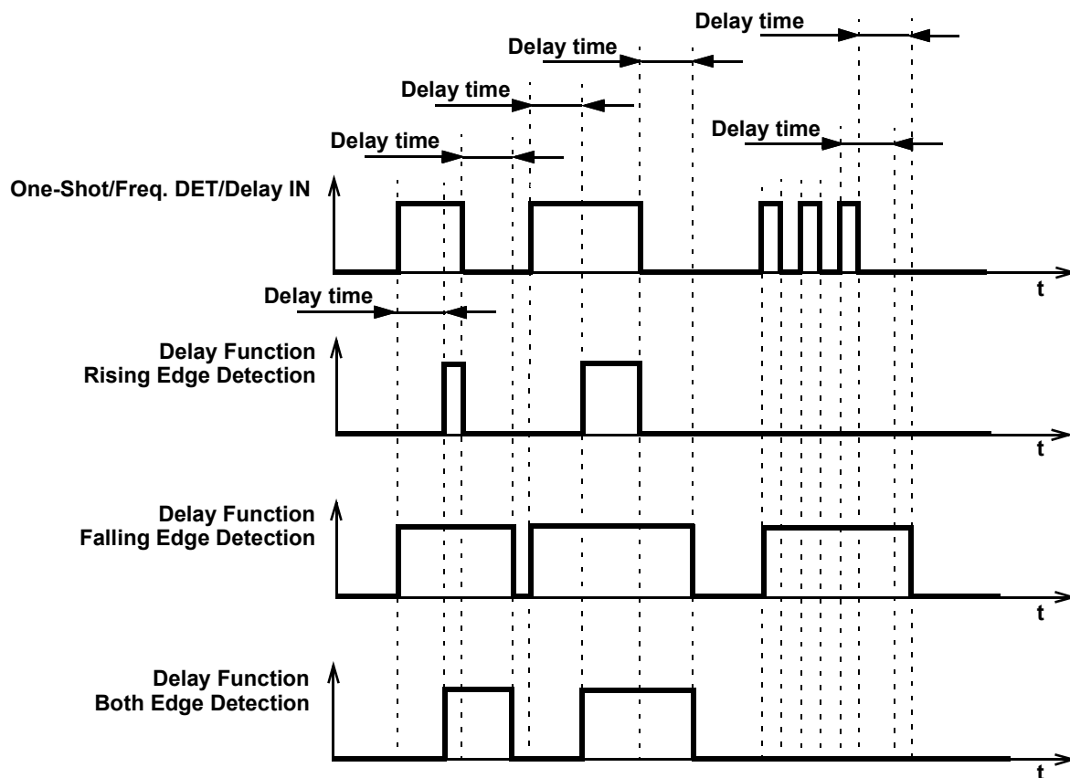
Figure 36. Delay Mode Timing Diagram
