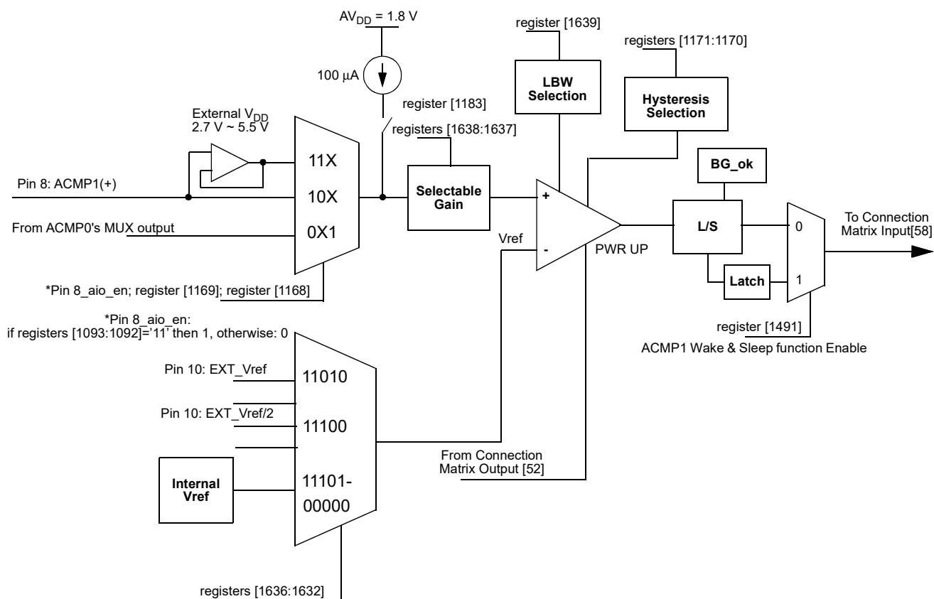
Figure 46: ACMP1 Block Diagram
