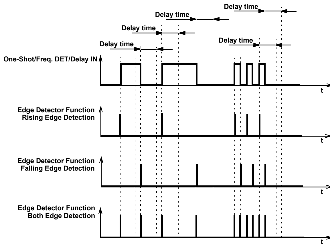
Figure 35. Edge Detection Mode Timing Diagram
