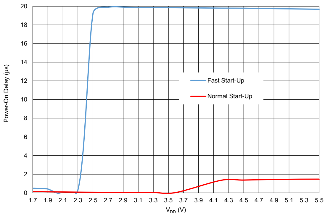
Figure 65. Oscillator Maximum Power-On Delay vs. V_{DD} at T_A = +25\text{ }^{\circ}\text{C} , OSC0 = 25 kHz
