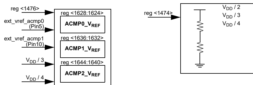
Figure 58. Voltage Reference Block Diagram
