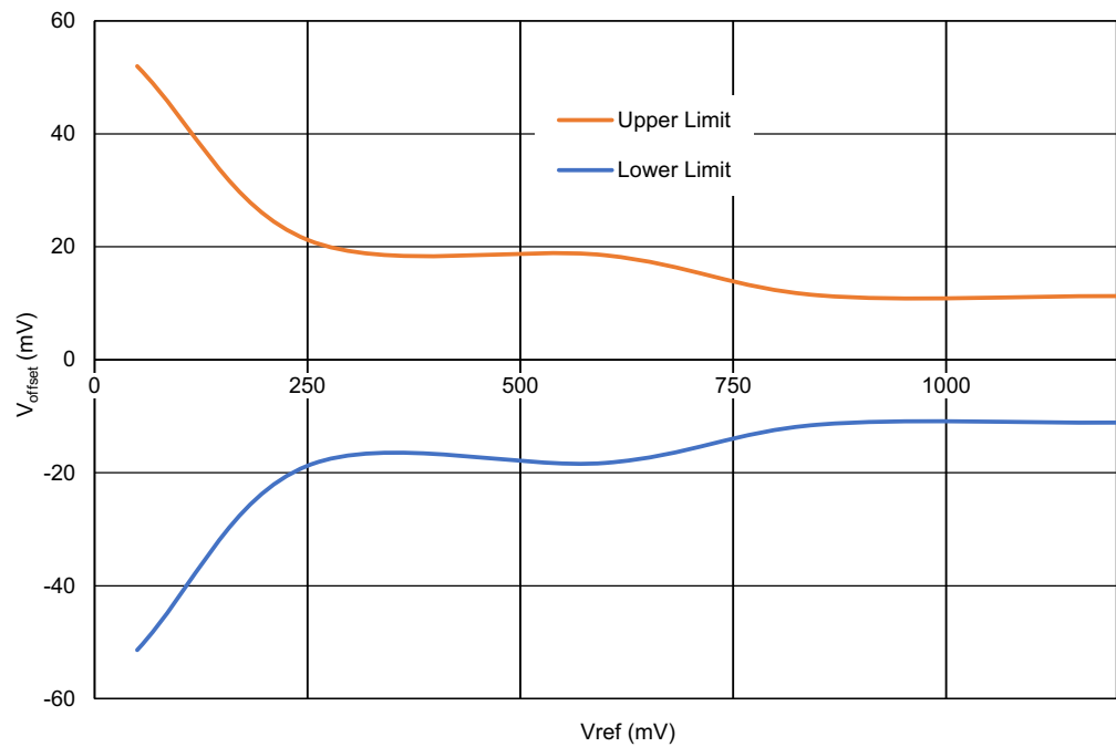
Figure 50. ACMPx Buffer Input Offset Voltage vs. V_{REF} at V_{DD} = 1.71\text{ V to }5.5\text{ V} , T_A = -40\text{ }^{\circ}\text{C to }+105\text{ }^{\circ}\text{C}
