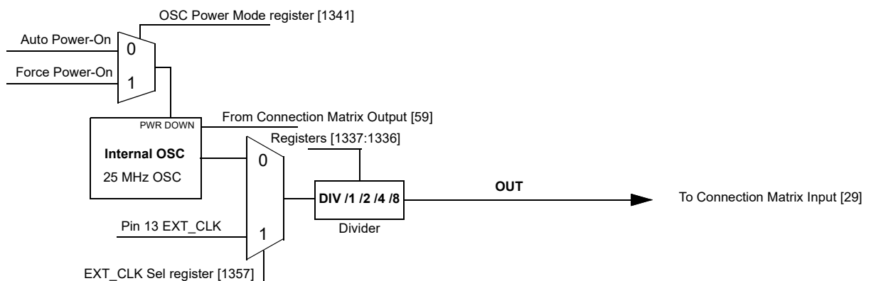
Figure 63. 25 MHz OSC1 Block Diagram
