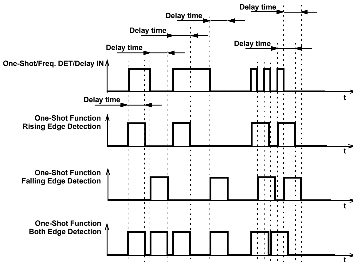
Figure 33. One-Shot Function Timing Diagram
