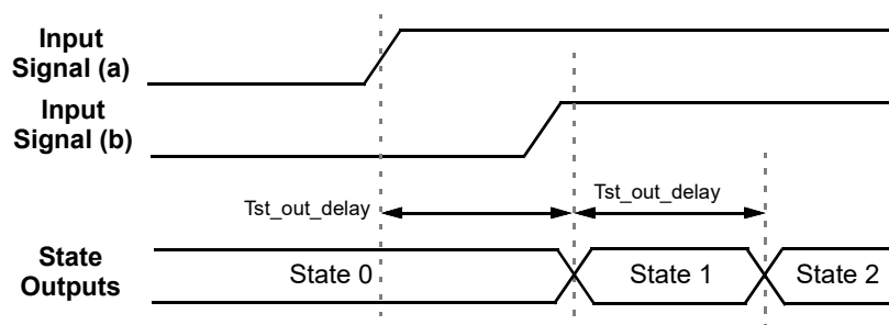
Figure 103. State Transition - Sequential Timing
