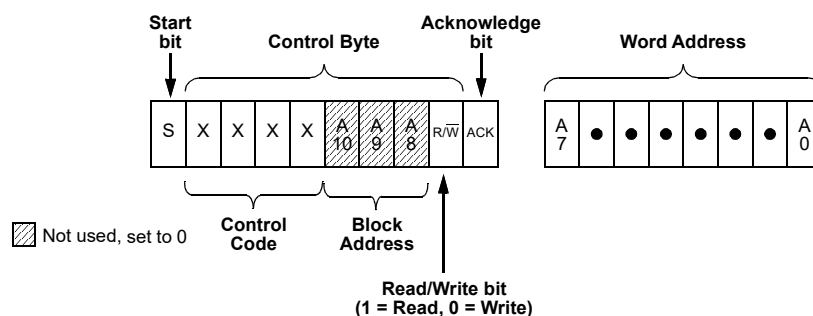
Figure 106. Basic Command Structure
