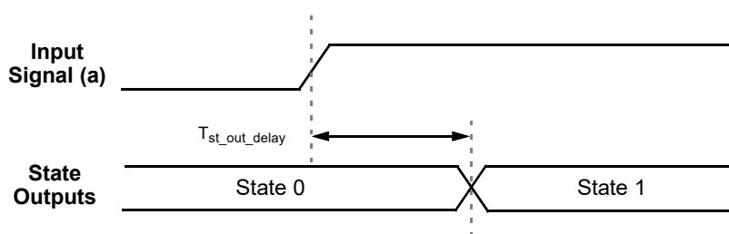
Figure 94. State Transition Timing
