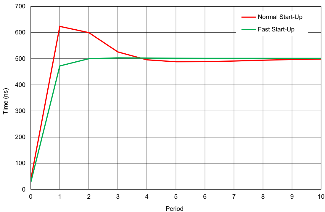
Figure 73. Oscillator0 Settling Time, V_{DD} = 3.3\text{ V} , T_A = +25\text{ }^{\circ}\text{C} , OSC0 = 2\text{ MHz}
