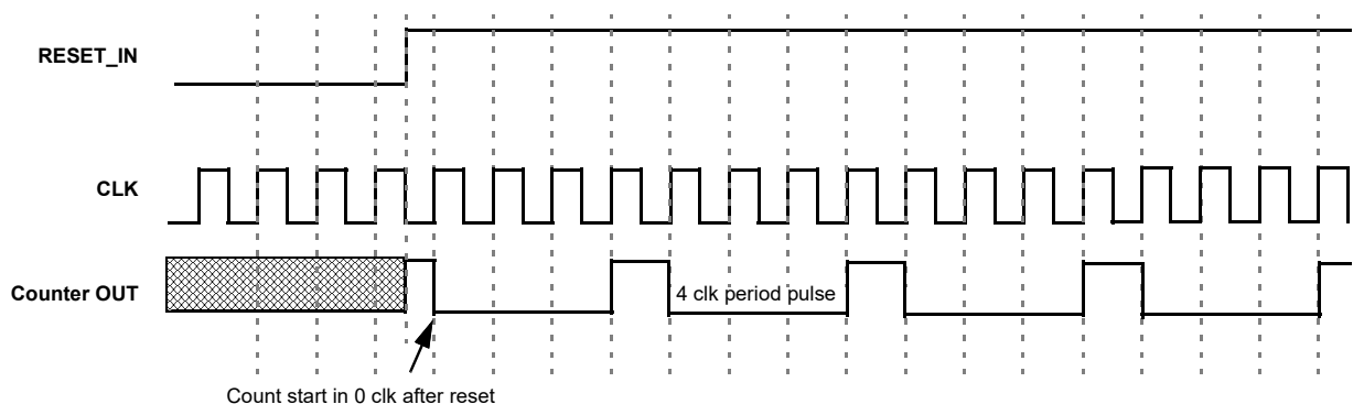
Figure 32. Counter Mode Timing Diagram
