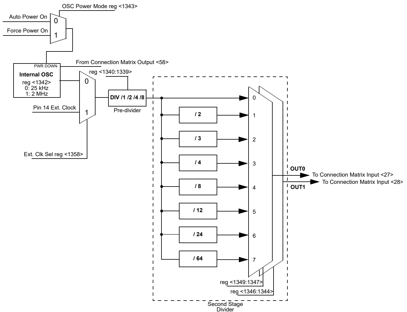
Figure 62. 25 kHz/2 MHz OSC0 Block Diagram
