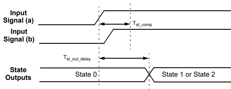
Figure 101. State Transition Timing - Competing Inputs Indeterminate
