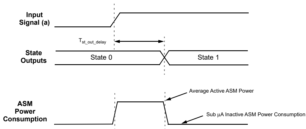
Figure 96. State Transition Timing and Power Consumption
