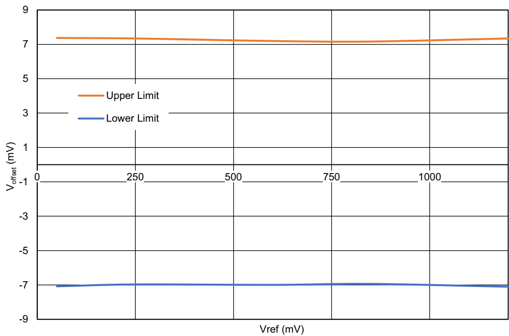
Figure 49. ACMPx Input Offset Voltage vs. V_{REF} at V_{DD} = 1.71\text{ V to }5.5\text{ V} , T_A = -40\text{ }^{\circ}\text{C to }+105\text{ }^{\circ}\text{C}
