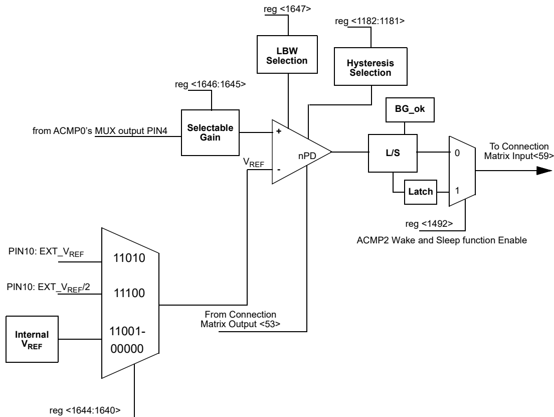
Figure 47. ACMP2 Block Diagram
