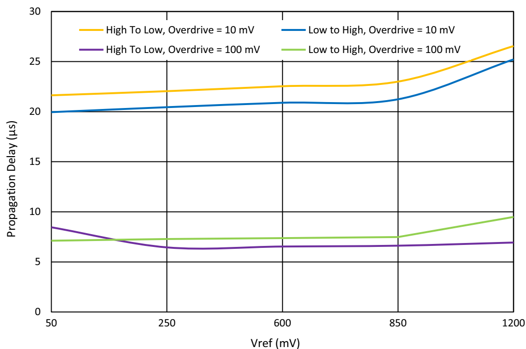
Figure 51. ACMPx Typical Propagation Delay at T_A = +25\text{ }^{\circ}\text{C} , Gain = 1, Hysteresis = 0, V_{DD} = 1.71\text{ V} to 5.5\text{ V} , LPF-Enable
