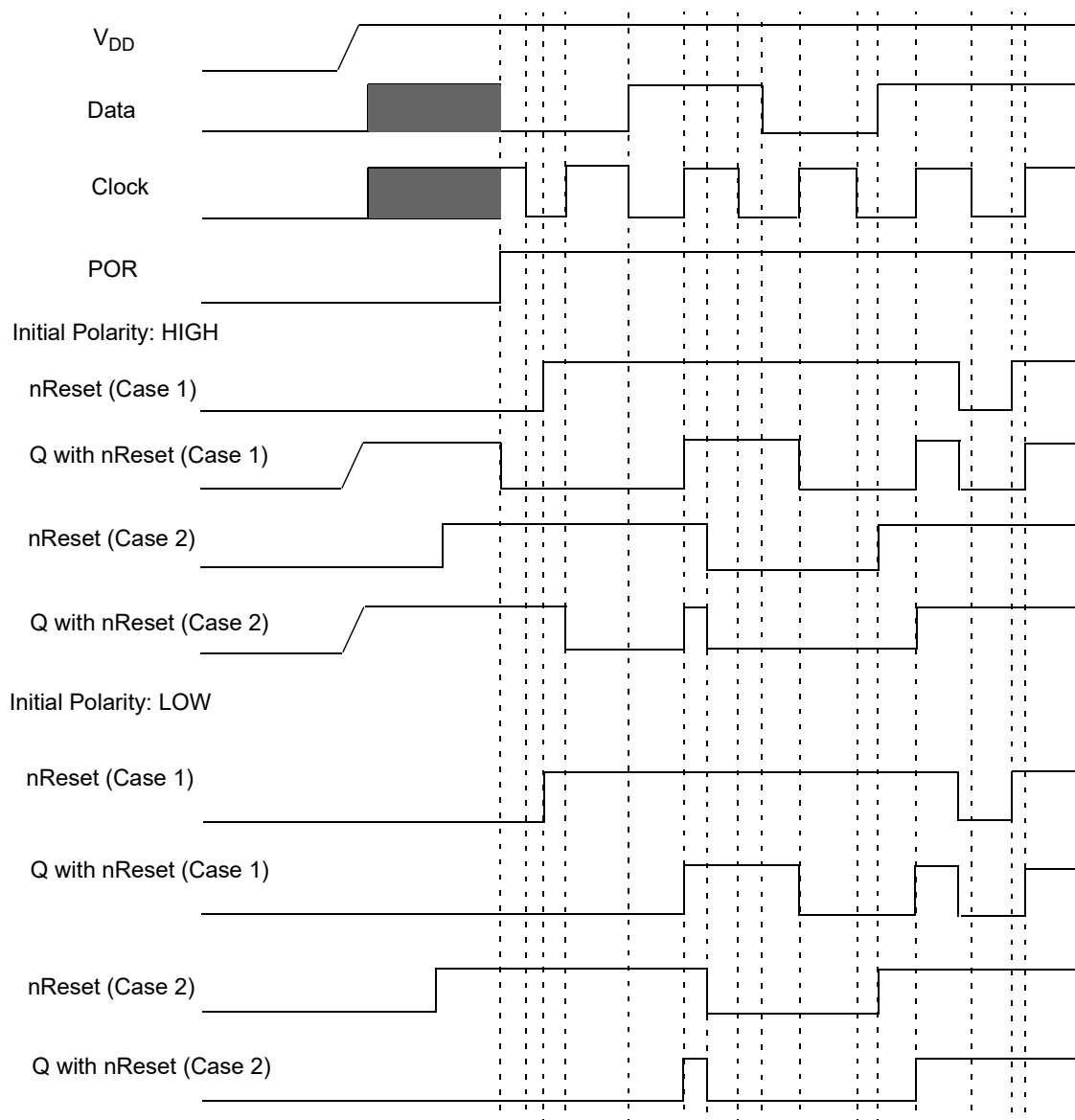
Figure 21. DFF Polarity Operations with n\text{Reset}
