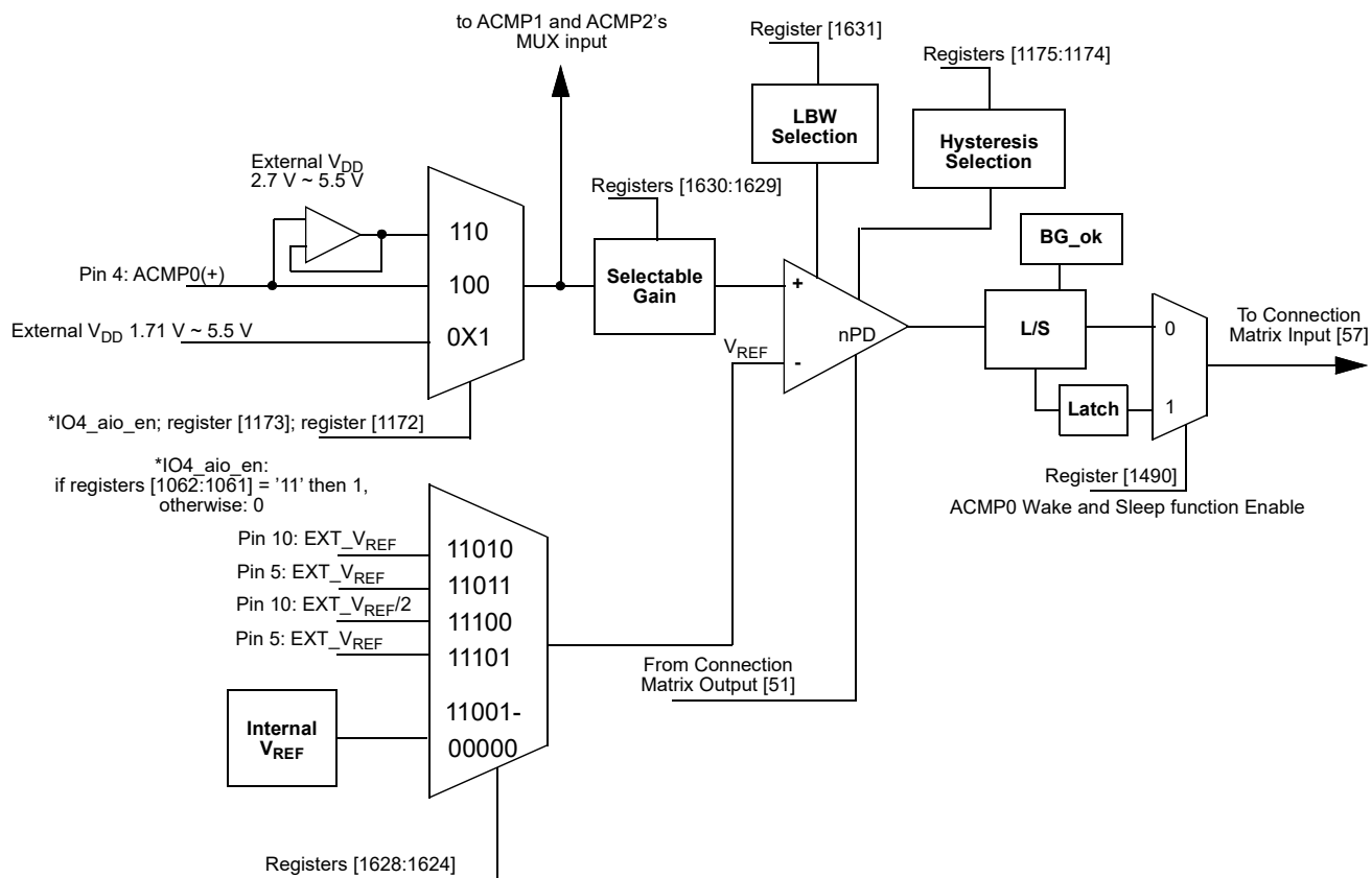
Figure 45. ACMP0 Block Diagram
