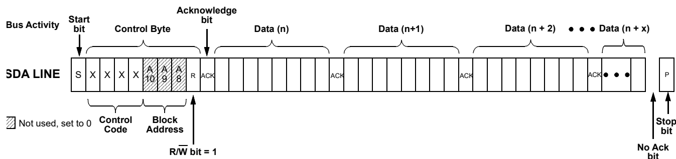
Figure 112. Sequential Read Command
