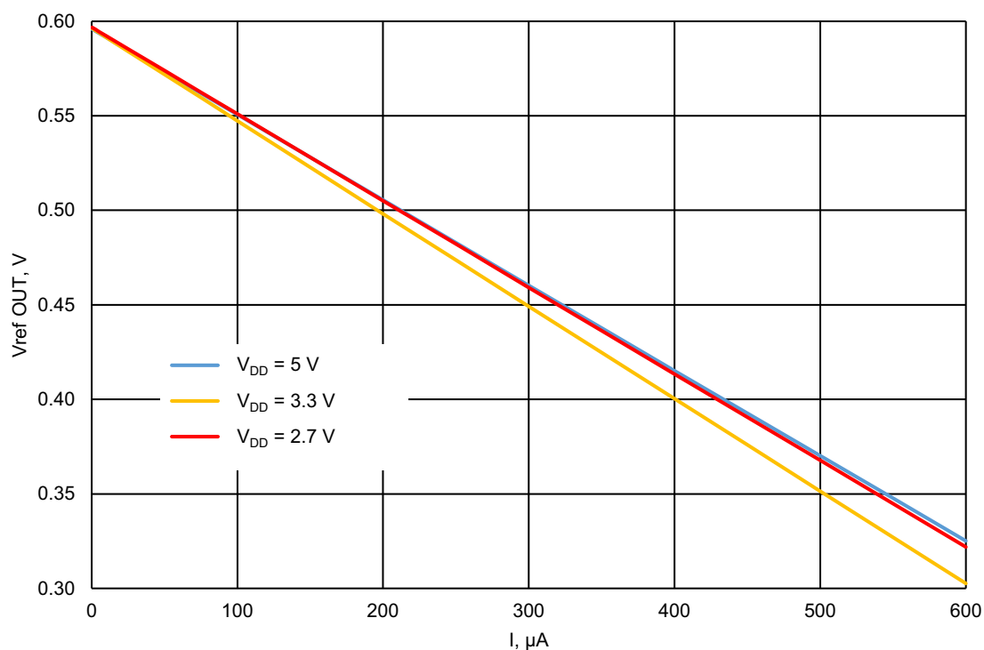
Figure 59. Typical Load Regulation, V_{REF} = 600 mV, T_A = -40 °C to +105 °C, Buffer - Enable
