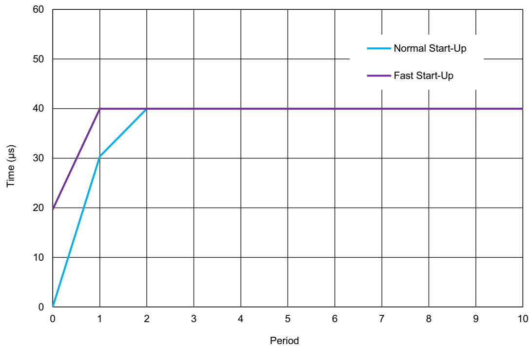
Figure 72. Oscillator0 Settling Time, V_{DD} = 3.3\text{ V} , T_A = +25\text{ }^{\circ}\text{C} , OSC0 = 25\text{ kHz}
