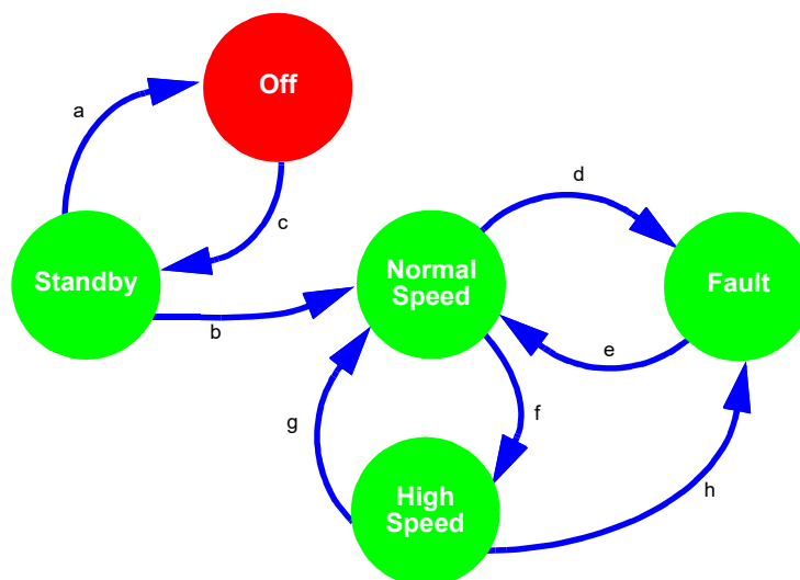
Figure 87. Asynchronous State Machine State Transitions
