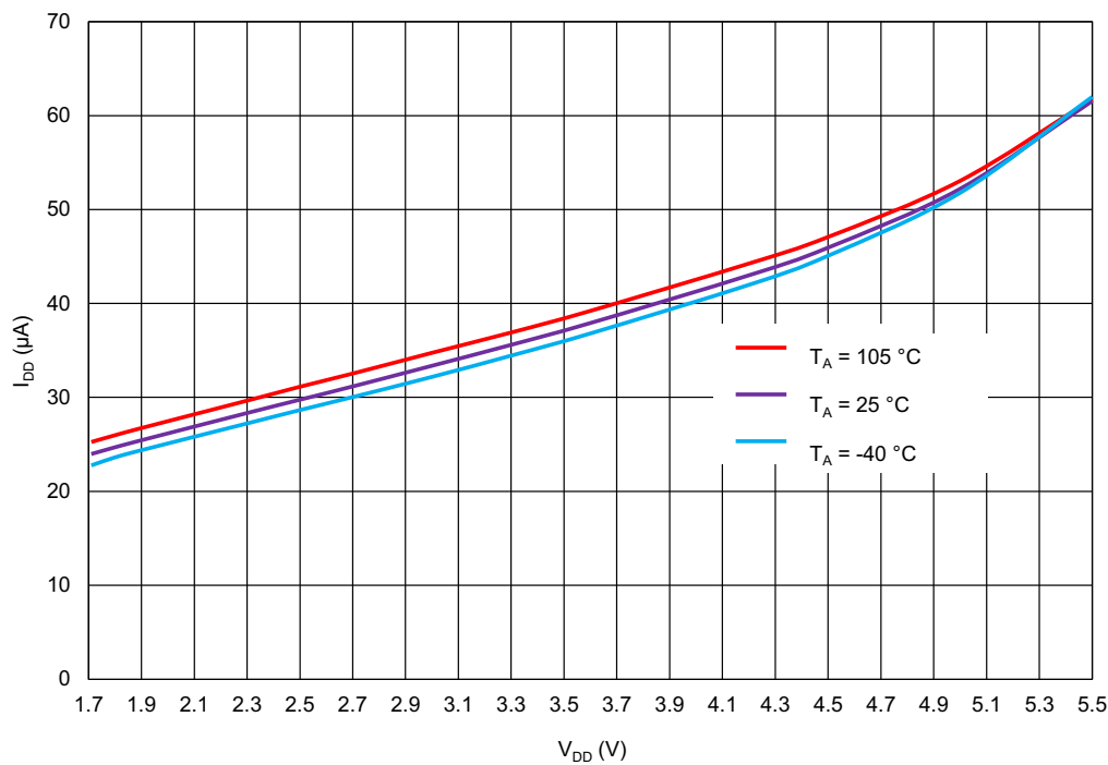
Figure 77. OSC0 (2 MHz) Current Consumption vs. V DD , Pre-Divider = 2
