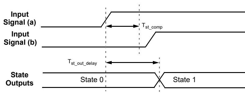
Figure 100. State Transition Timing - Competing Inputs Determinable
