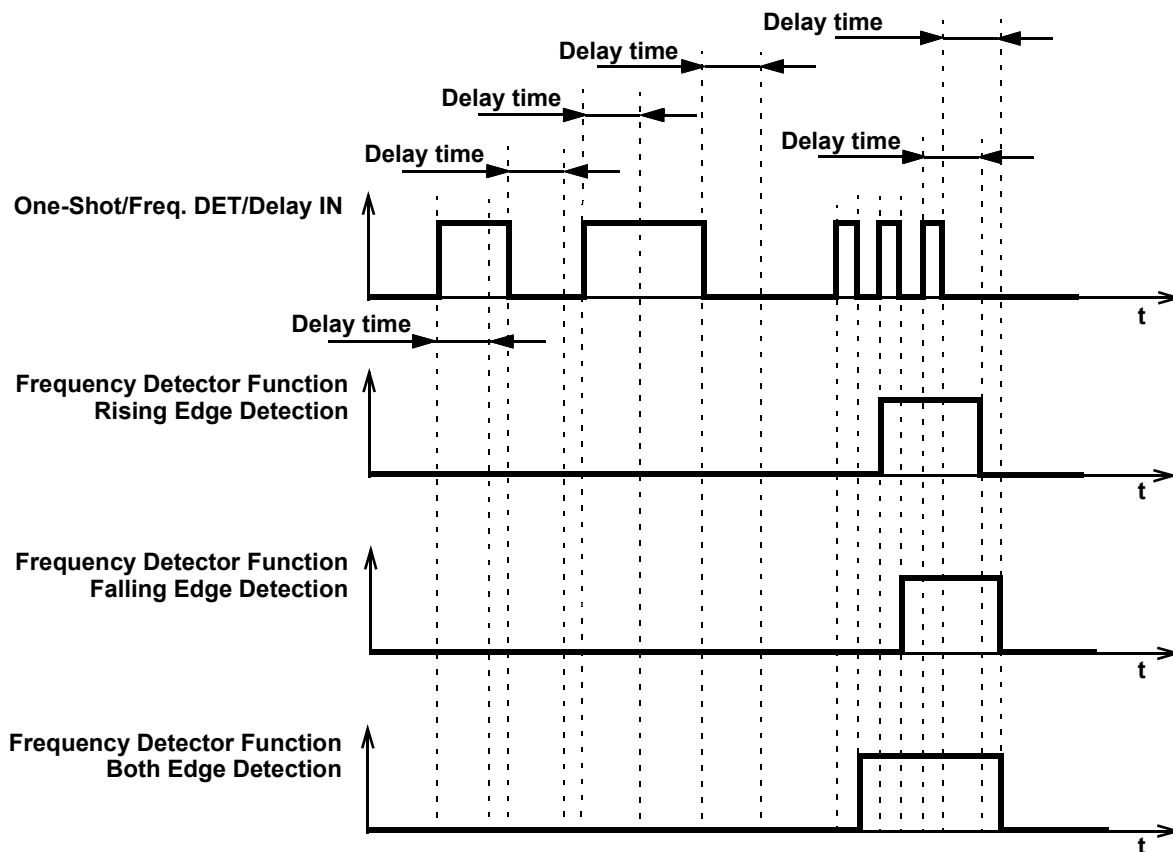
Figure 34. Frequency Detection Mode Timing Diagram
