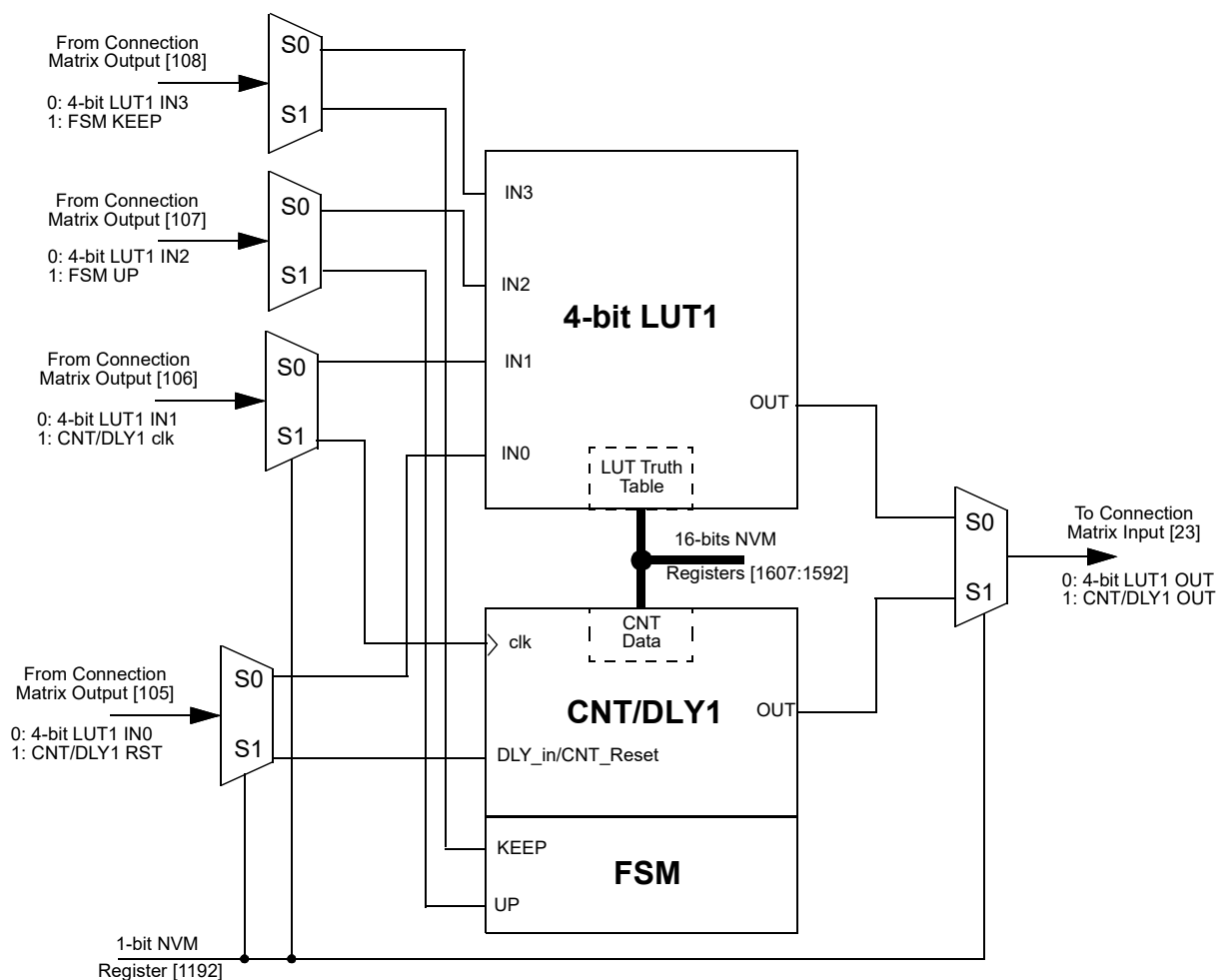
Figure 38. 4-bit LUT1 or CNT/DLY1
