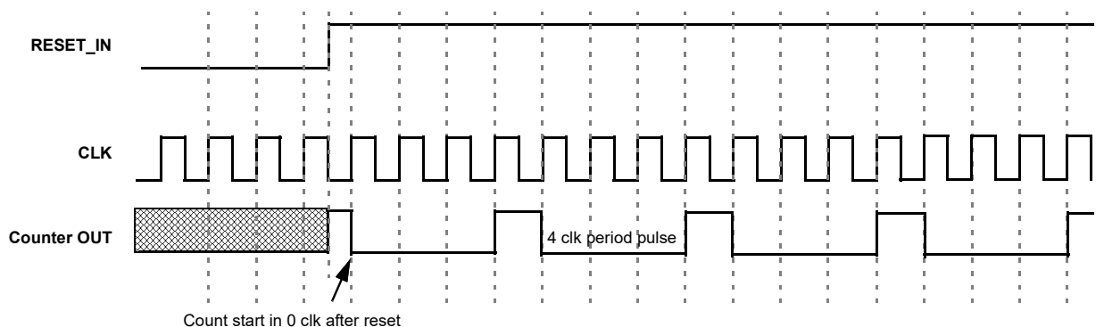
Figure 40. Counter Mode Timing Diagram
