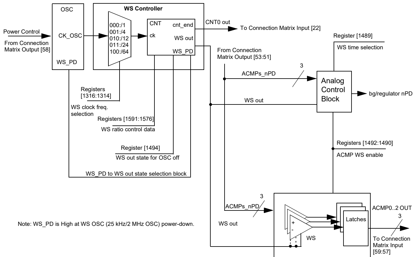
Figure 52. Wake/Sleep Controller
