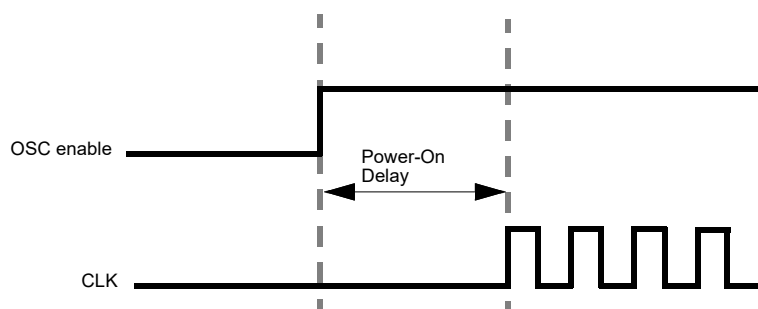
Figure 73. Oscillator Startup Diagram
