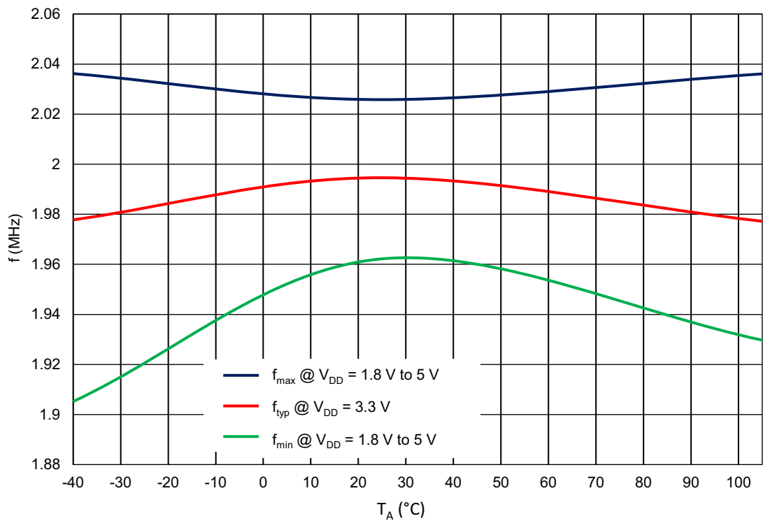
Figure 78. Oscillator Frequency vs. Ambient Temperature, OSC0 = 2 MHz
