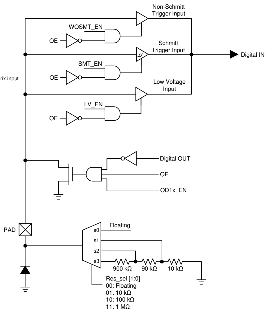
Figure 7. Matrix OE IO Structure Diagram
