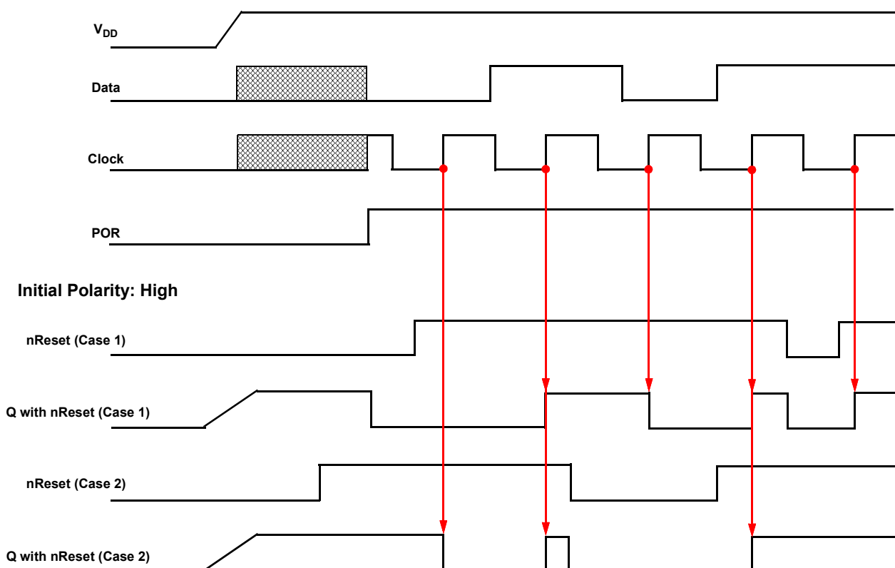
Figure 30. DFF Polarity Operations
