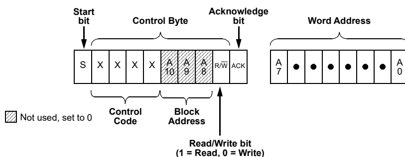
Figure 115. Basic Command Structure
