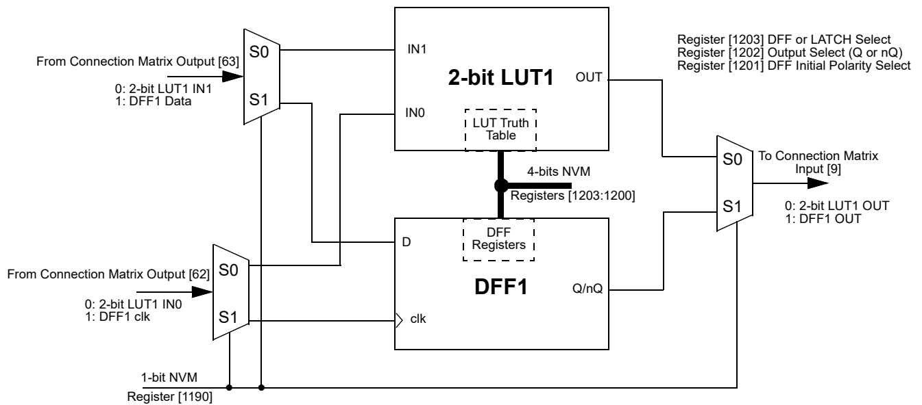
Figure 15. 2-bit LUT1 or DFF1
