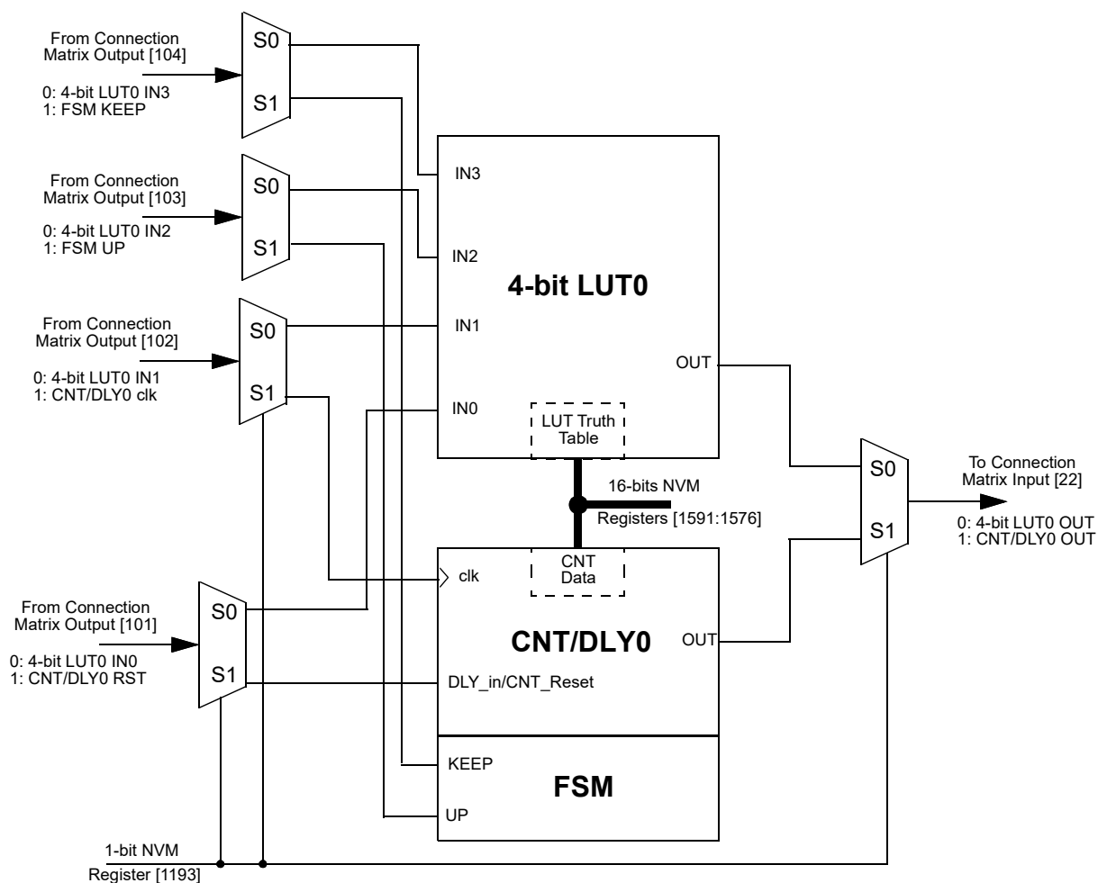
Figure 37. 4-bit LUT0 or CNT/DLY0
