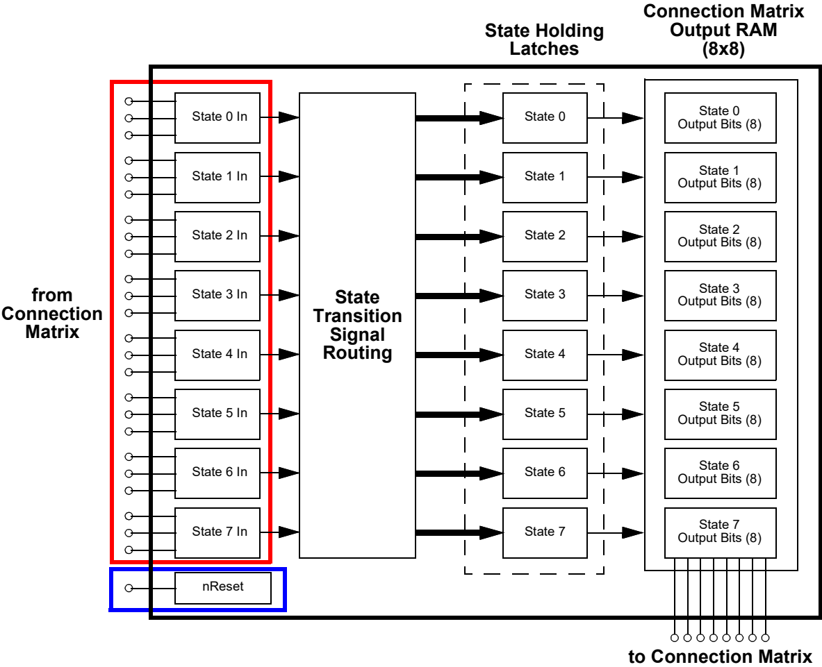
Figure 98. Asynchronous State Machine Inputs
