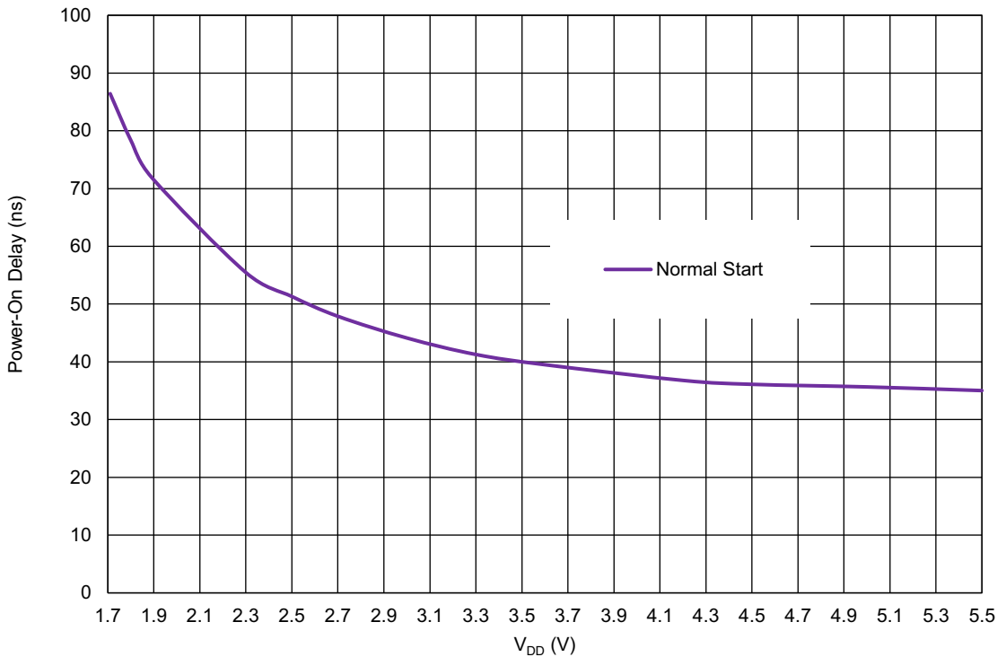
Figure 76. Oscillator Maximum Power-On Delay vs. V DD at T A = +25 °C, OSC1 = 25 MHz
