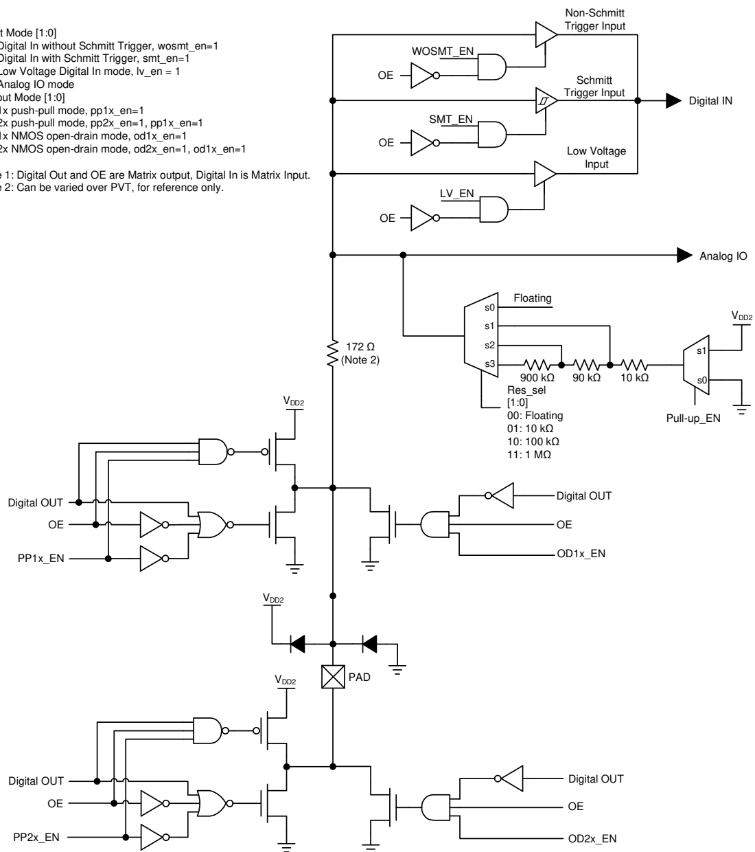
Figure 6. Matrix OE IO Structure Diagram
