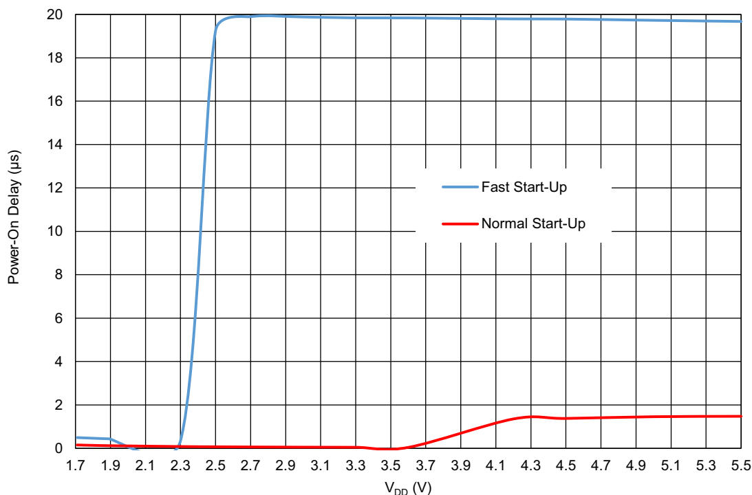
Figure 74. Oscillator Maximum Power-On Delay vs. V_{DD} at T_A = +25\text{ }^{\circ}\text{C} , OSC0 = 25 kHz
