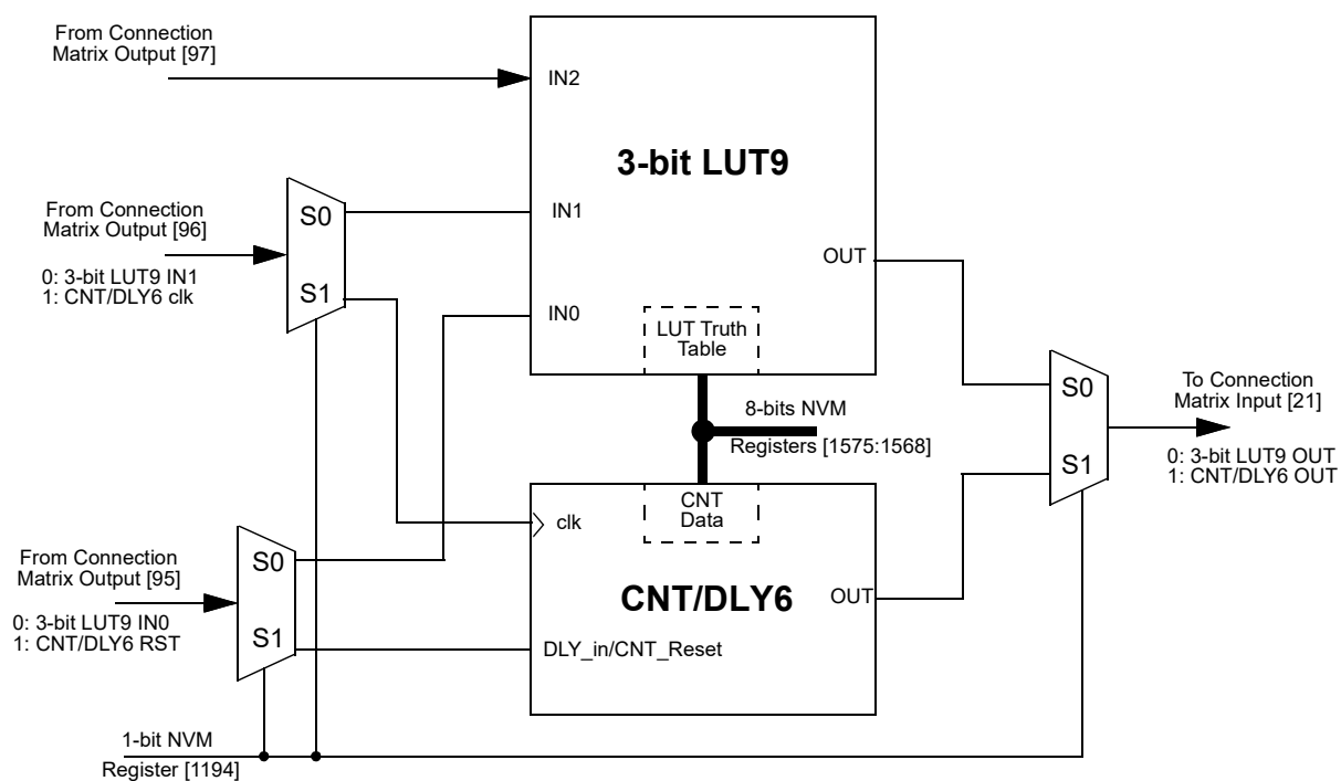
Figure 36. 3-bit LUT9 or CNT/DLY6
