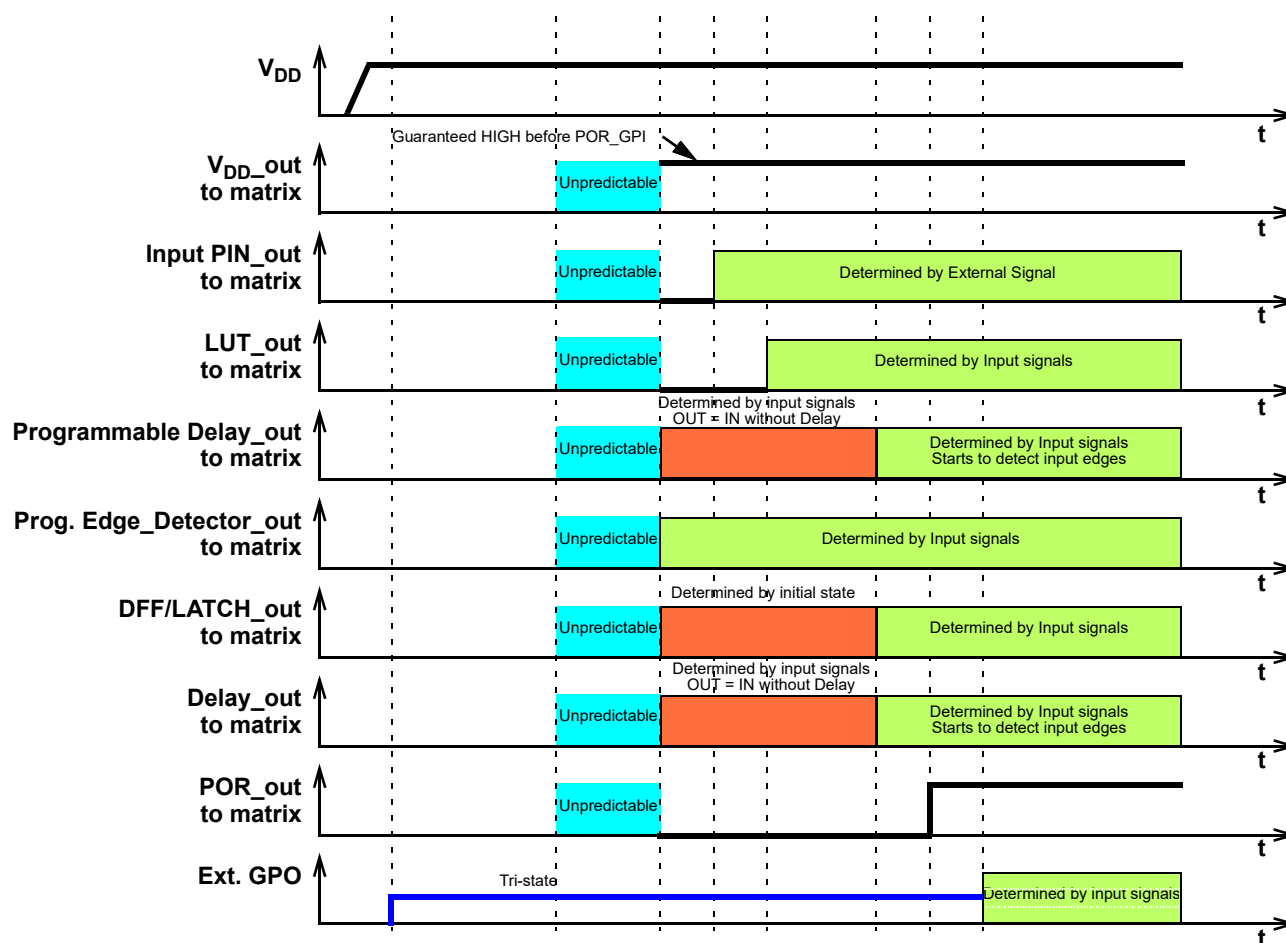
Figure 94. Internal Macrocell States during POR Sequence
