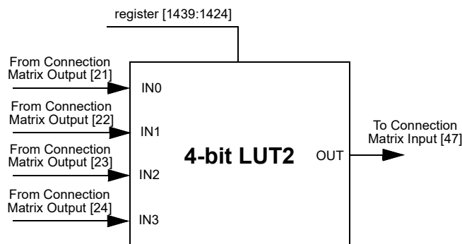
Figure 52. 4-bit LUT2
