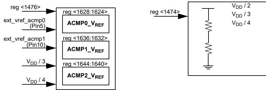
Figure 66. Voltage Reference Block Diagram
