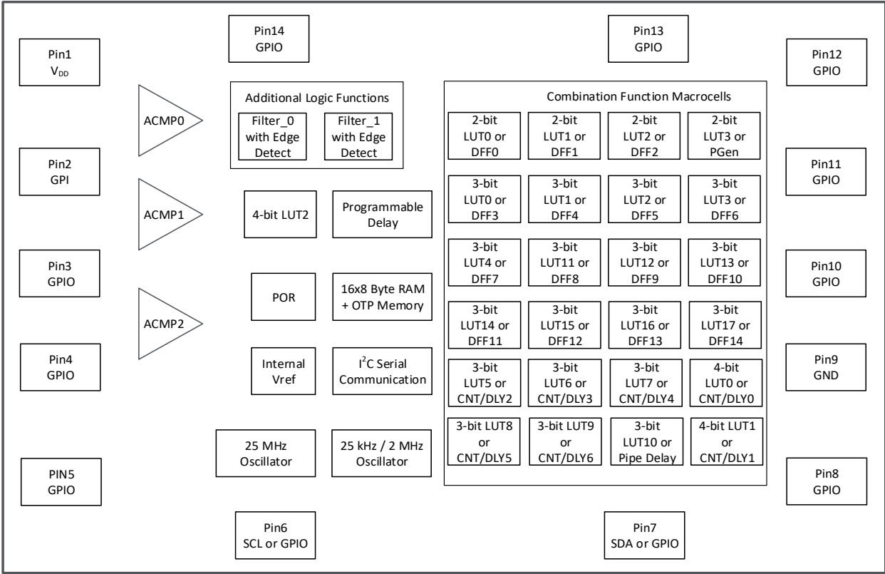
Figure 1. Block Diagram
