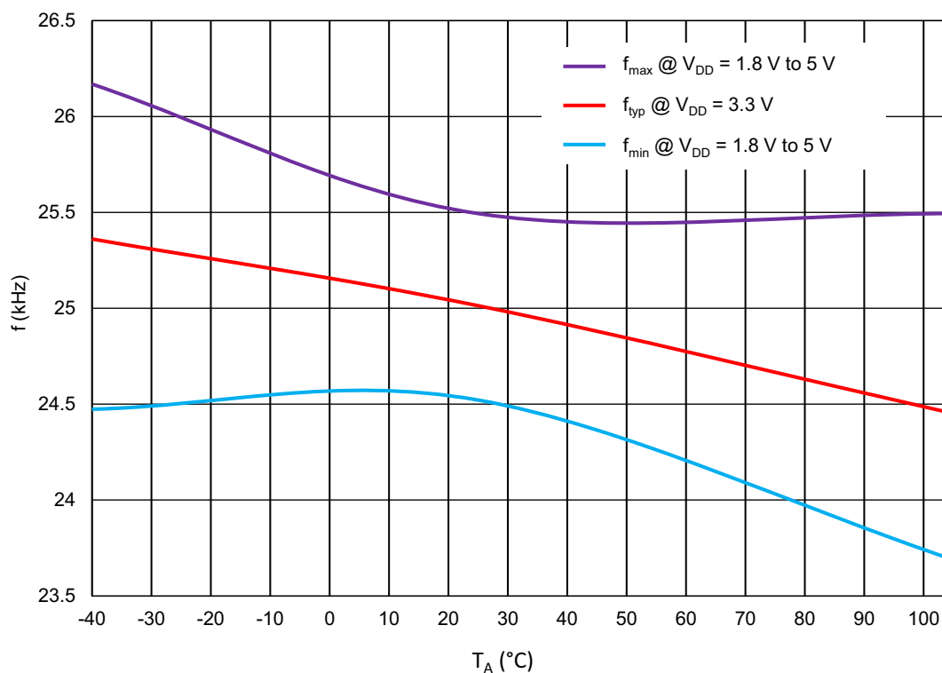
Figure 76. Oscillator Frequency vs. Ambient Temperature, OSC0 = 25 kHz
