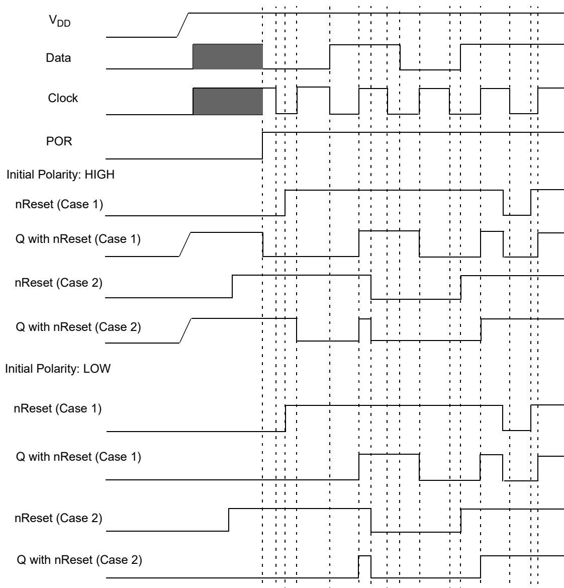
Figure 28. DFF Polarity Operations with n\text{Reset}
