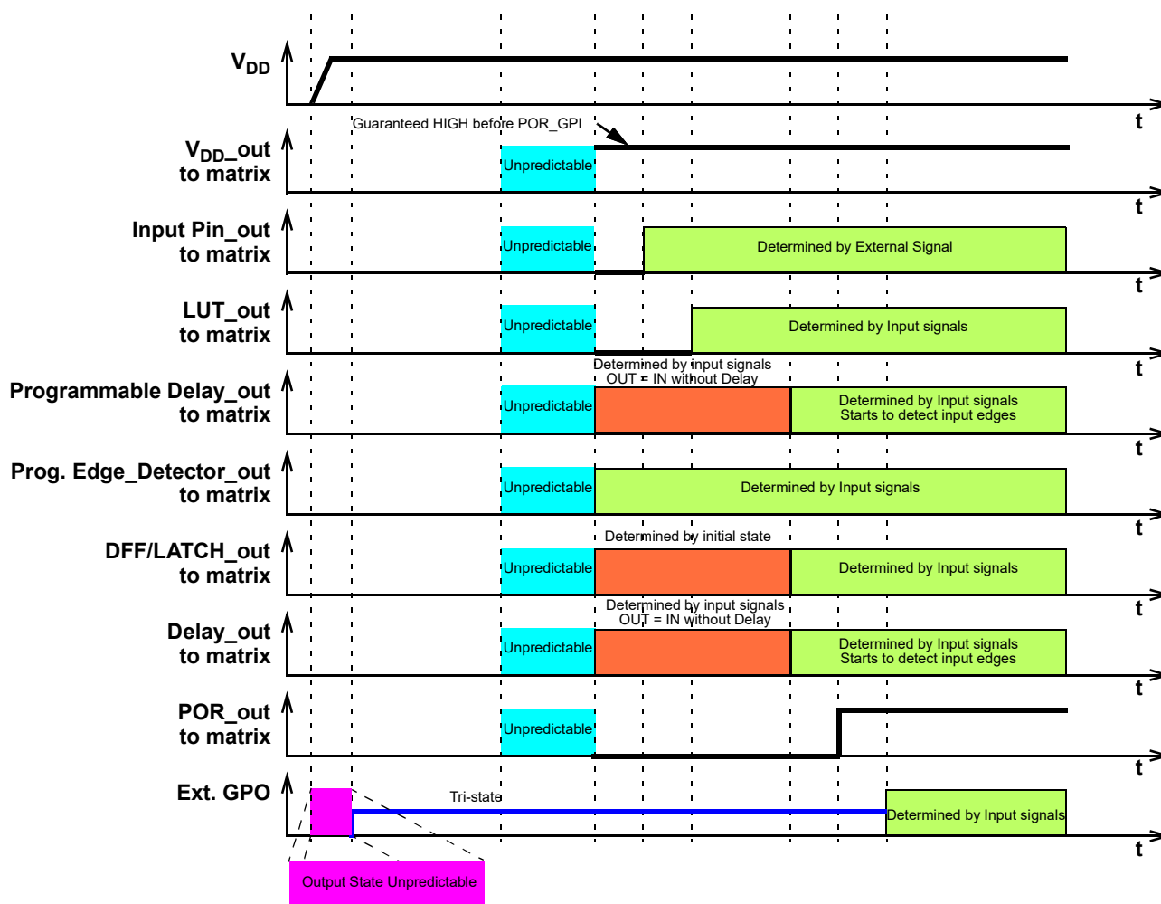
Figure 93. Internal Macrocell States during POR Sequence
