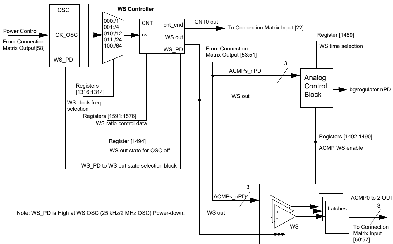
Figure 51. Wake/Sleep Controller
