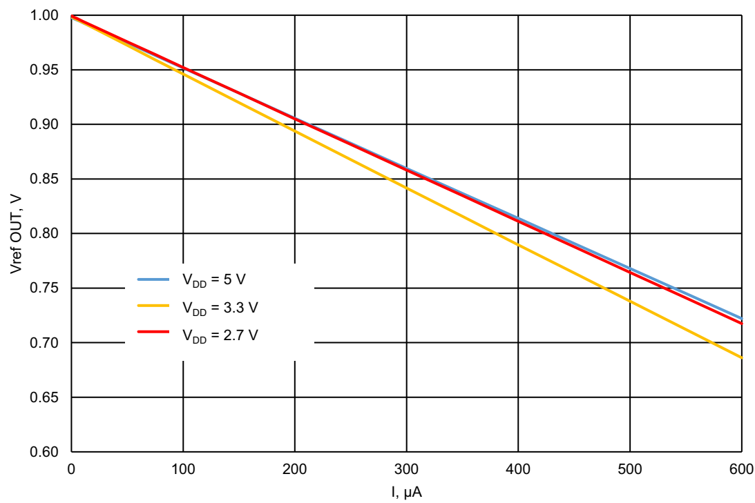
Figure 69. Typical Load Regulation, V_{REF} = 1200\ mV , T_A = -40\ ^\circ C to +105\ ^\circ C , Buffer - Enable
