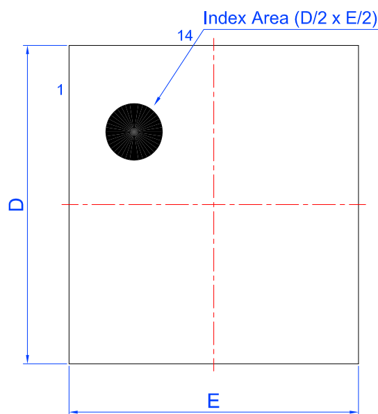
Top View (package face down)
