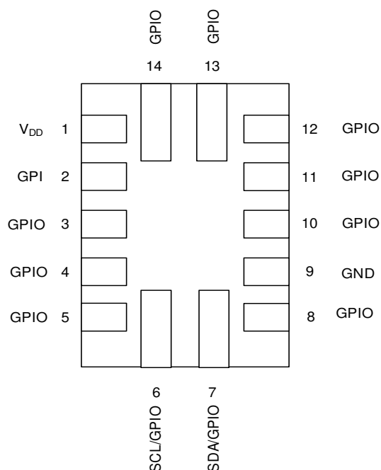
Figure 2. Pin Assignments - STQFN-14 (Top View)
