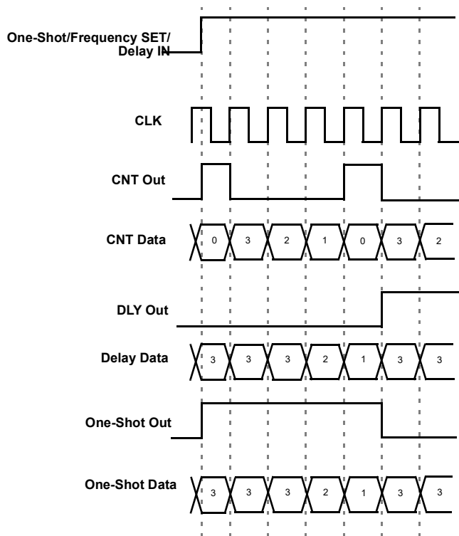
Figure 48. Counter Value, Counter Data = 3
