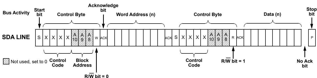
Figure 118. Random Read Command
