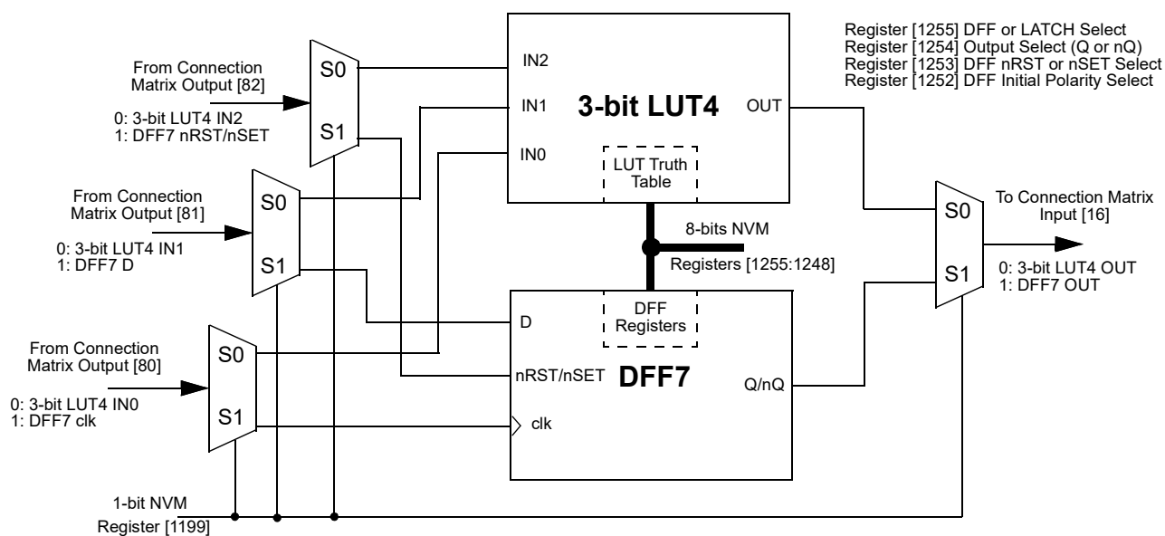
Figure 20. 3-bit LUT4 or DFF7 with RST/SET
