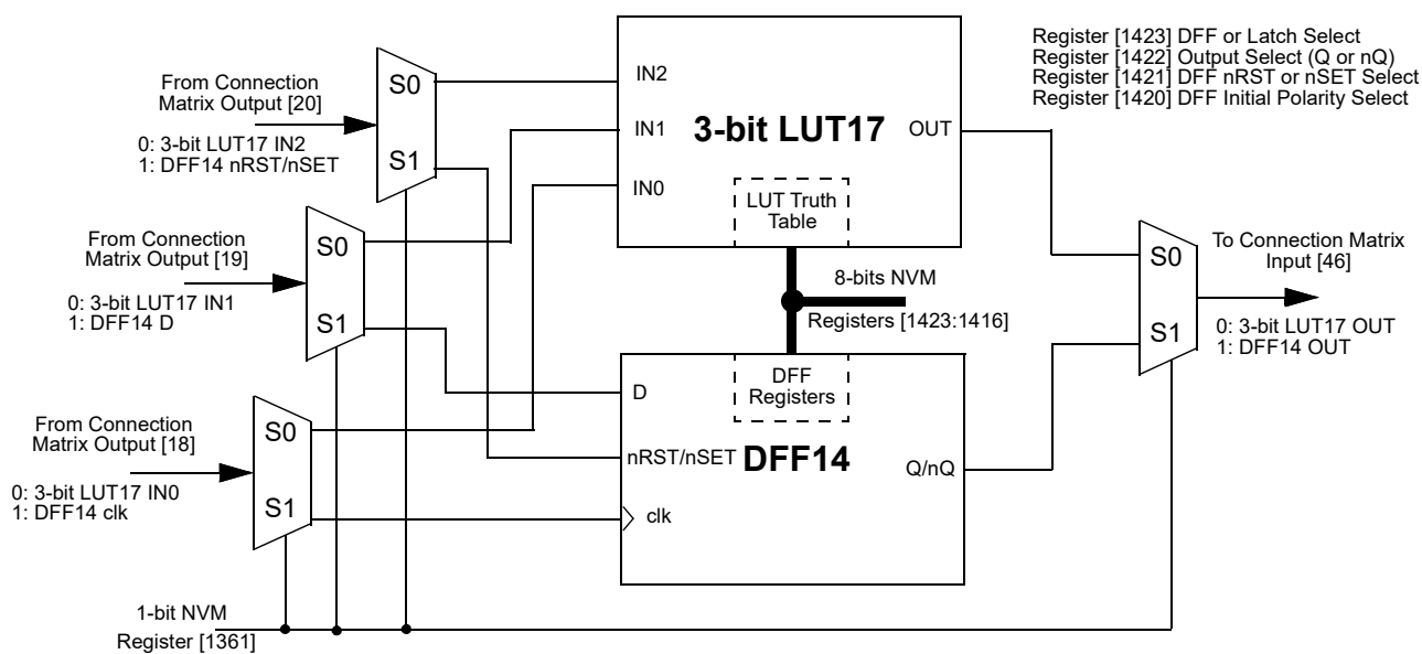
Figure 27. 3-bit LUT17 or DFF14 with RST/SET
