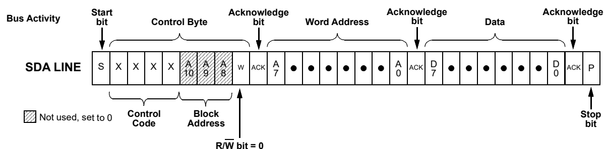
Figure 115. Byte Write Command, \overline{R/W} = 0
