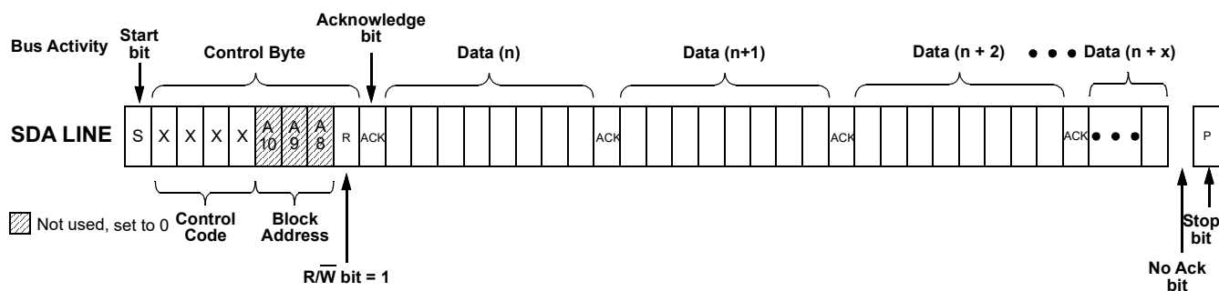
Figure 119. Sequential Read Command
