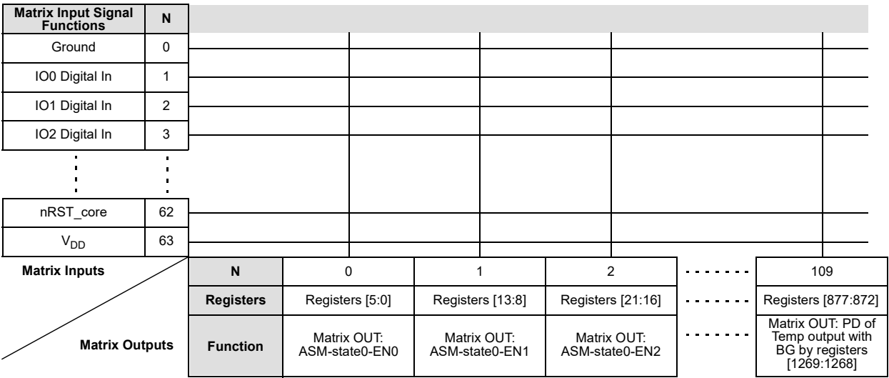
Figure 10. Connection Matrix
