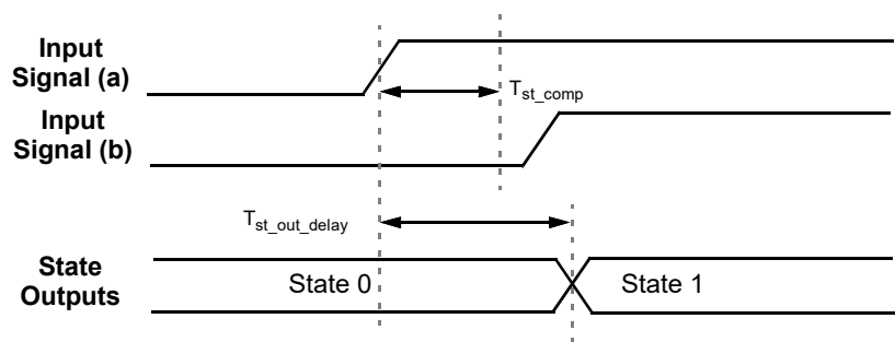
Figure 108. State Transition Timing - Competing Inputs Determinable
