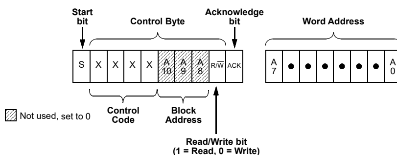
Figure 113. Basic Command Structure
