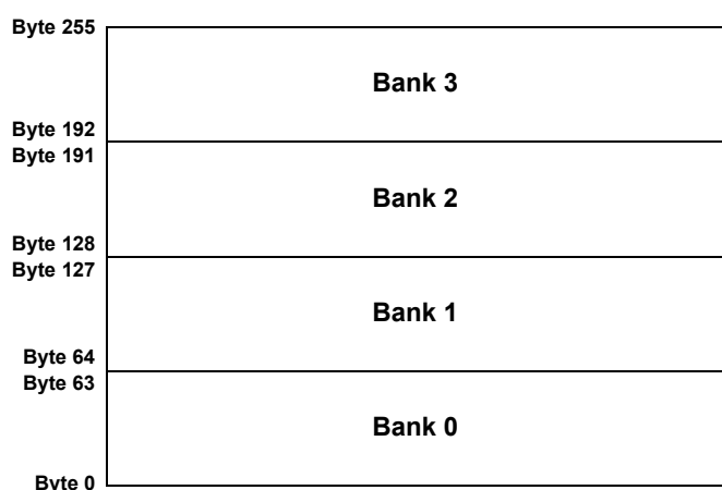
Figure 120. Register Bank Map
