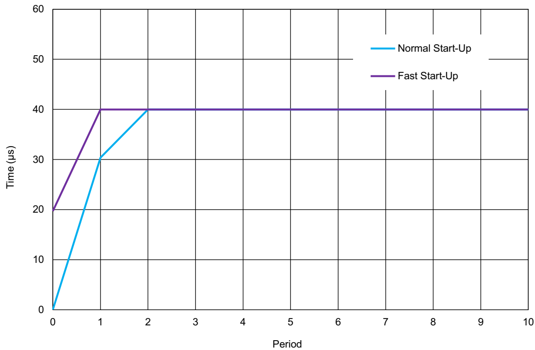
Figure 80. Oscillator0 Settling Time, V_{DD} = 3.3\text{ V} , T_A = +25\text{ }^{\circ}\text{C} , OSC0 = 25\text{ kHz}
