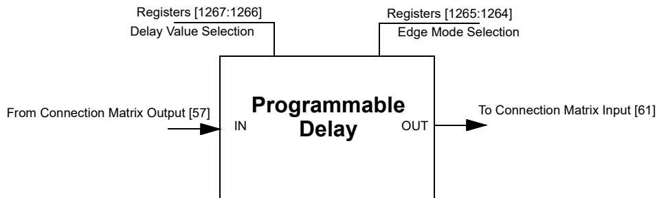
Figure 63. Programmable Delay
