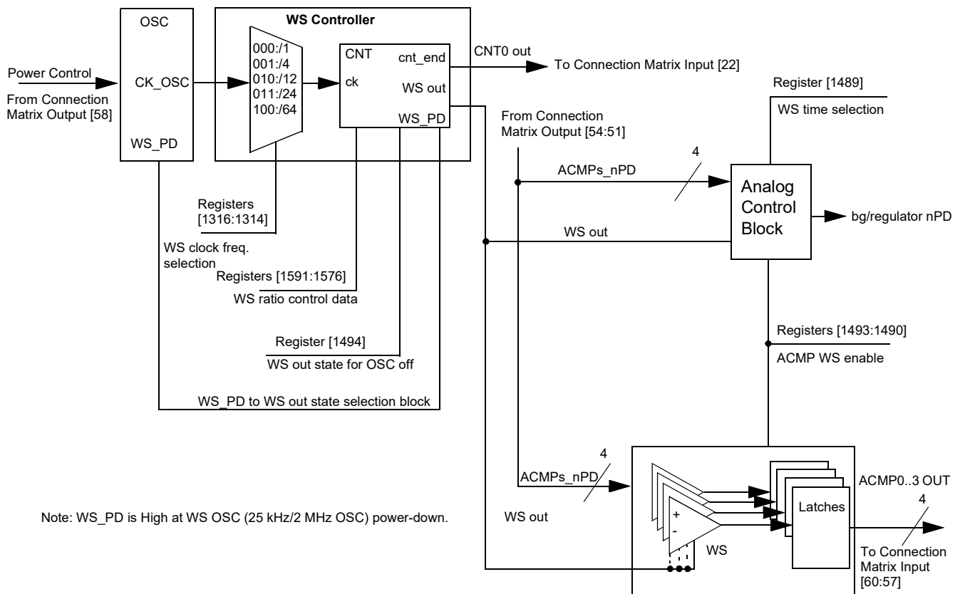
Figure 51. Wake/Sleep Controller
