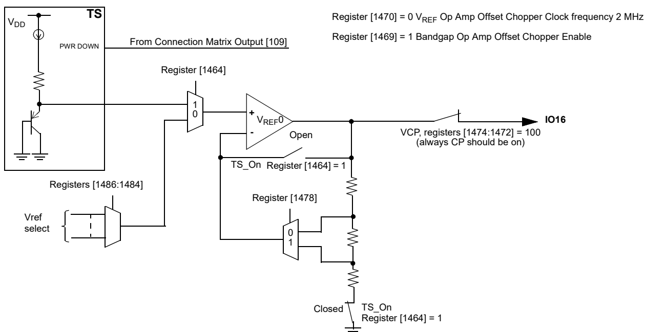
Figure 122. Analog Temperature Sensor Structure Diagram
