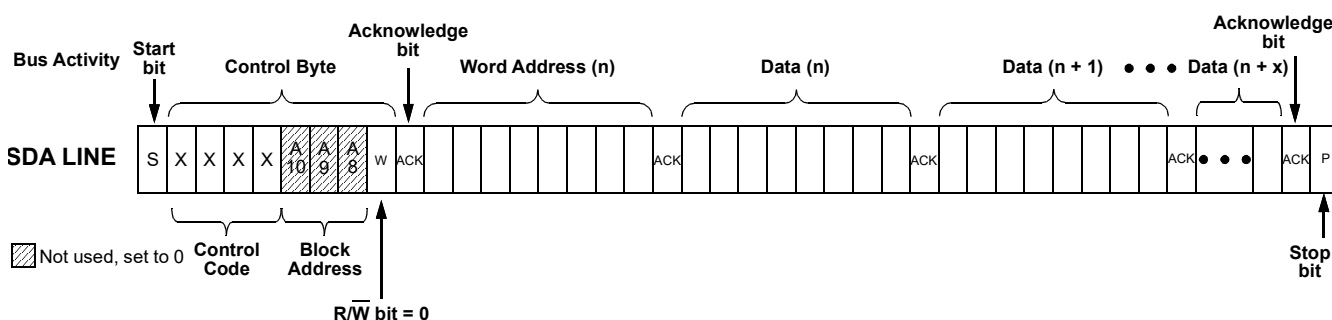
Figure 116. Sequential Write Command, \overline{R/W} = 0
