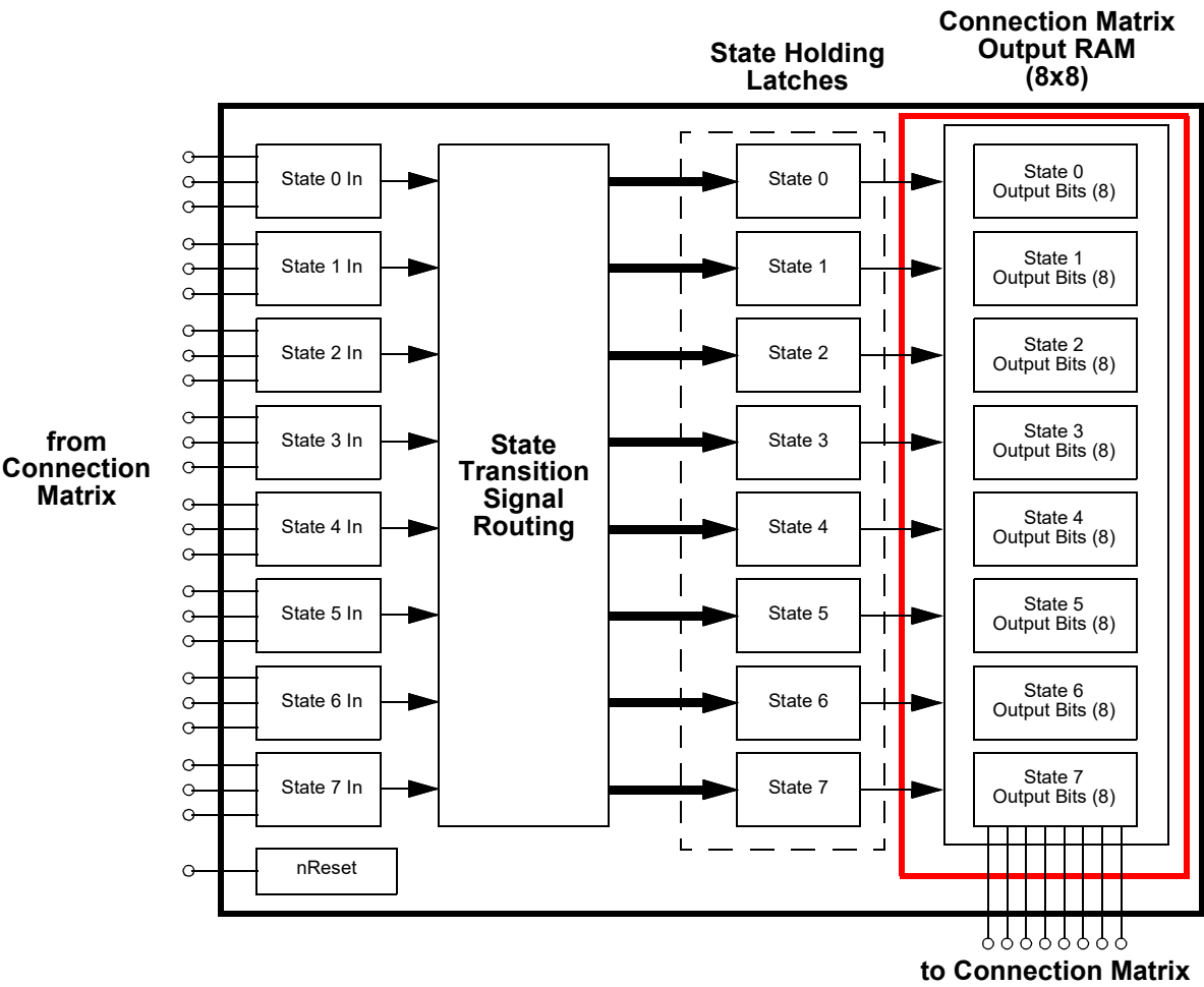
Figure 100. Connection Matrix Output RAM
