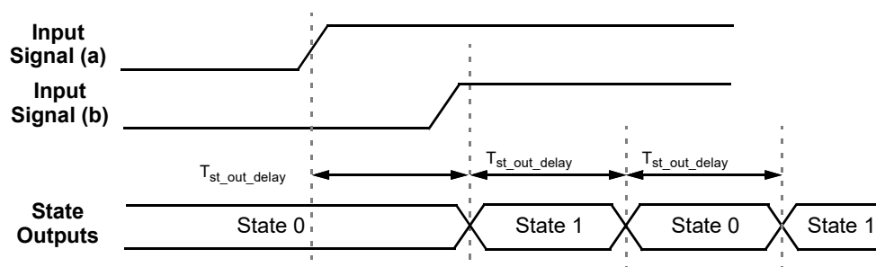
Figure 112. State Transition - Closed Cycling Timing
