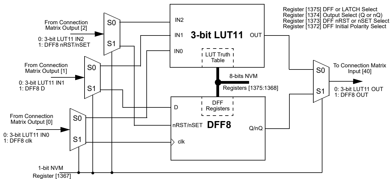
Figure 21. 3-bit LUT11 or DFF8 with RST/SET
