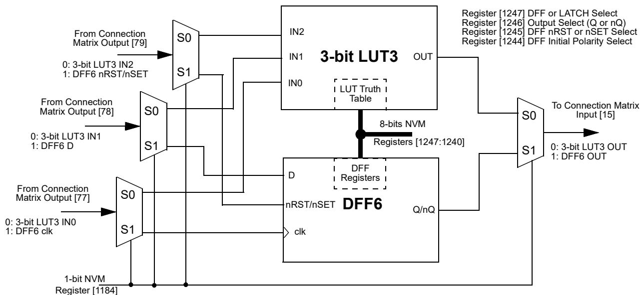
Figure 21. 3-bit LUT3 or DFF6 with RST/SET
