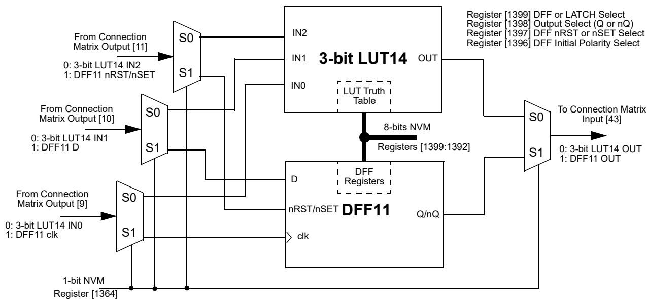
Figure 26. 3-bit LUT14 or DFF11 with RST/SET
