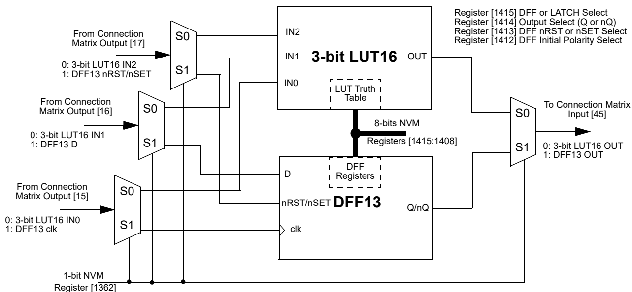
Figure 28. 3-bit LUT16 or DFF13 with RST/SET
