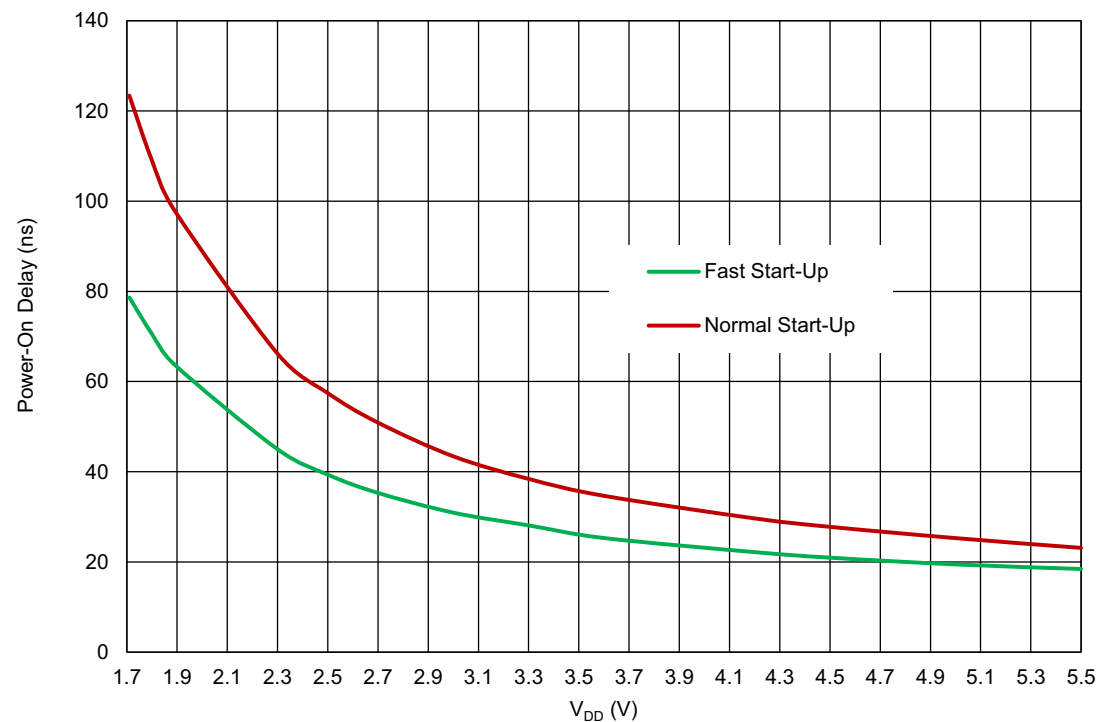
Figure 76. Oscillator Maximum Power-On Delay vs. V DD at T A = +25 °C, OSC0 = 2 MHz
