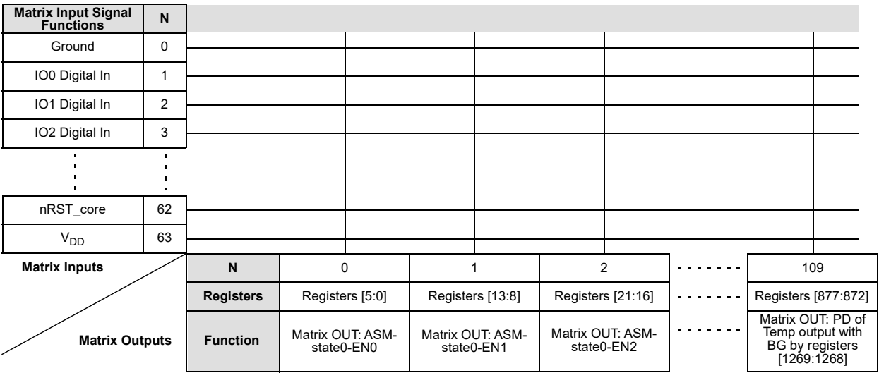
Figure 12. Connection Matrix
