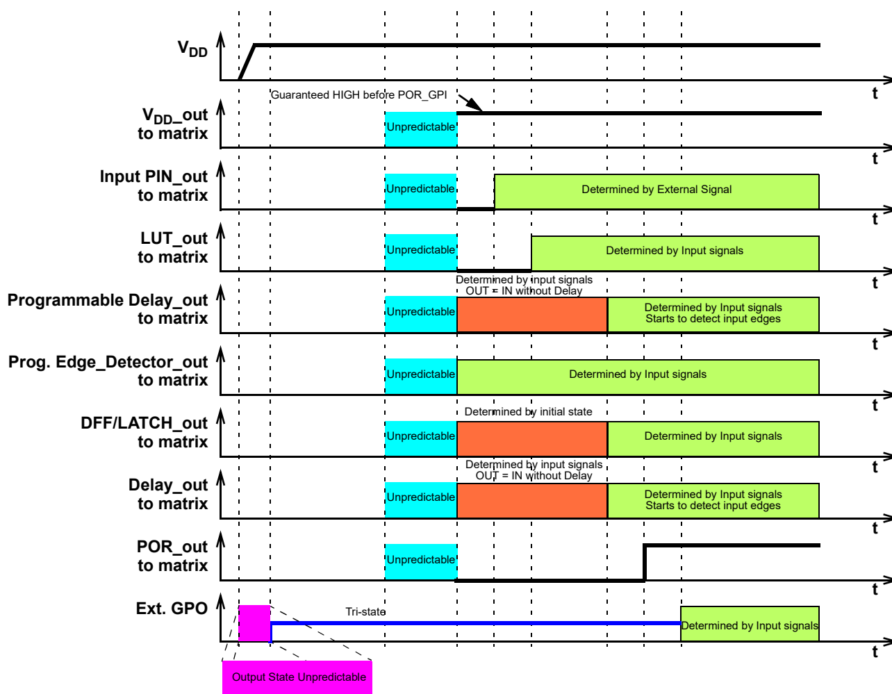
Figure 95. Internal Macrocell States during POR Sequence
