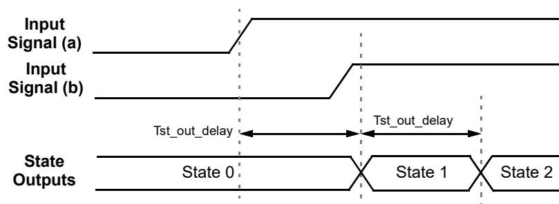
Figure 113. State Transition - Sequential Timing
