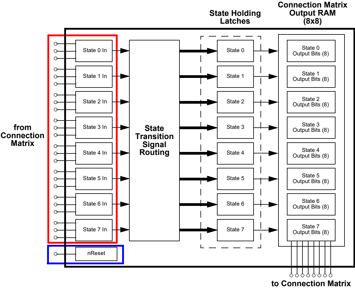
Figure 99. Asynchronous State Machine Inputs
