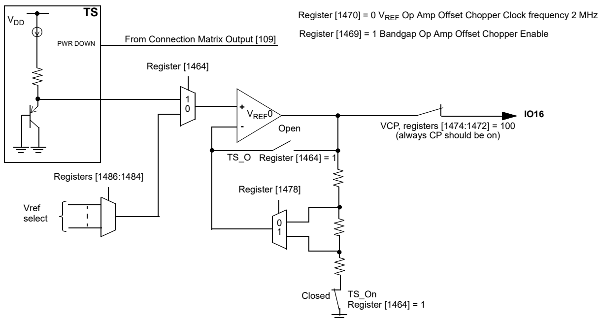
Figure 125. Analog Temperature Sensor Structure Diagram
