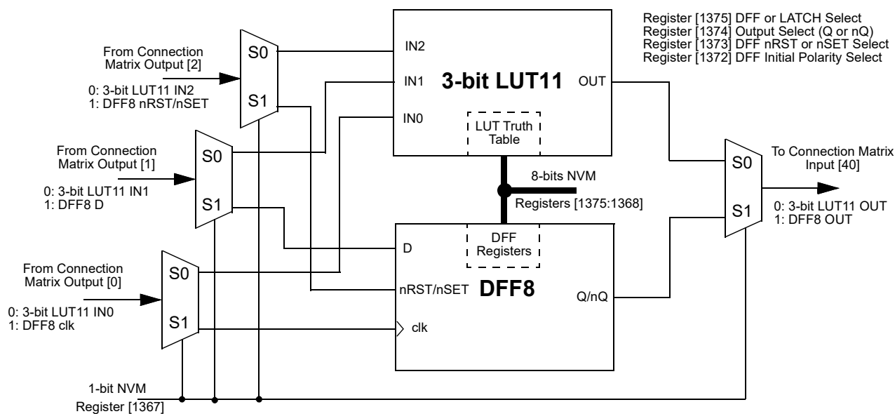
Figure 23. 3-bit LUT11 or DFF8 with RST/SET
