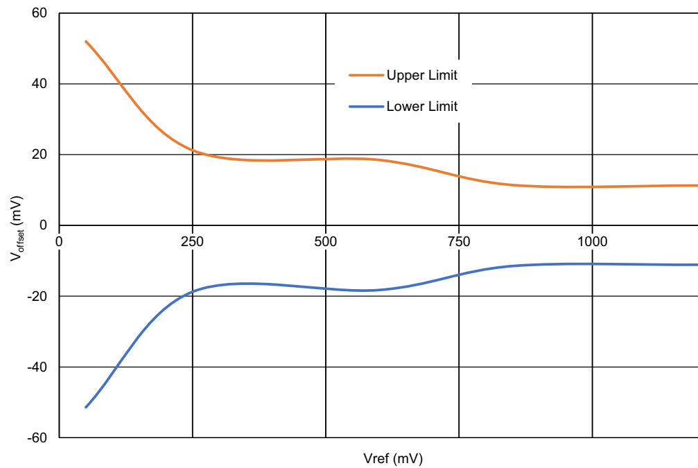
Figure 59. ACMPx Buffer Input Offset Voltage vs. V_{REF} at V_{DD} = 1.71\text{ V to }5.5\text{ V} , T_A = -40\text{ }^{\circ}\text{C to }+105\text{ }^{\circ}\text{C}
