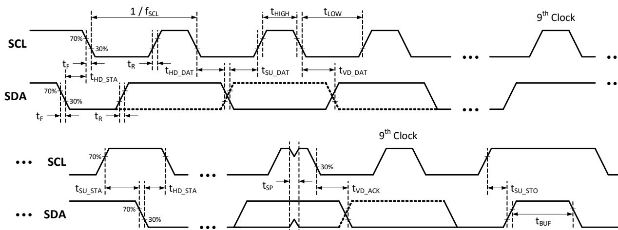
Figure 117. I 2 C General Timing Characteristics
