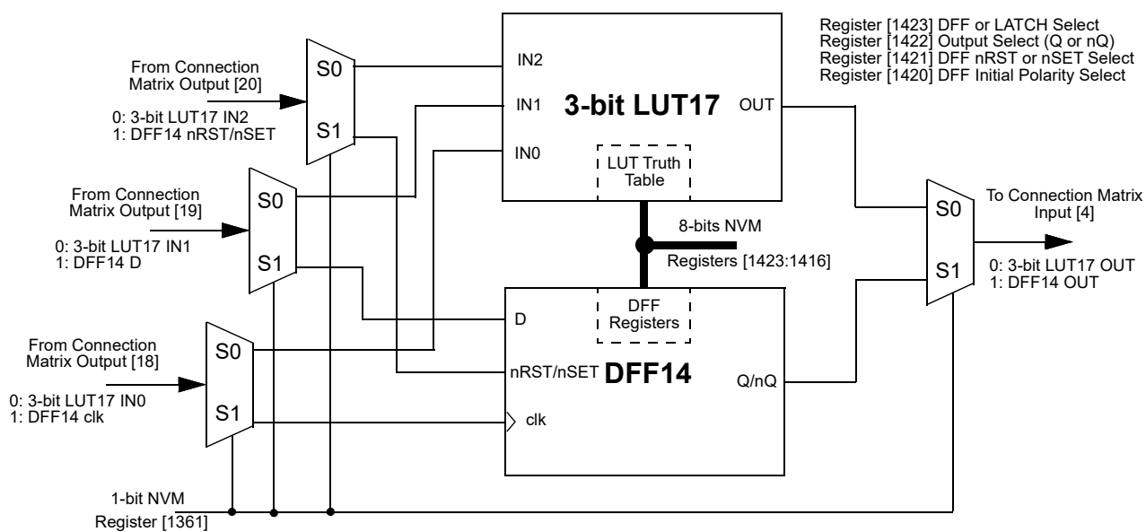
Figure 29. 3-bit LUT17 or DFF14 with RST/SET
