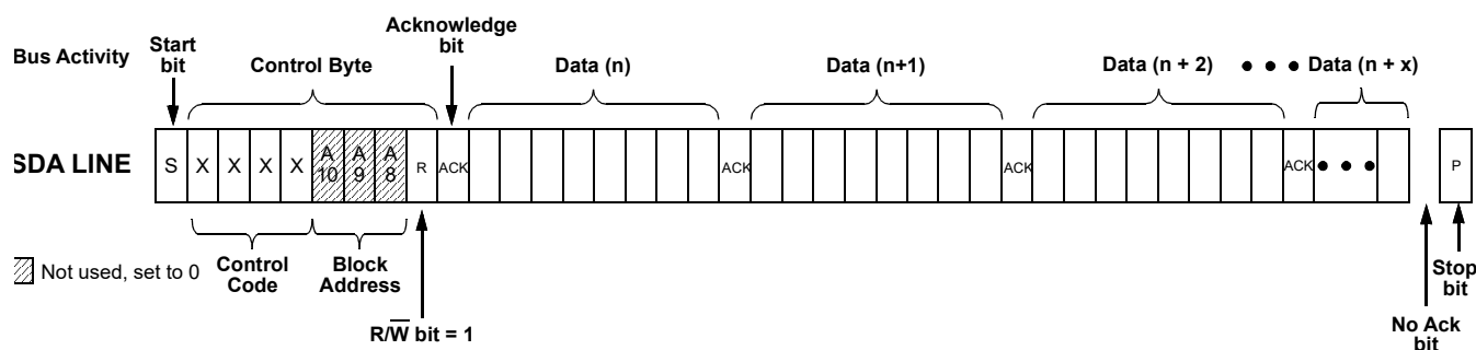
Figure 122. Sequential Read Command
