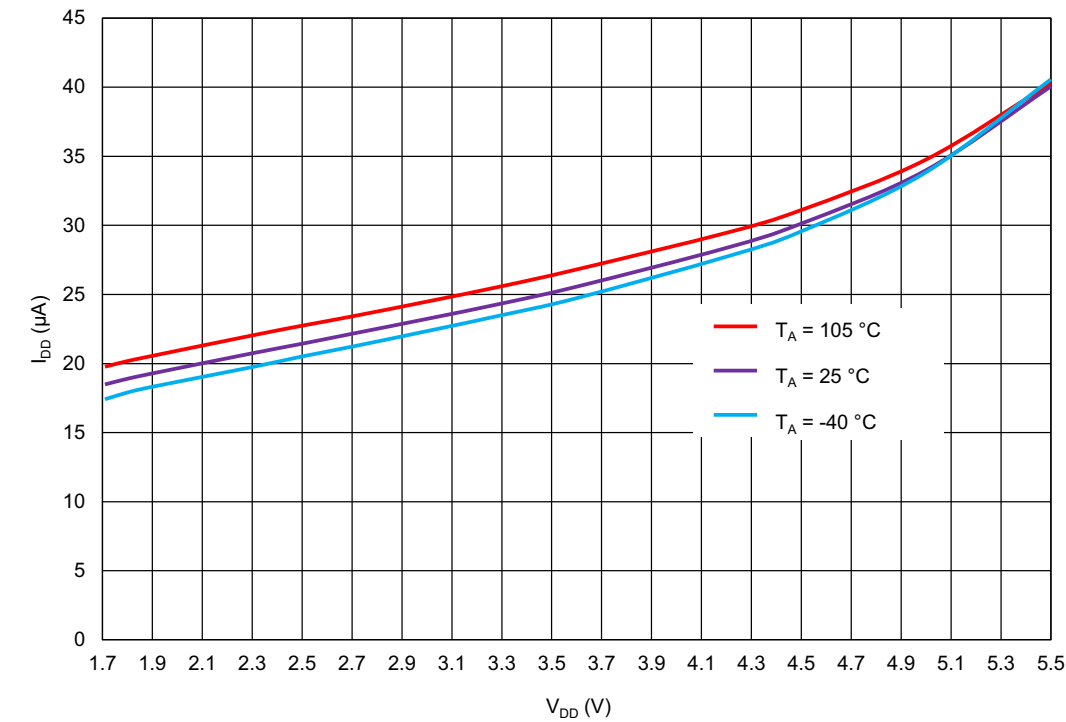
Figure 89. OSC0 (2 MHz) Current Consumption vs. V_{DD} , Pre-Divider = 8
