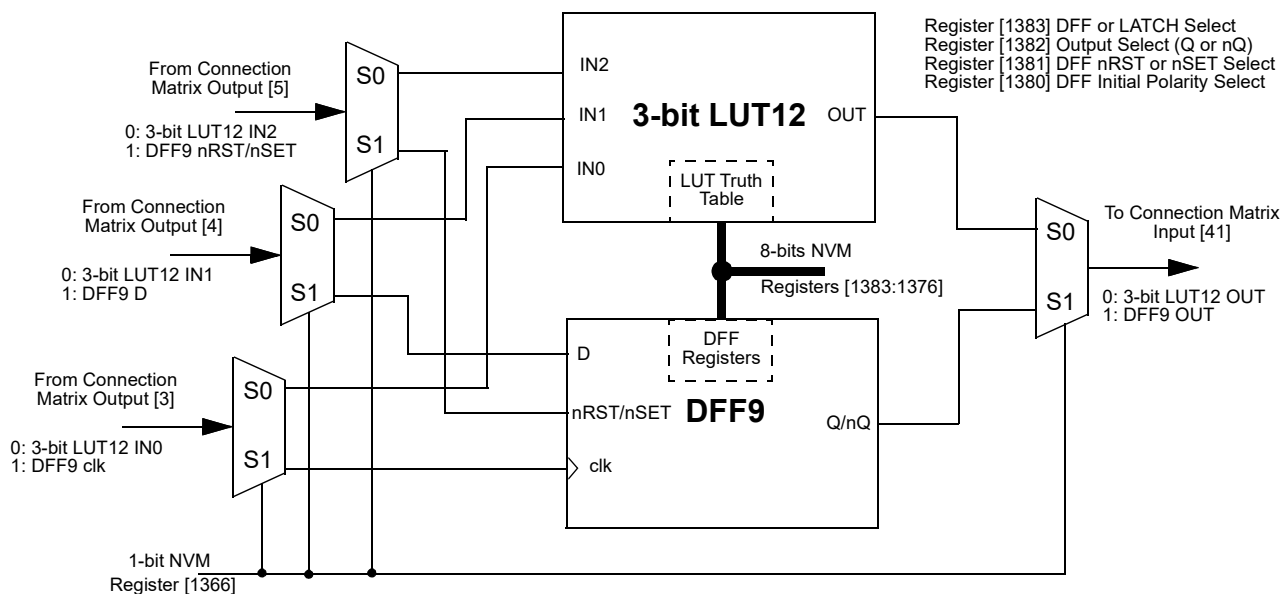
Figure 24. 3-bit LUT12 or DFF9 with RST/SET
