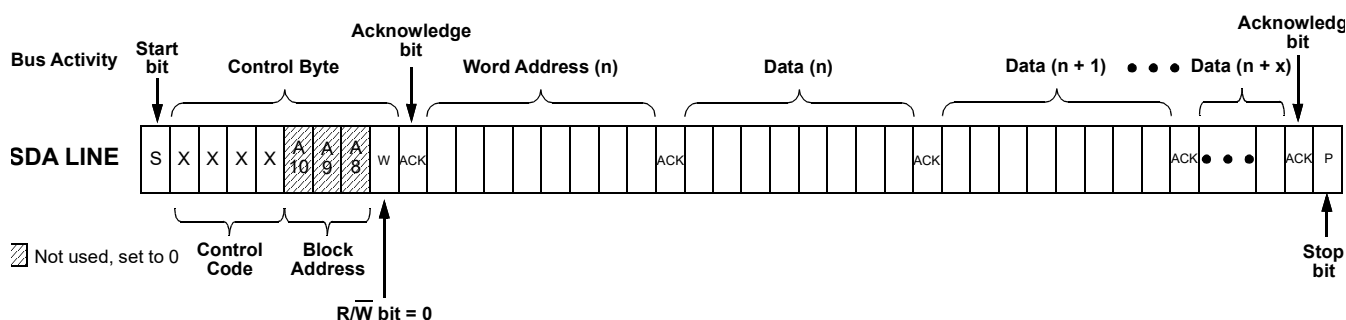
Figure 119. Sequential Write Command
