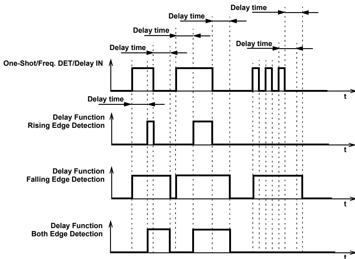
Figure 44. Delay Mode Timing Diagram
