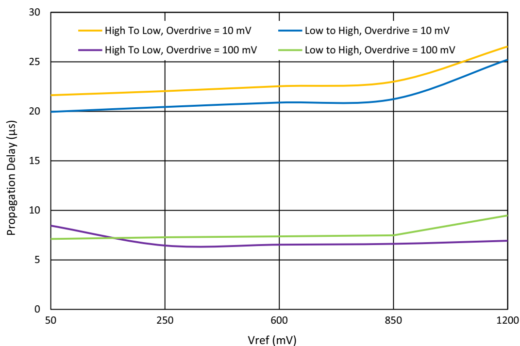
Figure 60. ACMPx Typical Propagation Delay at T_A = +25^\circ\text{C} , Gain = 1, Hysteresis = 0, V_{DD} = 1.71\text{ V} to 5.5\text{ V} , LPF-Enable
