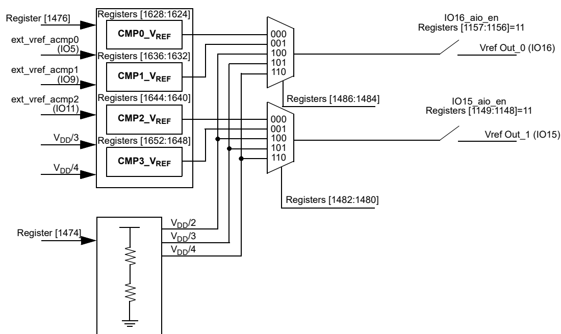
Figure 68. Voltage Reference Block Diagram
