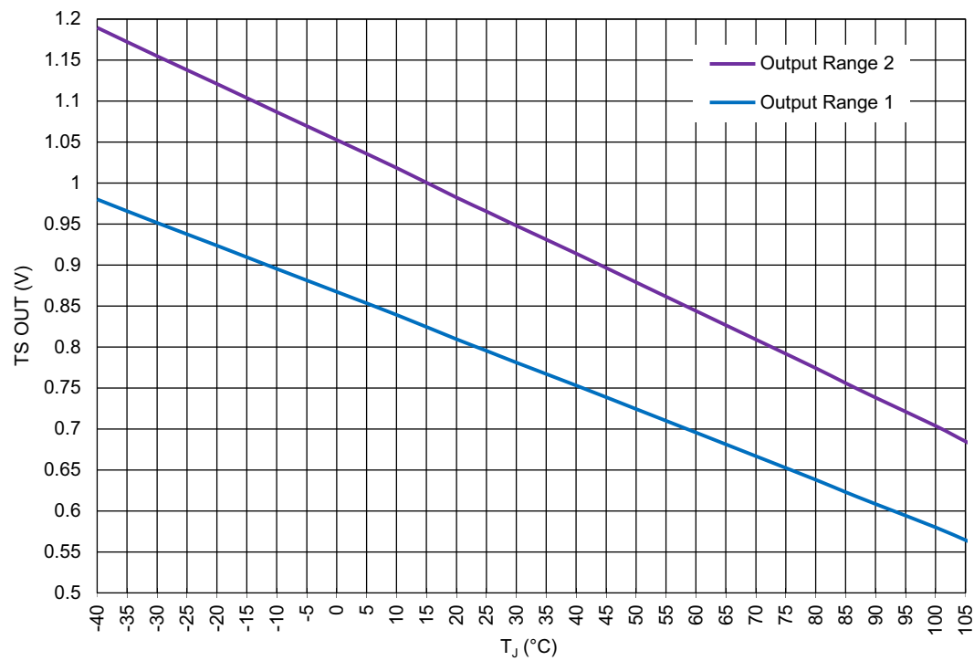
Figure 126. TS Output vs. Junction Temperature, V DD = 1.71 V to 5.5 V
