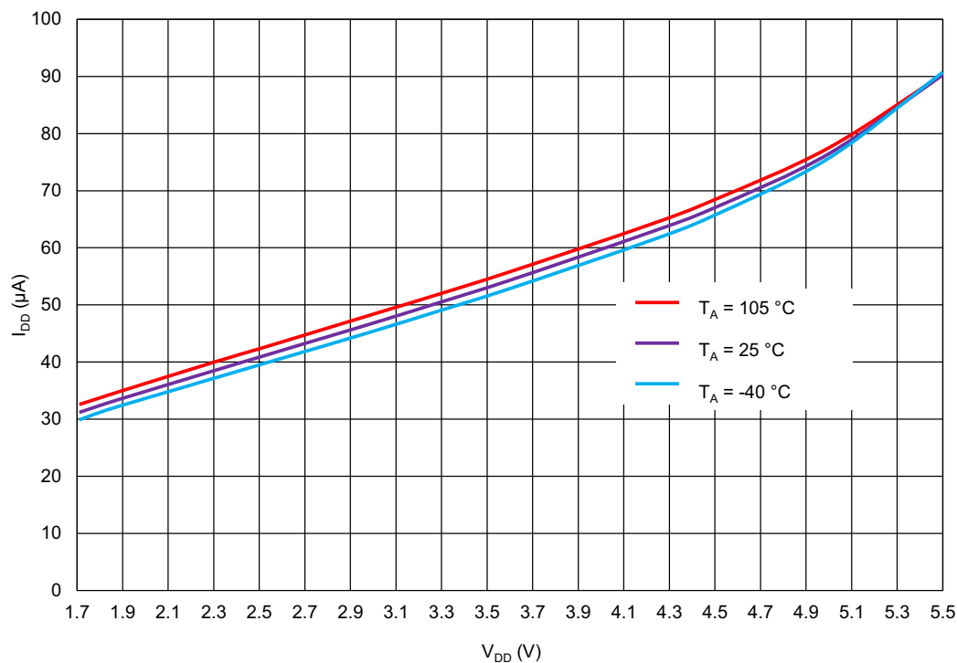
Figure 86. OSC0 (2 MHz) Current Consumption vs. V_{DD} , Pre-Divider = 1
