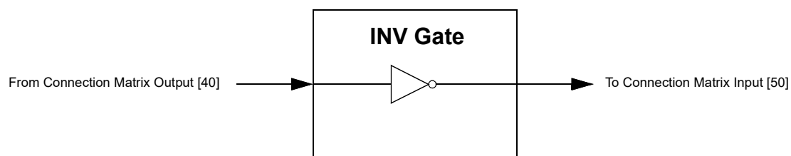
Figure 67. INV Gate
