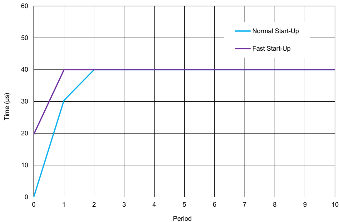
Figure 82. Oscillator0 Settling Time, V_{DD} = 3.3\text{ V} , T_A = +25\text{ }^{\circ}\text{C} , \text{OSC0} = 2\text{ kHz}
