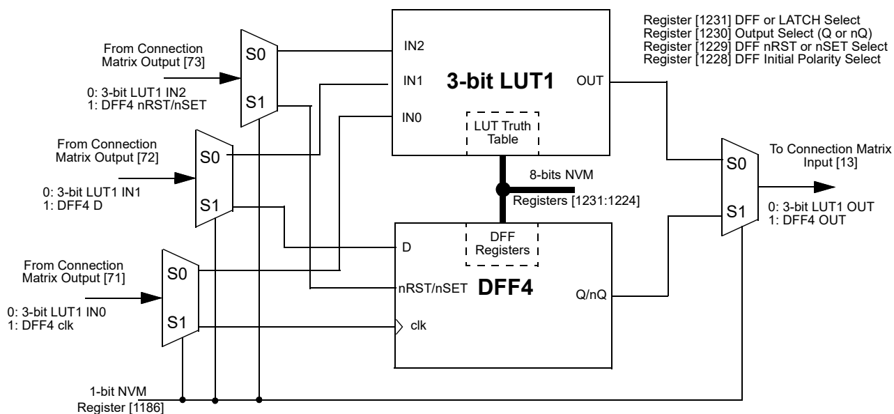
Figure 19. 3-bit LUT1 or DFF4 with RST/SET
