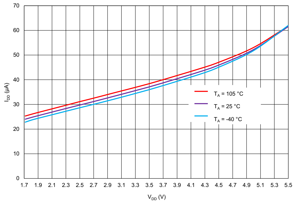
Figure 87. OSC0 (2 MHz) Current Consumption vs. V DD , Pre-Divider = 2
