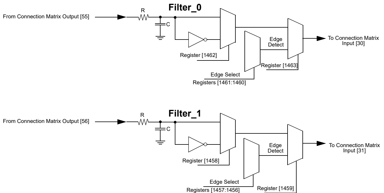
Figure 66. Deglitch Filter/Edge Detector
