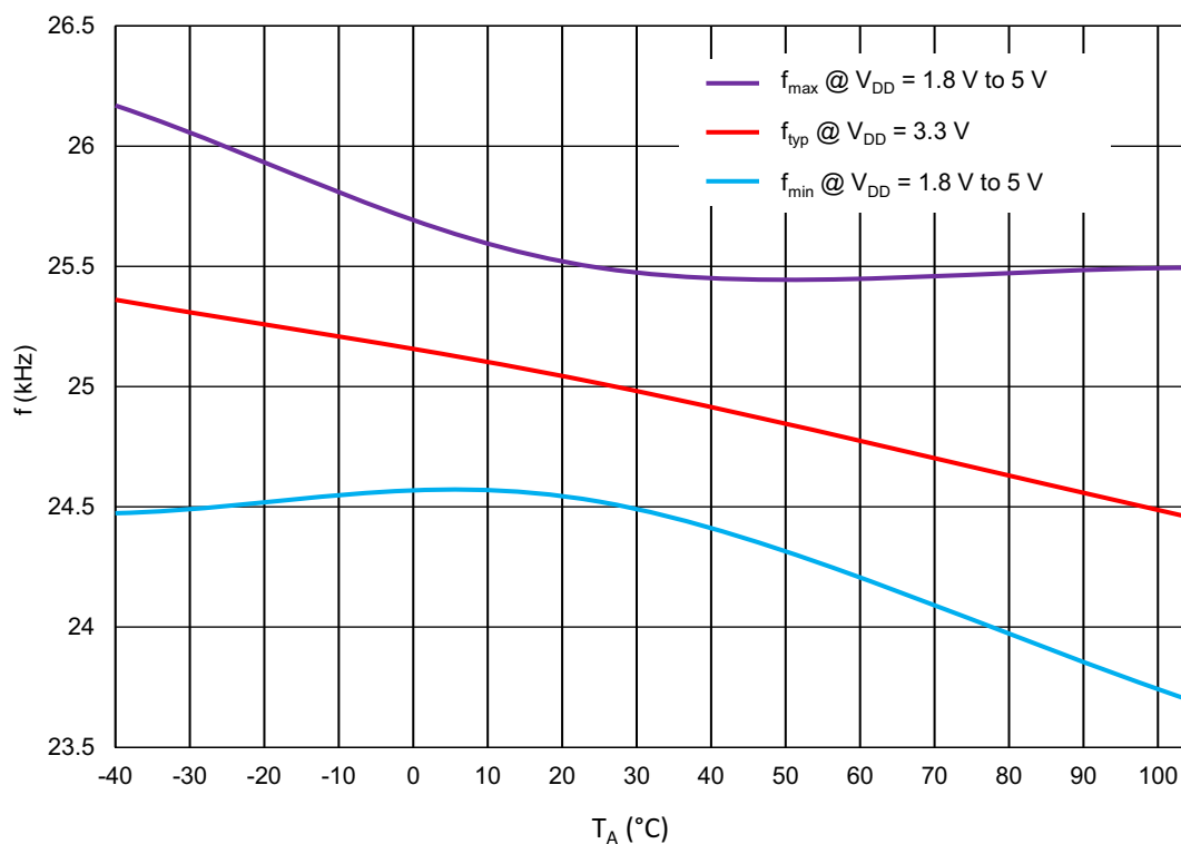
Figure 78. Oscillator Frequency vs. Ambient Temperature, OSC0 = 25 kHz
