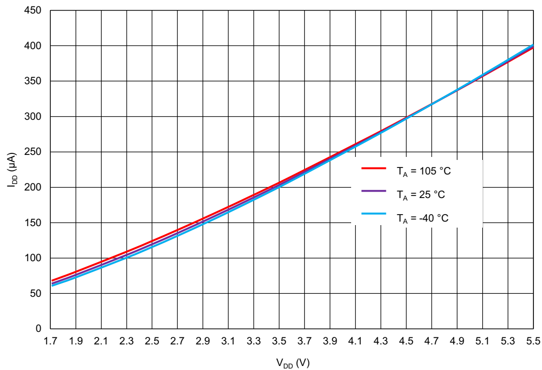
Figure 92. OSC1 (25 MHz) Current Consumption vs. V_{DD} , Pre-Divider = 4
