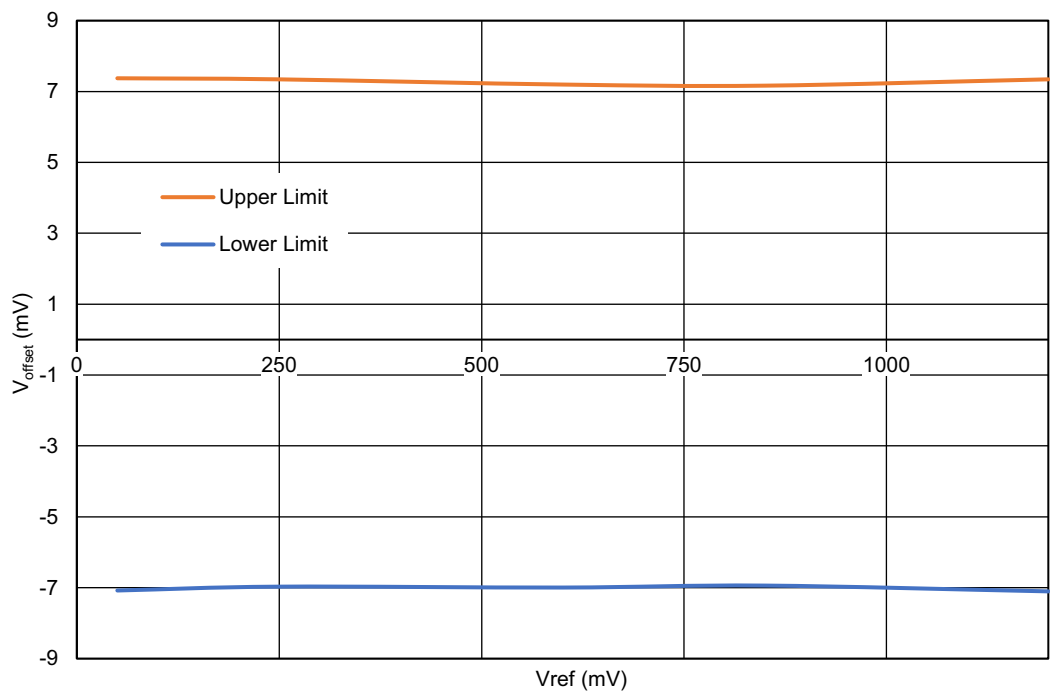
Figure 58. ACMPx Input Offset Voltage vs. V_{REF} at V_{DD} = 1.71\text{ V to }5.5\text{ V} , T_A = -40\text{ }^{\circ}\text{C to }+105\text{ }^{\circ}\text{C}
