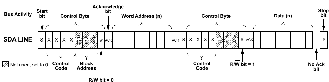
Figure 121. Random Read Command
