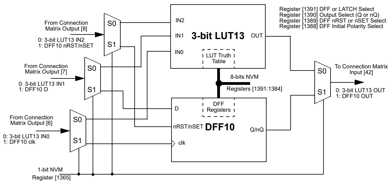
Figure 25. 3-bit LUT13 or DFF10 with RST/SET
