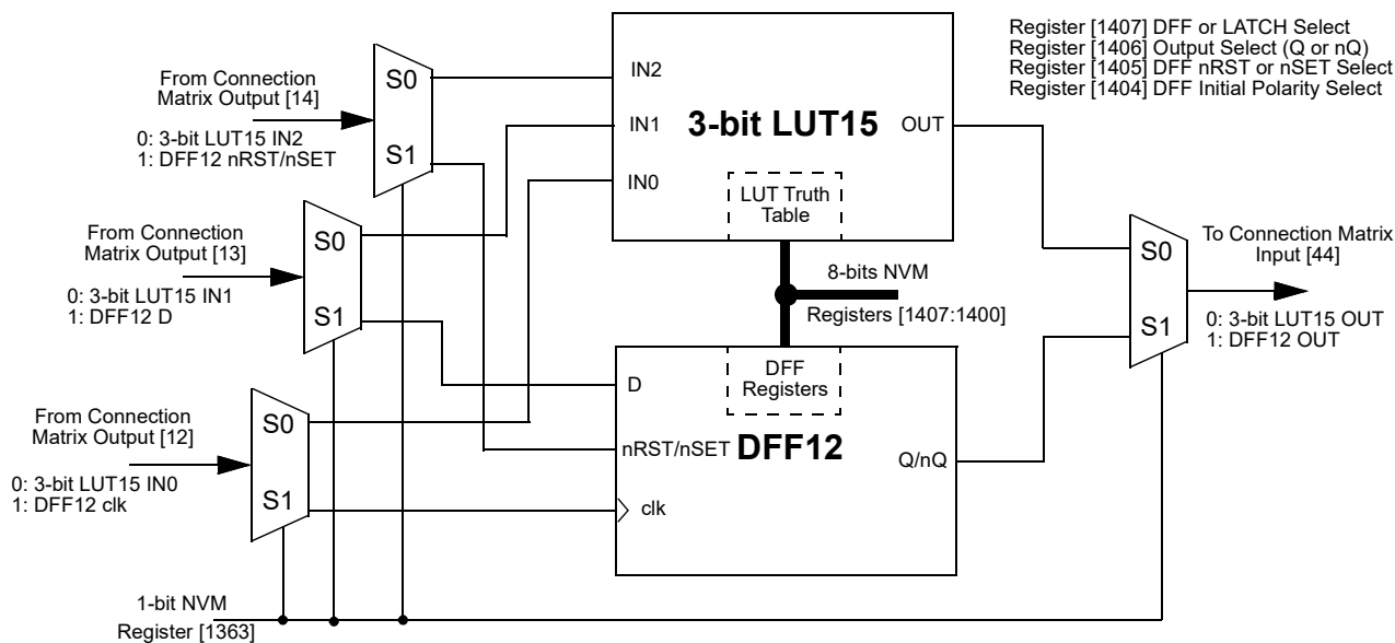
Figure 27. 3-bit LUT15 or DFF12 with RST/SET
