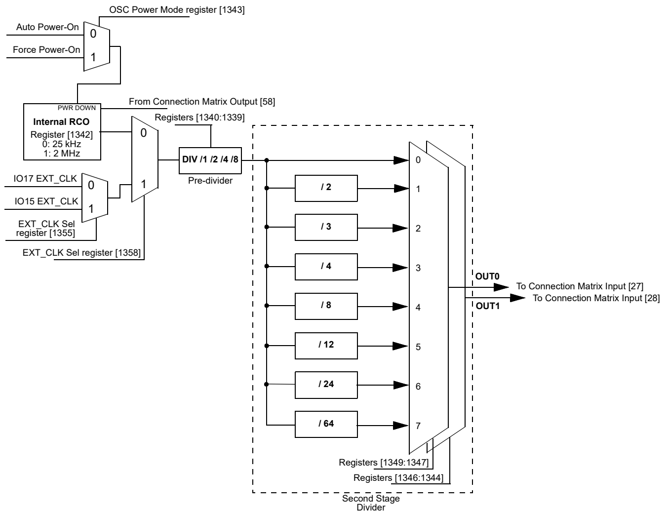
Figure 72. 25 kHz/2 MHz OSC Block Diagram
