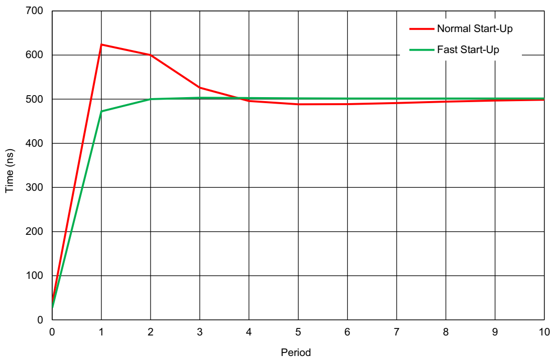
Figure 83. Oscillator0 Settling Time, V_{DD} = 3.3\text{ V} , T_A = +25\text{ }^{\circ}\text{C} , \text{OSC0} = 2\text{ MHz}
