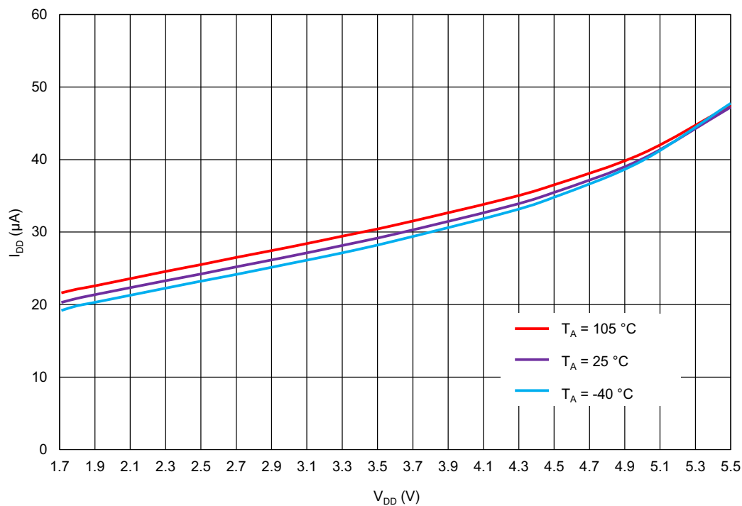
Figure 88. OSC0 (2 MHz) Current Consumption vs. V DD , Pre-Divider = 4
