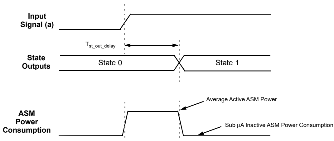
Figure 106. State Transition Timing and Power Consumption
