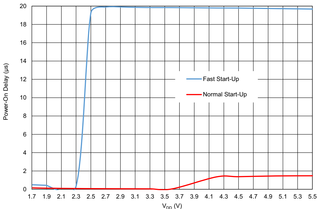
Figure 75. Oscillator Maximum Power-On Delay vs. V_{DD} at T_A = +25\text{ }^{\circ}\text{C} , OSC0 = 25 kHz
