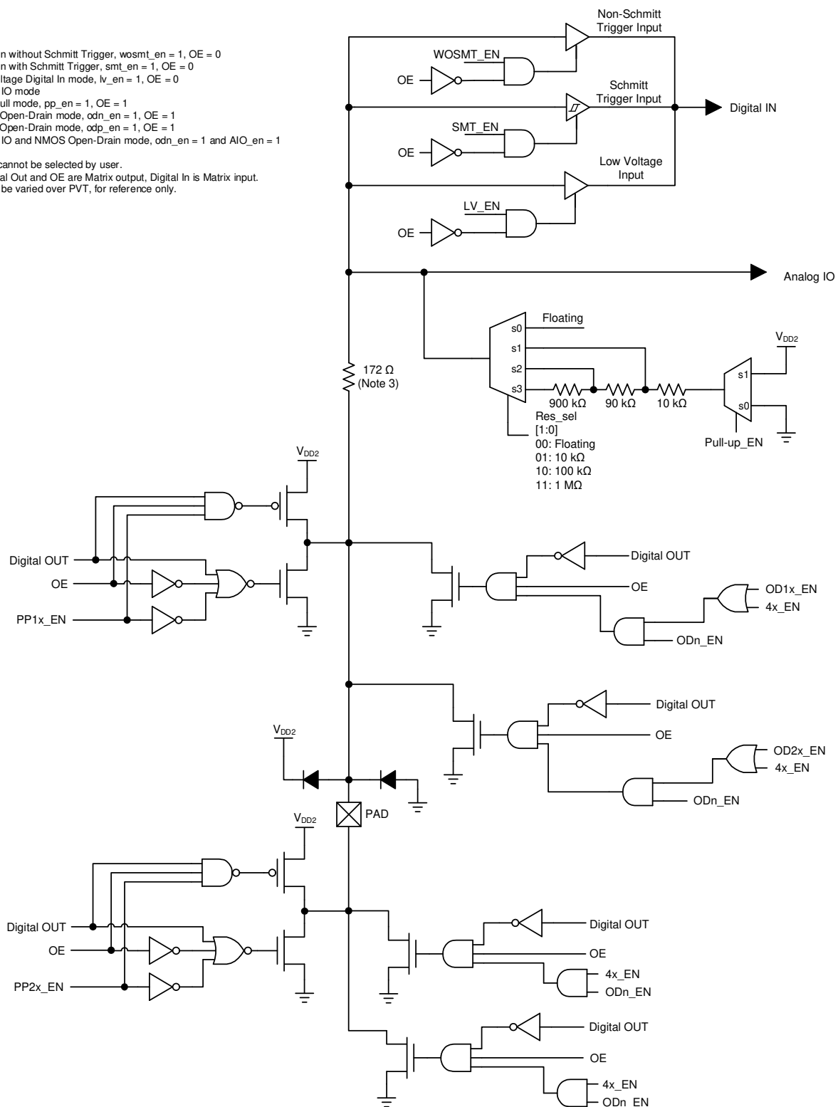
Figure 11. IO 4x Drive Structure Diagram
