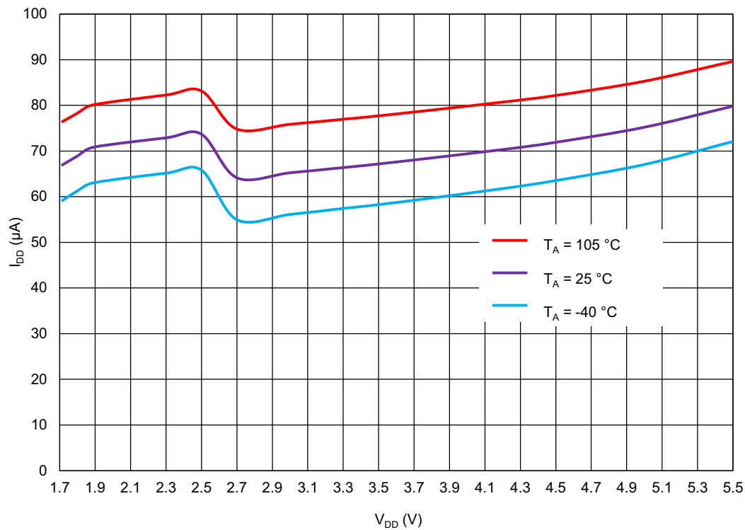
Figure 63. Buffered ACMPx Current Consumption vs. V_{DD} at V_{IN+} Connected to V_{DD} , Internal V_{REF} = 50\text{ mV}
