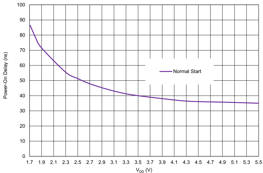
Figure 77. Oscillator Maximum Power-On Delay vs. V DD at T A = +25 °C, OSC1 = 25 MHz
