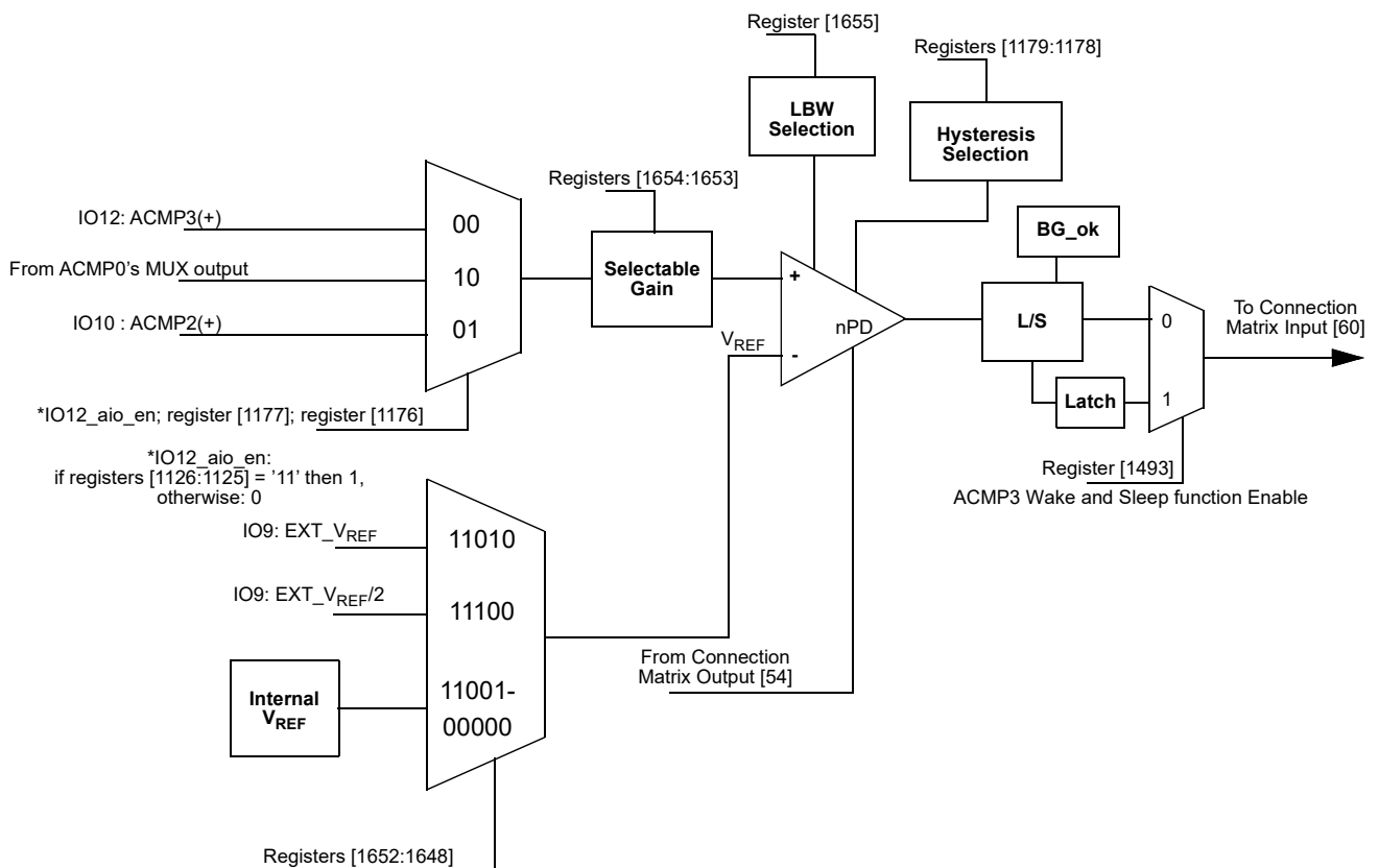
Figure 56. ACMP3 Block Diagram
