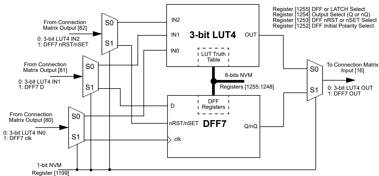
Figure 22. 3-bit LUT4 or DFF7 with RST/SET
