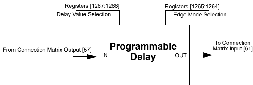
Figure 64. Programmable Delay
