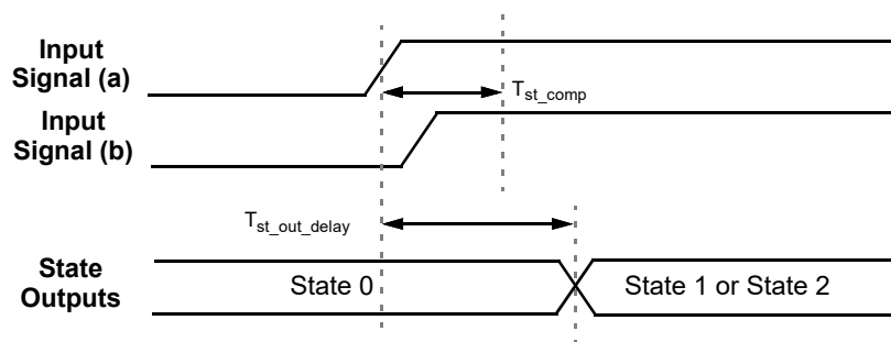
Figure 111. State Transition Timing - Competing Inputs Indeterminate
