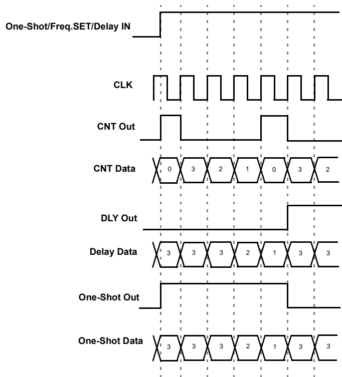
Figure 49. Counter Value, Counter Data = 3
