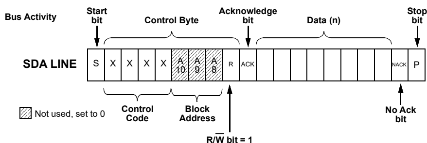
Figure 120. Current Address Read Command, \overline{R/W} = 1
