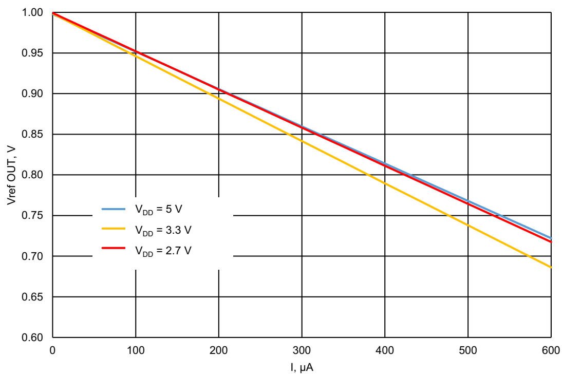
Figure 71. Typical Load Regulation, V_{REF} = 1200 mV, T_A = -40 °C to +105 °C, Buffer - Enable
