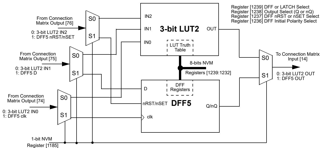
Figure 20. 3-bit LUT2 or DFF5 with RST/SET
