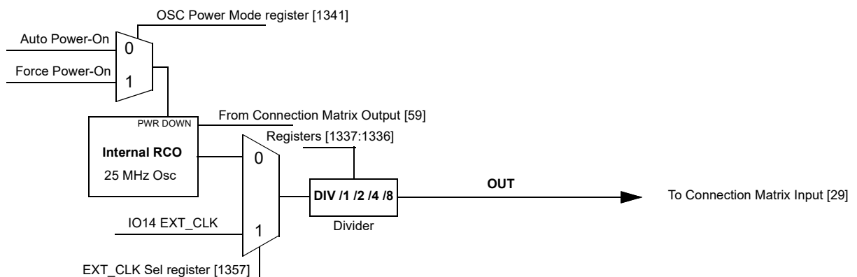
Figure 73. 25 MHz OSC Block Diagram
