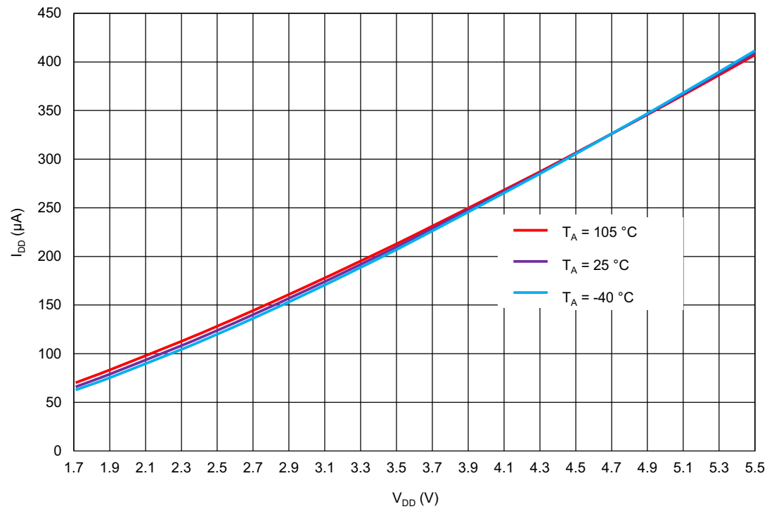
Figure 91. OSC1 (25 MHz) Current Consumption vs. V_{DD} , Pre-Divider = 2
