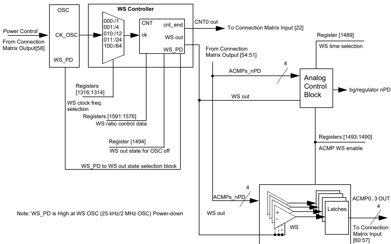
Figure 52. Wake/Sleep Controller
