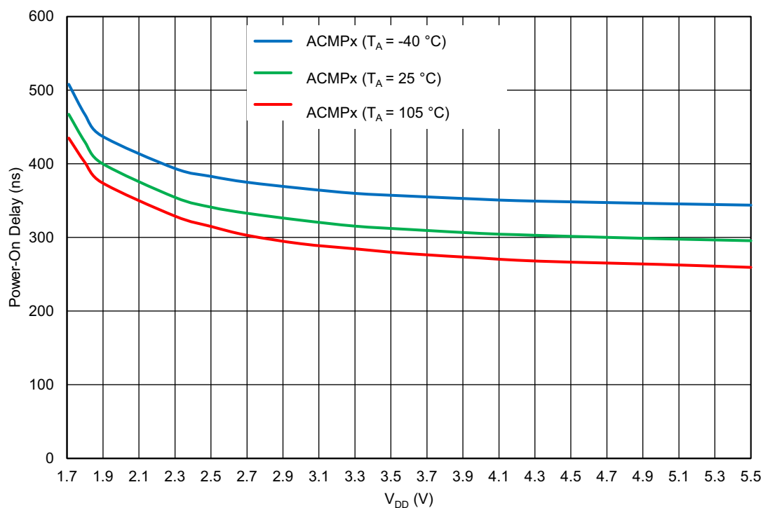
Figure 57. ACMPx Power-On Delay vs. VDD, BG Delay – Any
