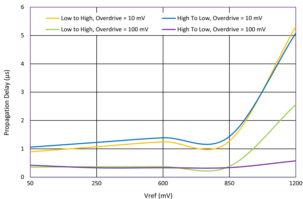
Figure 61. ACMPx Typical Propagation Delay at T_A = +25^\circ\text{C} , Gain = 1, Hysteresis = 0, V_{DD} = 1.71\text{ V} to 5.5\text{ V} , LPF-Disable
