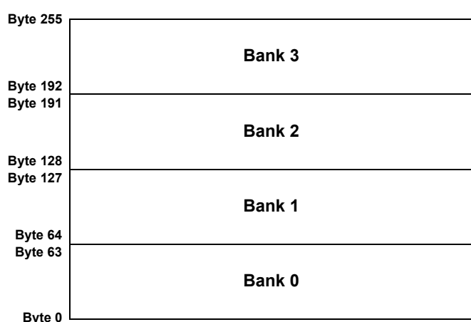
Figure 123. Register Bank Map
