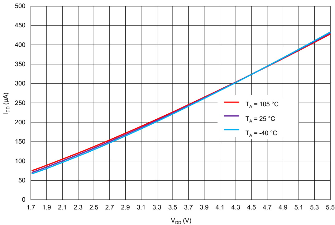
Figure 90. OSC1 (25 MHz) Current Consumption vs. V_{DD} , Pre-Divider = 1
