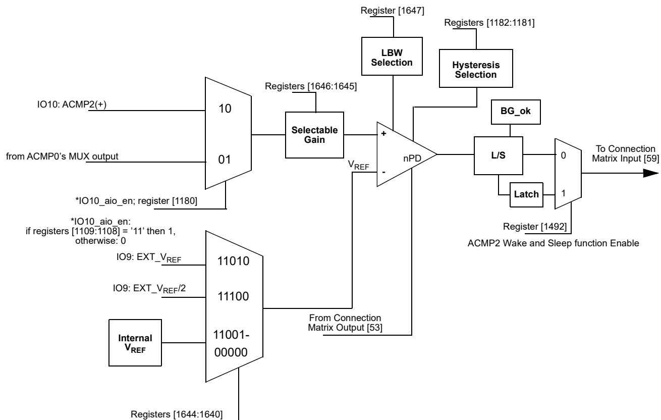
Figure 55. ACMP2 Block Diagram
