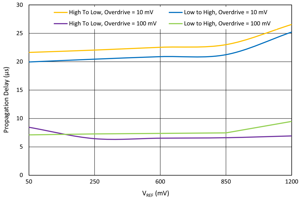
Figure 60. ACMPx Propagation Delay at T A = 25 °C, Gain = 1, Hysteresis = 0, V DD = 1.71 V to 5.5 V, LPF – Enable
