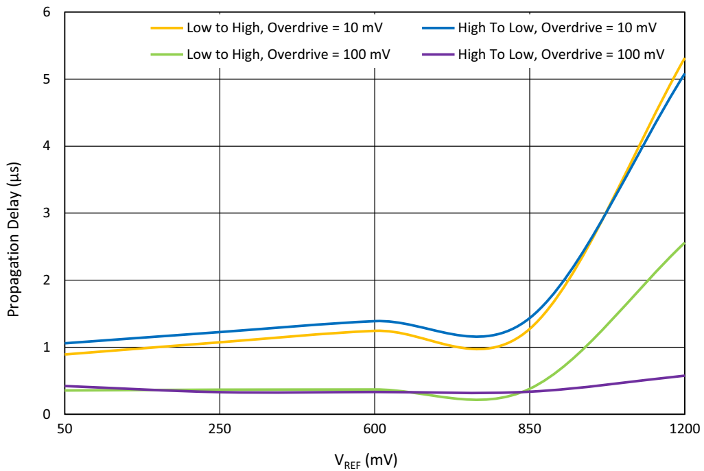
Figure 61. ACMPx Propagation Delay at T A = 25 °C, Gain = 1, Hysteresis = 0, V DD = 1.71 V to 5.5 V, LPF – Disable
