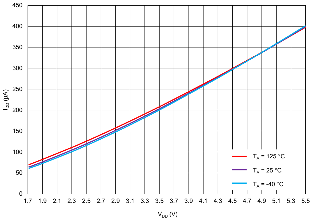
Figure 92. OSC1 (25 MHz) Current Consumption vs. V DD , Pre-Divider = 4
