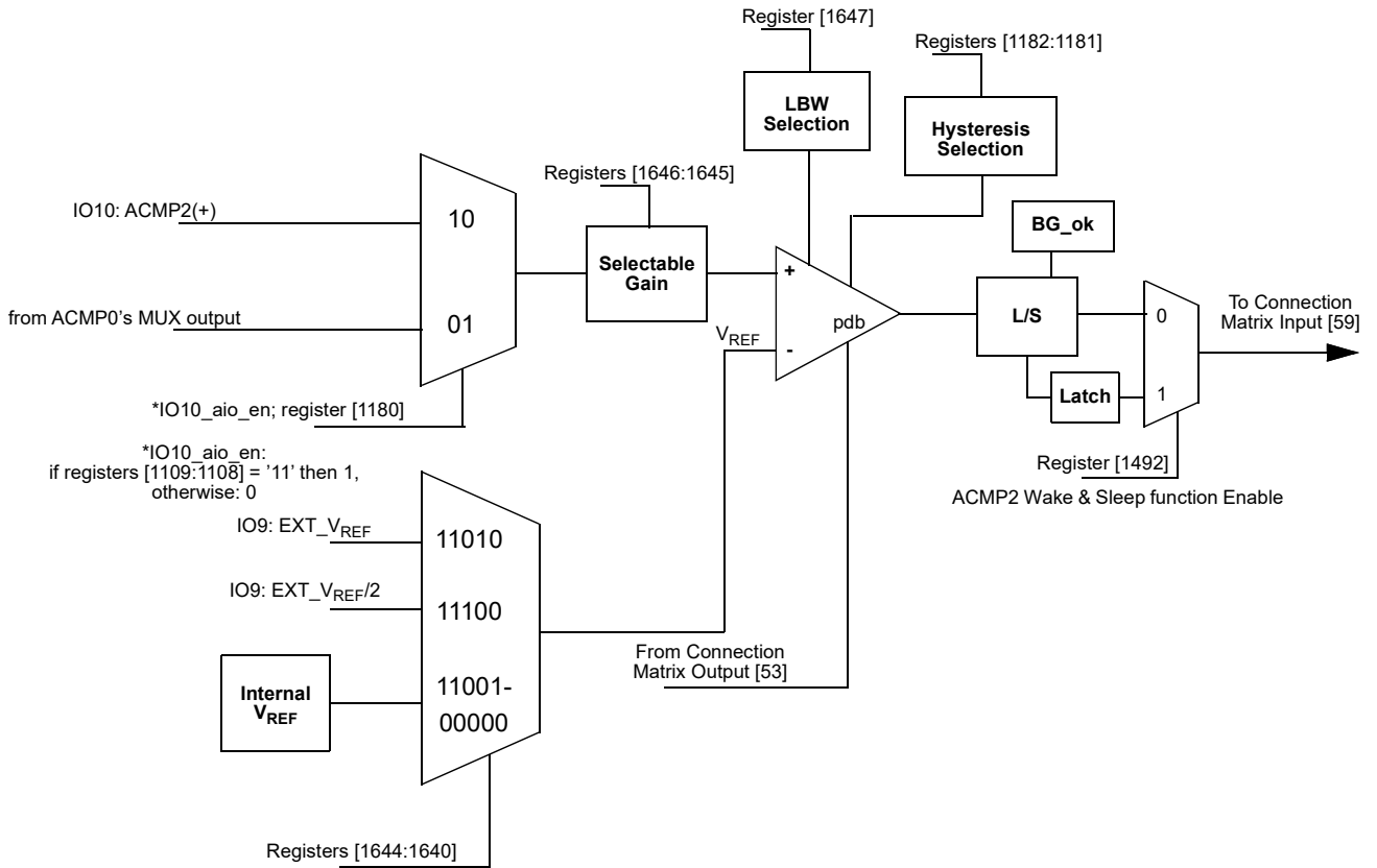
Figure 55. ACMP2 Block Diagram
