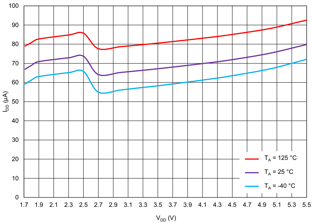
Figure 63. Buffered ACMPx Current Consumption vs. V DD at V IN+ Connected to V DD , Internal V REF = 50 mV
