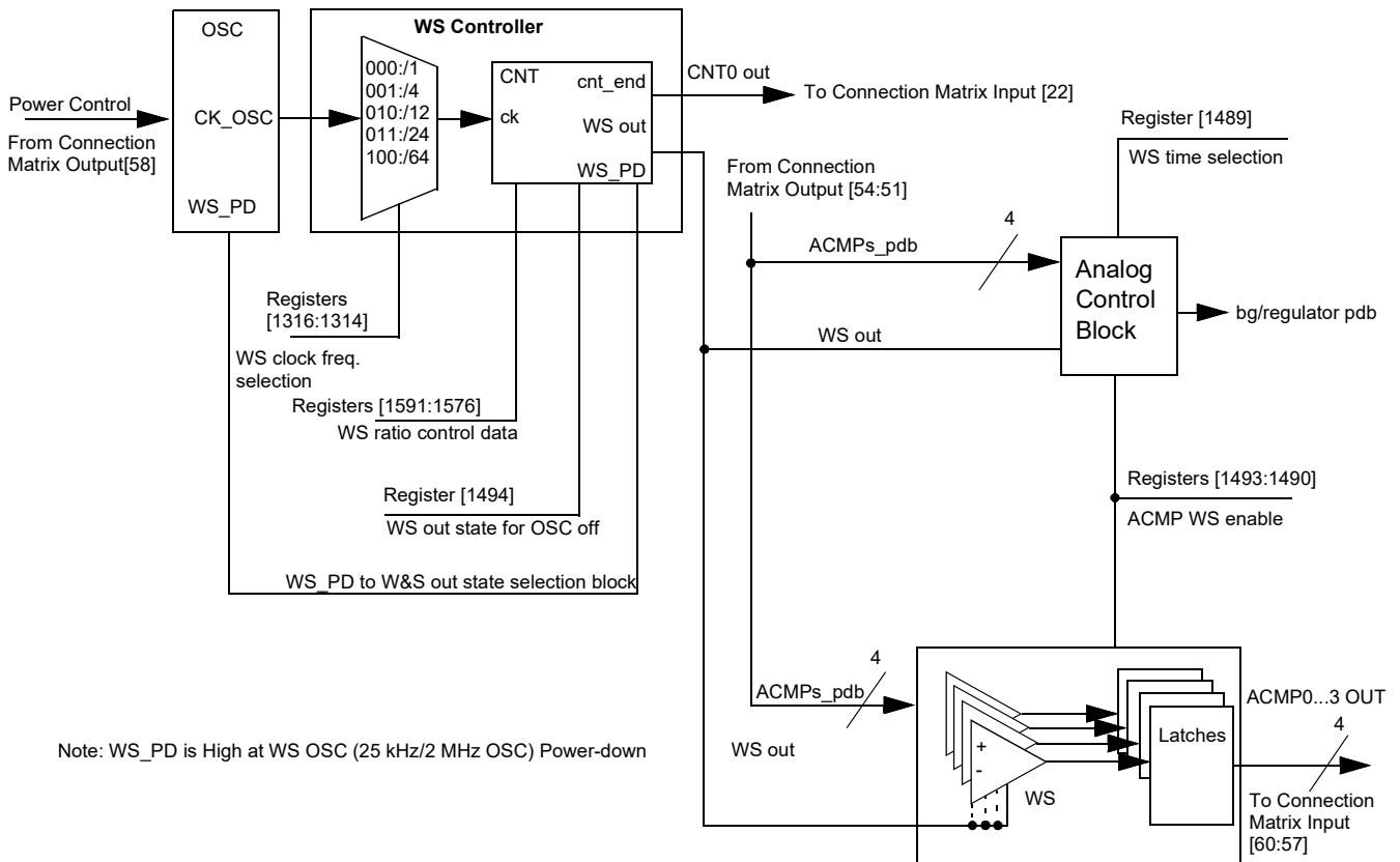
Figure 52. Wake/Sleep Controller
