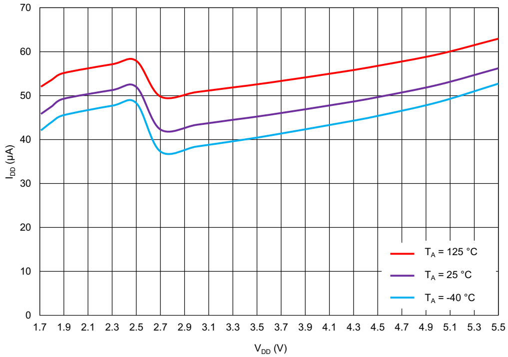
Figure 62. ACMPx Current Consumption vs. V DD at V IN+ Connected to V DD , Internal V REF = 50 mV
