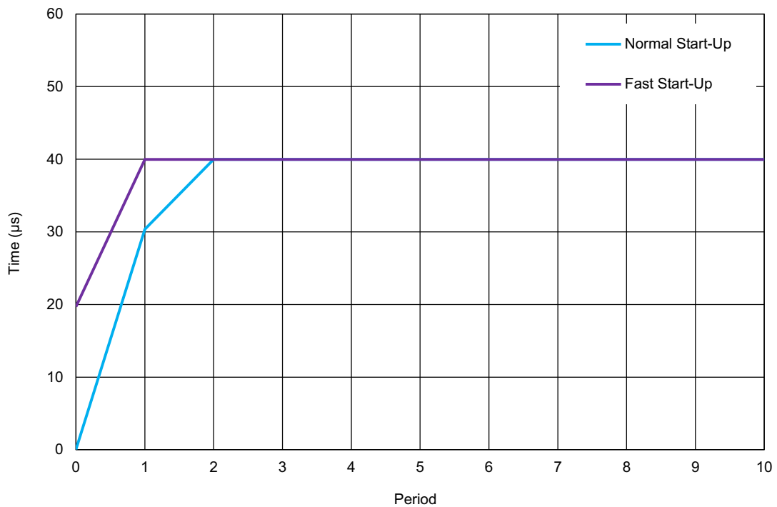
Figure 82. Oscillator0 Settling Time, V_{DD} = 3.3 V, T_A = 25 °C, OSC0 = 25 kHz
