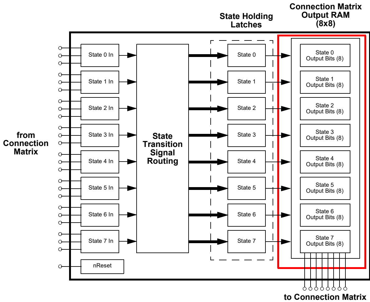
Figure 102. Connection Matrix Output RAM
