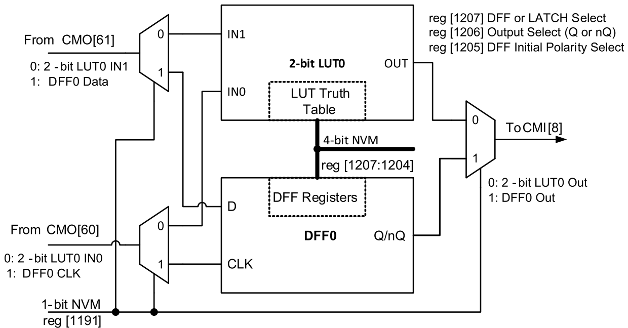
Figure 15. 2-bit LUT0 or DFF0
