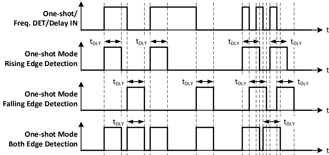
Figure 36. One-Shot Function Timing Diagram
