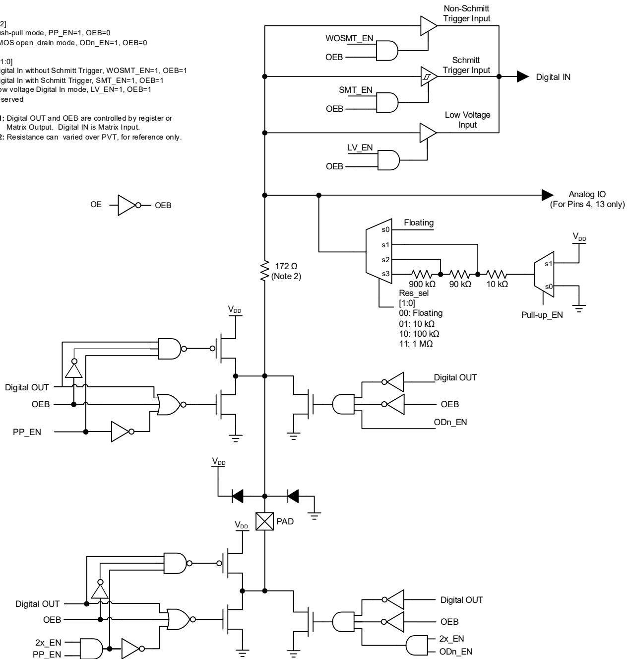
Figure 8. Matrix OE IO Structure Diagram (Pin 14)
