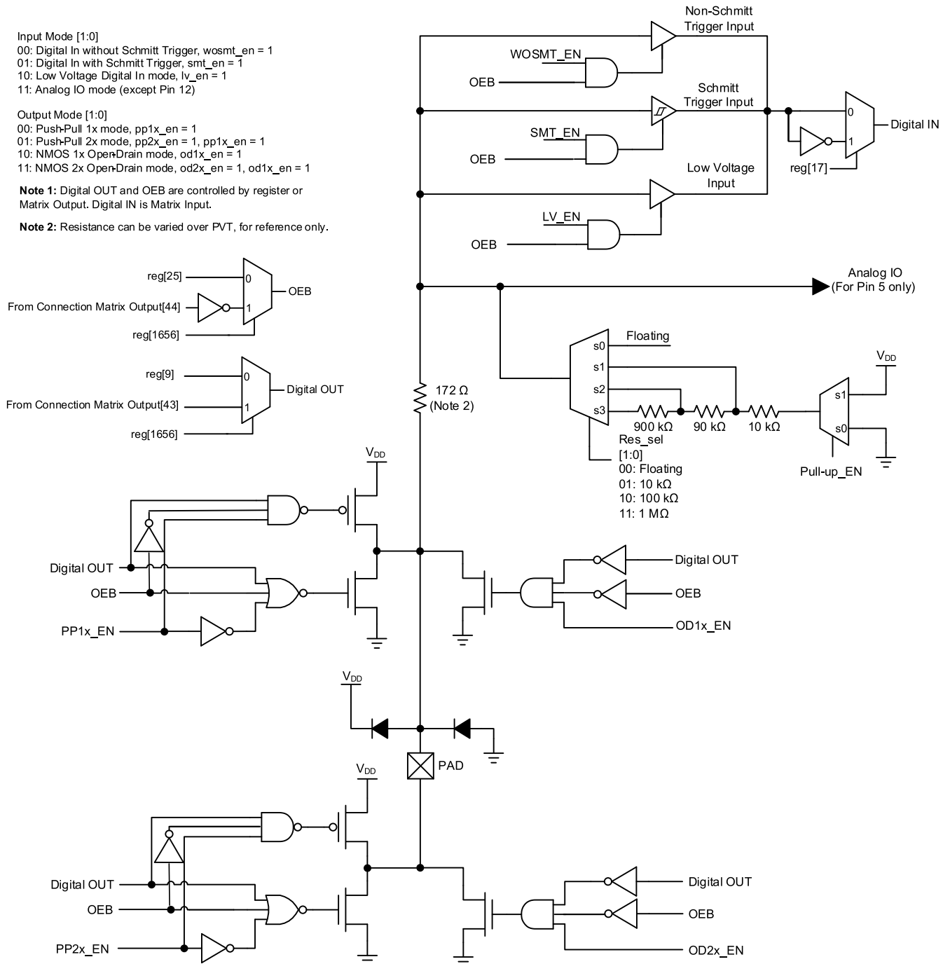
Figure 7. Matrix OE IO Structure Diagram (Pin 12)
