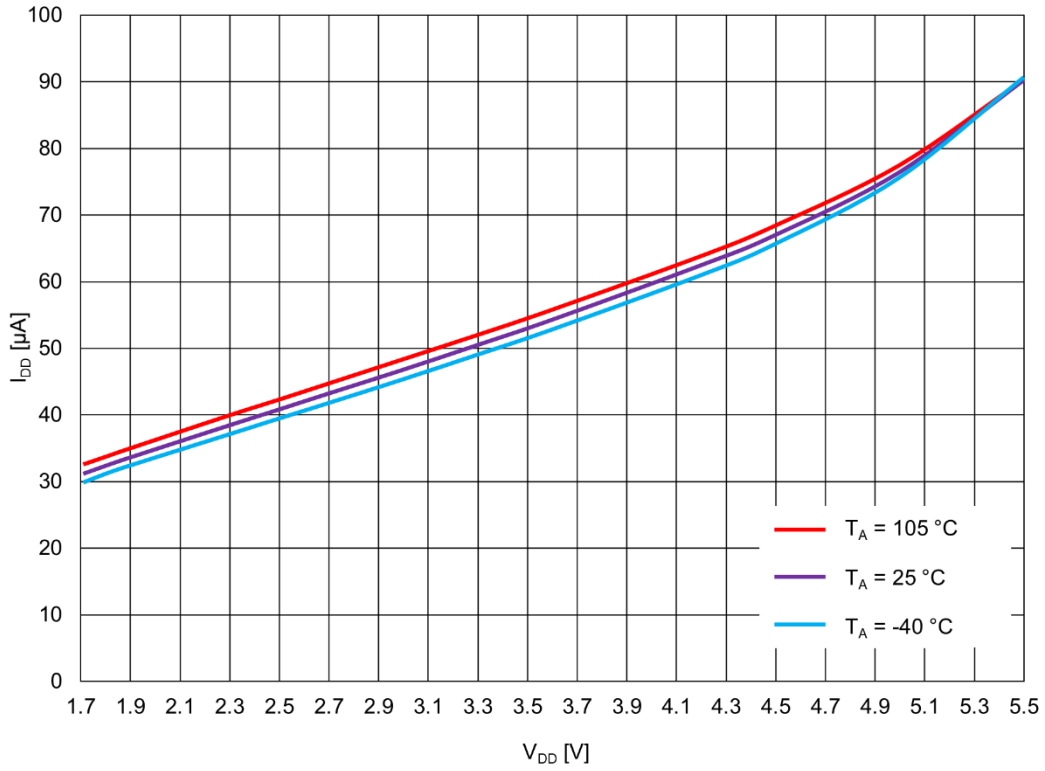
Figure 79. OSC0 (2 MHz) Current Consumption vs. V DD , Pre-Divider = 1
