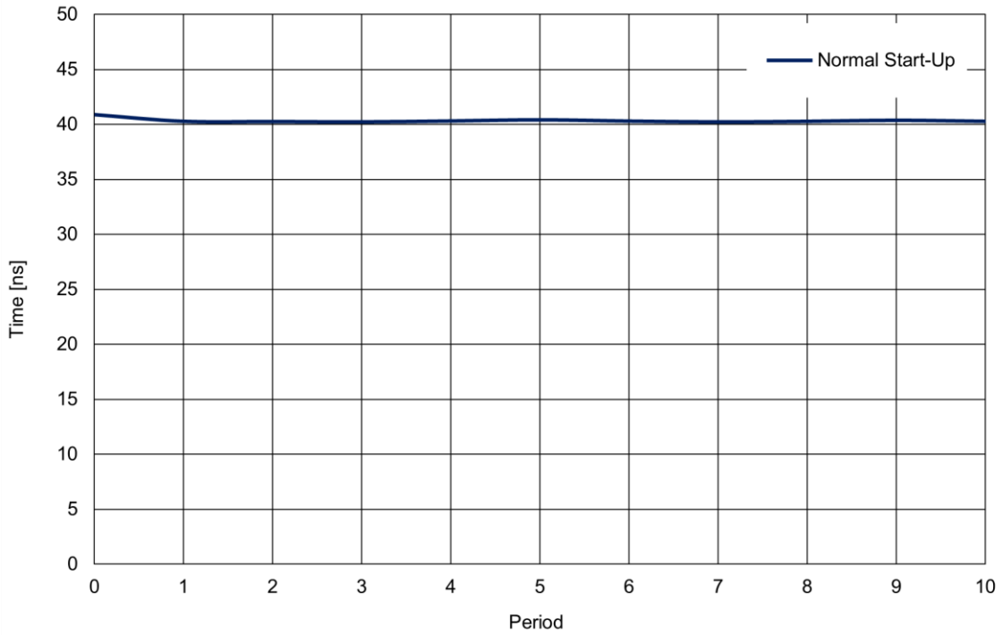
Figure 77. Oscillator0 Settling Time, V_{DD} = 3.3\text{ V} , T_A = +25\text{ }^\circ\text{C} , OSC1 = 25\text{ MHz}
