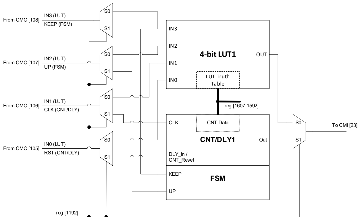
Figure 33. 4-bit LUT1 or CNT/DLY1
