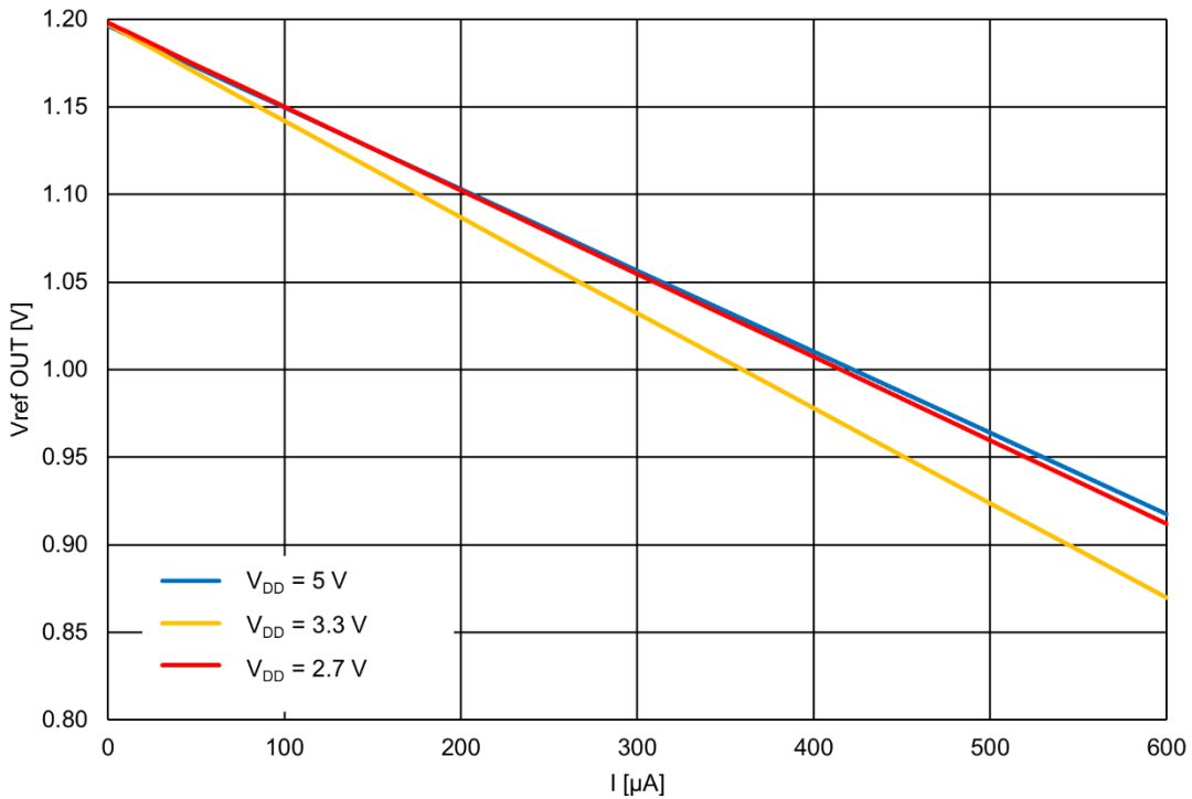
Figure 64. Typical Load Regulation, V REF = 1200 mV, T A = -40 °C to +85 °C, Buffer - Enable
