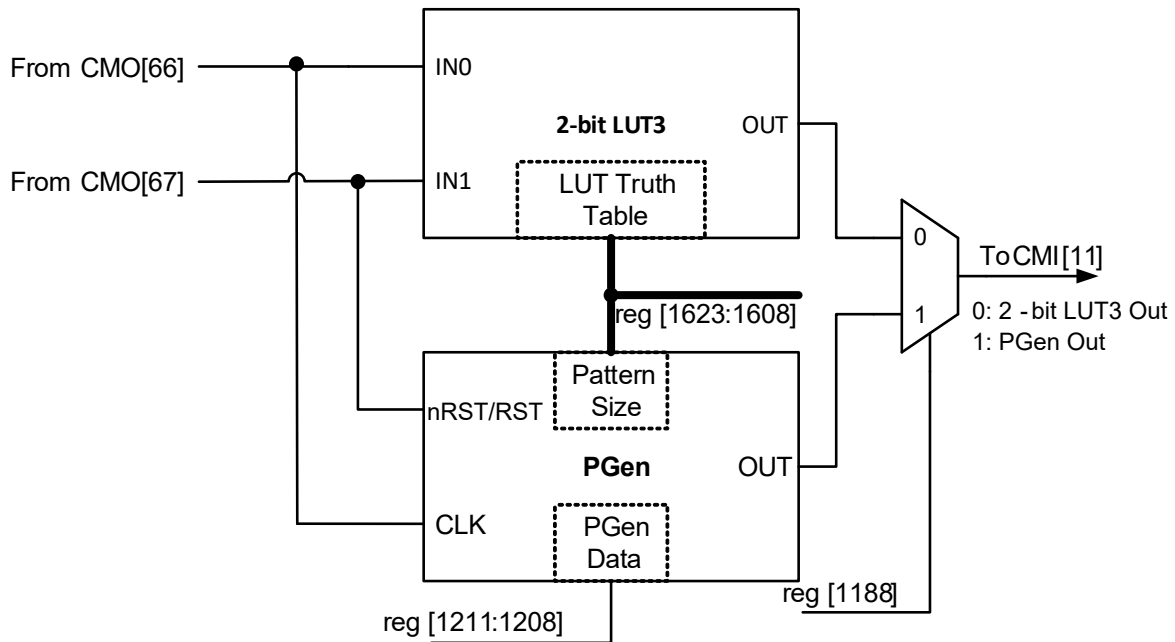
Figure 45. 2-bit LUT3 or PGen
