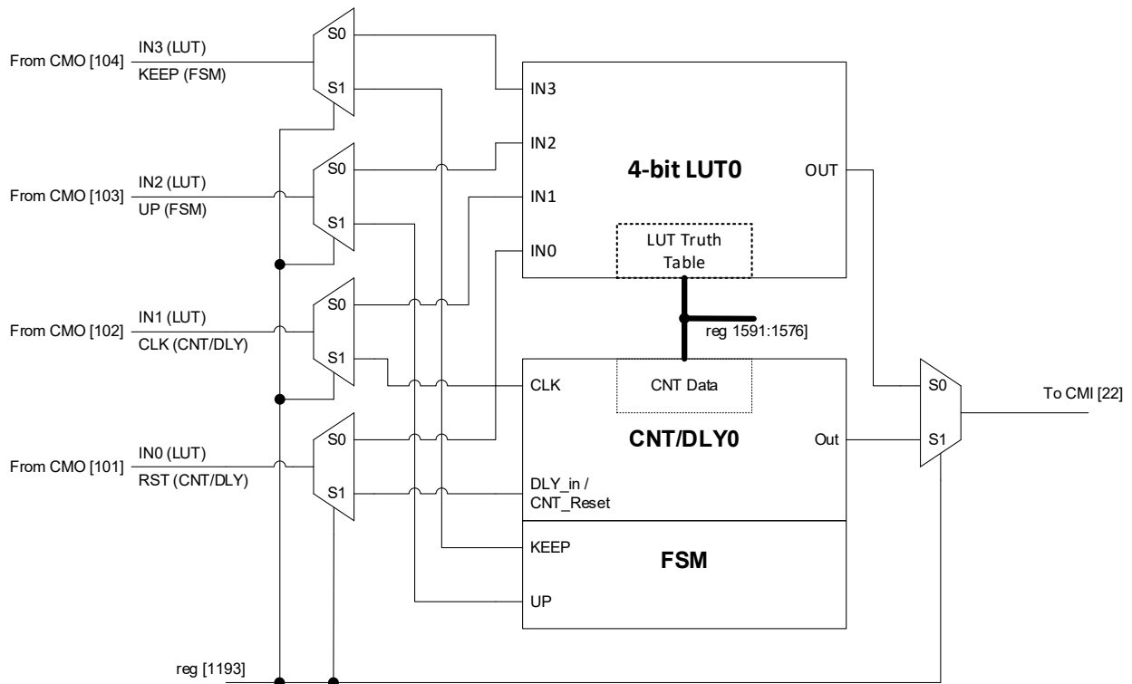
Figure 32. 4-bit LUT0 or CNT/DLY0
