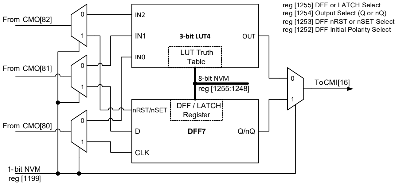
Figure 23. 3-bit LUT4 or DFF7 with RST/SET
