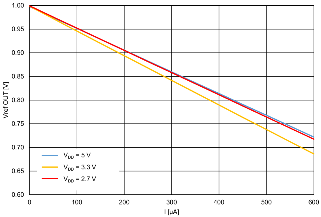
Figure 63. Typical Load Regulation, V REF = 1000 mV, T A = -40 °C to +85 °C, Buffer - Enable
