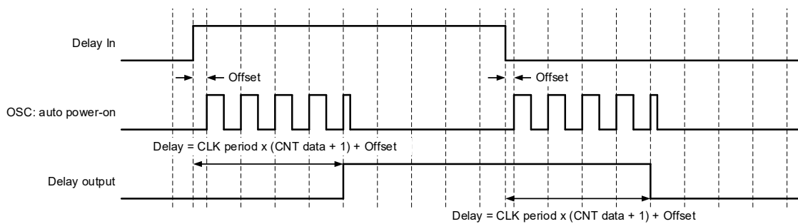
(Case 2) OSC: Auto Power-on (powers up from Delay In signal)
