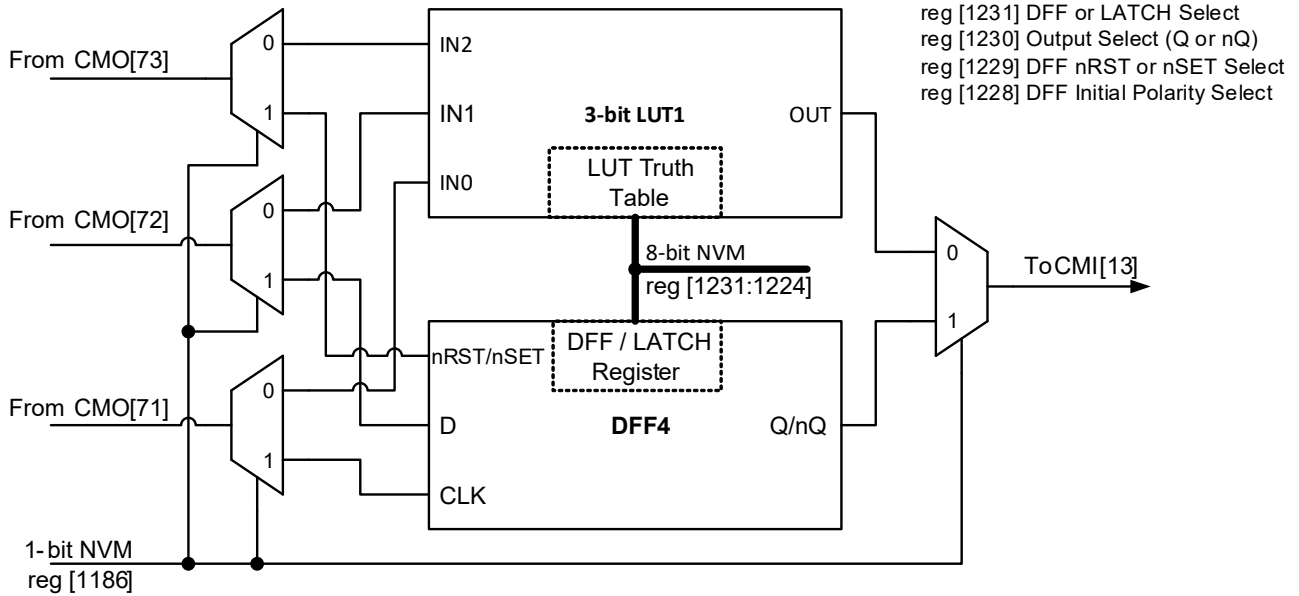
Figure 20. 3-bit LUT1 or DFF4 with RST/SET
