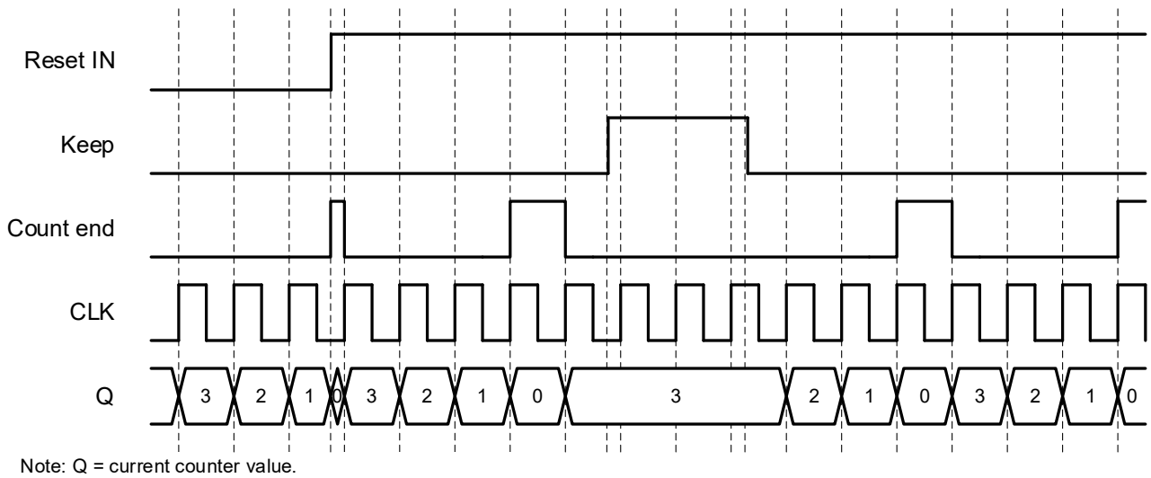
Figure 40. CNT/FSM Timing Diagram (Reset Rising Edge Mode, Oscillator is Forced On, UP = 0) for Counter Data = 3
