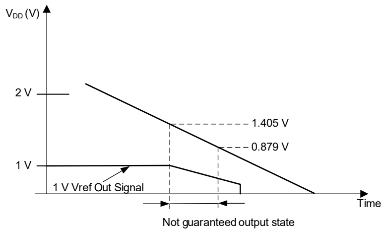
Figure 89. Power-Down
