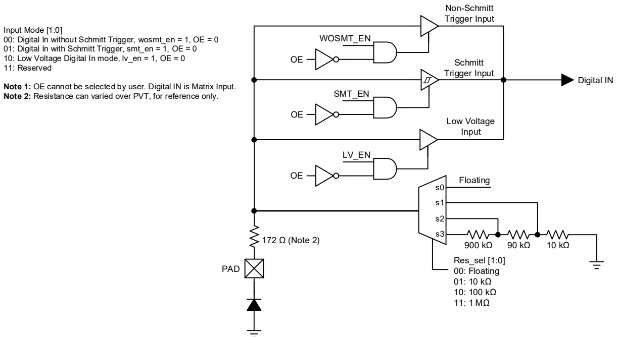
Figure 4. GPI Structure Diagram (Pin 2)
