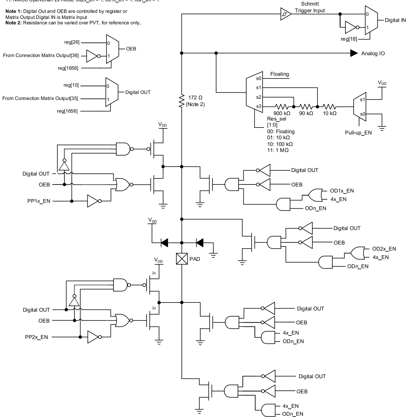
Figure 9. Matrix OE IO 4x Drive Structure Diagram (Pin 8)
