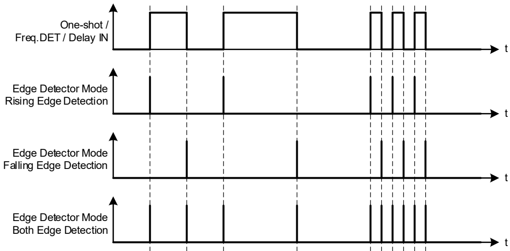
Figure 38. Edge Detection Mode Timing Diagram
