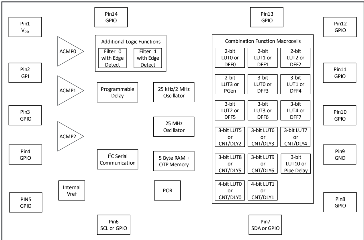
Figure 1. Block Diagram
