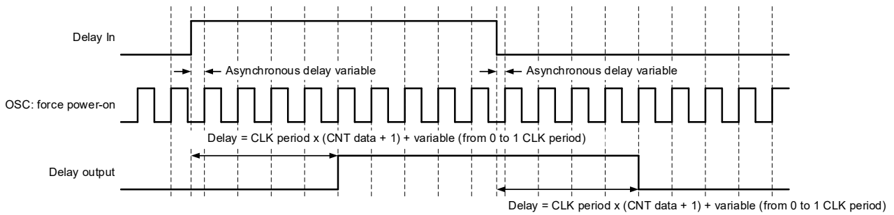
(Case 1) OSC: Forced Power-on (always running)
