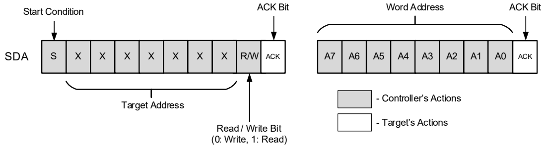
Figure 90. Basic Command Structure
