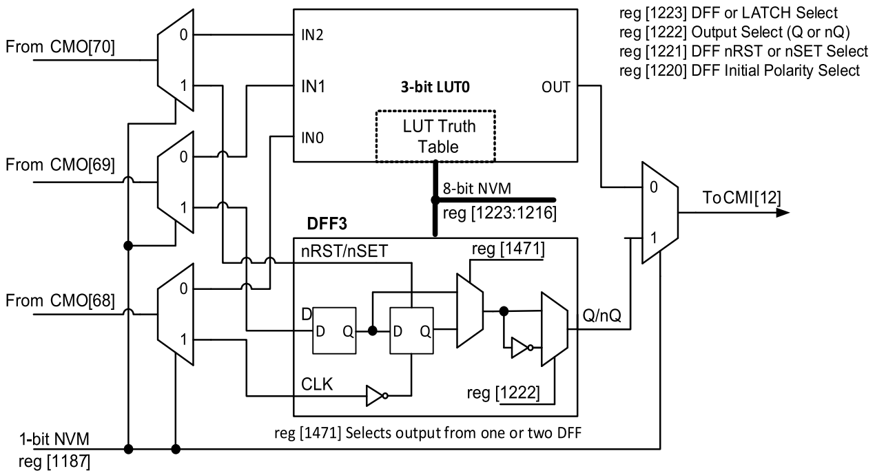
Figure 19. 3-bit LUT0 or DFF3 with RST/SET
