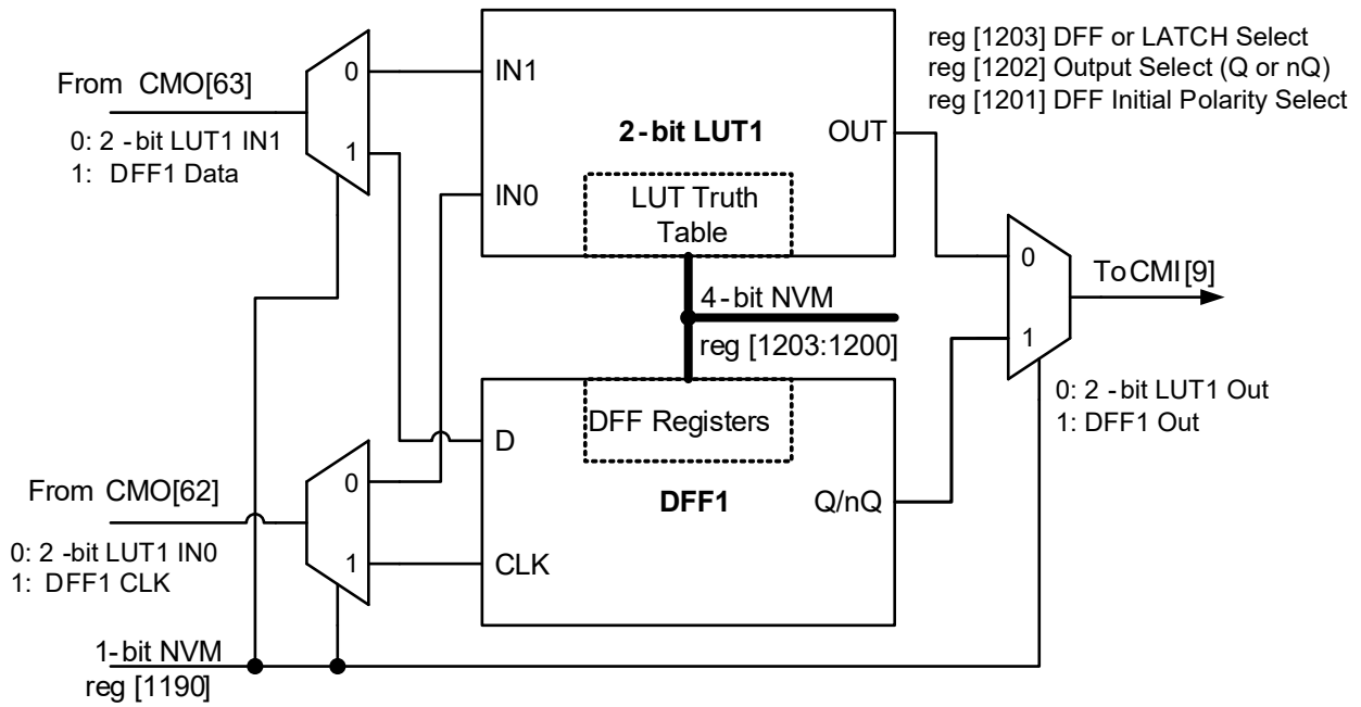
Figure 16. 2-bit LUT1 or DFF1
