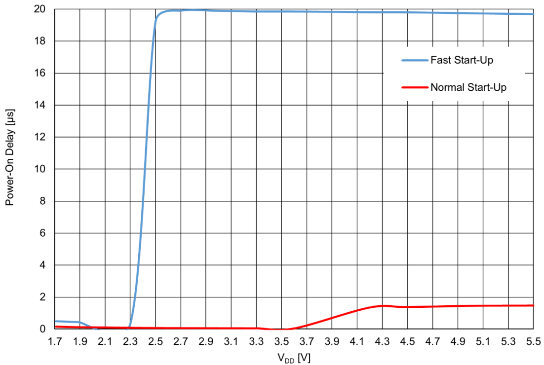
Figure 68. Oscillator Maximum Power-On Delay vs. V DD at T A = +25 °C, OSC0 = 25 kHz
