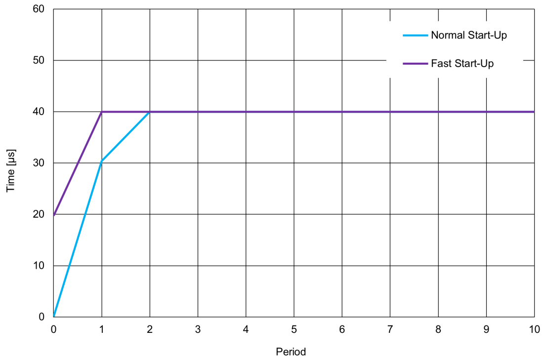
Figure 75. Oscillator0 Settling Time, V_{DD} = 3.3\text{ V} , T_A = +25\text{ }^\circ\text{C} , OSC0 = 25\text{ kHz}
