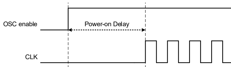
Figure 67. Oscillator Startup Diagram
