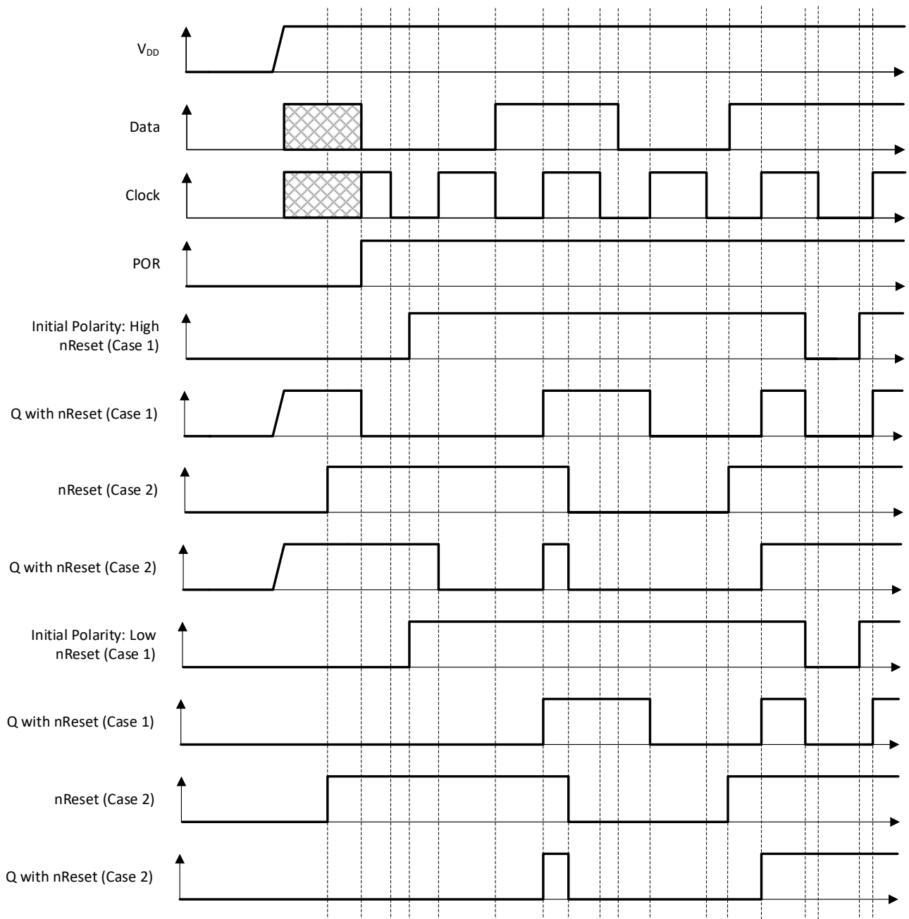
Figure 24. DFF Polarity Operations with nReset
