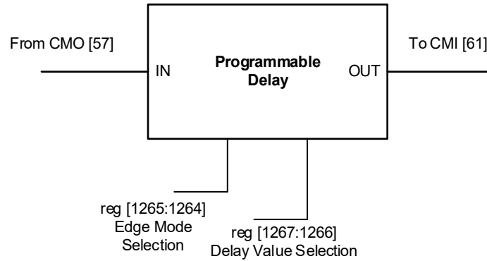
Figure 58. Programmable Delay
