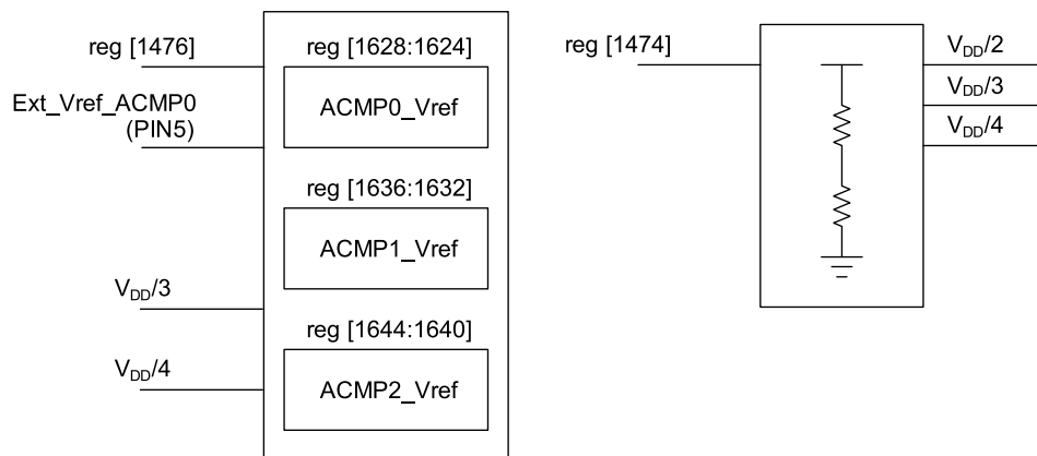
Figure 61. Voltage Reference Block Diagram
