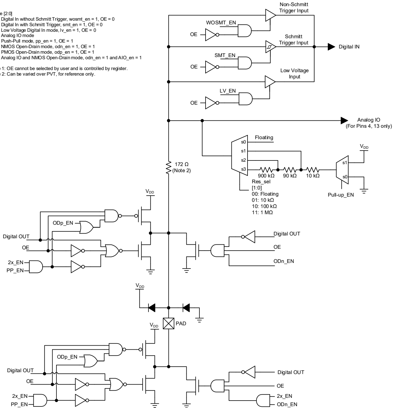
Figure 11. IO Structure Diagram (Pin 3, 4, 13)
