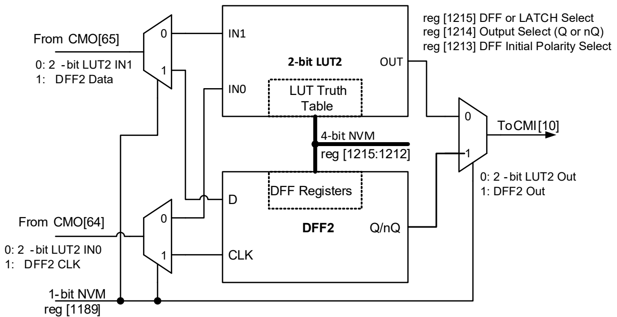
Figure 17. 2-bit LUT2 or DFF2
