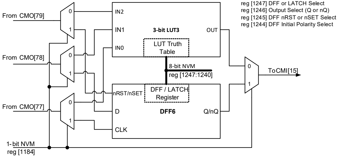
Figure 22. 3-bit LUT3 or DFF6 with RST/SET
