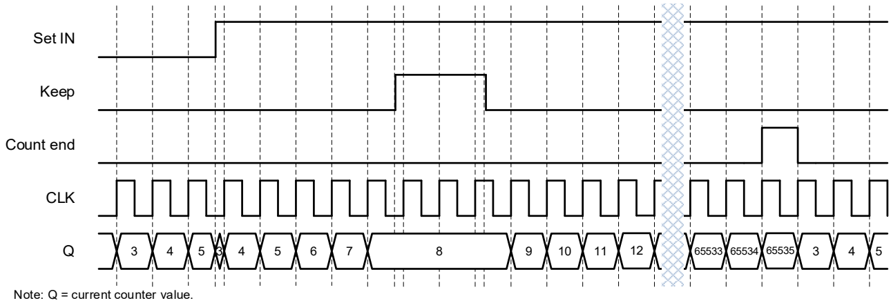
Figure 43. CNT/FSM Timing Diagram (Set Rising Edge Mode, Oscillator is Forced On, UP = 1) for Counter Data = 3
