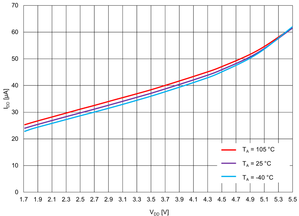
Figure 80. OSC0 (2 MHz) Current Consumption vs. V DD , Pre-Divider = 2
