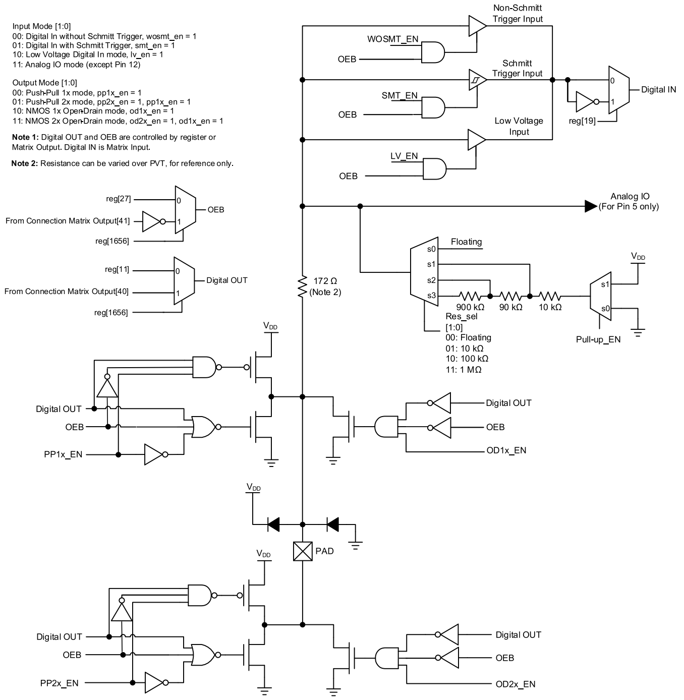
Figure 6. Matrix OE IO Structure Diagram (Pin 11)
