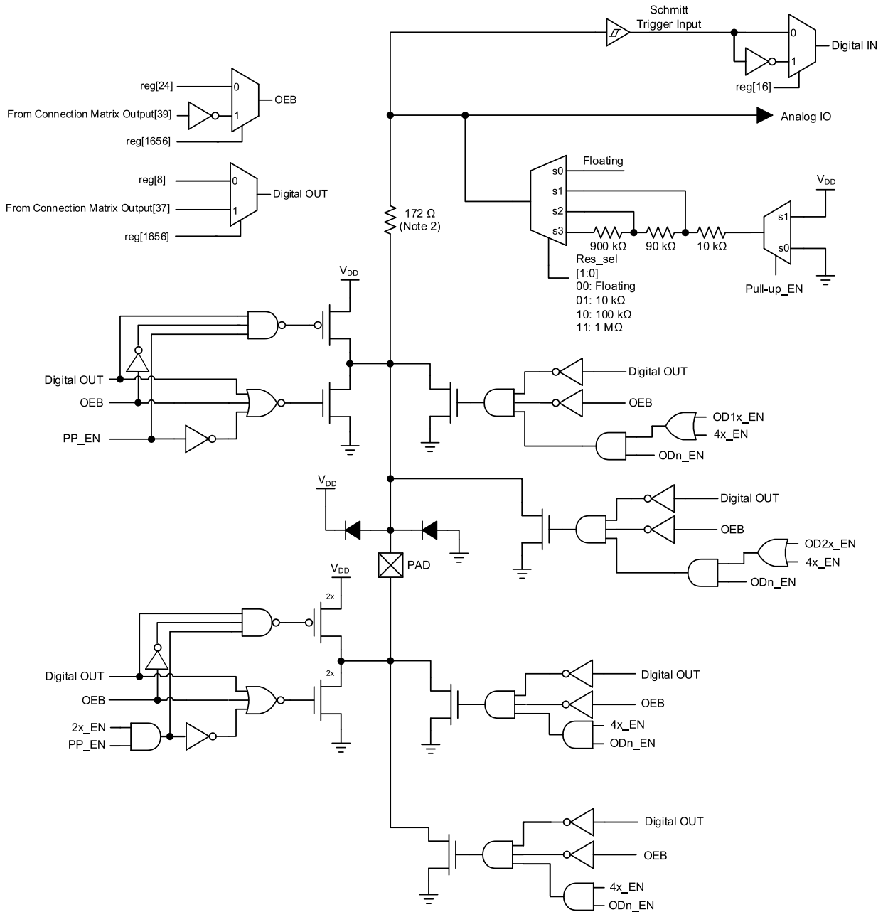
Figure 10. Matrix OE IO 4x Drive Structure Diagram (Pin 10)
