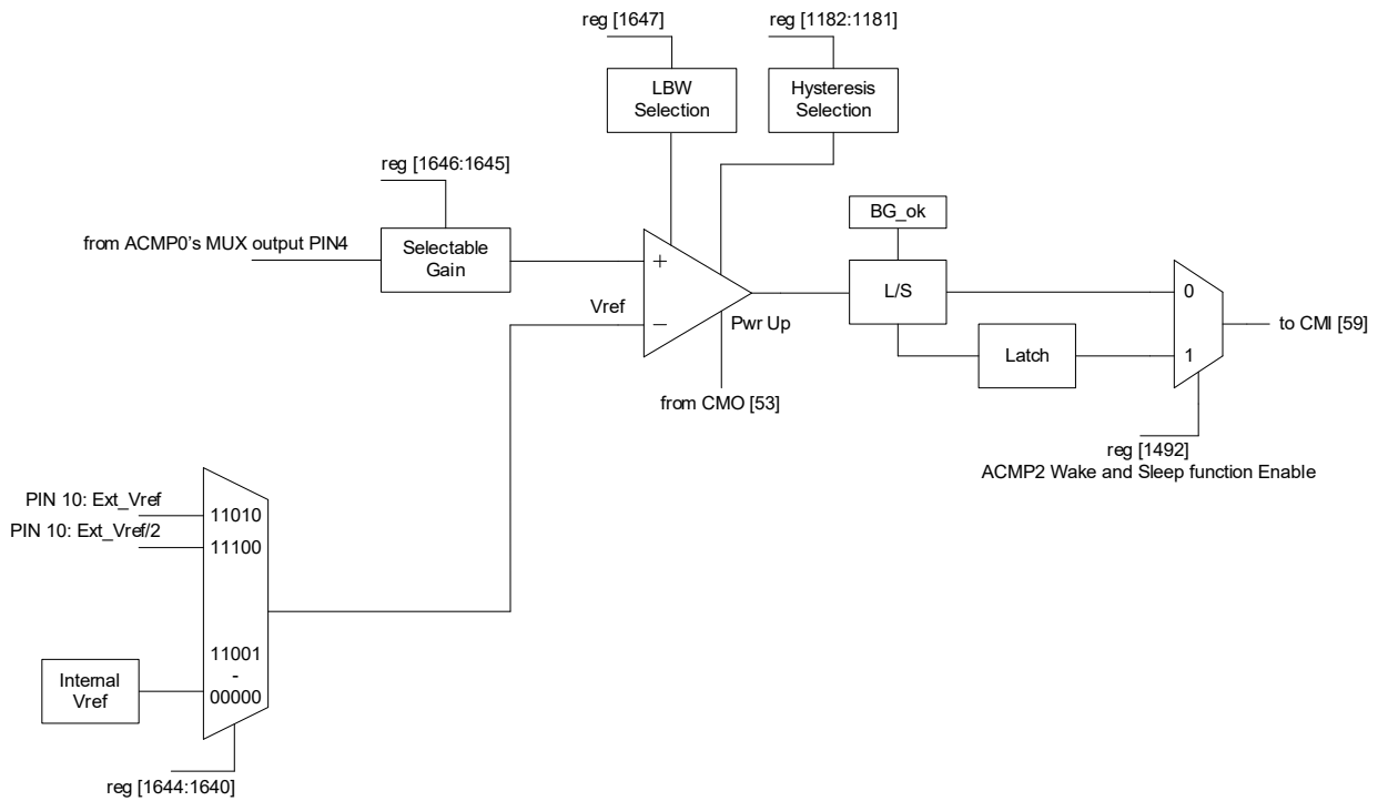
Figure 50. ACMP2 Block Diagram
