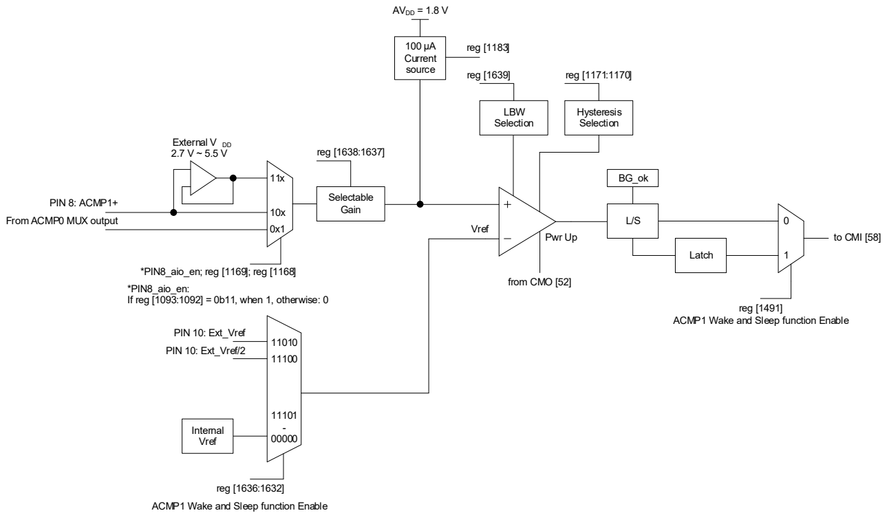
Figure 49. ACMP1 Block Diagram
