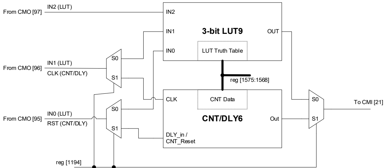
Figure 31. 3-bit LUT9 or CNT/DLY6
