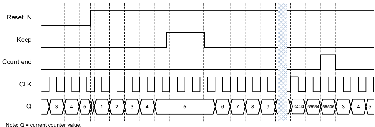
Figure 42. CNT/FSM Timing Diagram (Reset Rising Edge Mode, Oscillator is Forced On, UP = 1) for Counter Data = 3
