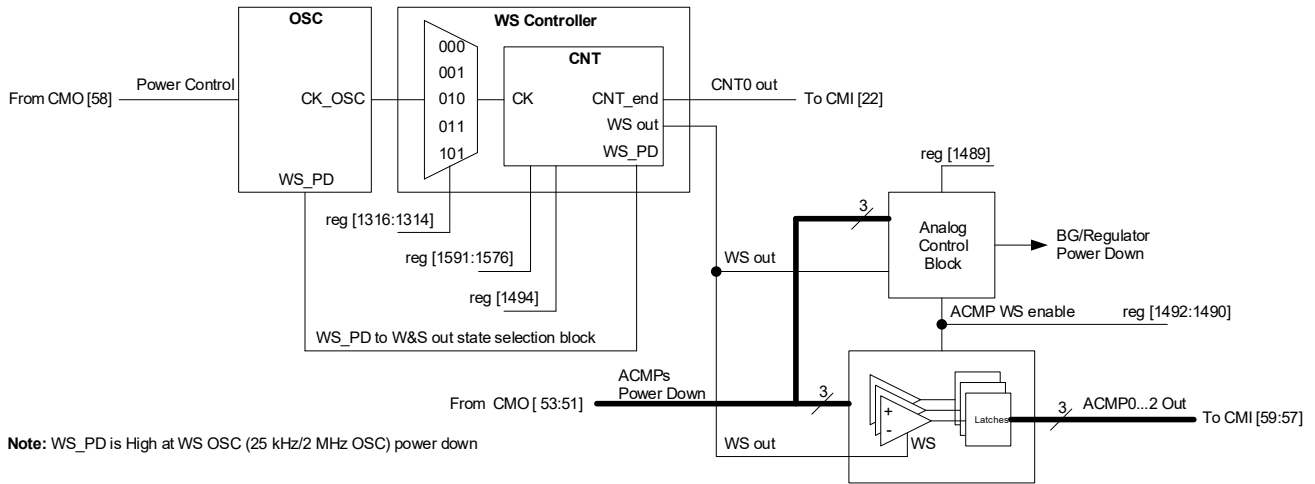
Figure 47. Wake/Sleep Controller
