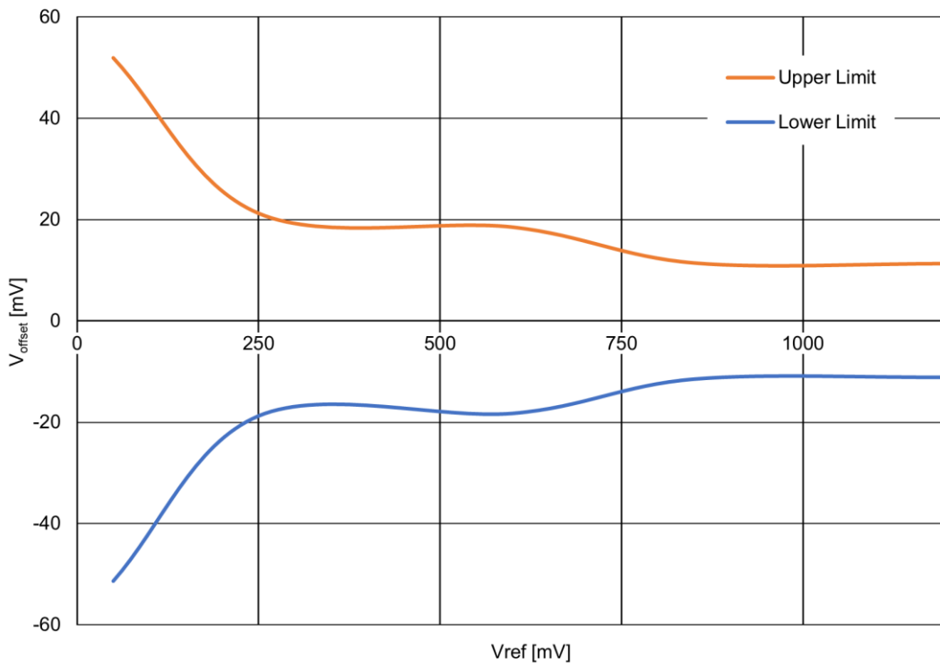
Figure 53. ACMPx Buffer Input Offset Voltage vs. V REF at V DD = 1.71 V to 5.5 V, T A = -40 °C to +85 °C
