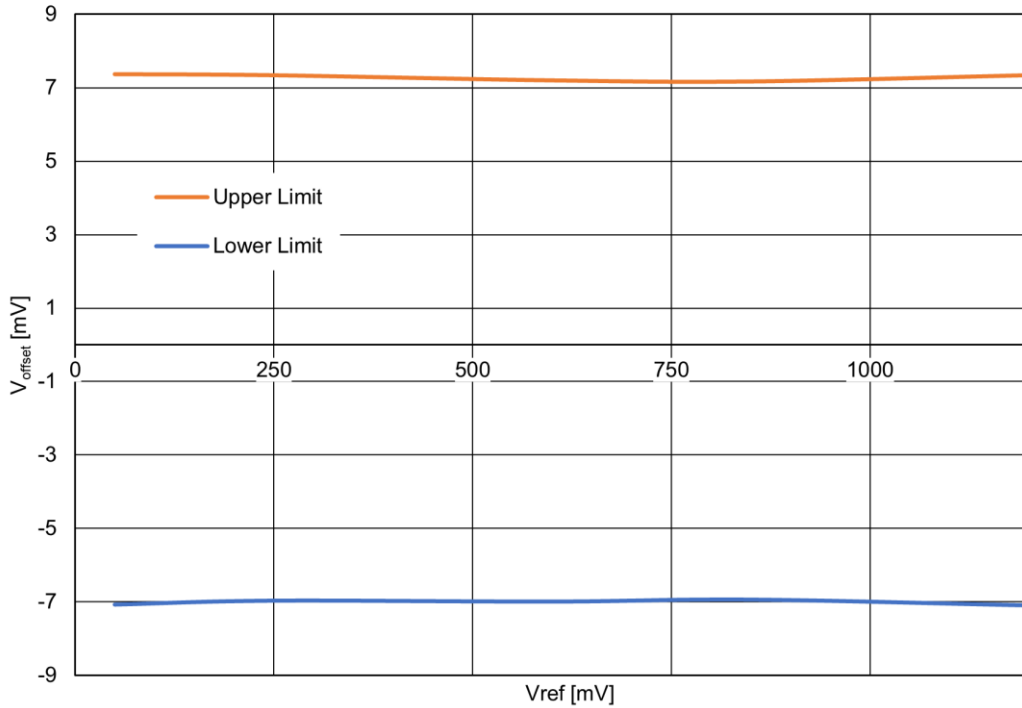
Figure 52. ACMPx Input Offset Voltage vs. V REF at V DD = 1.71 V to 5.5 V, T A = -40 °C to +85 °C
