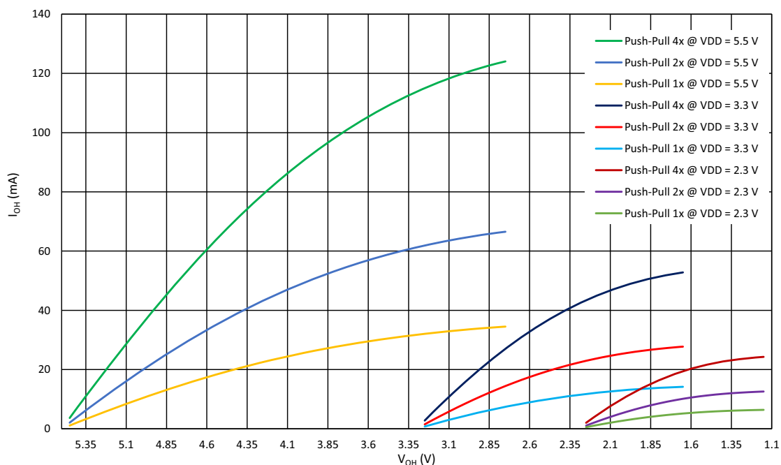
Figure 8. Typical High Level Output Current vs. High Level Output Voltage at T_A = 25^\circ\text{C}
