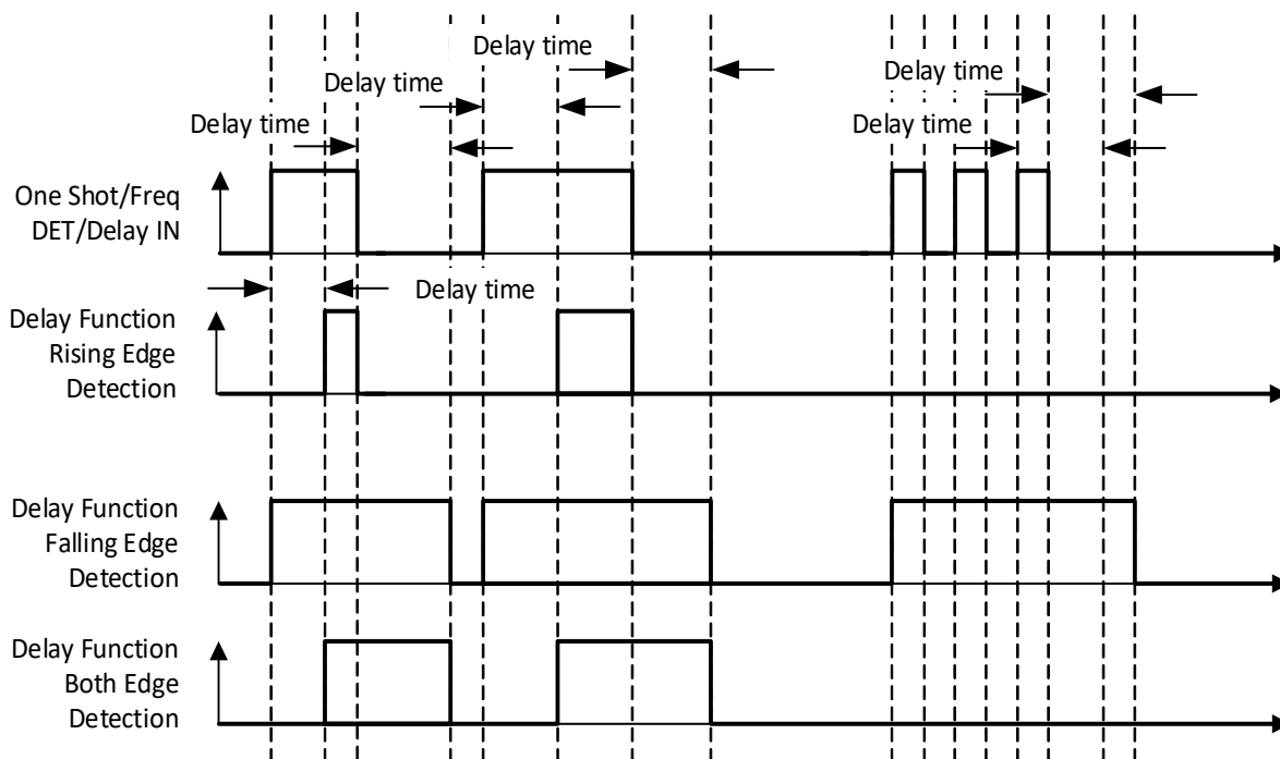
Figure 49. Delay Mode Timing Diagram for Different Edge Select Mode
