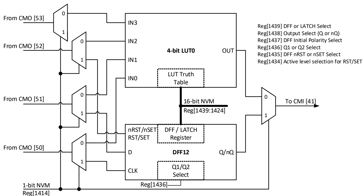
Figure 36. 4-bit LUT0 or DFF12
