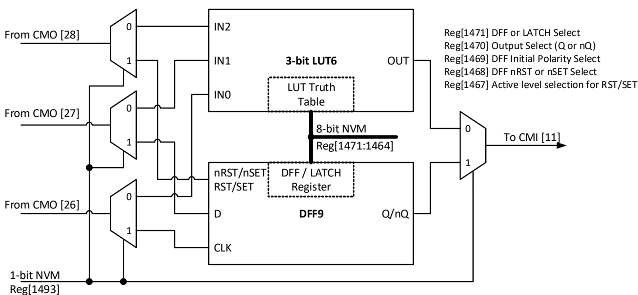
Figure 31. 3-bit LUT6 or DFF9
