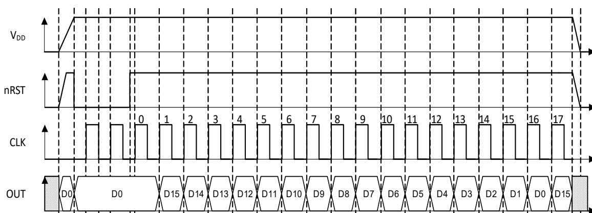
Figure 24. PGen Timing Diagram
