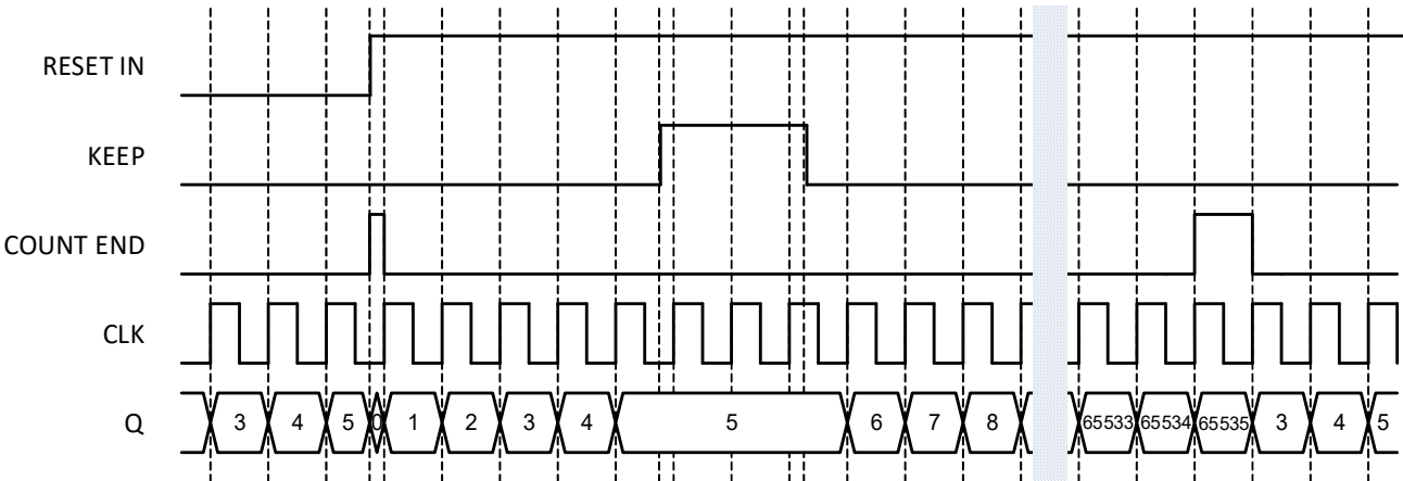
Figure 58. CNT/FSM Timing Diagram (Reset Rising Edge Mode, Oscillator is Forced On, UP = 1)
