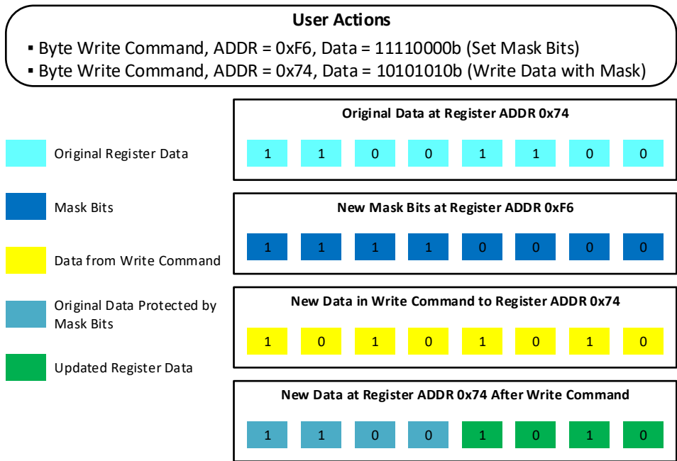
Figure 111. Example of I 2 C Byte Write Bit Masking
