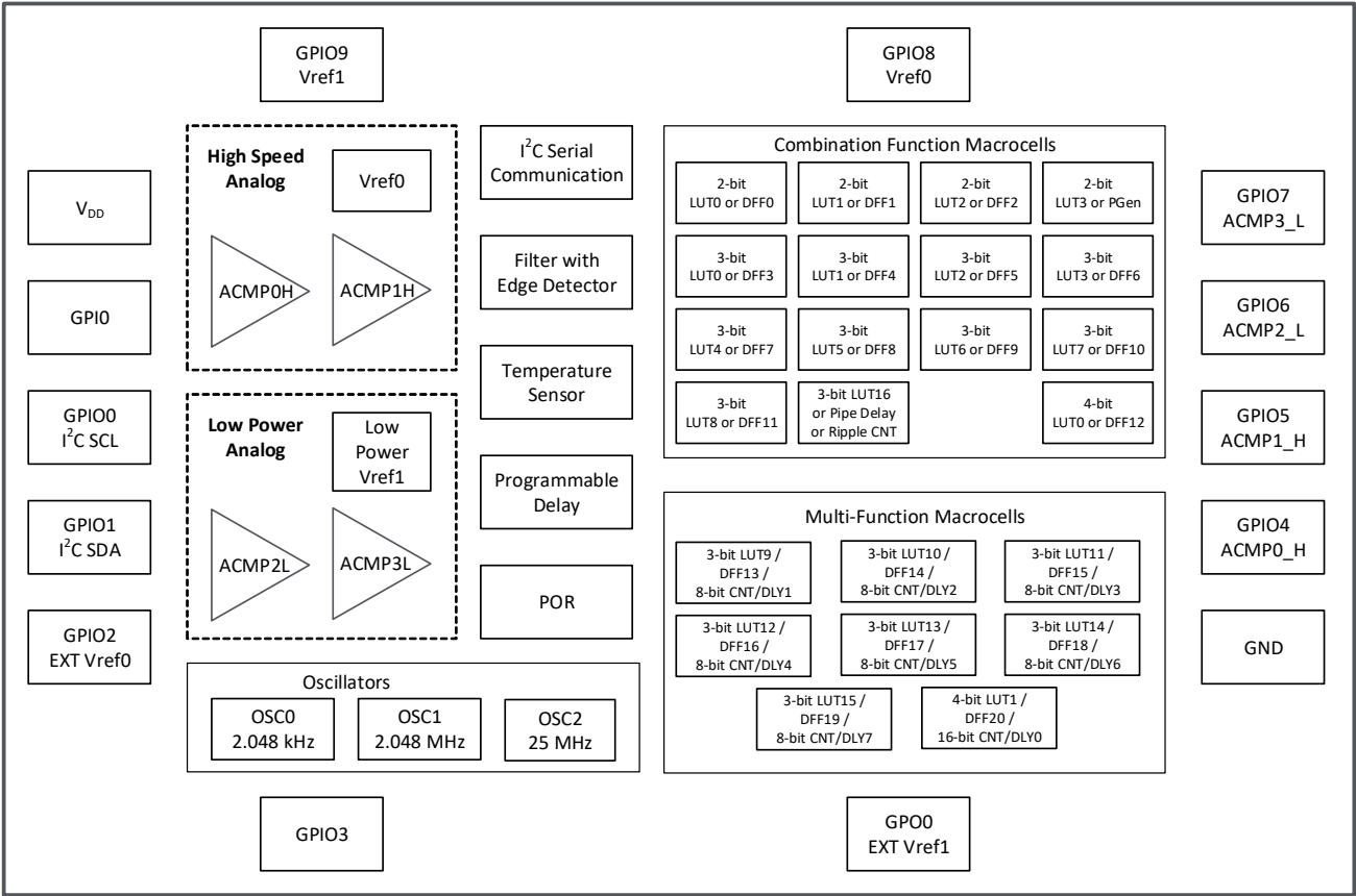
Figure 1. Block Diagram
