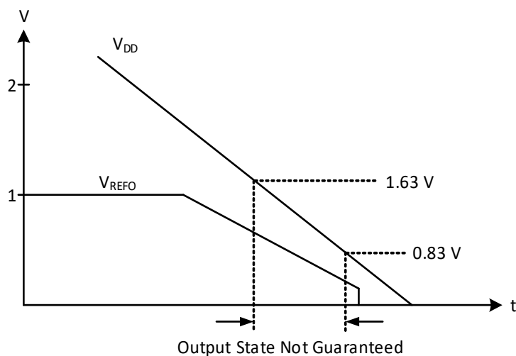
Figure 102. Power-Down
