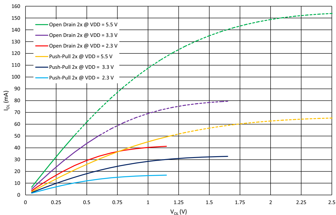
Figure 11. Typical Low Level Output Current vs. Low Level Output Voltage, 2x Drive at T_A = 25^\circ\text{C} , Full Range
