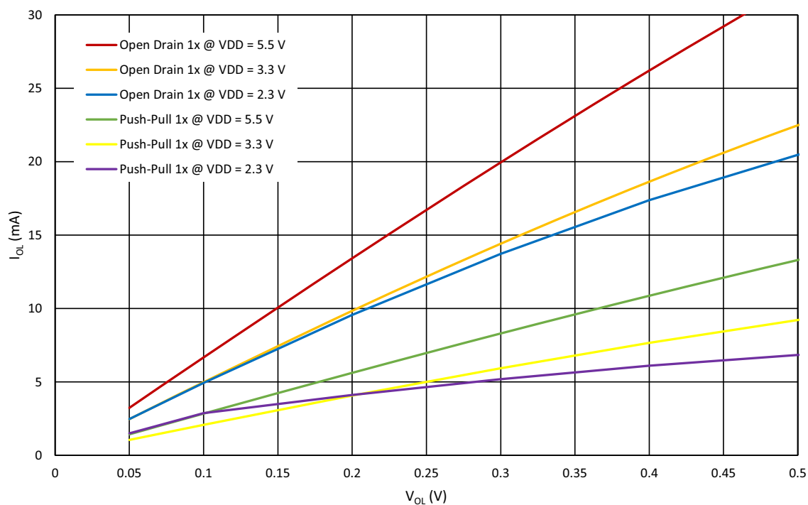
Figure 10. Typical Low Level Output Current vs. Low Level Output Voltage, 1x Drive at T_A = 25^\circ\text{C}
