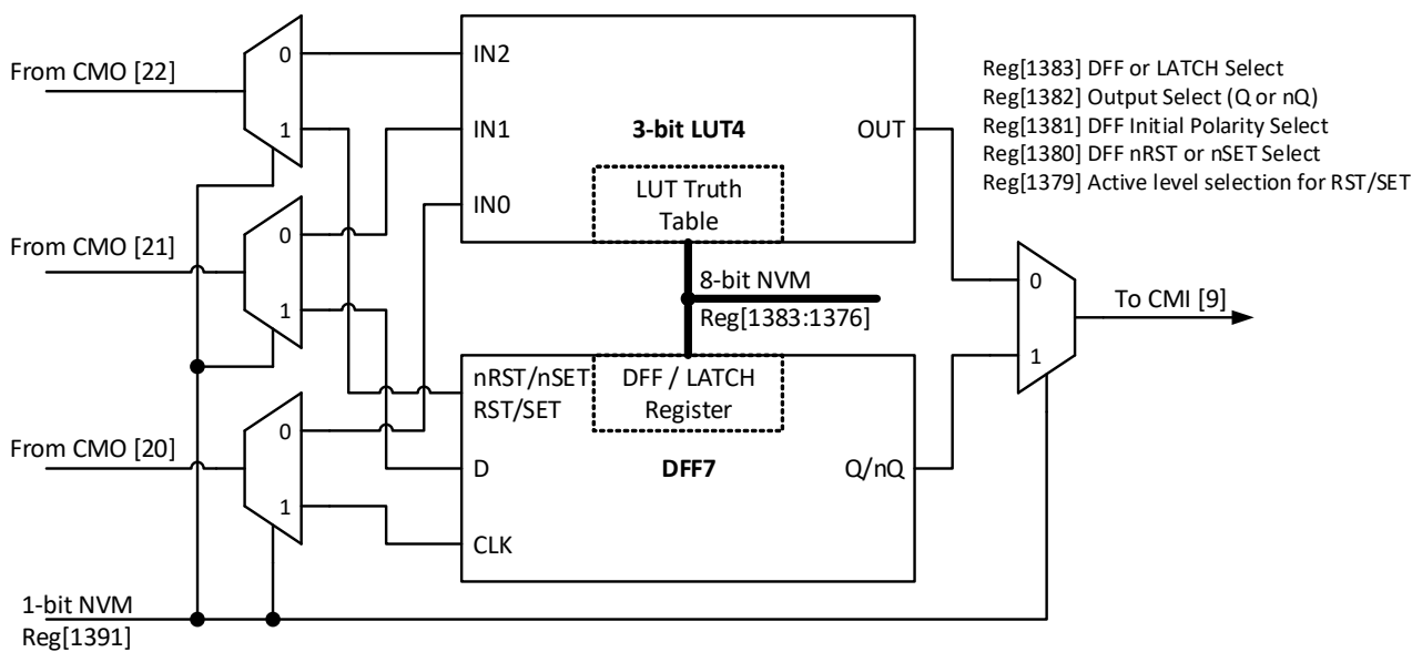
Figure 29. 3-bit LUT4 or DFF7
