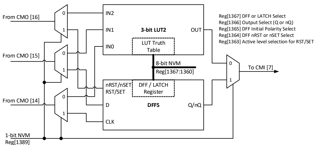
Figure 27. 3-bit LUT2 or DFF5
