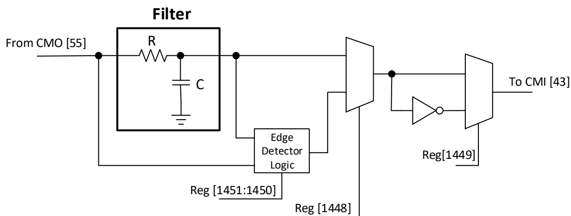
Figure 78. Deglitch Filter/Edge Detector
