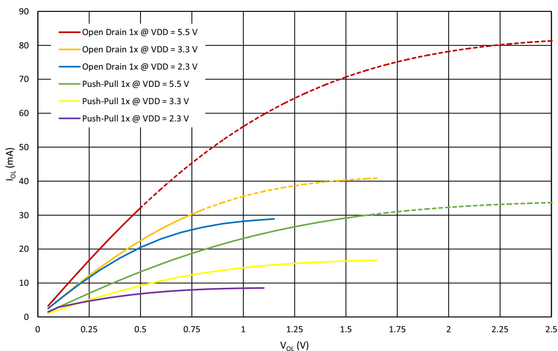
Figure 9. Typical Low Level Output Current vs. Low Level Output Voltage, 1x Drive at T_A = 25^\circ\text{C} , Full Range
