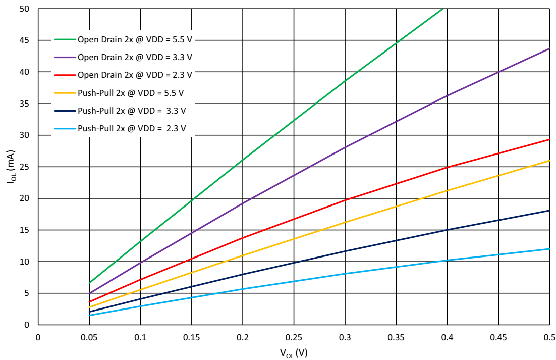
Figure 12. Typical Low Level Output Current vs. Low Level Output Voltage, 2x Drive at T_A = 25^\circ\text{C}
