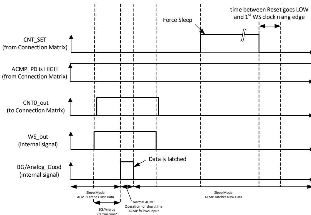
Figure 65. Wake/Sleep Timing Diagram, Short Wake Mode, Counter Set is Used
