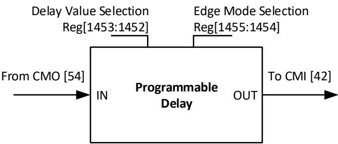
Figure 76. Programmable Delay
