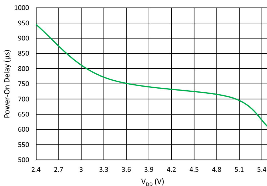
Figure 89. Oscillator0 Maximum Power-On Delay vs. V_{DD} at T_A = 25\text{ }^{\circ}\text{C} , OSC0 = 2.048 kHz
