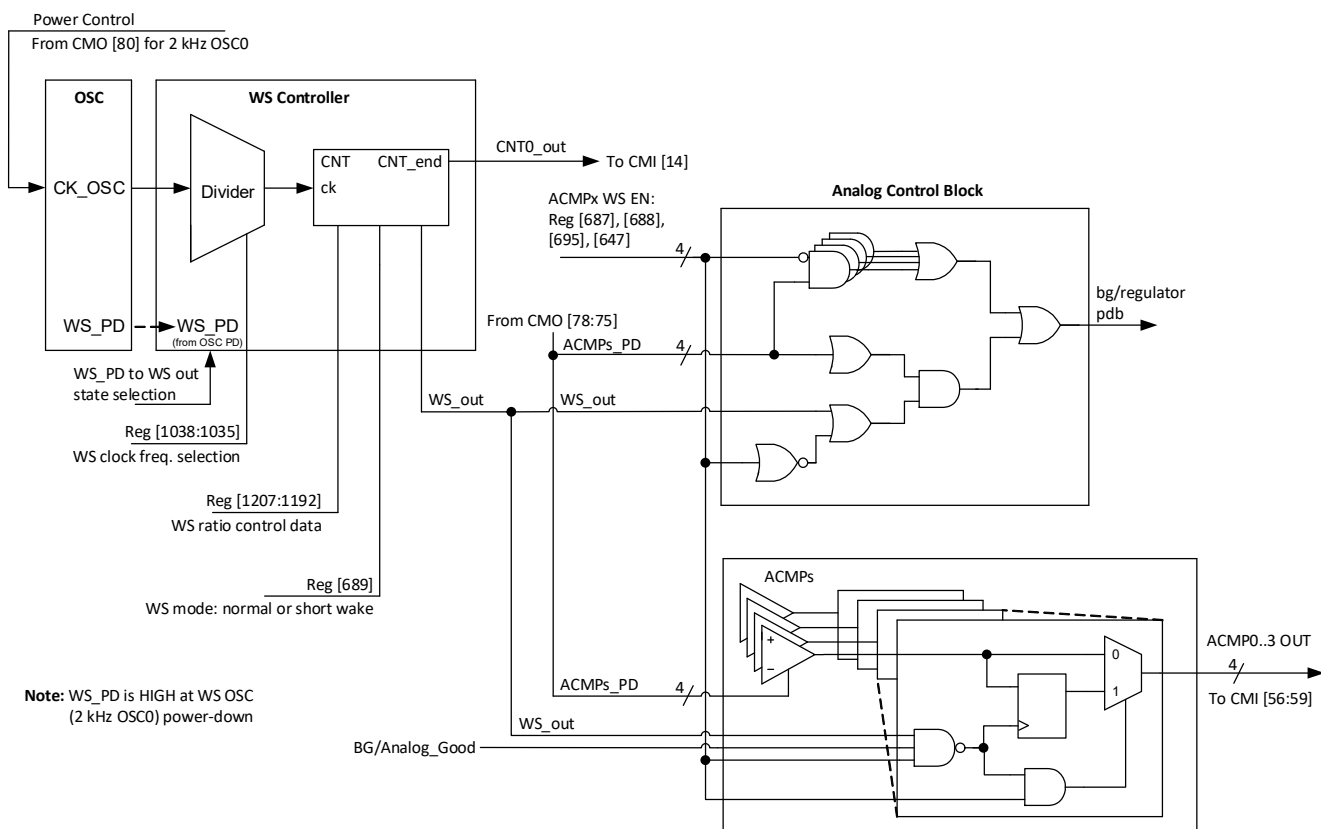
Figure 61. Wake/Sleep Controller
