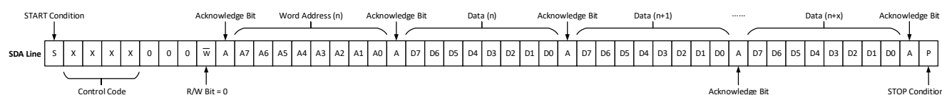
Figure 106. Sequential Write Command
