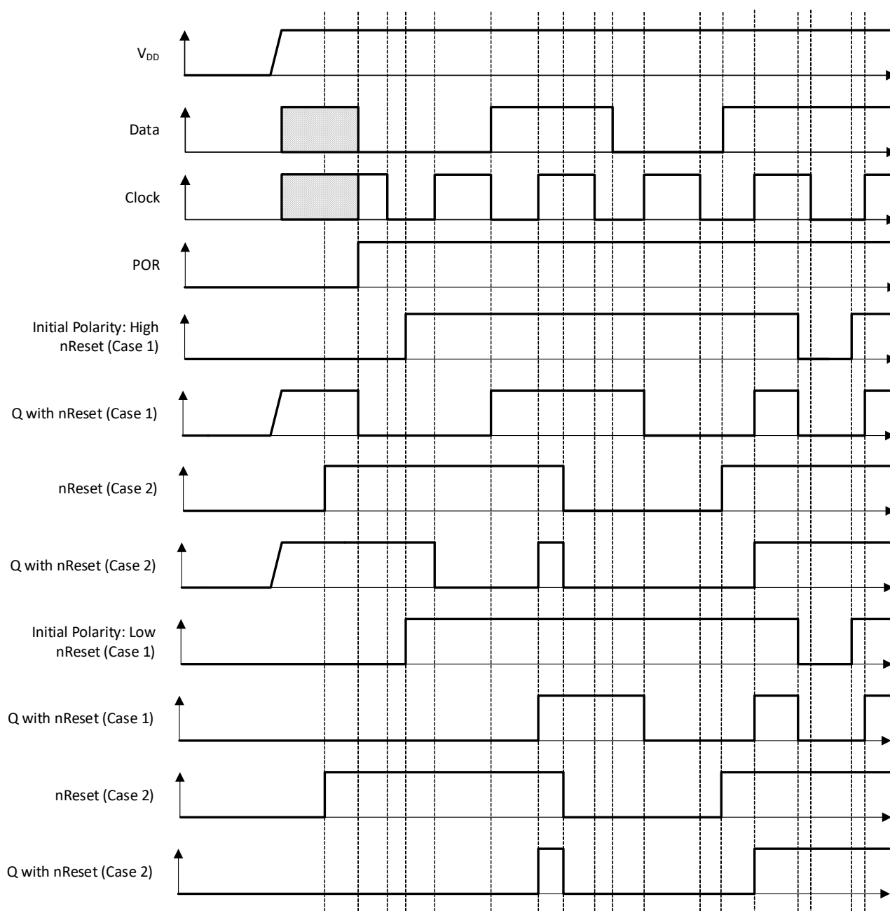
Figure 34. DFF Polarity Operations with nReset
