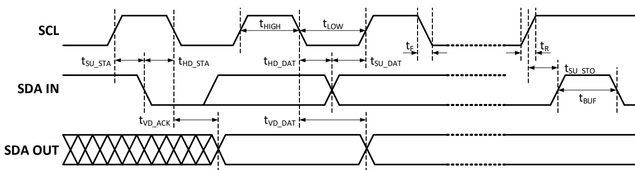
Figure 104. I 2 C General Timing Characteristics
