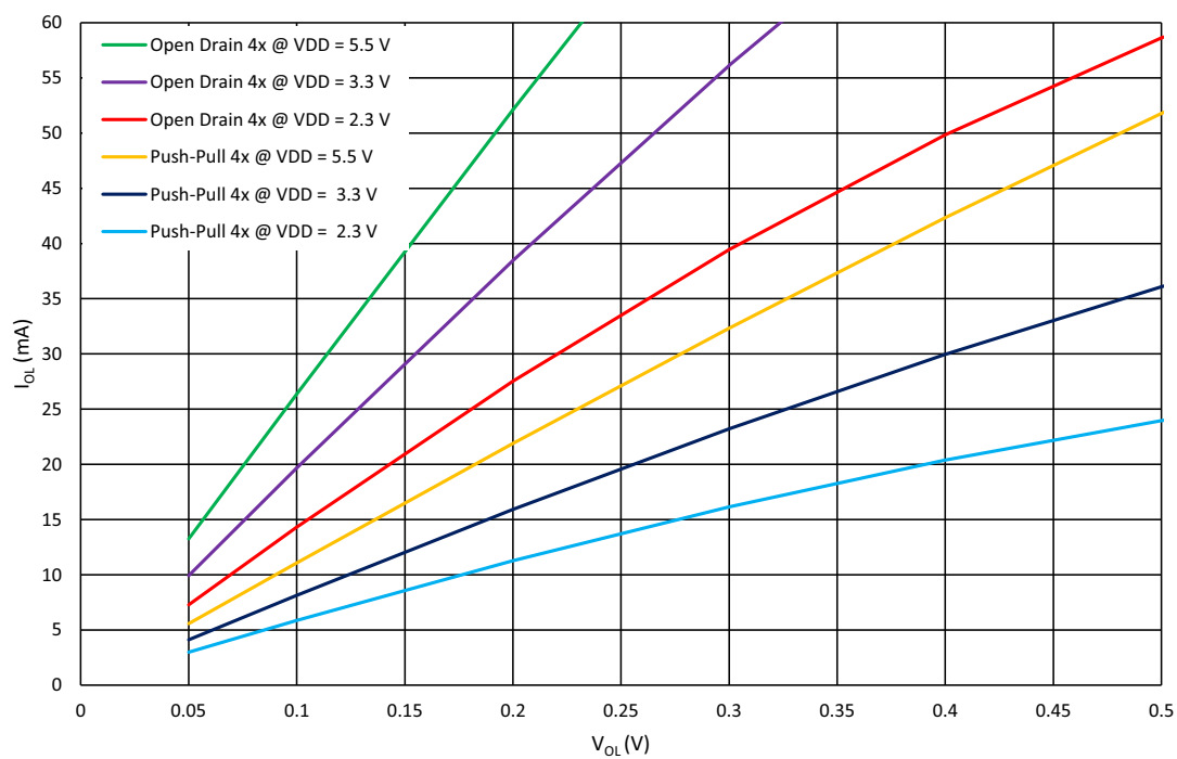
Figure 16. Typical Low Level Output Current vs. Low Level Output Voltage, 4x Drive at T_A = 25^\circ\text{C}
