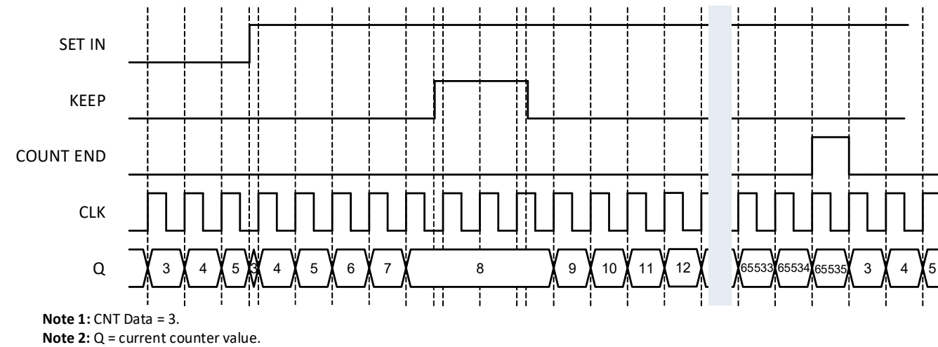
Figure 59. CNT/FSM Timing Diagram (Set Rising Edge Mode, Oscillator Is Forced On, UP = 1)
