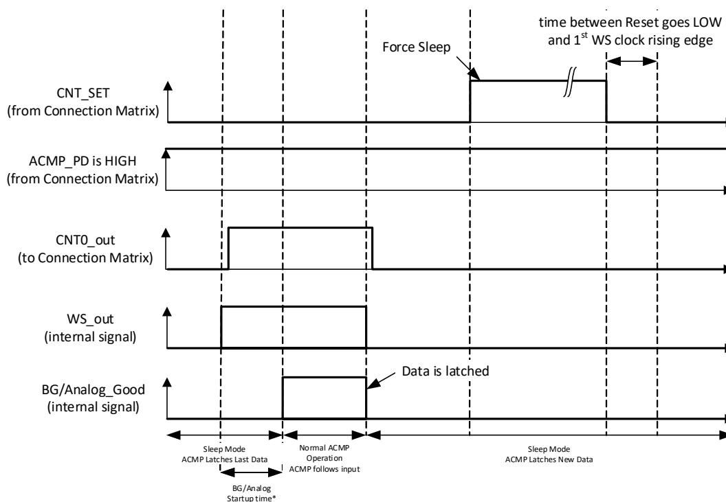
Figure 64. Wake/Sleep Timing Diagram, Normal Wake Mode, Counter Set is Used
