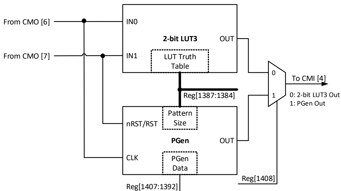
Figure 23. 2-bit LUT3 or PGen
