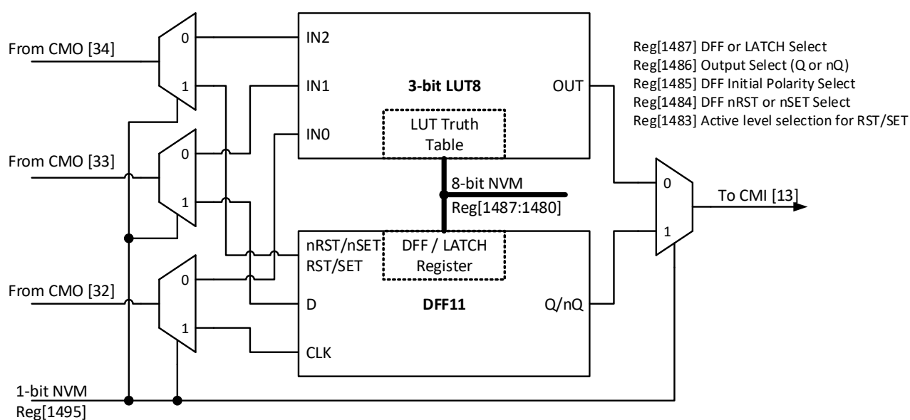
Figure 33. 3-bit LUT8 or DFF11
