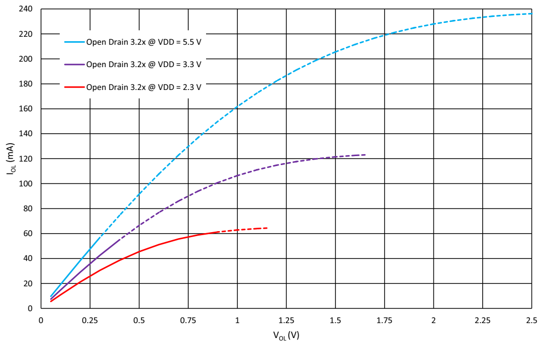
Figure 13. Typical Low Level Output Current vs. Low Level Output Voltage, 3.2x Drive at T_A = 25^\circ\text{C} , Full Range
