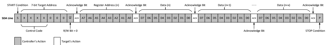
Figure 156. Sequential Write Command
