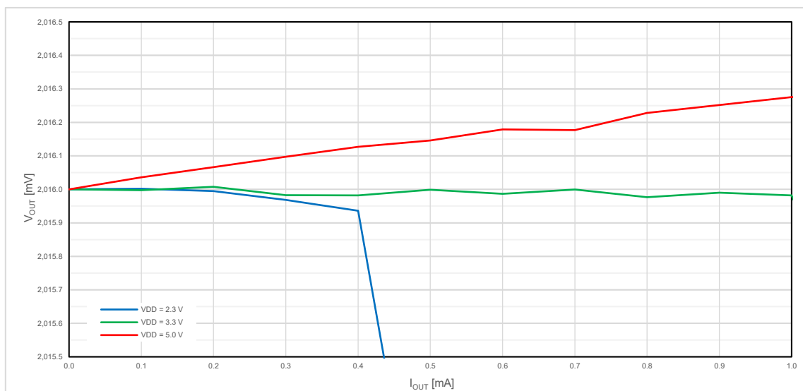
Figure 60. Typical Load Regulation in Source Mode at V_{REF} = 2016 mV, T_A = -40 °C to +105 °C
