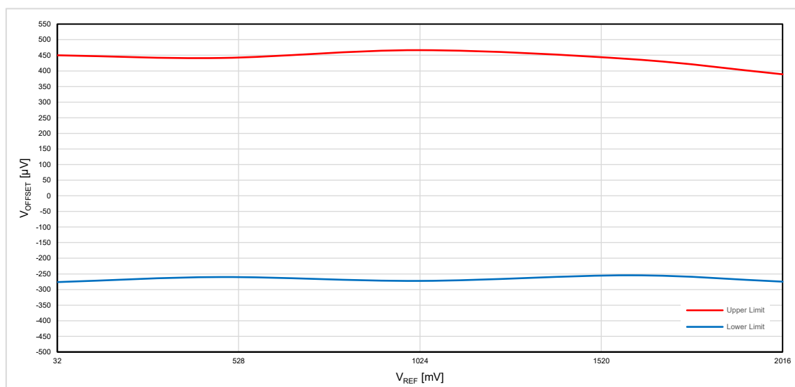
Figure 111. MS-ACMP Input Offset Voltage vs. V_{REF} at V_{DD} = 2.3 \text{ V to } 5.5 \text{ V} , Gain = 1, T_A = -40^\circ\text{C to } +105^\circ\text{C}
