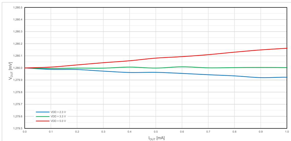
Figure 59. Typical Load Regulation in Source Mode at V_{REF} = 1280 mV, T_A = -40 °C to +105 °C
