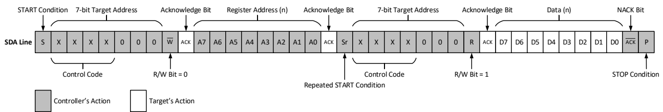
Figure 158. Random Read Command
