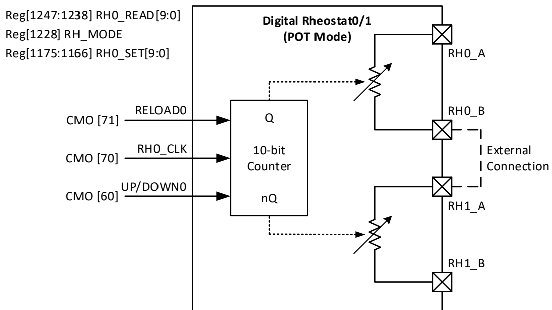
Figure 116. Two Rheostats in Potentiometer Mode
