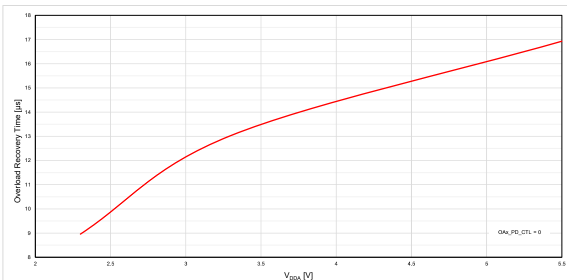
Figure 95. OpAmp Overload Recovery Time vs. V_{DDA} at G = 1 , R_{LOAD} = 50 k \Omega , Rising
