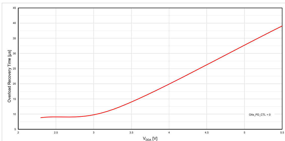
Figure 96. OpAmp Overload Recovery Time vs. V_{DDA} at G = 1 , R_{LOAD} = 50 k \Omega , Falling
