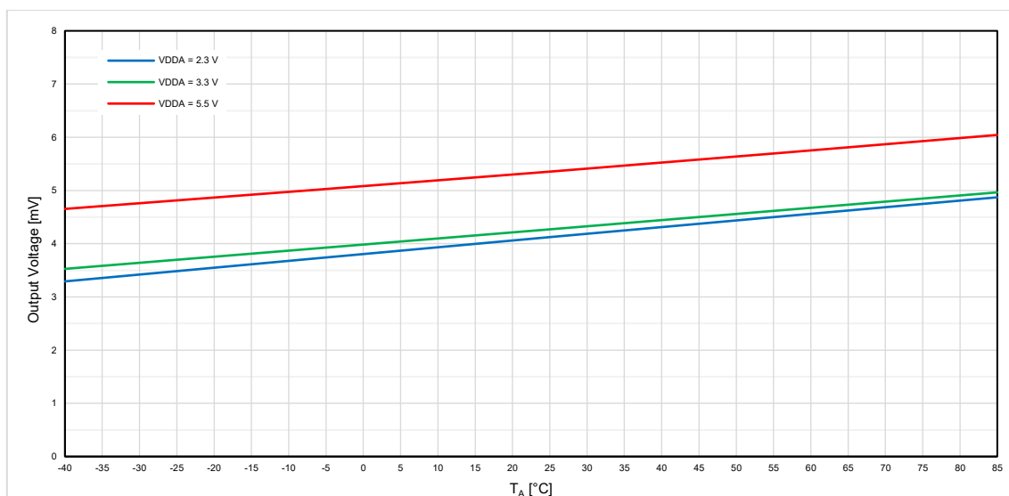
Figure 94. OpAmp Output Voltage High ( V_{DDA} - V_{OAX\_OUT} ) vs. T_A at R_{LOAD} = 50 k \Omega
