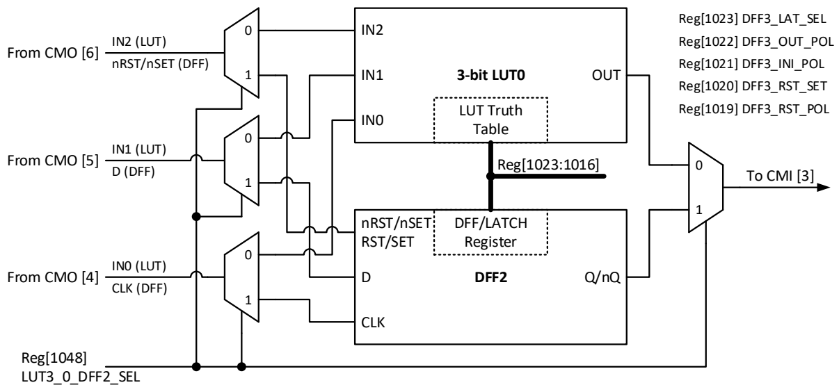
Figure 18. 3-bit LUT0 or DFF2
