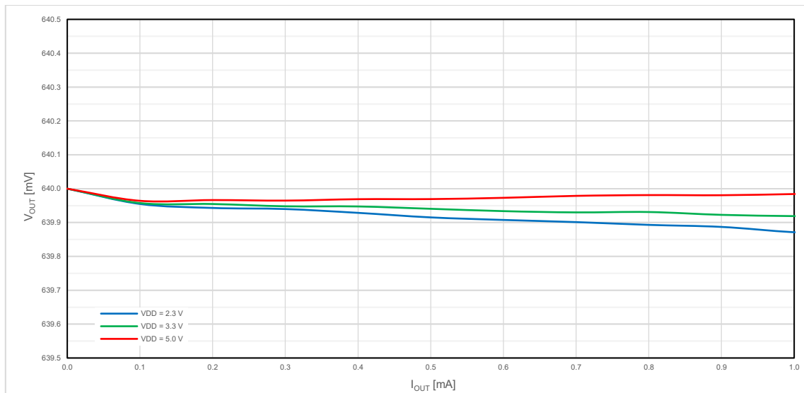
Figure 58. Typical Load Regulation in Source Mode at V_{REF} = 640 mV, T_A = -40 °C to +105 °C
