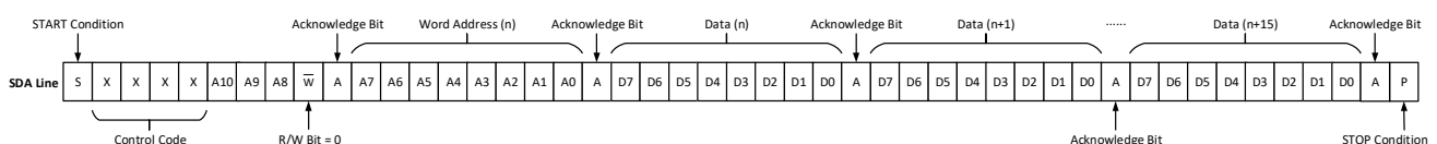
Figure 246. Page Write Command
