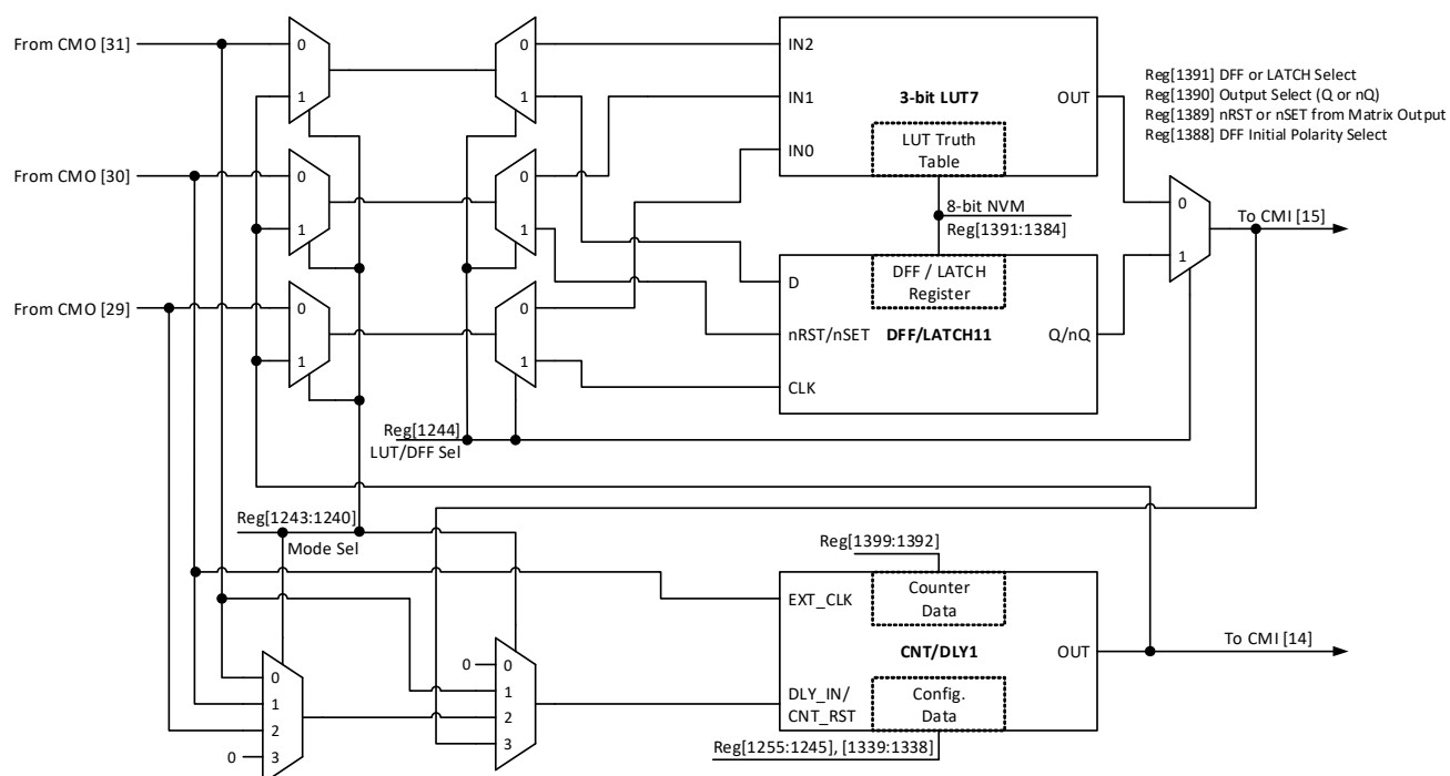
Figure 33. 8-bit Multi-Function Macrocells Block Diagram (3-bit LUT7/DFF11, CNT/DLY1)
