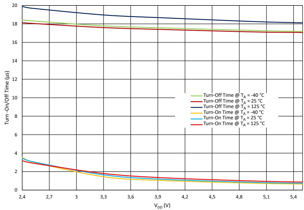
Figure 164. Opampx Turn-On/Off Time vs. V_{DD} at V_{IN} = V_{DD}/2 , BW = 8 \text{ MHz}
