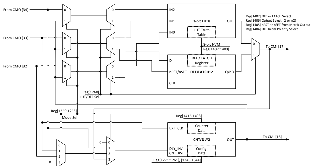
Figure 34. 8-bit Multi-Function Macrocells Block Diagram (3-bit LUT8/DFF12, CNT/DLY2)
