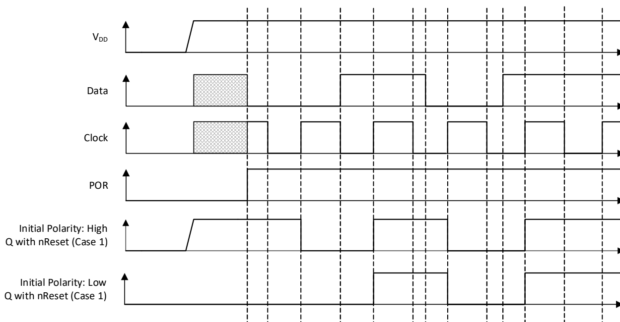
Figure 17. DFF Polarity Operations
