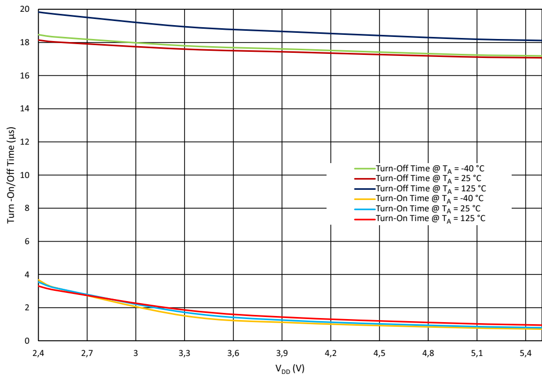
Figure 163. Opampx Turn-On/Off Time vs. V_{DD} at V_{IN} = V_{DD}/2 , BW = 2 \text{ MHz}
