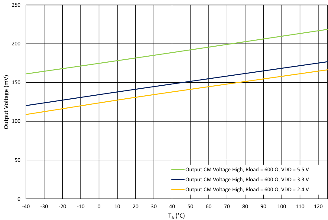
Figure 149. Output Voltage High ( V_{DDA} - V_{OUT} ) vs. Ambient Temperature at BW = 2 \text{ MHz} , R_{LOAD} = 600 \Omega
