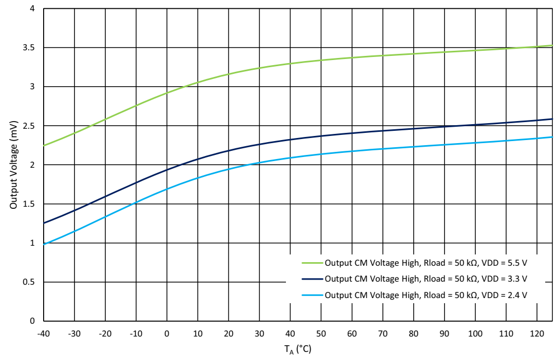
Figure 150. Output Voltage High ( V_{DDA} - V_{OUT} ) vs. Ambient Temperature at BW = 2 \text{ MHz} , R_{LOAD} = 50 k\Omega
