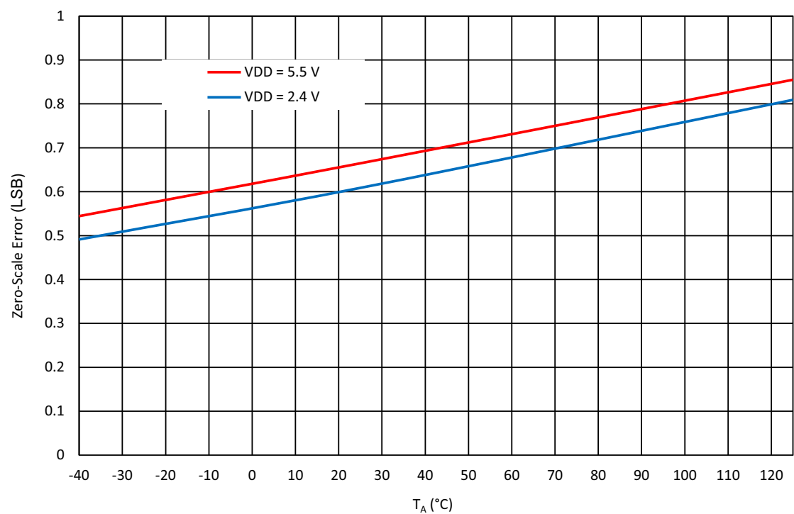
Figure 187. RHx Zero Scale Error vs. Ambient Temperature ( V_{IN} = 1\text{ V} )
