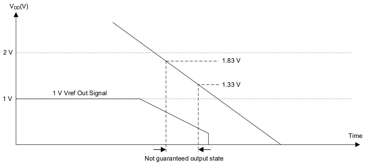
Figure 130. Power-Down
