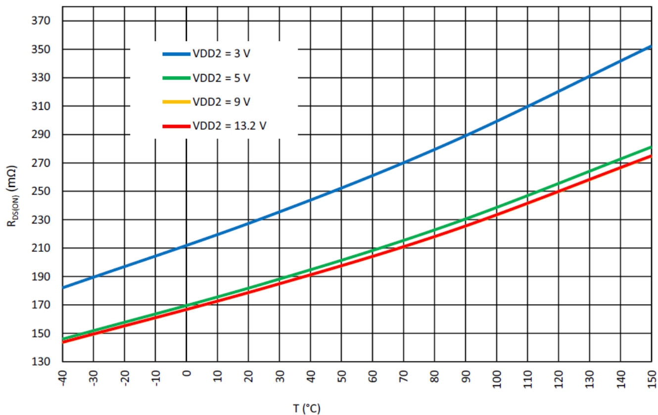
Figure 22. Full Bridge Typical Drain-Source Low Side On-Resistance vs. Temperature at I_{LOAD} = 0.5\text{ A} , V_{DD} = 2.3\text{ V}
