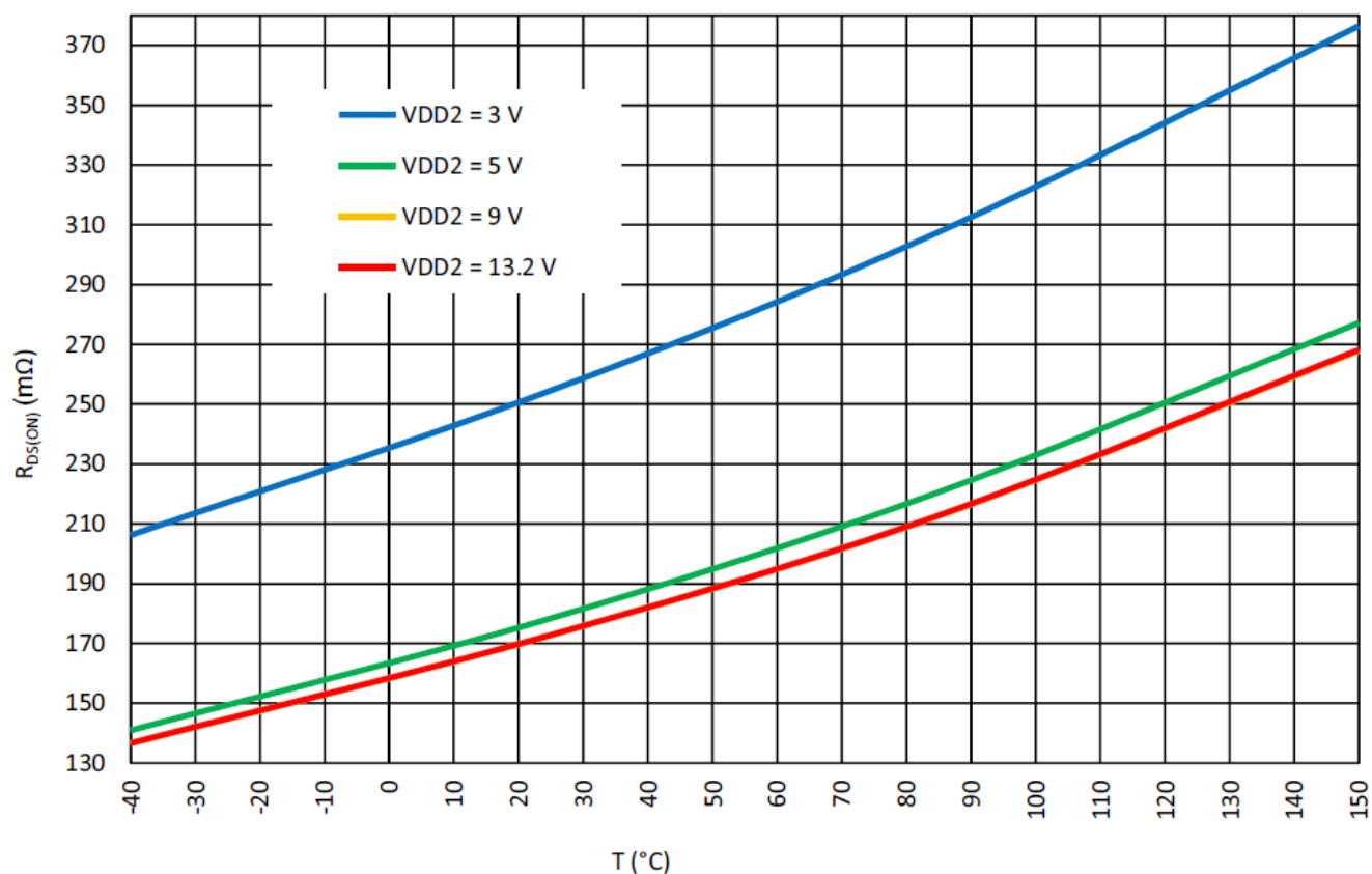
Figure 20. Full Bridge Typical Drain-Source High Side On-Resistance vs. Temperature at I_{LOAD} = 0.5 A, V_{DD} = 2.3 V
