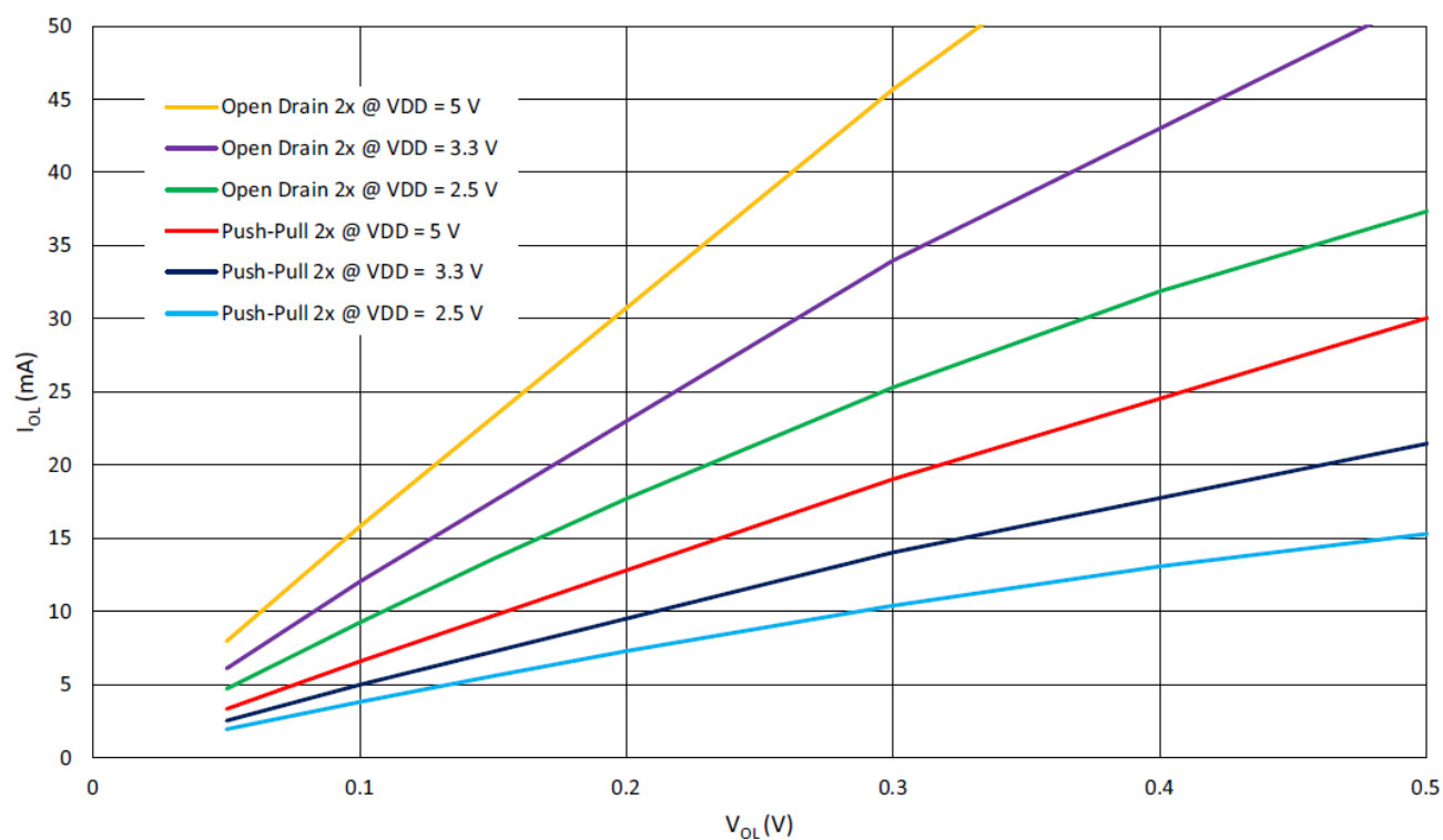
Figure 12. Typical Low Level Output Current vs. Low Level Output Voltage, 2x Drive at T = +25\text{ }^{\circ}\text{C}
