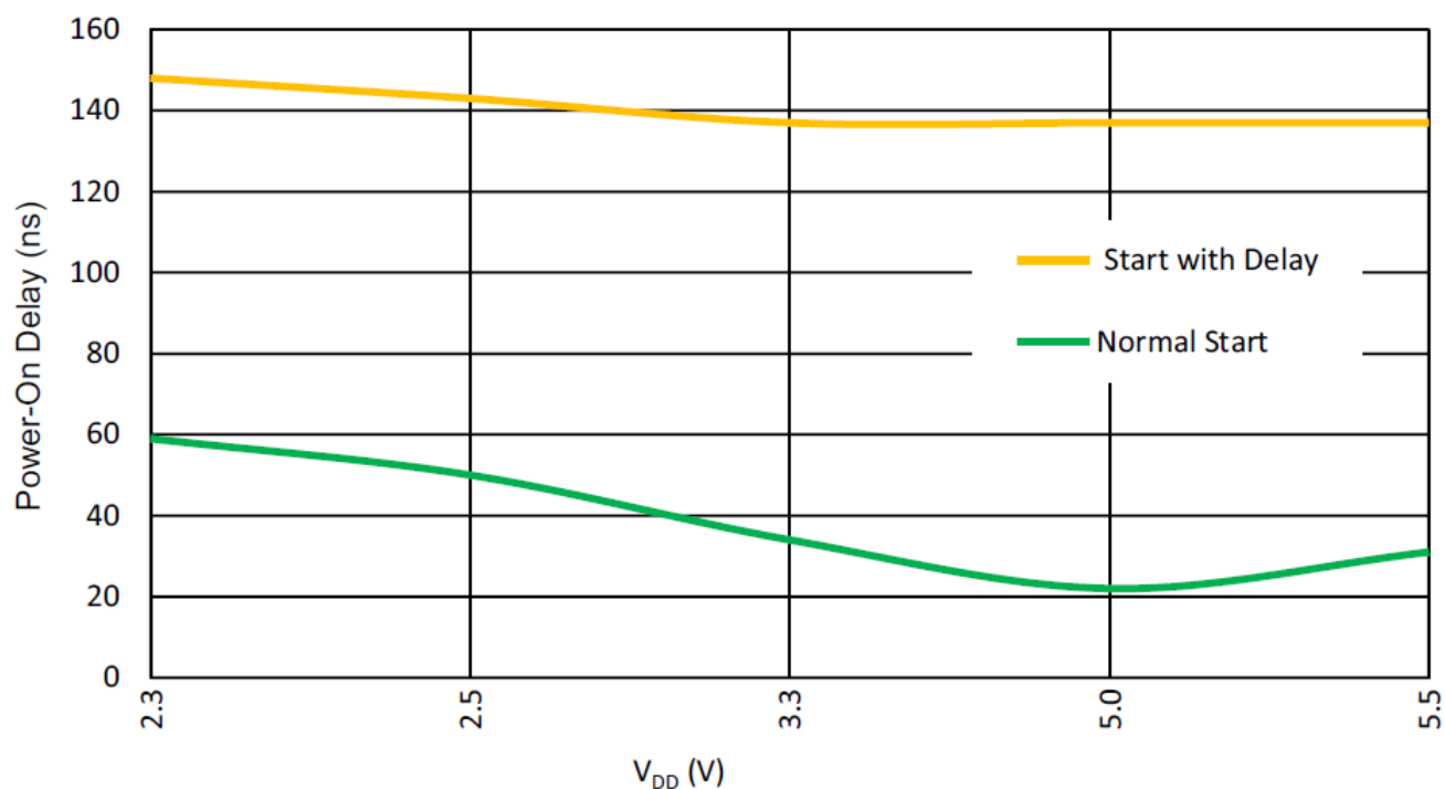
Figure 115. Oscillator1 Maximum Power-On Delay vs. V_{DD} at T = +25^{\circ}\text{C} , \text{OSC1} = 25\text{ MHz}
