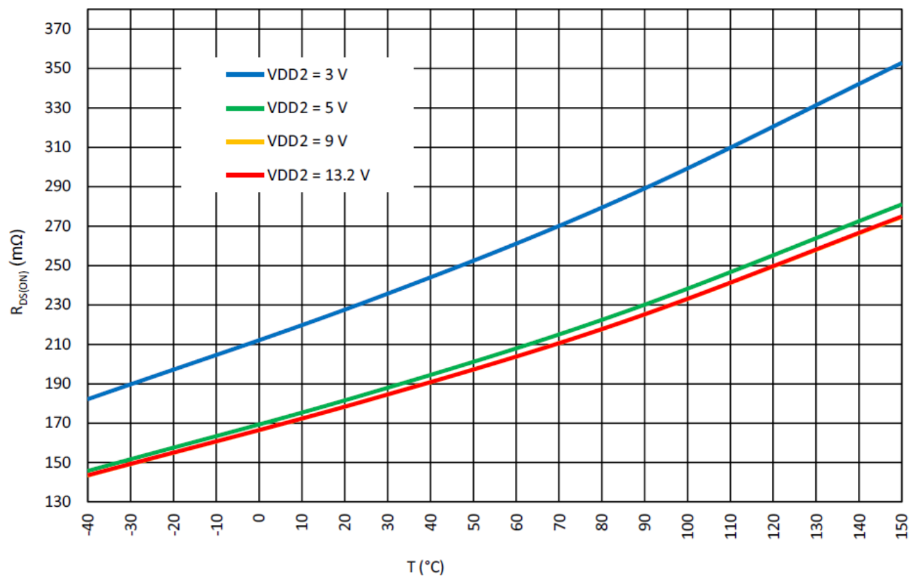
Figure 23. Full Bridge Typical Drain-Source Low Side On-Resistance vs. Temperature at I_{LOAD} = 0.5\text{ A} , V_{DD} = 5.5\text{ V}
