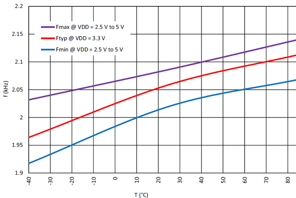
Figure 116. Oscillator0 Frequency vs. Temperature, \text{OSC0} = 2.048\text{ kHz}
