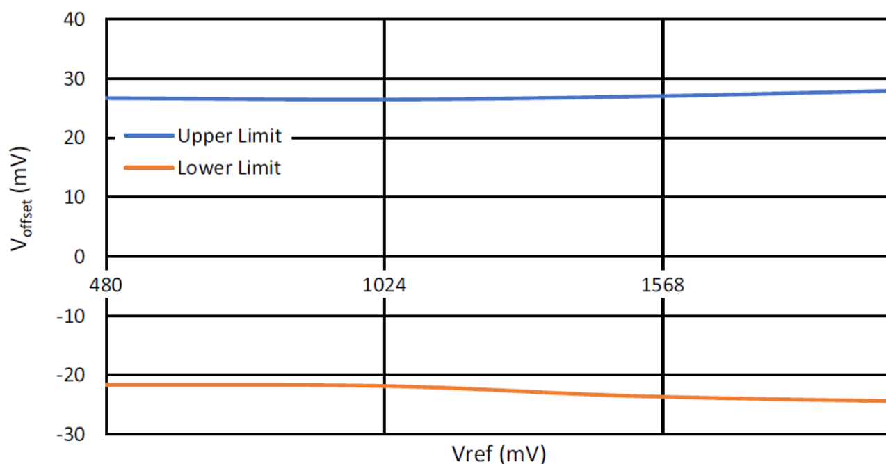
Figure 35. Input Offset Voltage Error vs. V_{\text{REF}} for CCMP (including Amplifier Offset and ACMP Offset)
