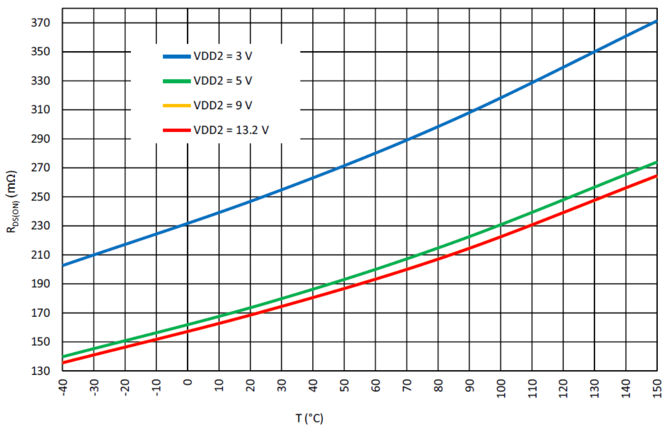
Figure 21. Full Bridge Typical Drain-Source High Side On-Resistance vs. Temperature at I_{LOAD} = 0.5 A, V_{DD} = 5.5 V
