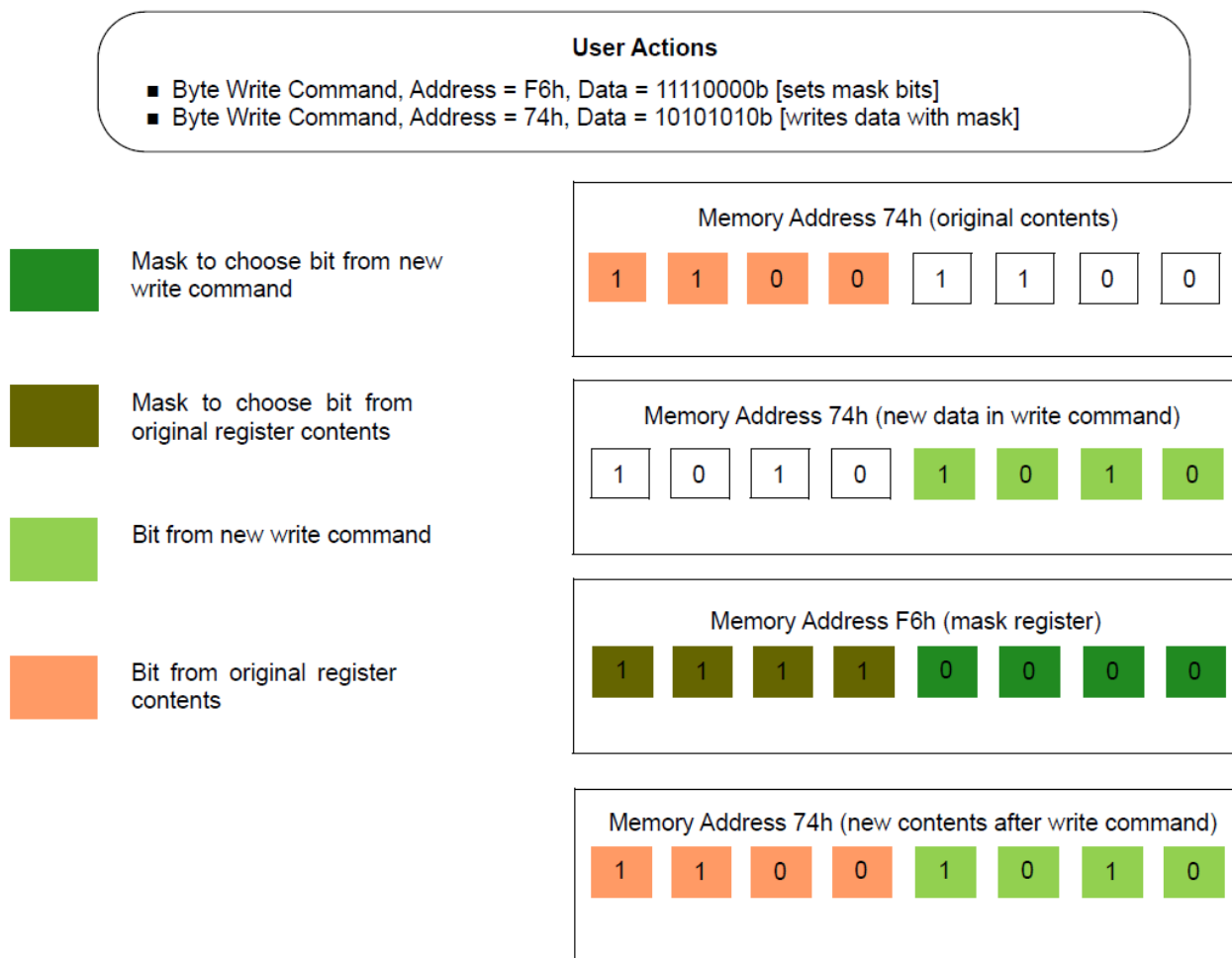
Figure 139. Example of I 2 C Byte Write Bit Masking
