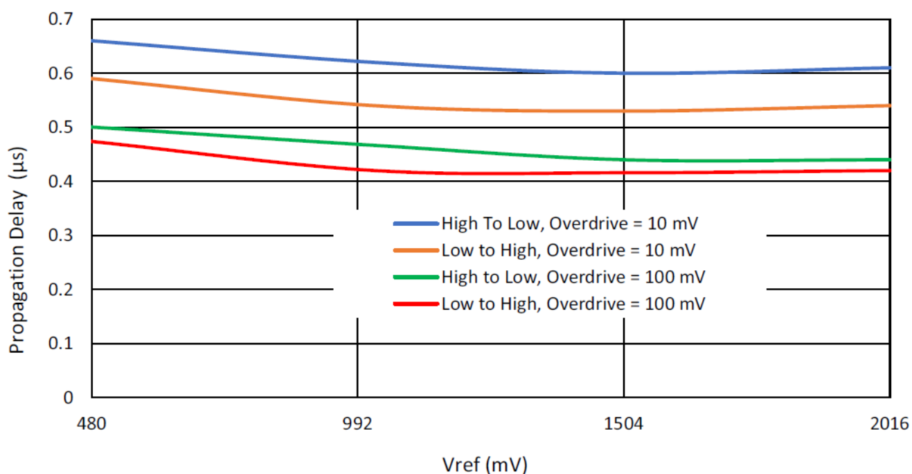
Figure 36. Typical Propagation Delay vs. V_{\text{REF}} for CCMP at T = +25\text{ }^{\circ}\text{C} , at V_{\text{DD}} = 2.3\text{ V} to 5.5\text{ V} , Gain = 4
