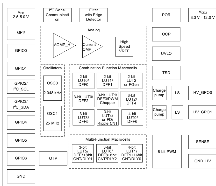
Figure 1. Block Diagram
