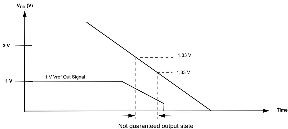
Figure 148. Power-Down
