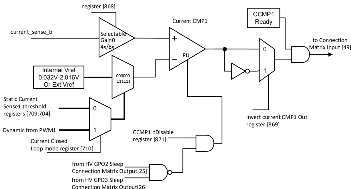
Figure 43. Current Sense Comparator1 Block Diagram
