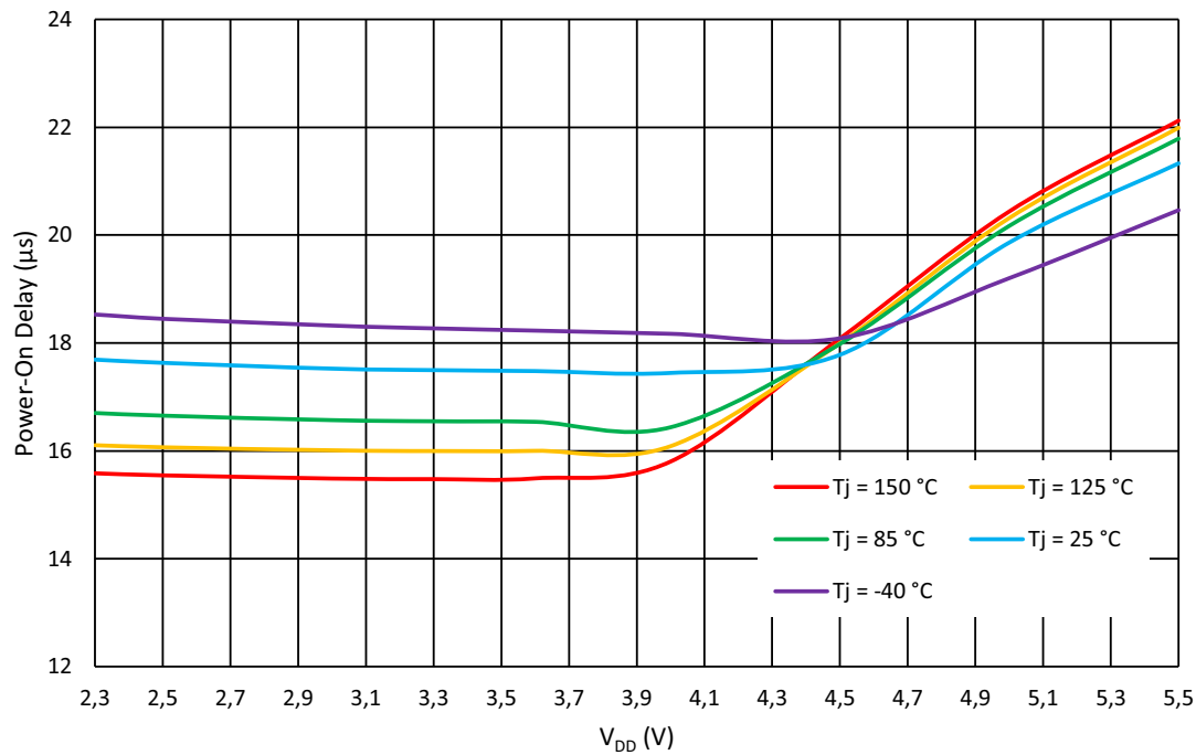
Figure 115. ACMPxH Power-On Delay vs. V DD
