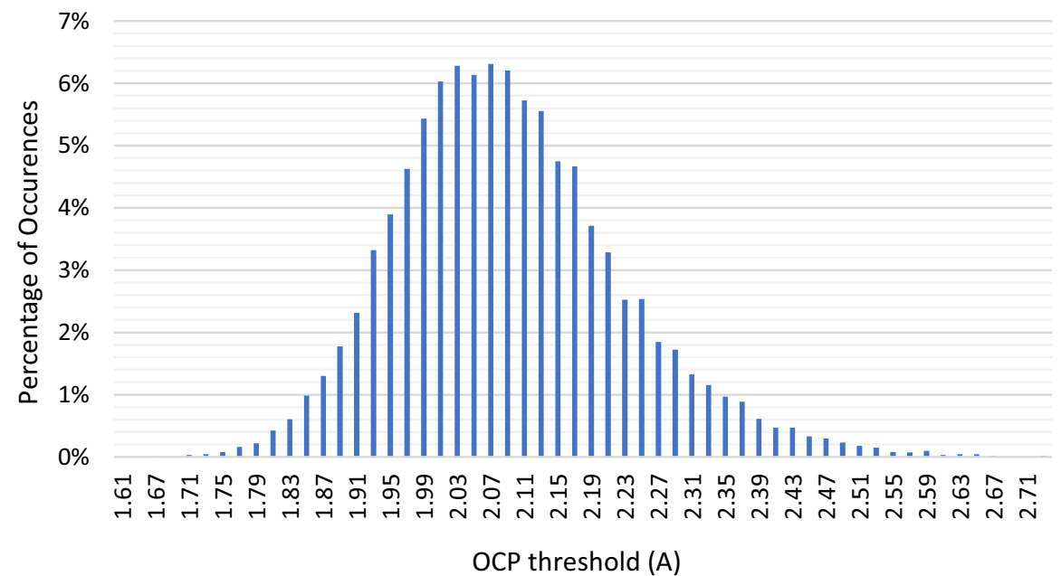
Figure 29. Full Bridge Low Side OCP Threshold Distribution at V_{DD} =2.3V to 5.5V, V_{DD2} = 3V to 13.2V, T_J = -40 °C to 150 °C
