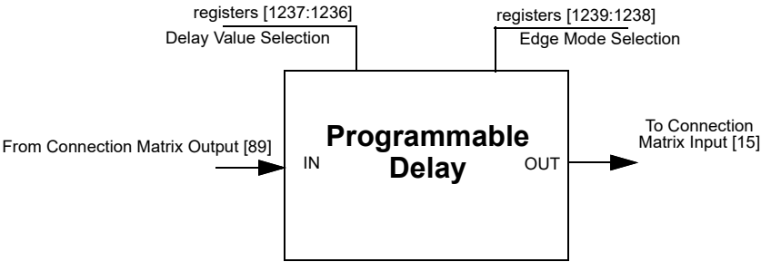
Figure 119. Programmable Delay
