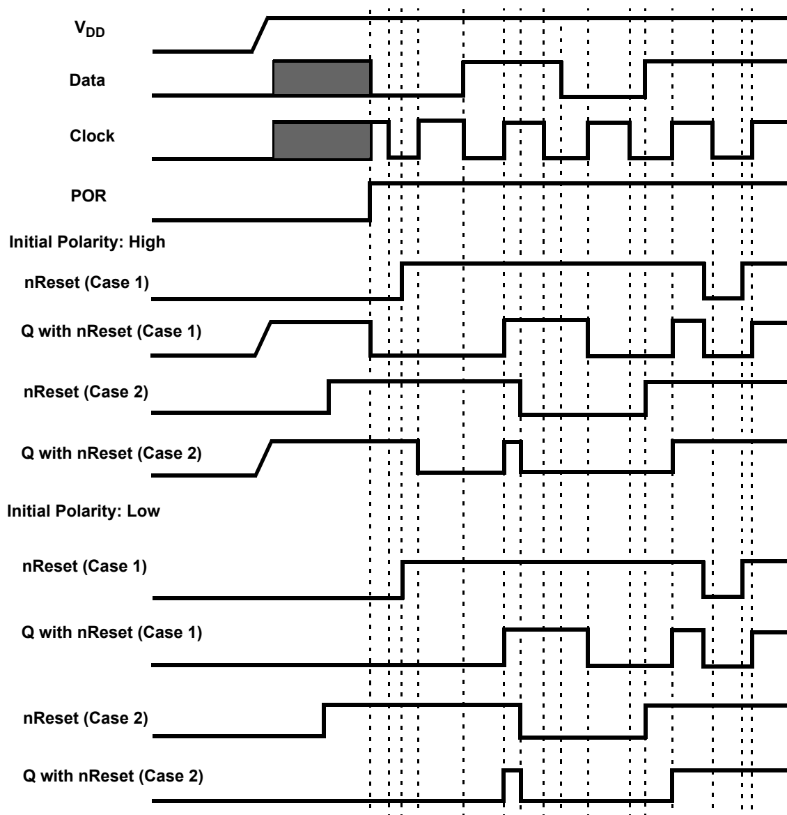
Figure 70. DFF Polarity Operations with n\text{Reset}
