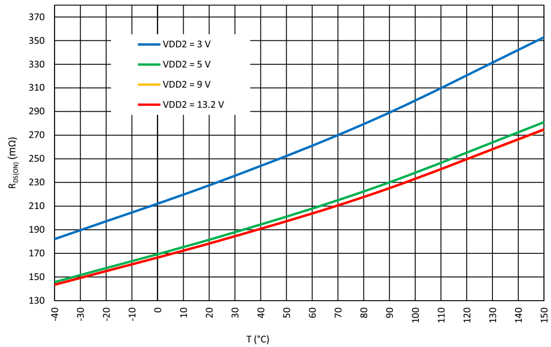
Figure 25. Full Bridge Typical Drain-Source Low Side On-Resistance vs. Temperature at I_{LOAD} = 0.5\text{ A} , V_{DD} = 5.5\text{ V}
