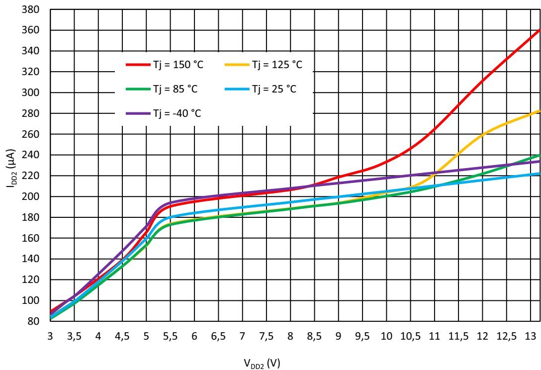
Figure 35. One Half Bridge I_{DD2} vs. V_{DD2} at V_{DD} = 5.5 V
