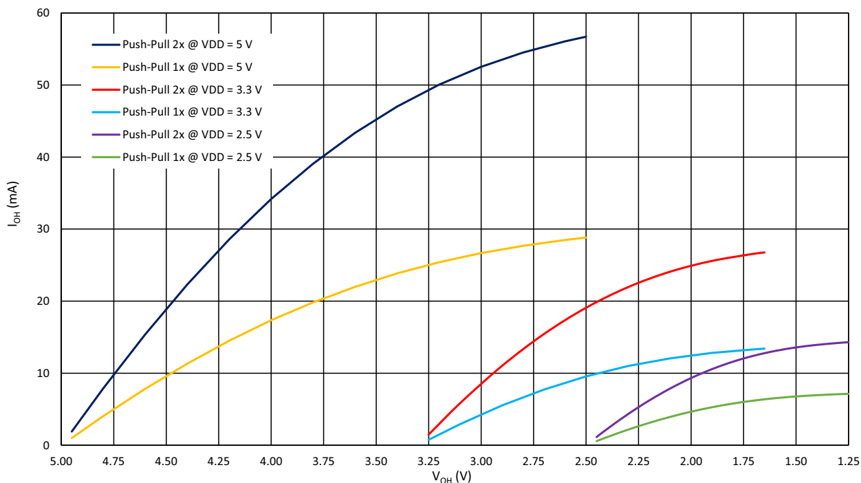
Figure 9. Typical High Level Output Current vs. High Level Output Voltage at T_A = 25^\circ\text{C}
