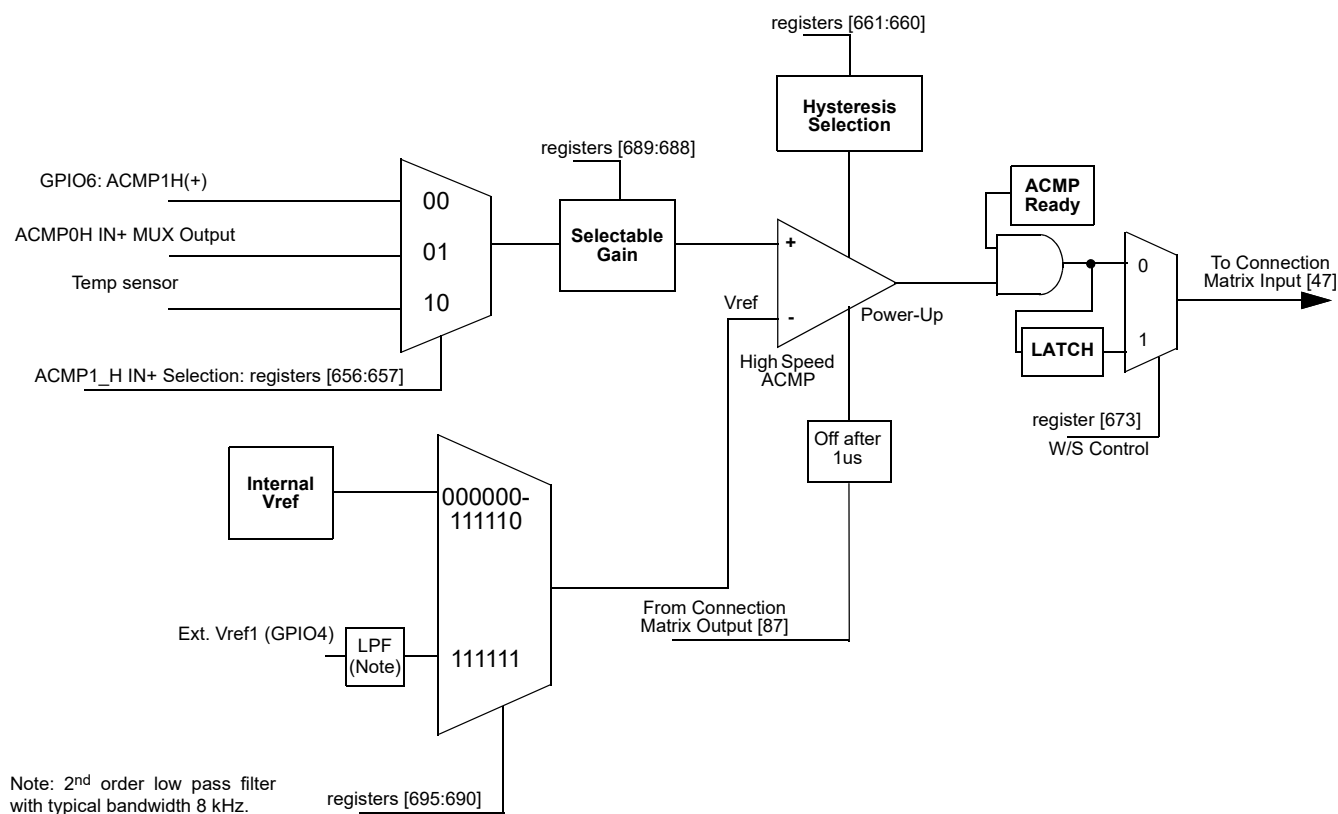
Figure 112. ACMP1H Block Diagram
