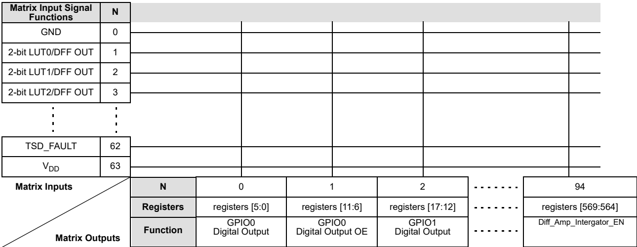
Figure 47. Connection Matrix
