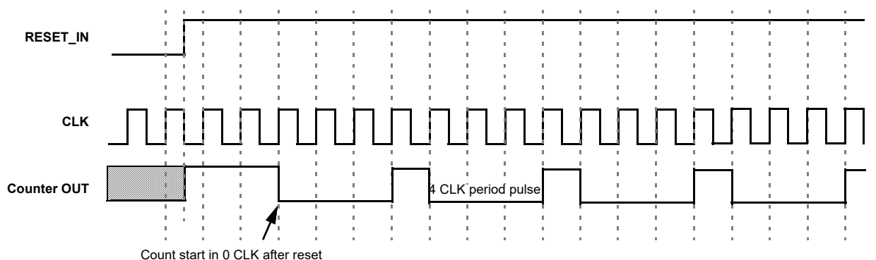
Figure 84. Counter Mode Timing Diagram with Two DFFs Synced Up
