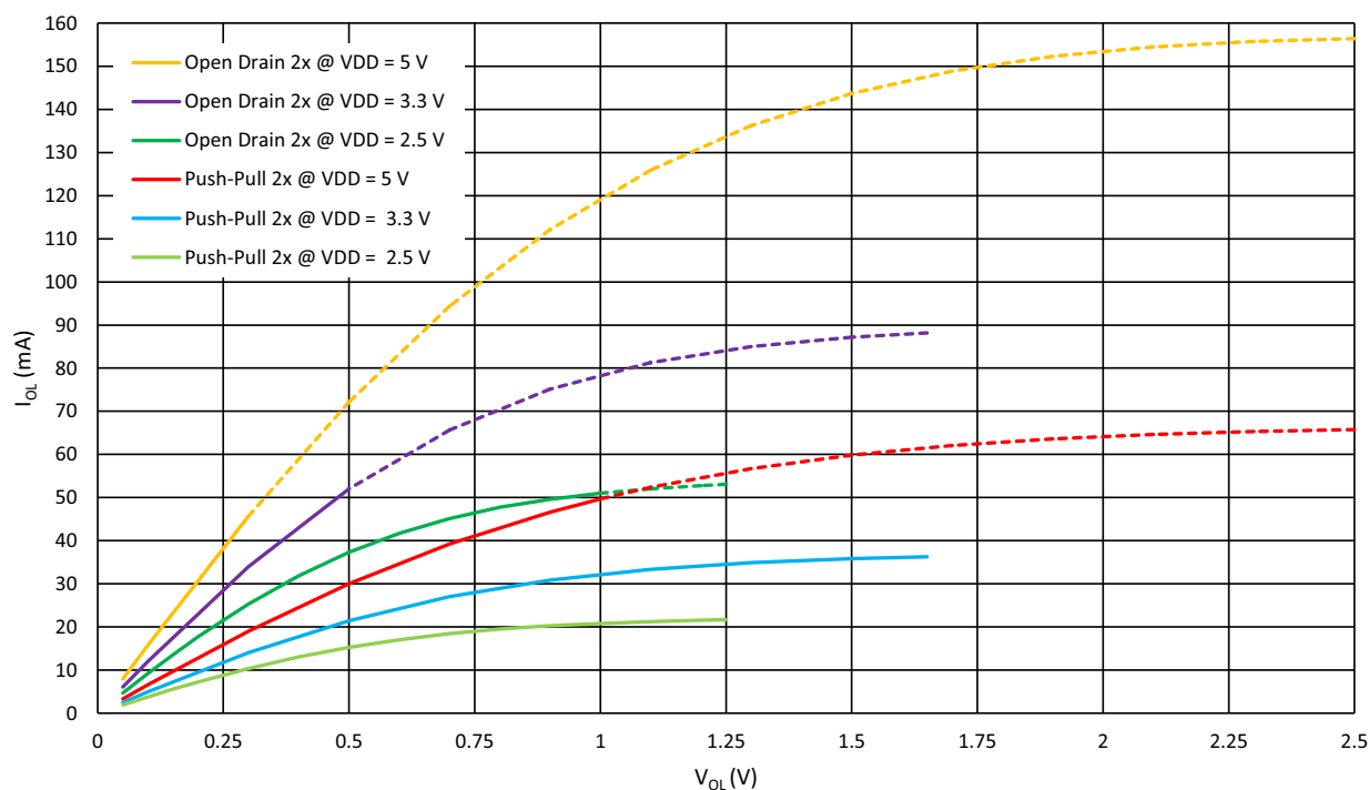
Figure 12. Typical Low Level Output Current vs. Low Level Output Voltage, 2x Drive at T_A = 25\text{ }^{\circ}\text{C} , Full Range
