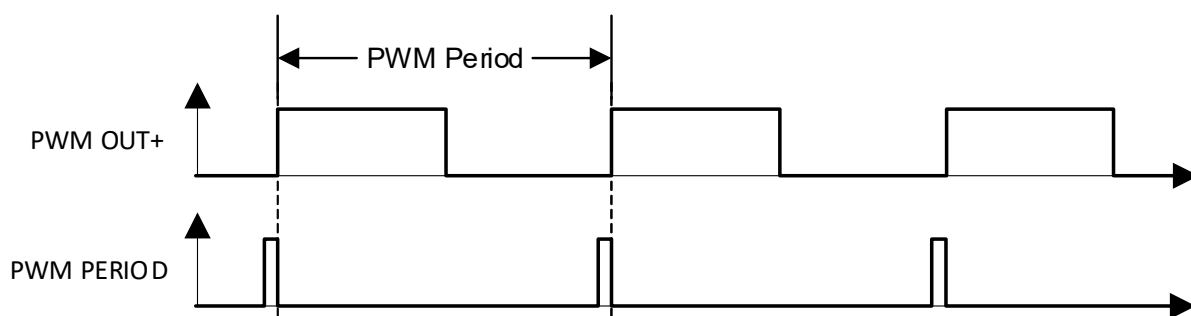
Figure 108. PWM Period Waveform
