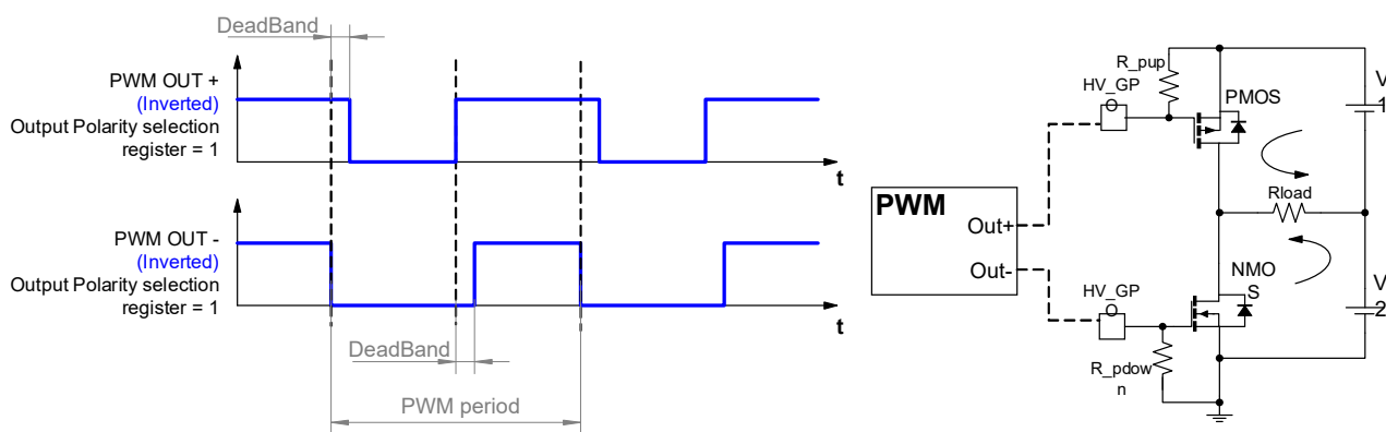
Figure 100. PWM Output Waveforms and Test Circuit Example for Driving NMOS and PMOS FETs
