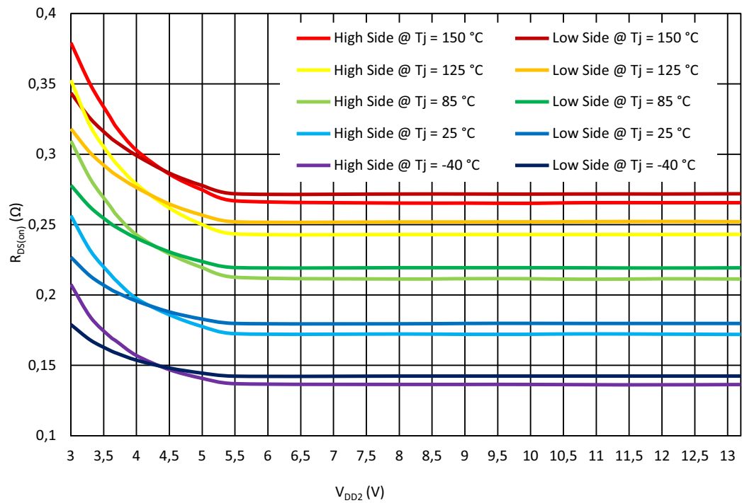
Figure 26. Full Bridge Typical Drain-Source On-Resistance vs. V_{DD2} at V_{DD} = 5.5\text{ V} , I_{LOAD} = 0.1\text{ A}
