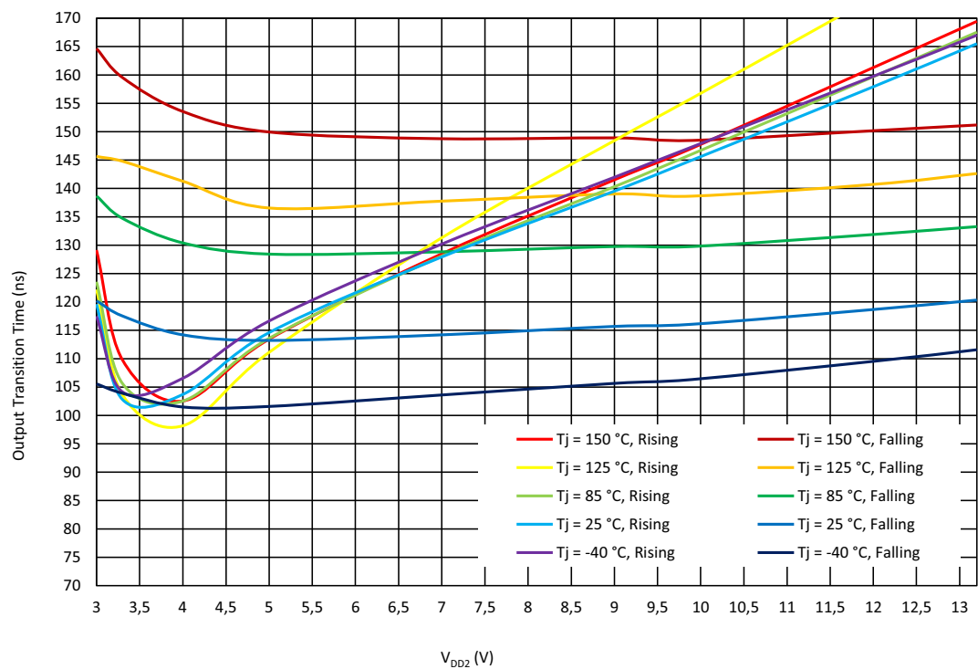
Figure 34. Half Bridge Output Transition Time vs. V_{DD2} at V_{DD} = 2.3 V to 5.5 V, f = 50 kHz for Regular Mode
