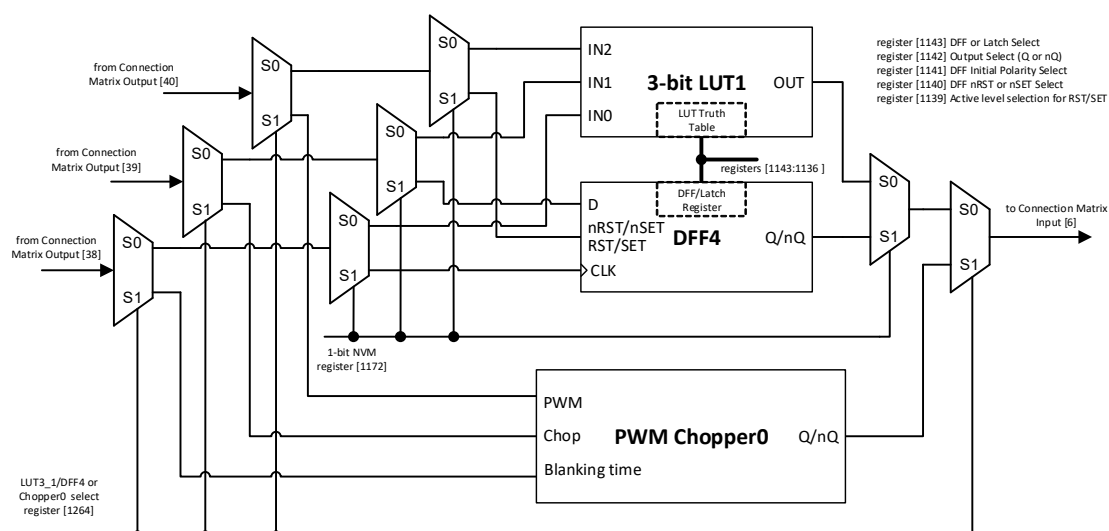
Figure 61. 3-bit LUT1 or DFF4
