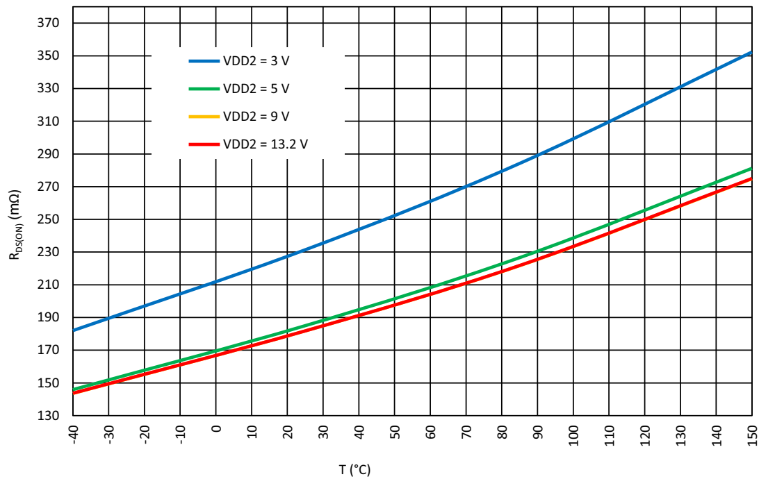
Figure 24. Full Bridge Typical Drain-Source Low Side On-Resistance vs. Temperature at I_{LOAD} = 0.5\text{ A} , V_{DD} = 2.3\text{ V}
