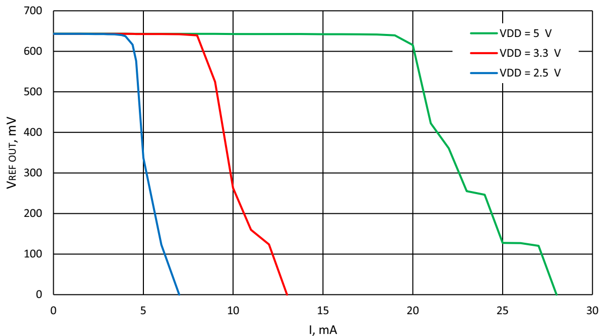
Figure 124. Typical Load Regulation, Vref = 640 mV, T_A = -40\text{ }^{\circ}\text{C} to +105\text{ }^{\circ}\text{C} , Buffer - Enabled
