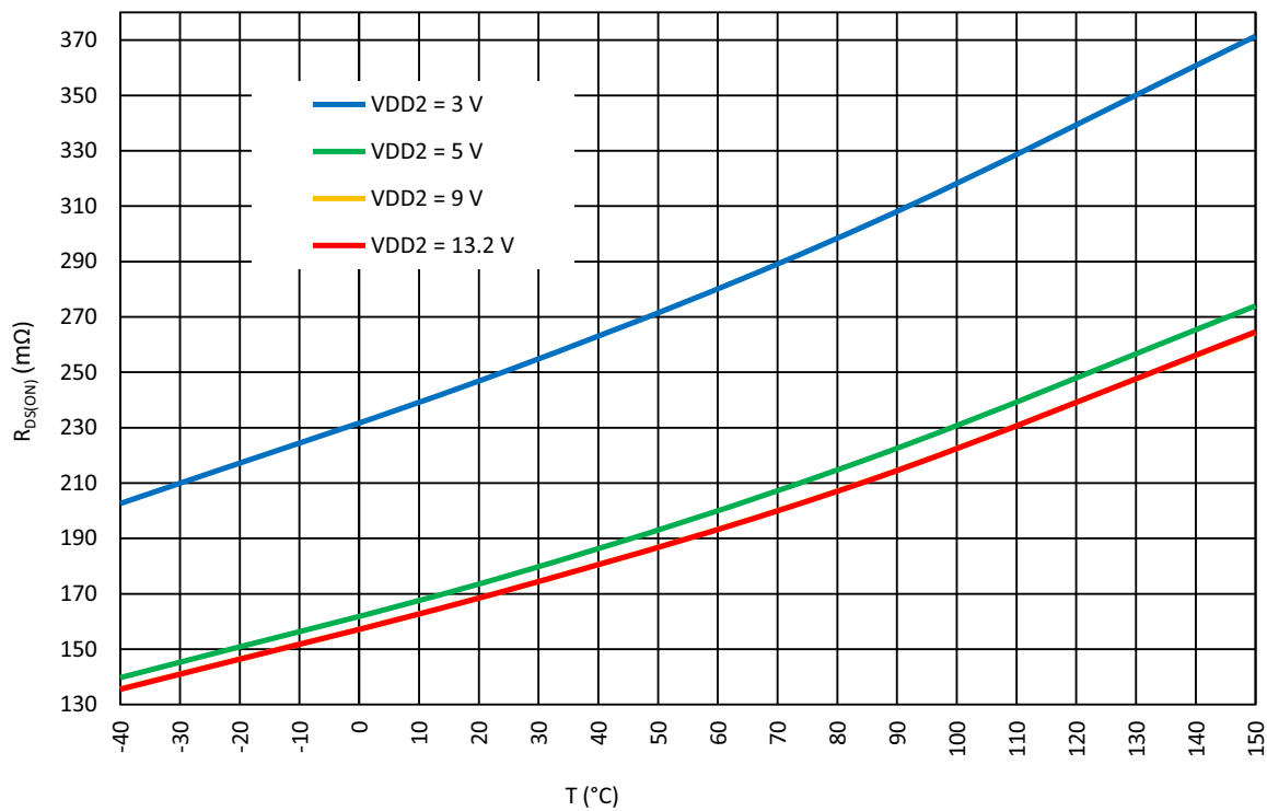
Figure 23. Full Bridge Typical Drain-Source High Side On-Resistance vs. Temperature at I_{LOAD} = 0.5\text{ A} , V_{DD} = 5.5\text{ V}
