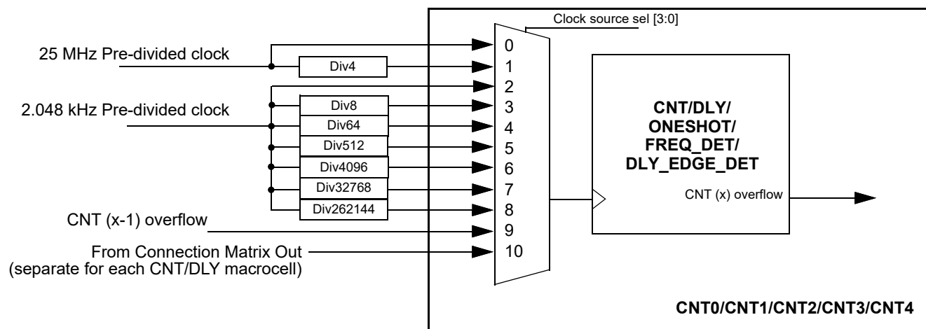
Figure 129. Clock Scheme
