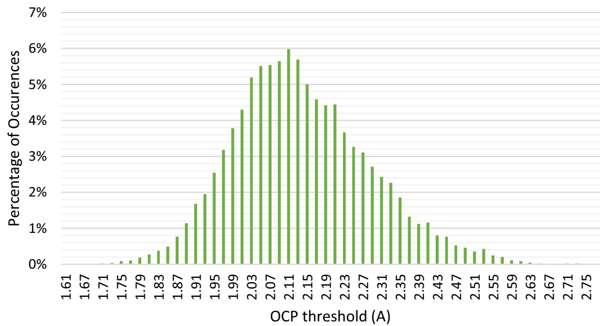
Figure 28. Full Bridge High Side OCP Threshold Distribution at V_{DD} =2.3V to 5.5V, V_{DD2} =3V to 13.2V, T_J =-40 °C to 150 °C
