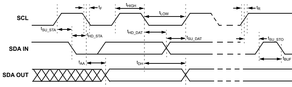
Figure 150. I 2 C General Timing Characteristics
