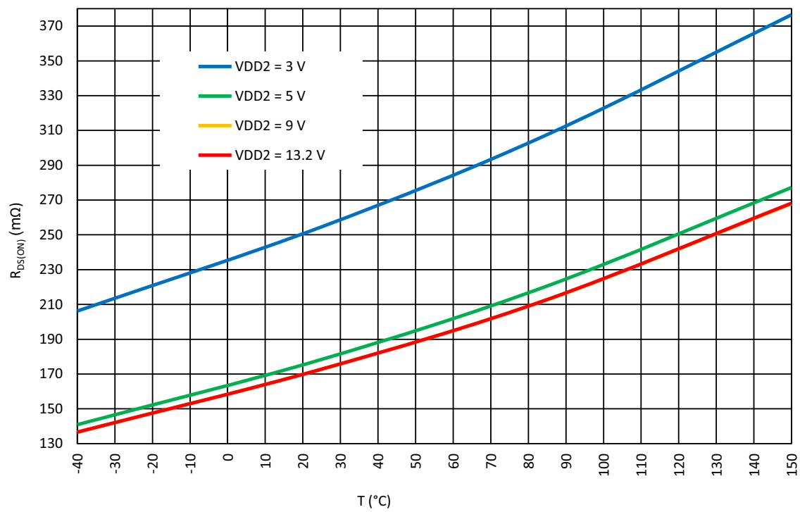
Figure 22. Full Bridge Typical Drain-Source High Side On-Resistance vs. Temperature at I_{LOAD} = 0.5\text{ A} , V_{DD} = 2.3\text{ V}
