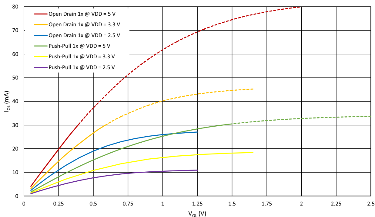
Figure 10. Typical Low Level Output Current vs. Low Level Output Voltage, 1x Drive at T_A = 25^\circ\text{C} , Full Range
