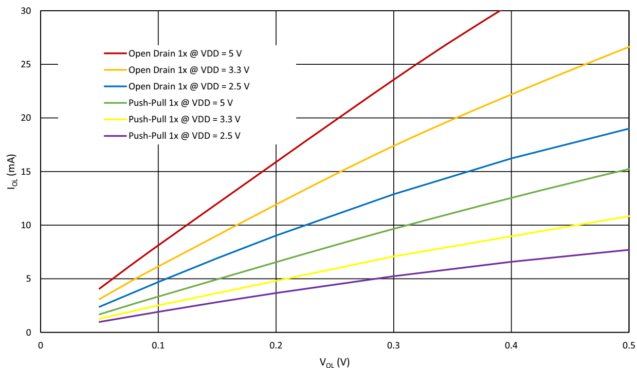
Figure 11. Typical Low Level Output Current vs. Low Level Output Voltage, 1x Drive at T_A = 25\text{ }^{\circ}\text{C}
