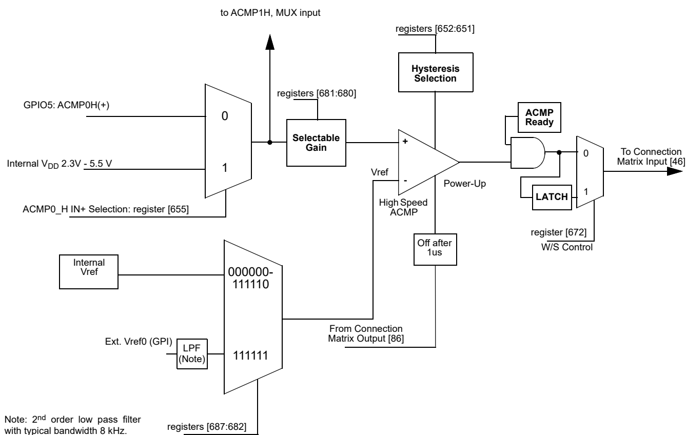
Figure 111. ACMP0H Block Diagram
