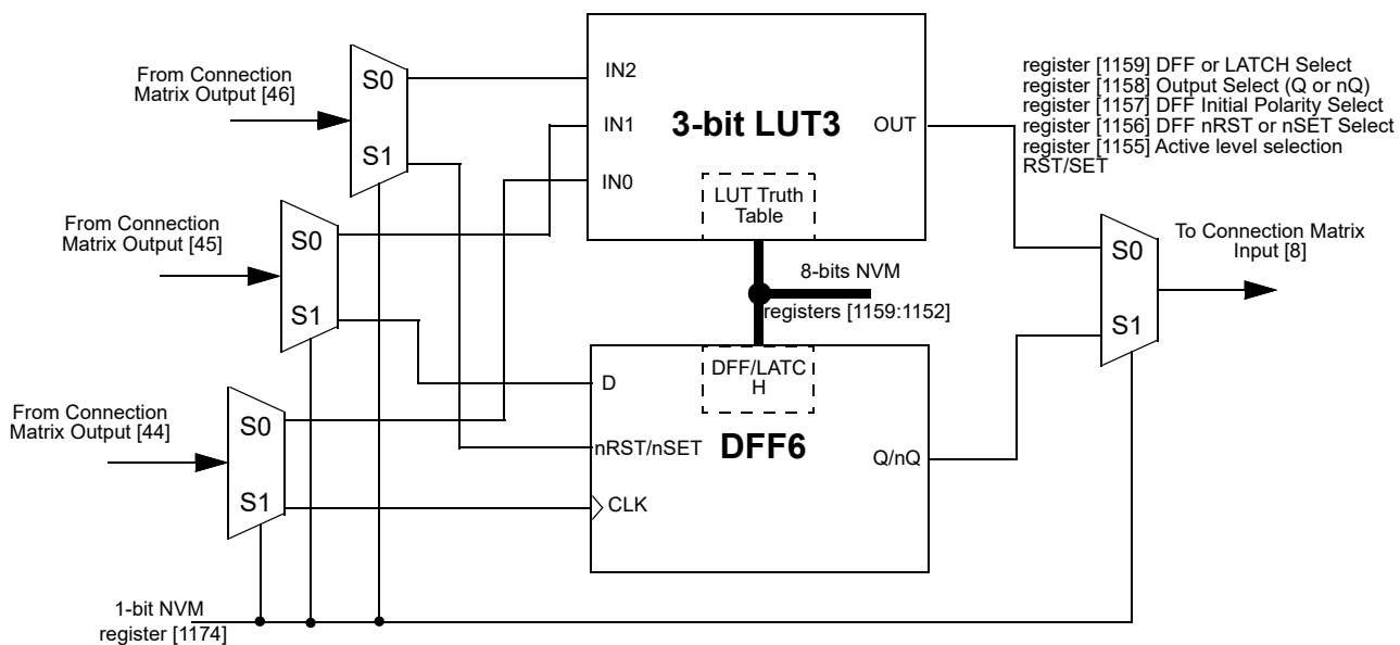
Figure 56. 3-bit LUT3 or DFF6
