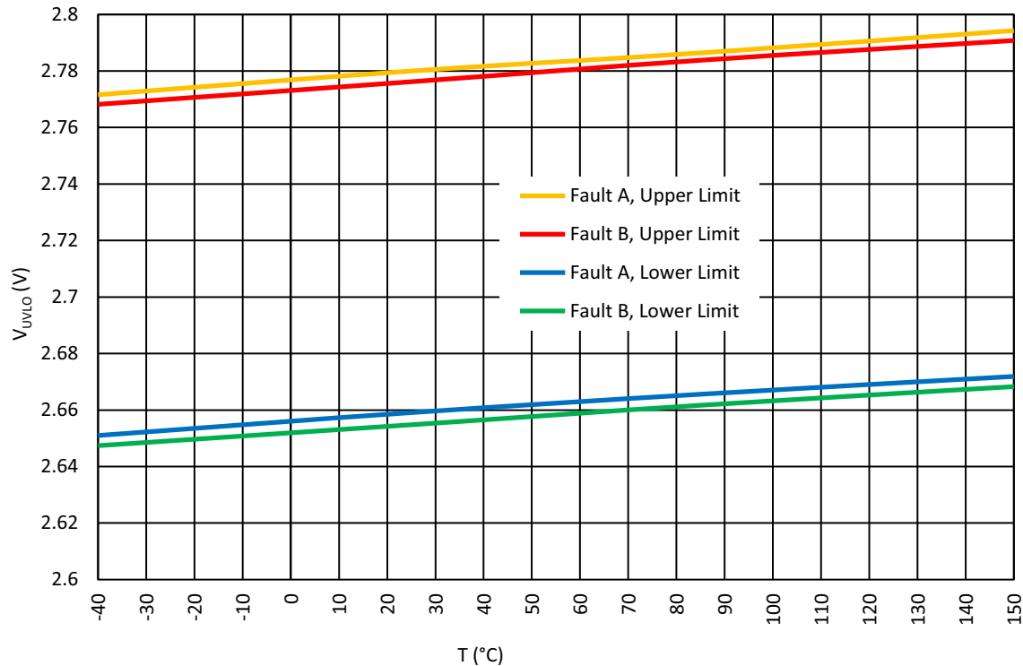
Figure 27. Half Bridge Under-voltage Lockout Value vs. Temperature at V_{DD} = 3.3\text{ V}
