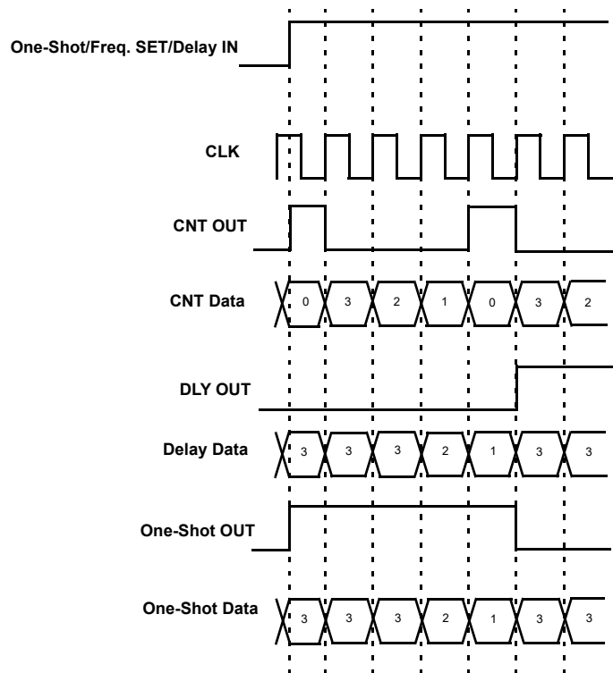
Figure 93. Counter Value, Counter Data = 3
