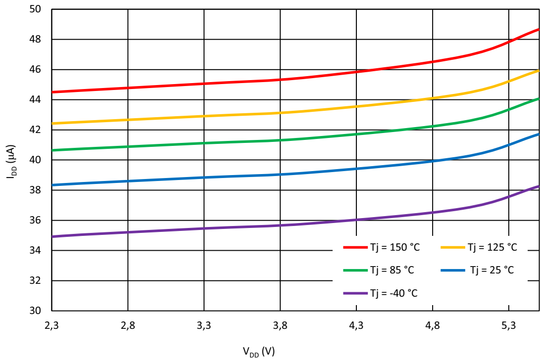
Figure 117. ACMPxH Current Consumption vs. V_{DD} at V_{ref} = 1024\text{ mV}
