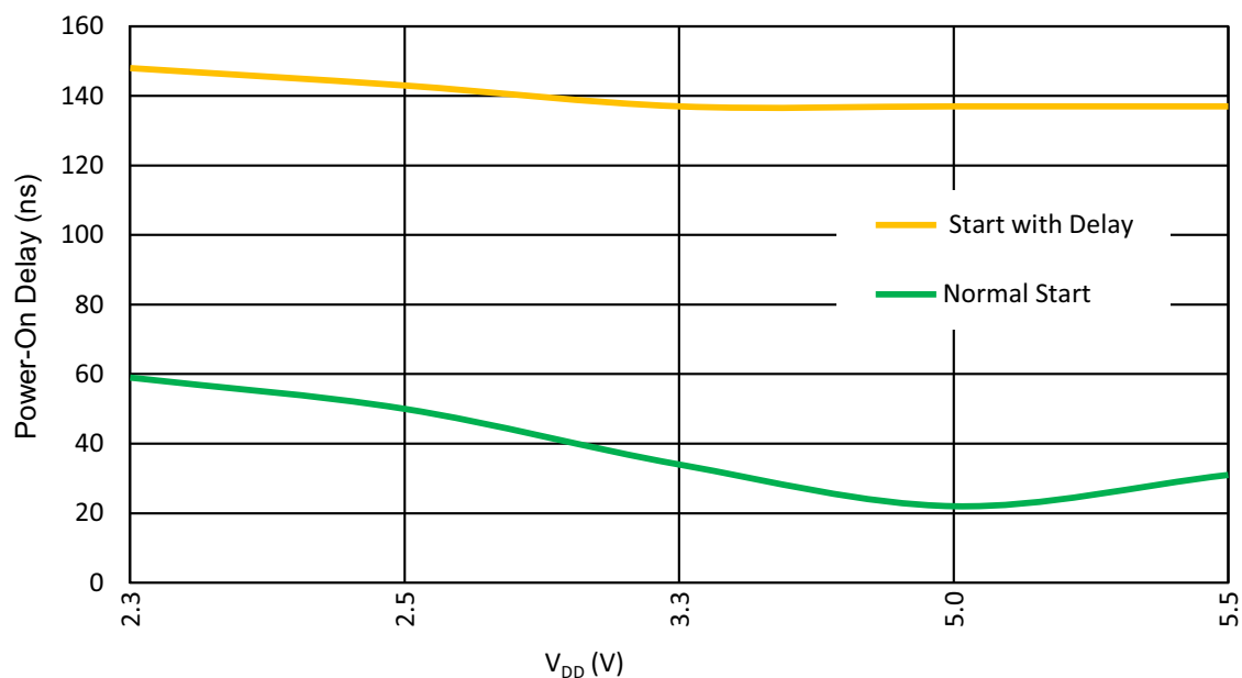
Figure 133. Oscillator1 Maximum Power-On Delay vs. V_{DD} at T_A = 25\text{ }^{\circ}\text{C} , OSC1 = 25 MHz
