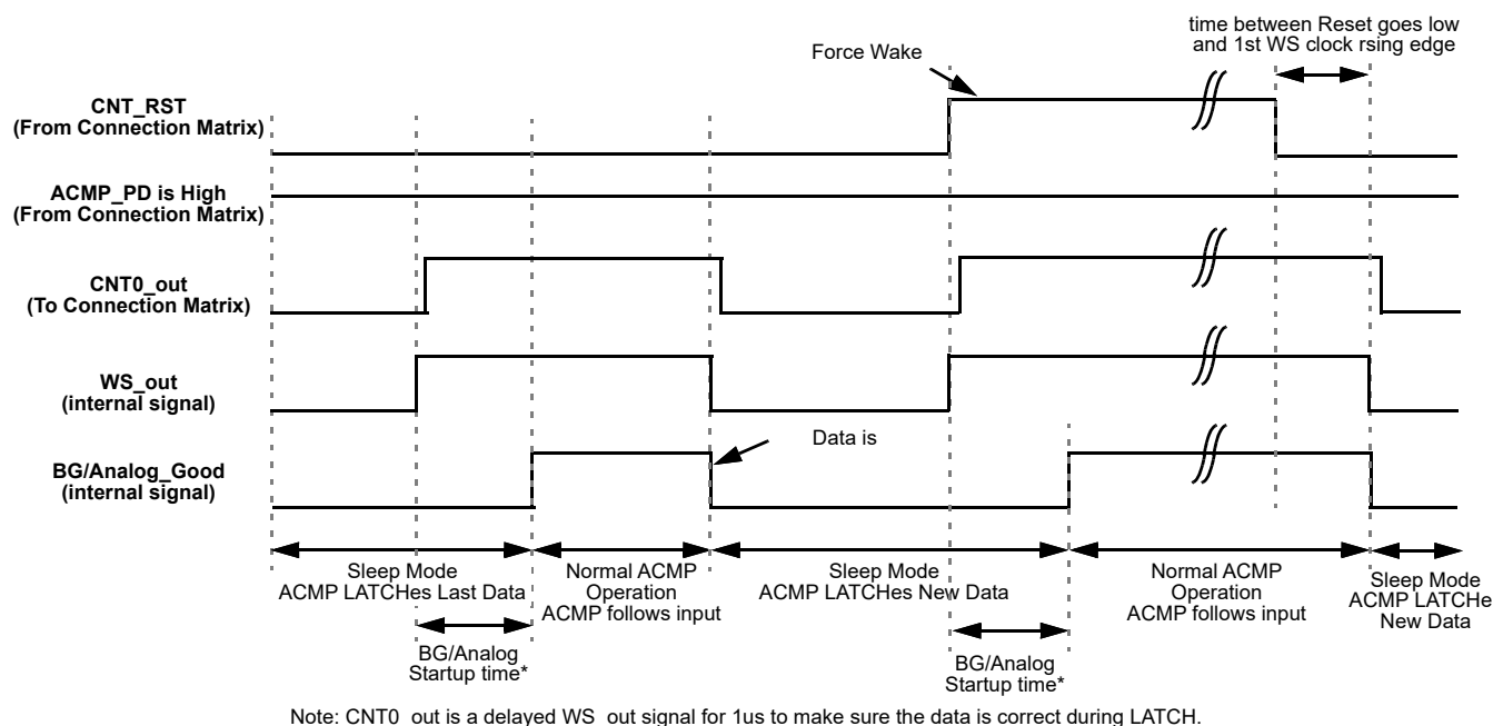
Figure 95. Wake/Sleep Timing Diagram, Normal Wake Mode, Counter Reset is Used
