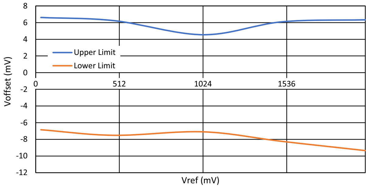
Figure 113. ACMPxH Input Offset Voltage vs. Vref at V_{DD} = 2.3\text{ V to }5.5\text{ V} , T_A = -40\text{ }^{\circ}\text{C to }105\text{ }^{\circ}\text{C}
