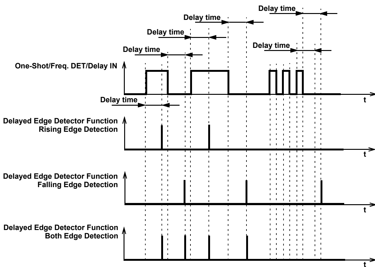
Figure 88. Delayed Edge Detection Mode Timing Diagram
