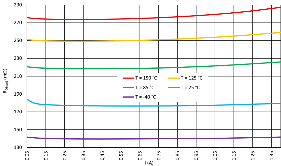
Figure 20. Full Bridge Typical Drain-Source High Side On-Resistance vs. Load Current at V_{DD} = 5.5\text{ V} , V_{DD2} = 5\text{ V}
