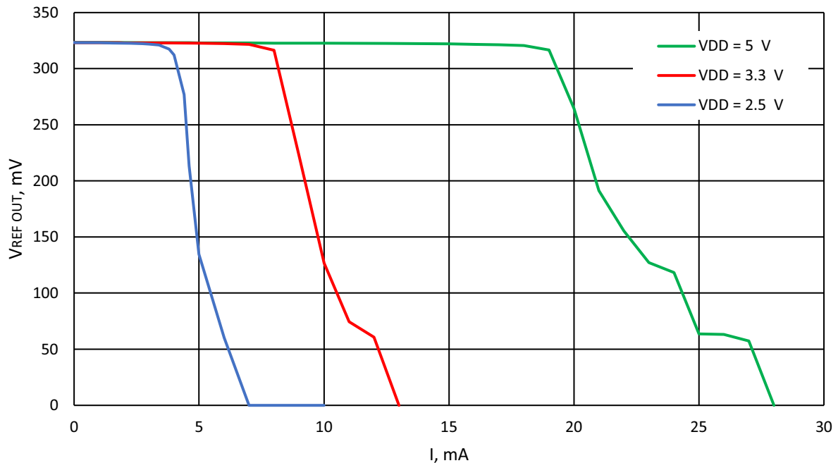
Figure 123. Typical Load Regulation, Vref = 320 mV, T_A = -40\text{ }^{\circ}\text{C} to +105\text{ }^{\circ}\text{C} , Buffer - Enabled
