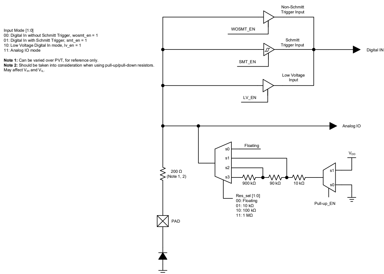
Figure 4. GPI Structure Diagram
