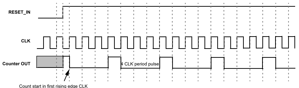
Figure 83. Counter Mode Timing Diagram without Two DFFs Synced Up
