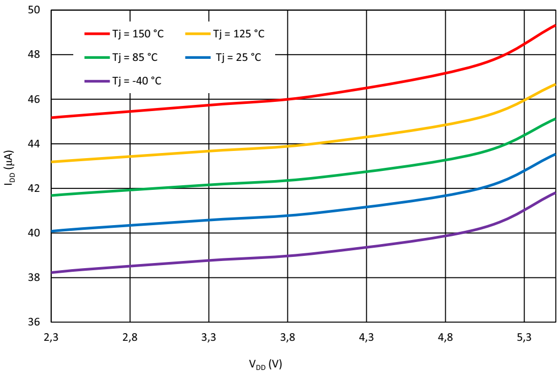
Figure 118. ACMPxH Current Consumption vs. V_{DD} at V_{ref} = 2016\text{ mV}
