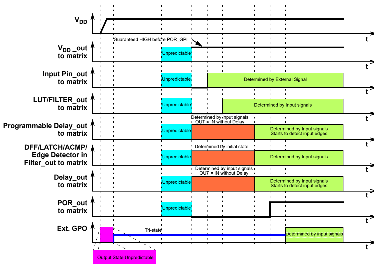
Figure 147. Internal Macrocell States During POR Sequence
