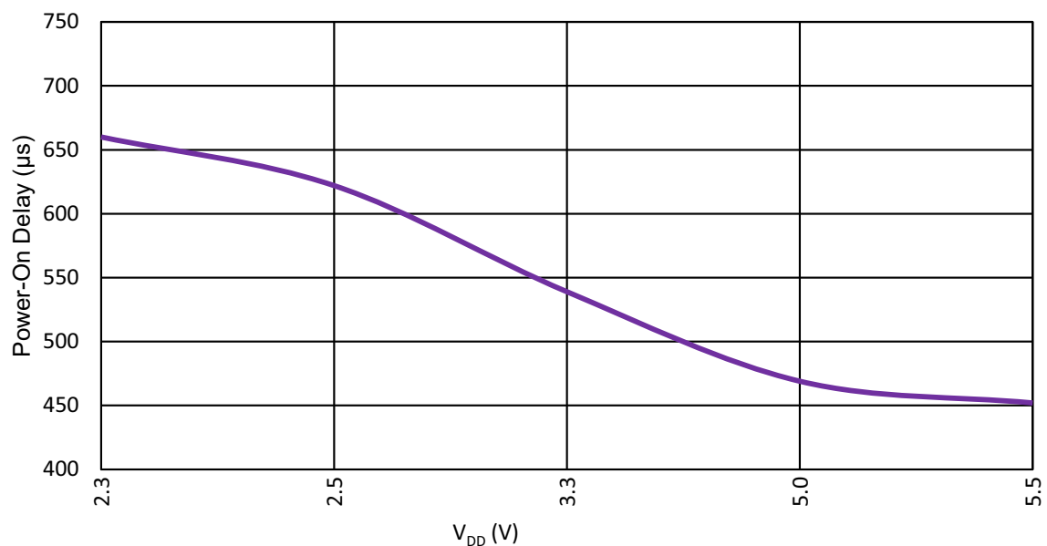
Figure 132. Oscillator0 Maximum Power-On Delay vs. V_{DD} at T_A = 25\text{ }^{\circ}\text{C} , OSC0 = 2.048 kHz
