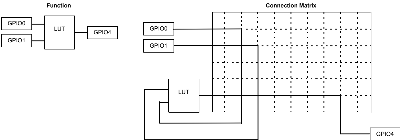
Figure 48. Connection Matrix Example
