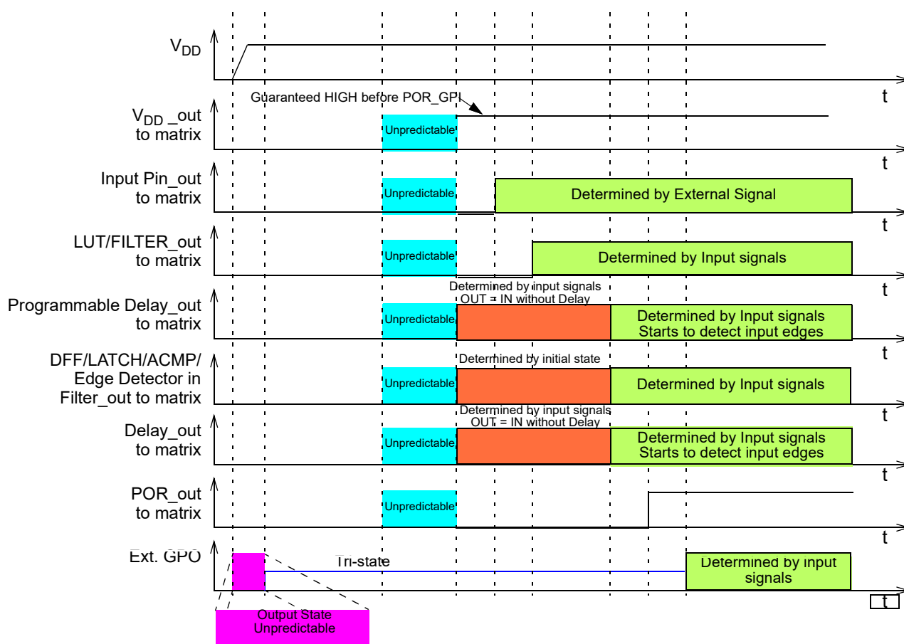
Figure 152. Internal Macrocell States during POR Sequence
