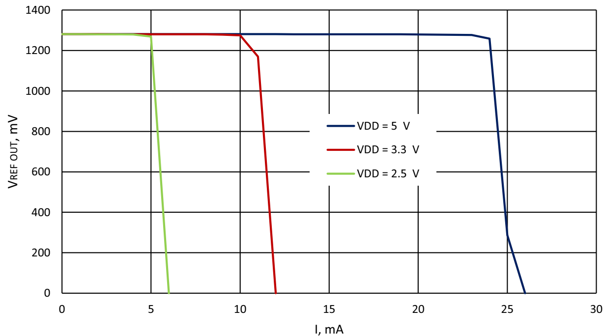
Figure 130. Typical Load Regulation, V_{ref} = 1280\text{ mV} , T_A = -40\text{ }^{\circ}\text{C} to +85\text{ }^{\circ}\text{C} , Buffer - Enabled
