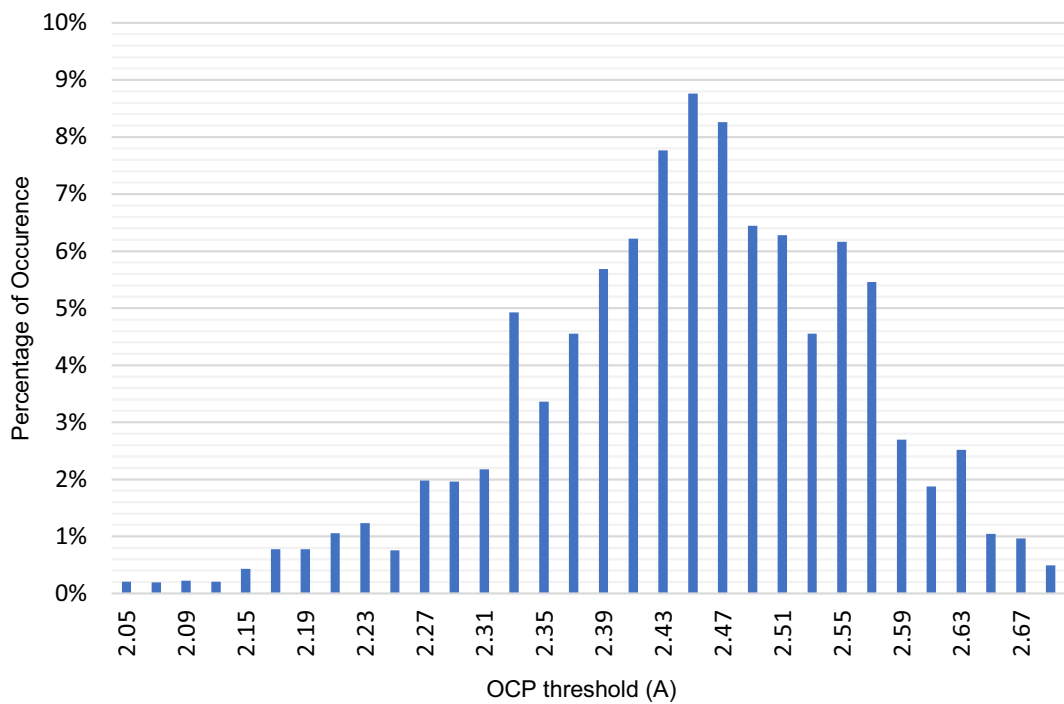
Figure 24. Full Bridge High-side OCP Threshold Distribution at V_{DD}=2.3\text{ V} to 5.5\text{ V} , V_{DD2}=3\text{ V} to 26.4\text{ V} , T_J=-40\text{ }^{\circ}\text{C} to 150\text{ }^{\circ}\text{C}
