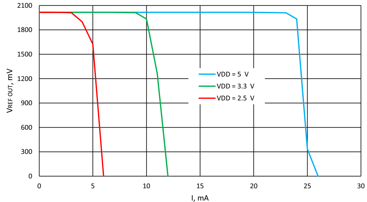
Figure 131. Typical Load Regulation, V_{ref} = 2016\text{ mV} , T_A = -40\text{ }^{\circ}\text{C} to +85\text{ }^{\circ}\text{C} , Buffer - Enabled
