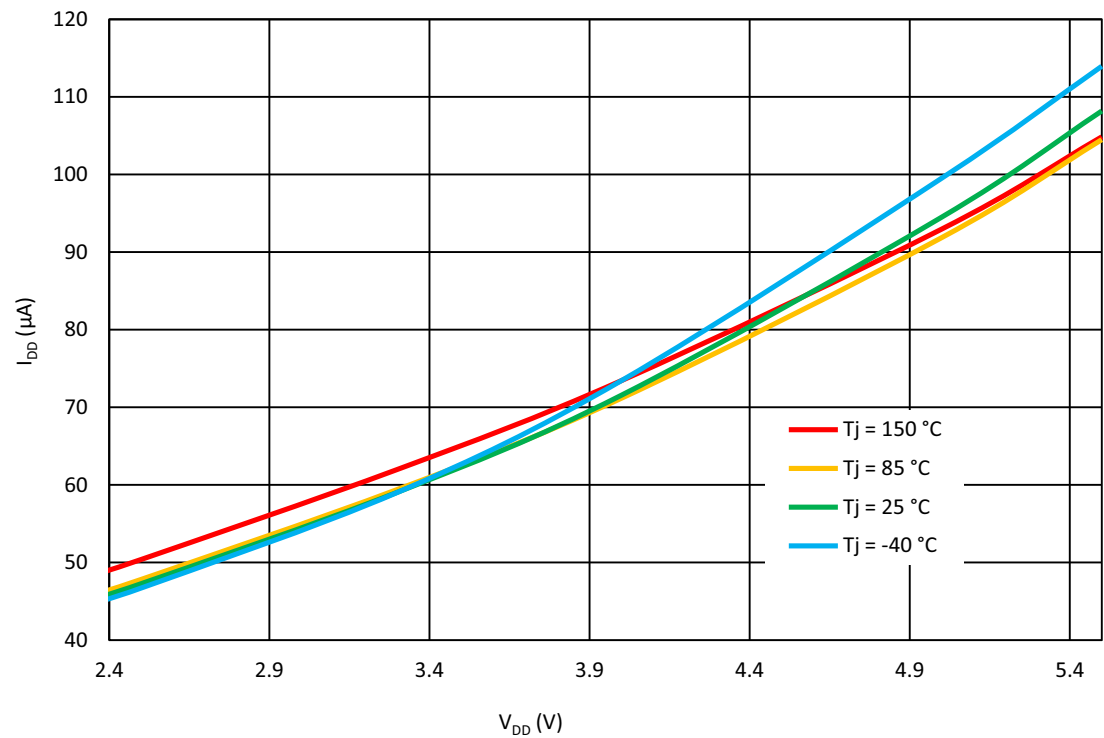
Figure 147. OSC1 Current Consumption vs. V_{DD} (Pre-Divider = 2)
