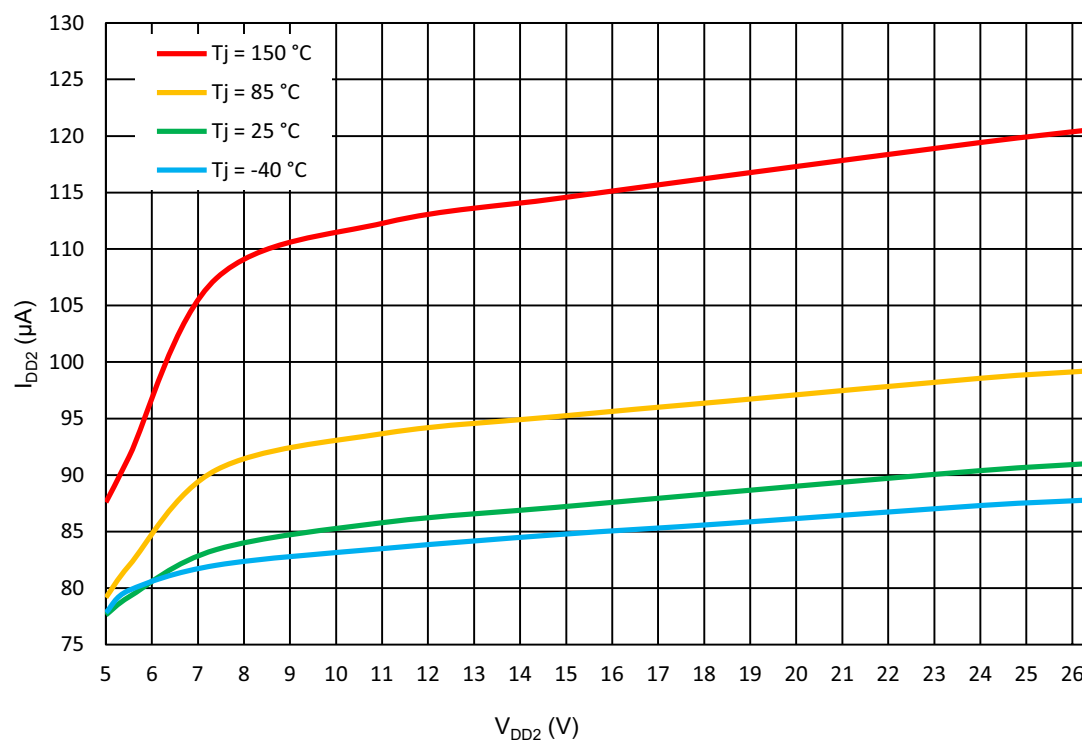
Figure 35. One Half Bridge + CCMP I DD2 vs. V DD2 at V DD = 5.5 V
