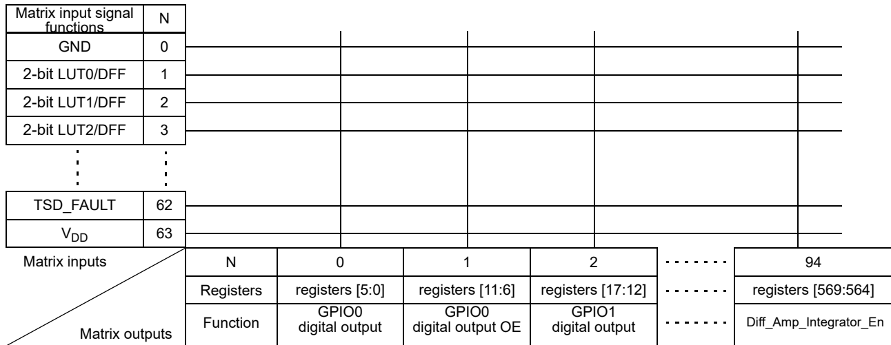
Figure 52. Connection Matrix
