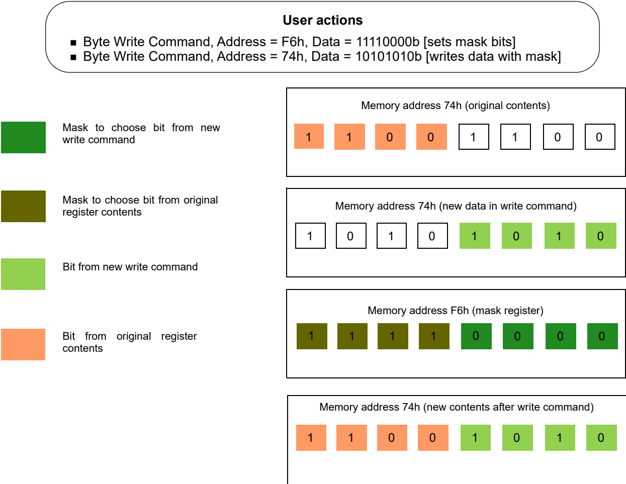
Figure 162. Example of I 2 C Byte Write Bit Masking
