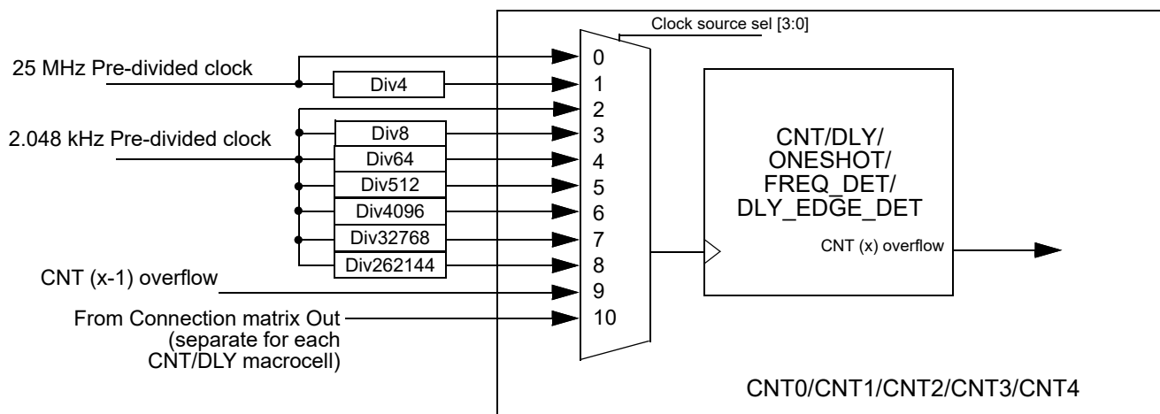
Figure 134. Clock Scheme
