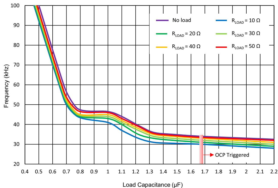
Figure 39. Two Half Bridges in Parallel Safe Operating Area. Frequency vs. C_{\text{LOAD}} at T_A = 25\ ^\circ\text{C} , V_{\text{DD2}} = 24\ \text{V}
