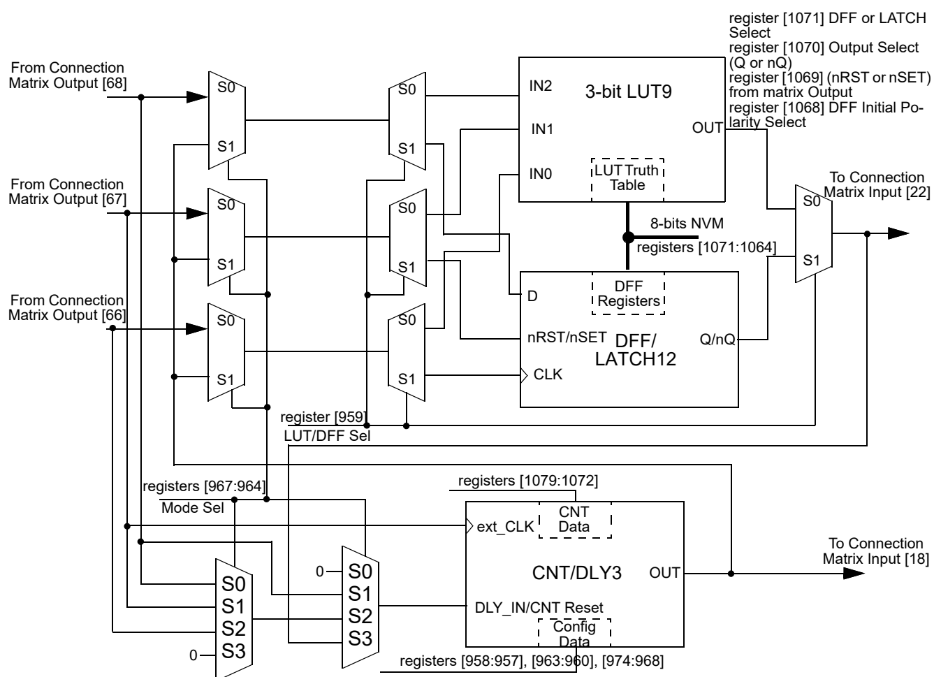
Figure 83. 8-bit Multi-Function Macrocells Block Diagram (3-bit LUT9/DFF12, CNT/DLY3)
