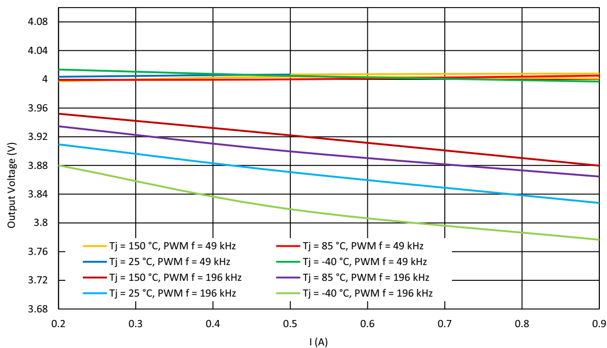
Figure 47. Typical Load Regulation at V_{OUT} = 4.096 V, V_{DD} = 2.3 V to 5.5 V, V_{DD2} = 9 V
