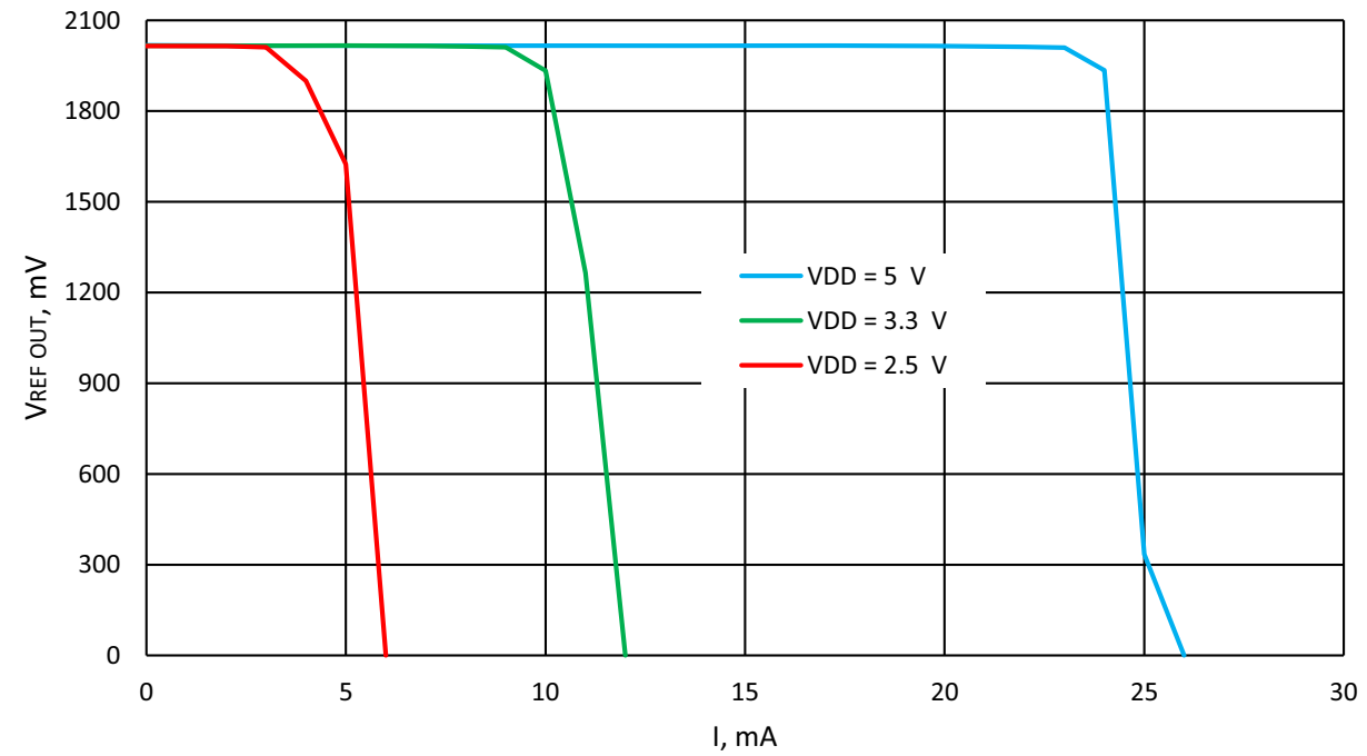
Figure 131. Typical Load Regulation, V_{ref} = 2016\text{ mV} , T_A = -40\text{ }^{\circ}\text{C} to +105\text{ }^{\circ}\text{C} , Buffer - Enabled
