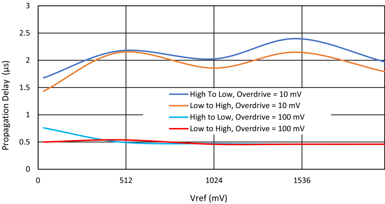
Figure 119. Propagation Delay vs. V_{\text{ref}} for ACMPxH at T_A = 25^\circ\text{C} , at V_{\text{DD}} = 2.3\text{ V to }5.5\text{ V} , Gain = 1, Hysteresis = 0
