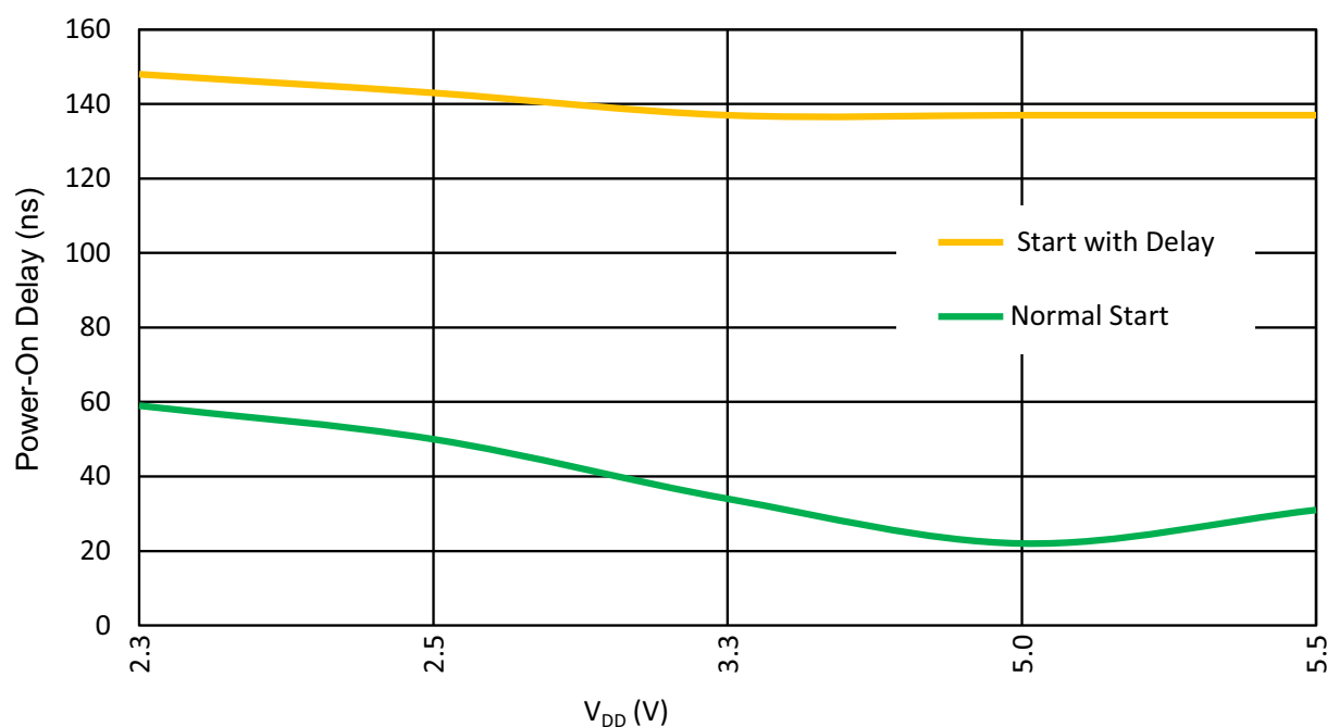
Figure 138. Oscillator1 Maximum Power-On Delay vs. V_{DD} at T_A = 25\text{ }^{\circ}\text{C} , OSC1 = 25 MHz
