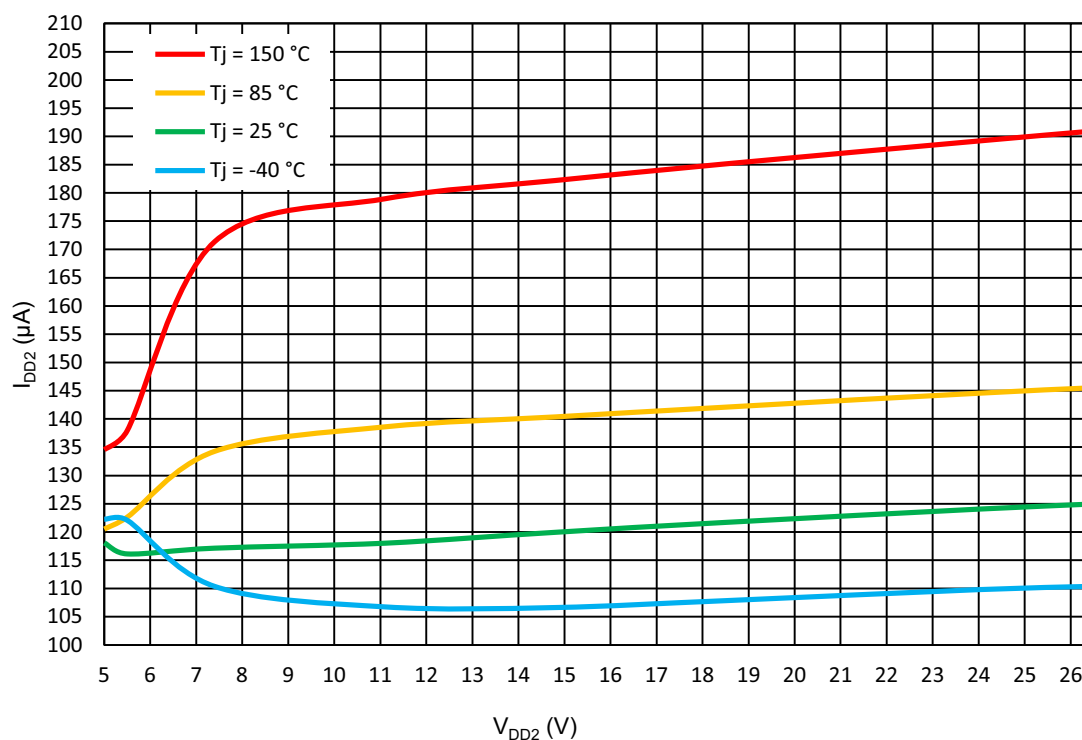
Figure 36. Full Bridge + CCMP I DD2 vs. V DD2 at V DD = 5.5 V
