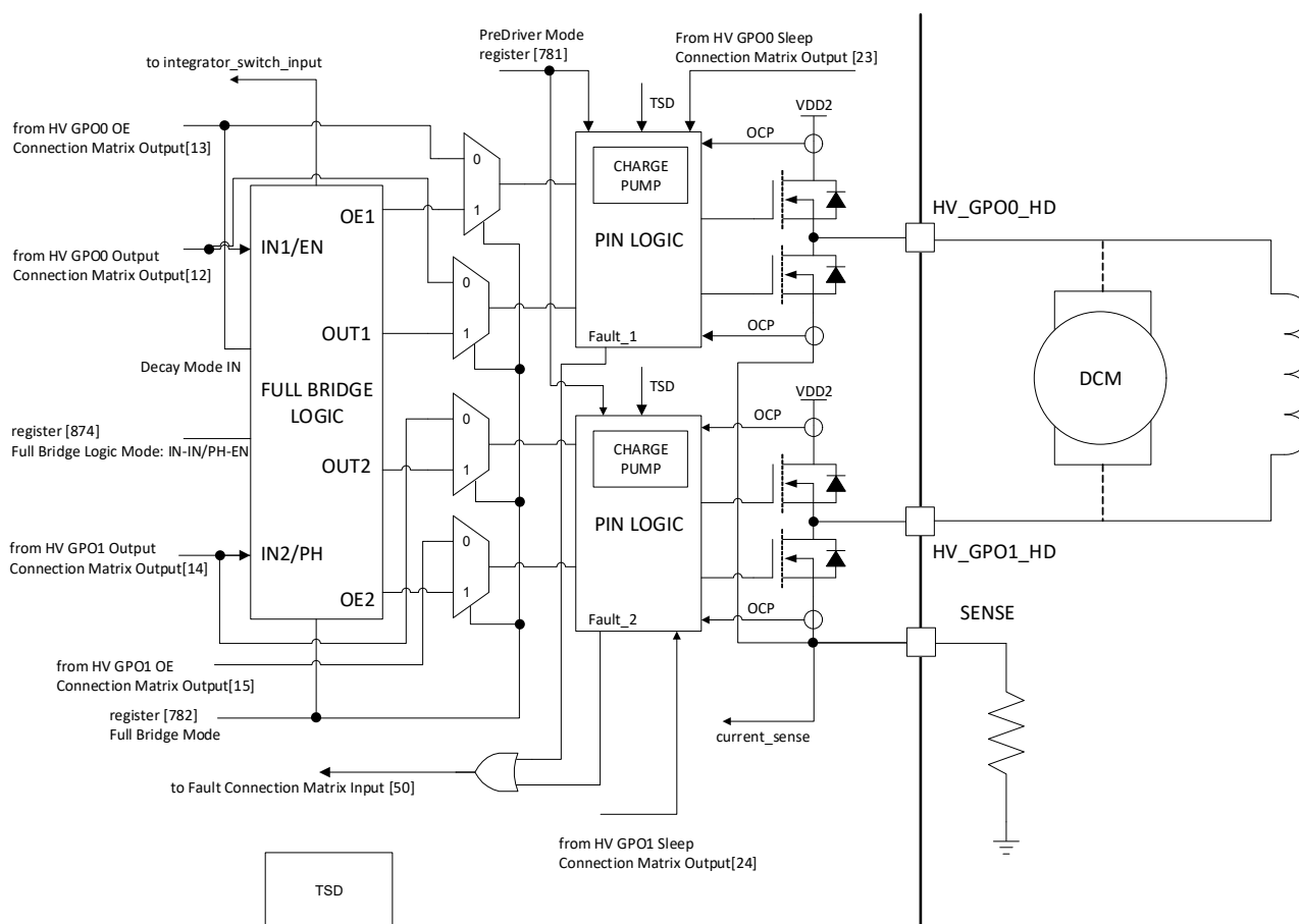
Figure 13. HV OUT Block Diagram
