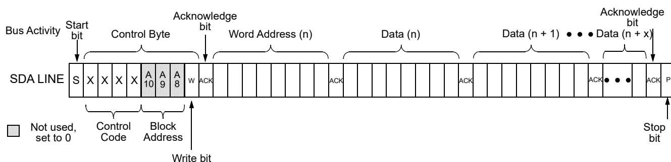
Figure 157. Sequential Write Command
