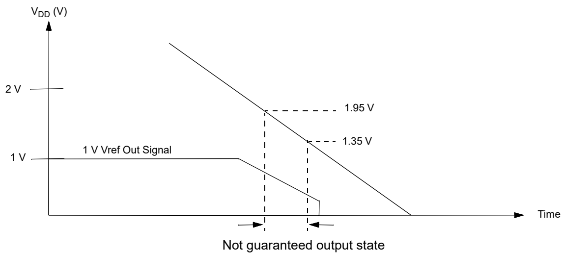
Figure 153. Power-Down
