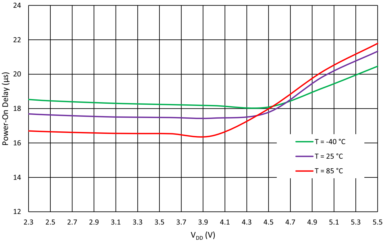
Figure 120. ACMPxH Power-On Delay vs. V_{\text{DD}}
