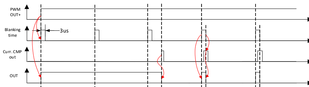
Figure 74. PWM Chopper. Overcurrent when 100 % Duty Cycle
