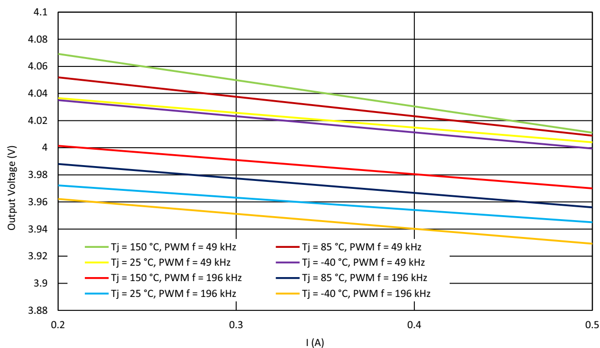
Figure 46. Typical Load Regulation at V_{OUT} = 4.096 V, V_{DD} = 2.3 V to 5.5 V, V_{DD2} = 5 V
