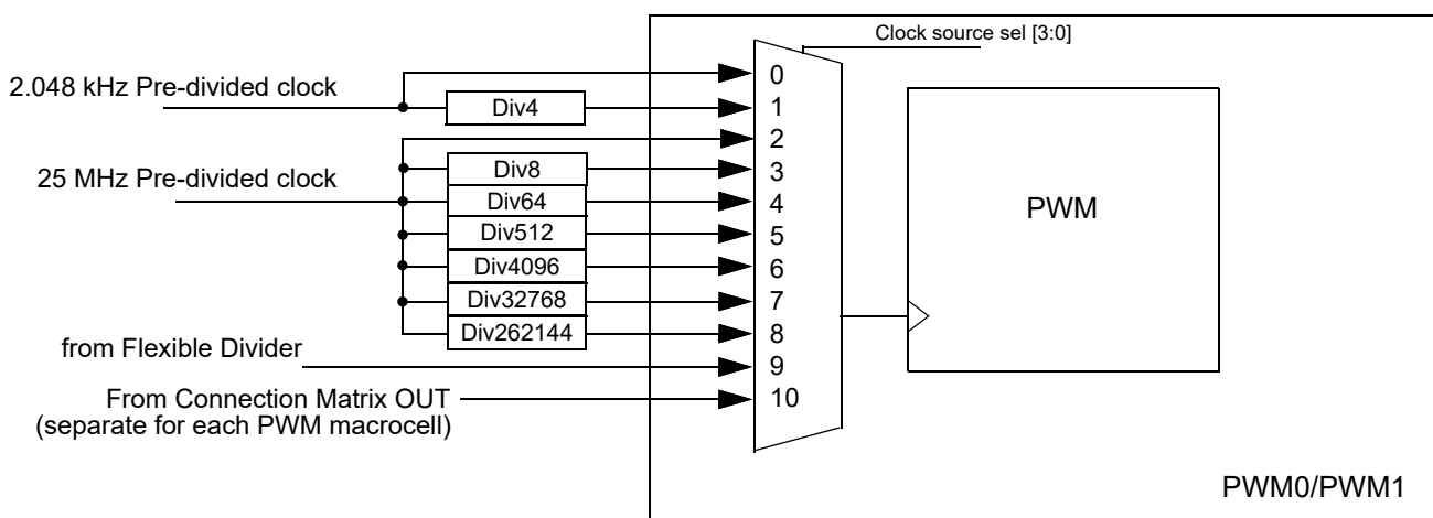
Figure 135. PWM Clock Scheme
