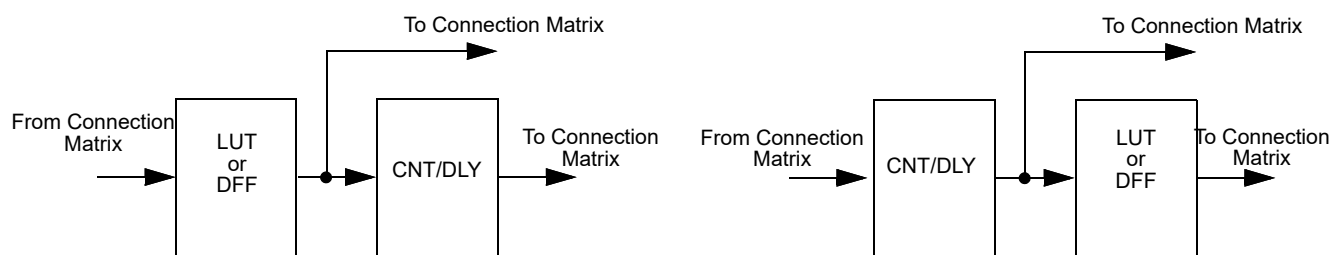
Figure 80. Possible Connections inside Multi-Function Macrocell
