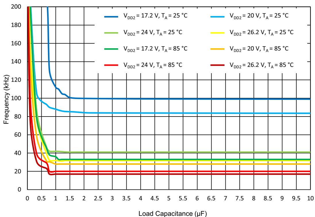
Figure 44. Full Bridge Safe Operating Area. Frequency vs. C_{\text{LOAD}} at R_{\text{LOAD}} = 20 \Omega
