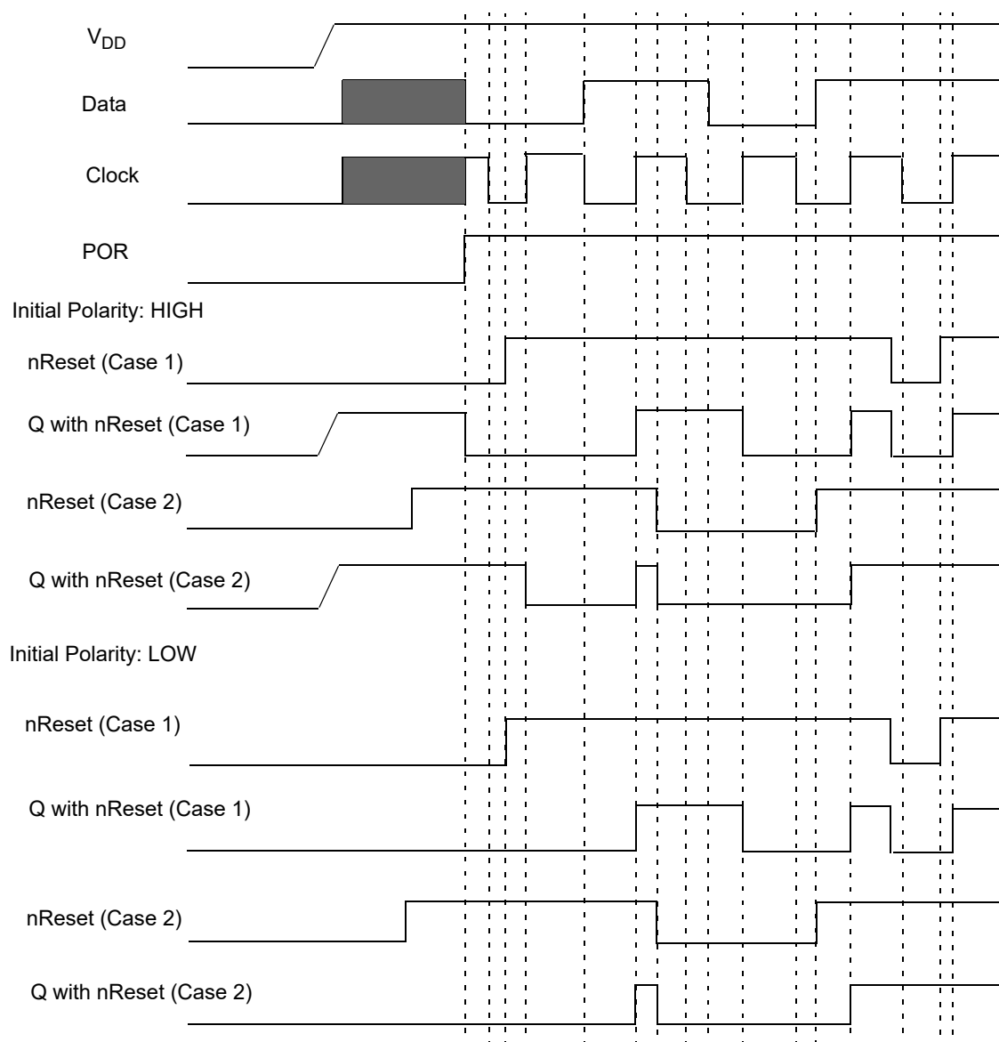
Figure 75. DFF Polarity Operations with n\text{Reset}
