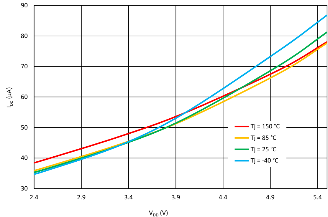
Figure 149. OSC1 Current Consumption vs. V_{DD} (Pre-Divider = 8)
