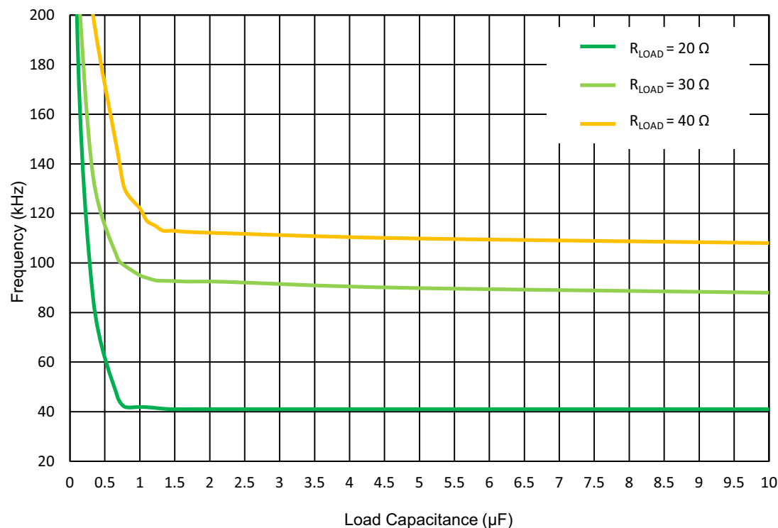
Figure 40. Full Bridge Safe Operating Area. Frequency vs. C_{\text{LOAD}} at T_A = 25\ ^\circ\text{C} , V_{\text{DD2}} = 24\ \text{V}
