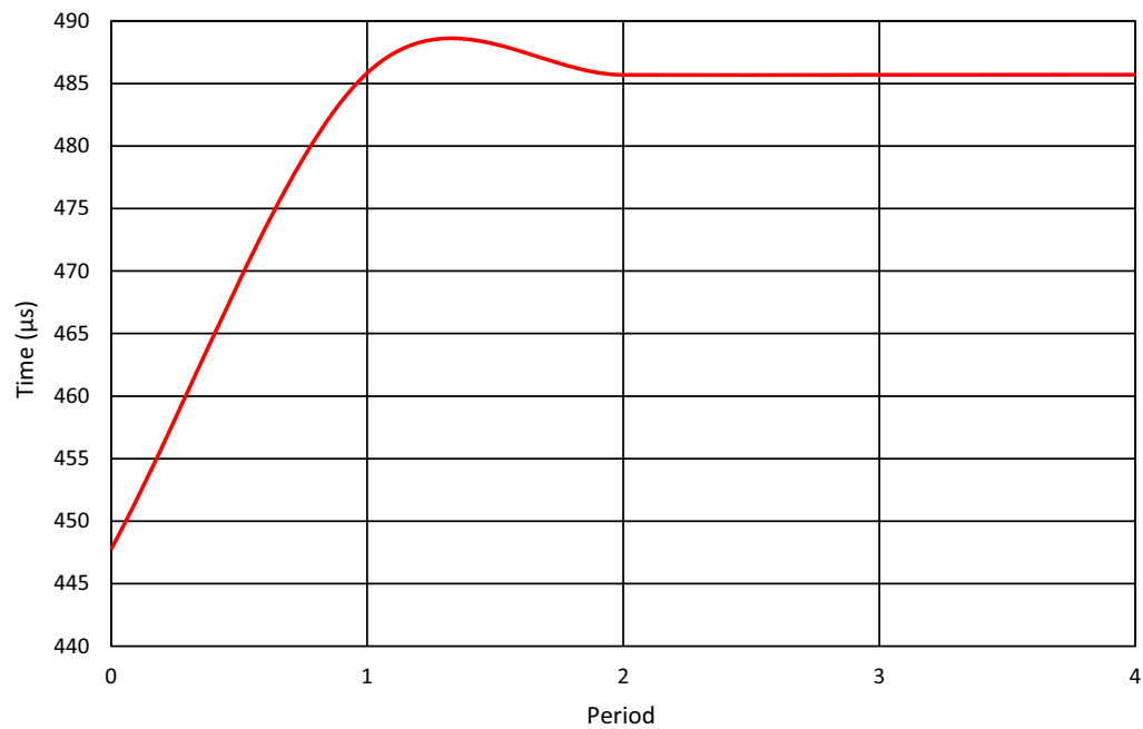
Figure 142. Oscillator0 Settling Time, V_{DD} = 3.3\text{ V} , T_A = 25\text{ }^{\circ}\text{C} , \text{OSC0} = 2\text{ kHz}
