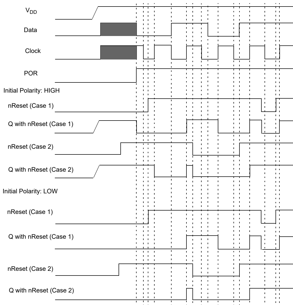
Figure 64. DFF Polarity Operations with n\text{Reset}
