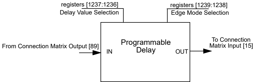
Figure 124. Programmable Delay
