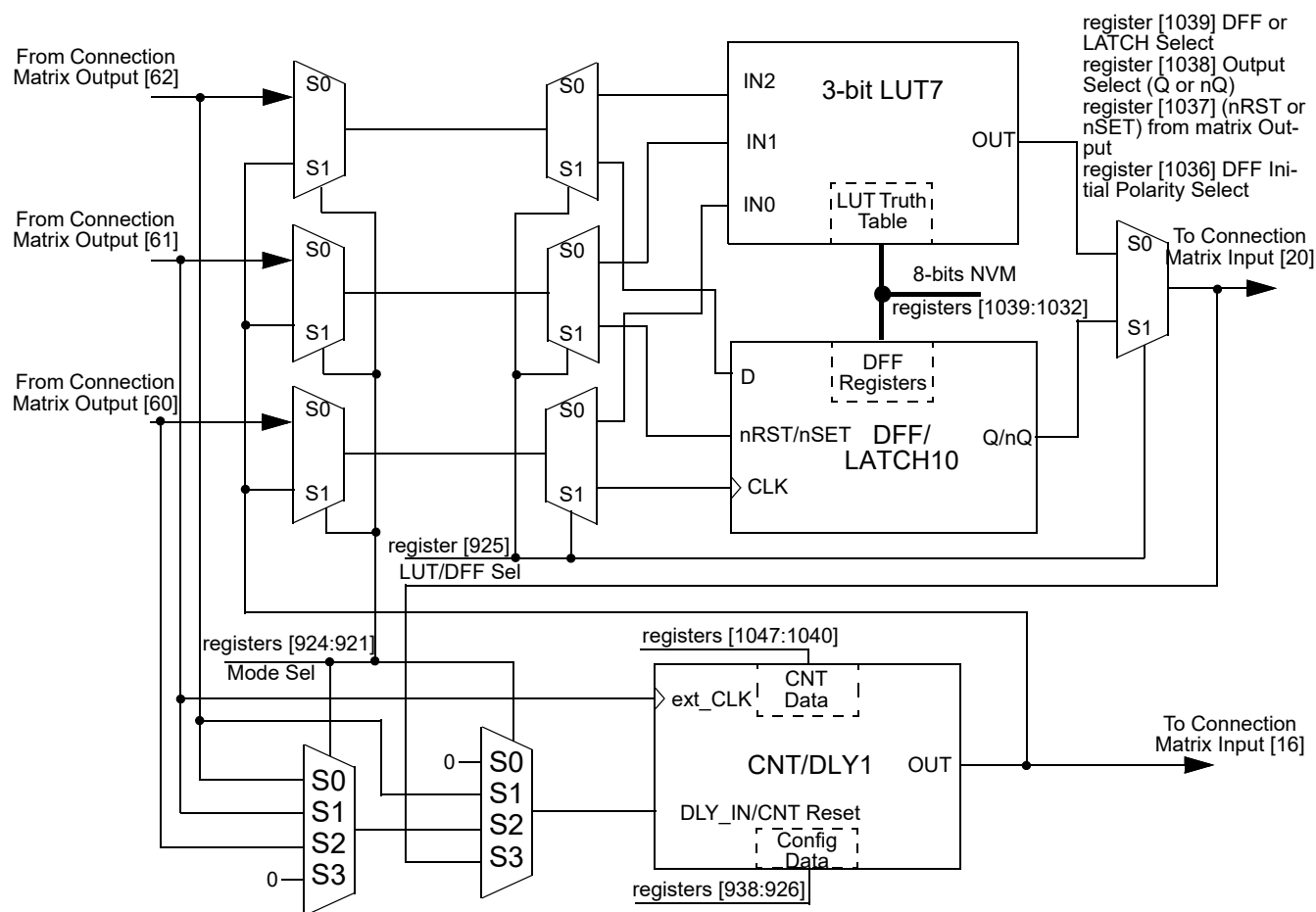
Figure 81. 8-bit Multi-Function Macrocells Block Diagram (3-bit LUT7/DFF10, CNT/DLY1)
