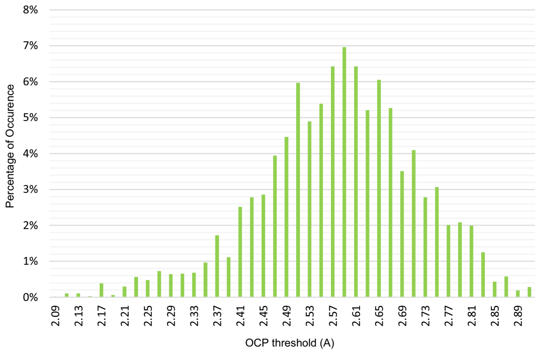
Figure 25. Full Bridge Low-side OCP Threshold Distribution at V_{DD}=2.3V to 5.5V , V_{DD2}=3V to 26.4V , T_J=-40^{\circ}C to 105^{\circ}C
