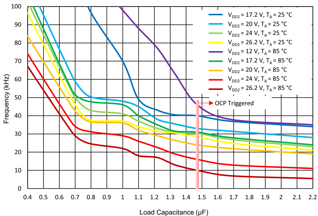
Figure 43. Two Half Bridges in Parallel Safe Operating Area. Frequency vs. C_{\text{LOAD}} at R_{\text{LOAD}} = 10 \Omega
