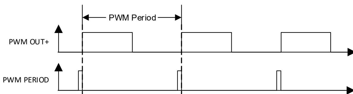
Figure 113. PWM Period Waveform
