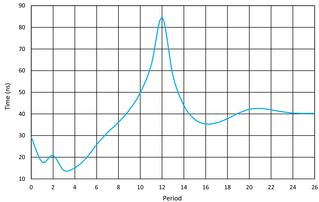
Figure 143. Oscillator1 Settling Time, V_{DD} = 3.3\text{ V} , T_A = 25\text{ }^{\circ}\text{C} , \text{OSC1} = 25\text{ MHz} (Normal Start)
