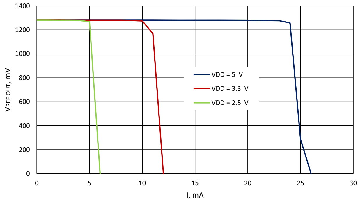
Figure 130. Typical Load Regulation, V_{ref} = 1280\text{ mV} , T_A = -40\text{ }^{\circ}\text{C} to +105\text{ }^{\circ}\text{C} , Buffer - Enabled
