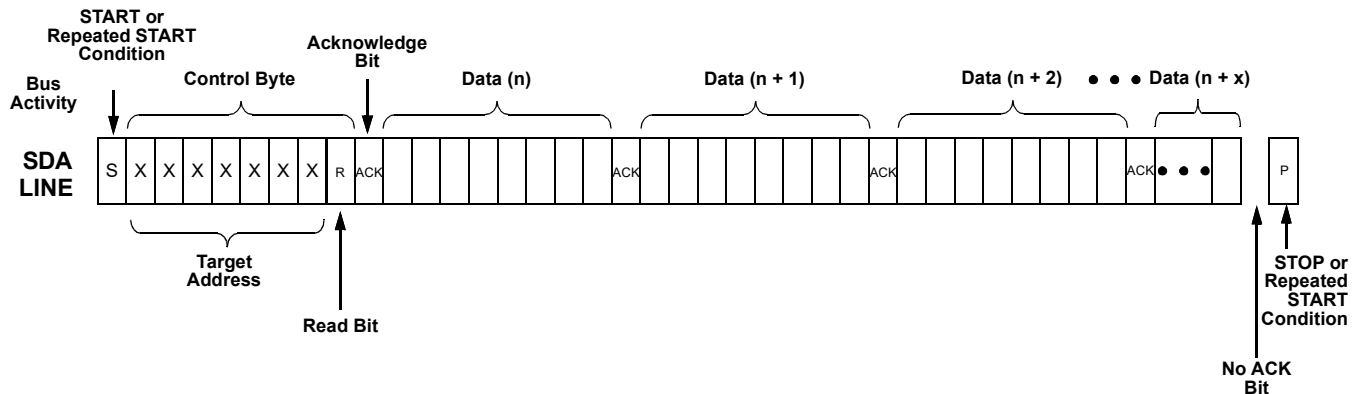
Figure 104: Sequential Read Command
