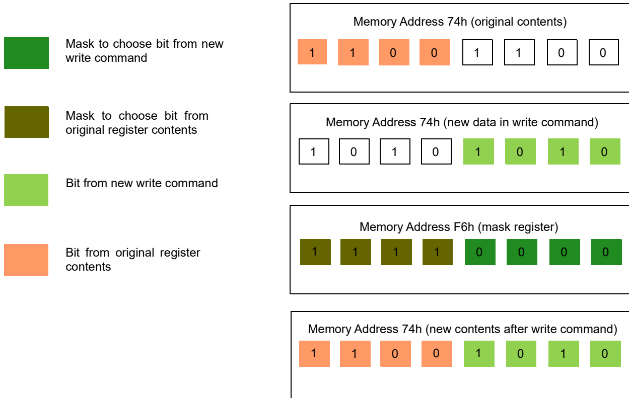
Figure 106: Example of I 2 C Byte Write Bit Masking
