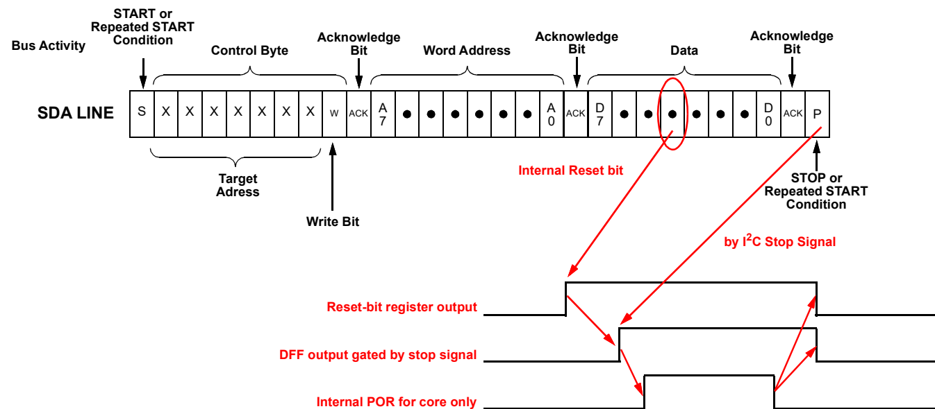
Figure 105: Reset Command Timing
