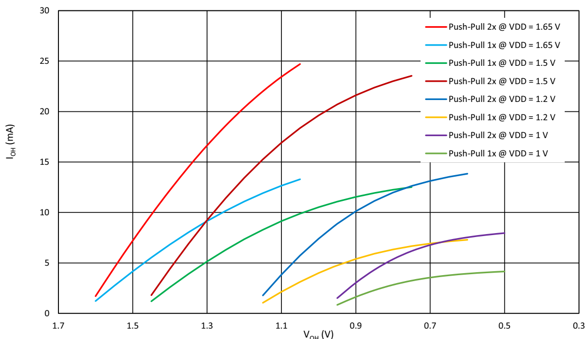
Figure 6: Typical High Level Output Current vs. High Level Output Voltage at T = +25\text{ }^{\circ}\text{C}
