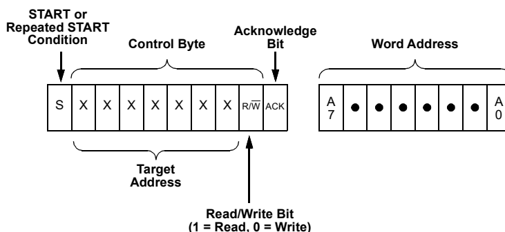
Figure 98: Basic Command Structure
