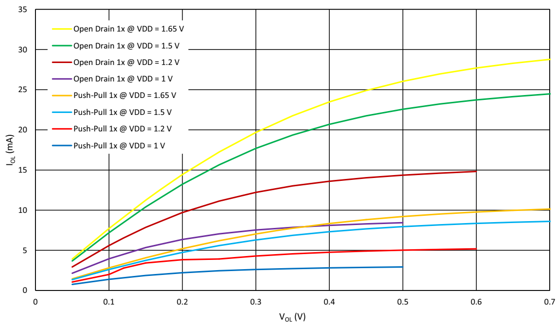
Figure 7: Typical Low Level Output Current vs. Low Level Output Voltage, 1x Drive at T = +25\text{ }^{\circ}\text{C} , Full Range
