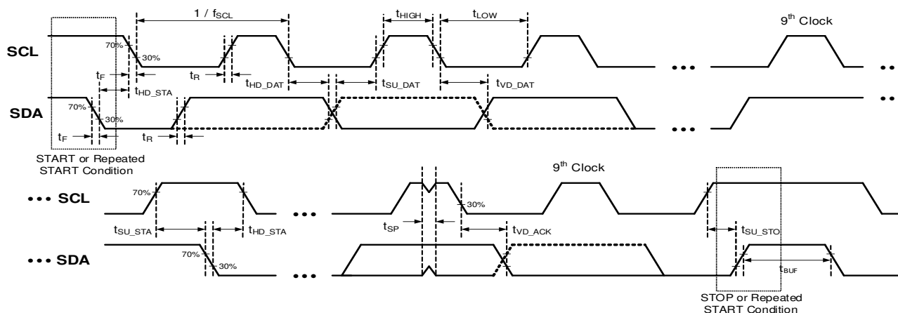
Figure 99: I 2 C General Timing Characteristics
