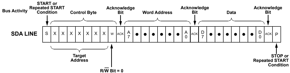
Figure 100: Byte Write Command, R/\bar{W} = 0
