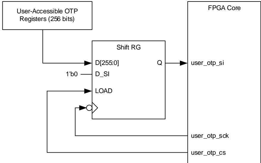
Figure 24. Serial Interface for User Access to OTP
