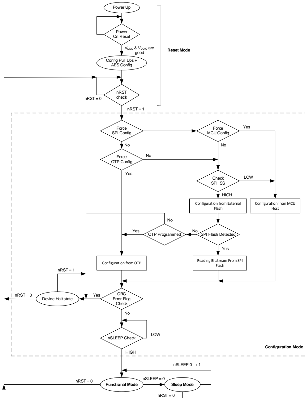
Figure 35. Power-Up Sequence
