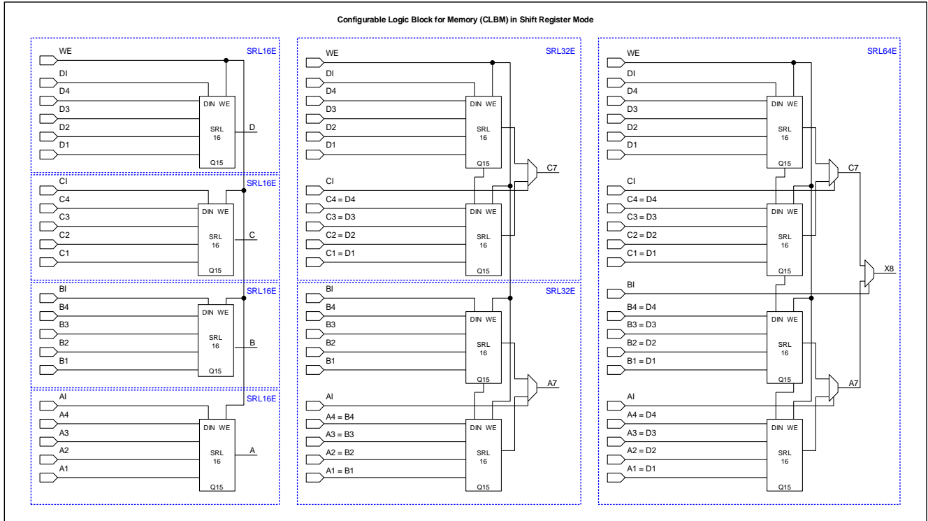
Figure 21. Configurable Logic Blocks for Memory Used in Shift Register Mode
