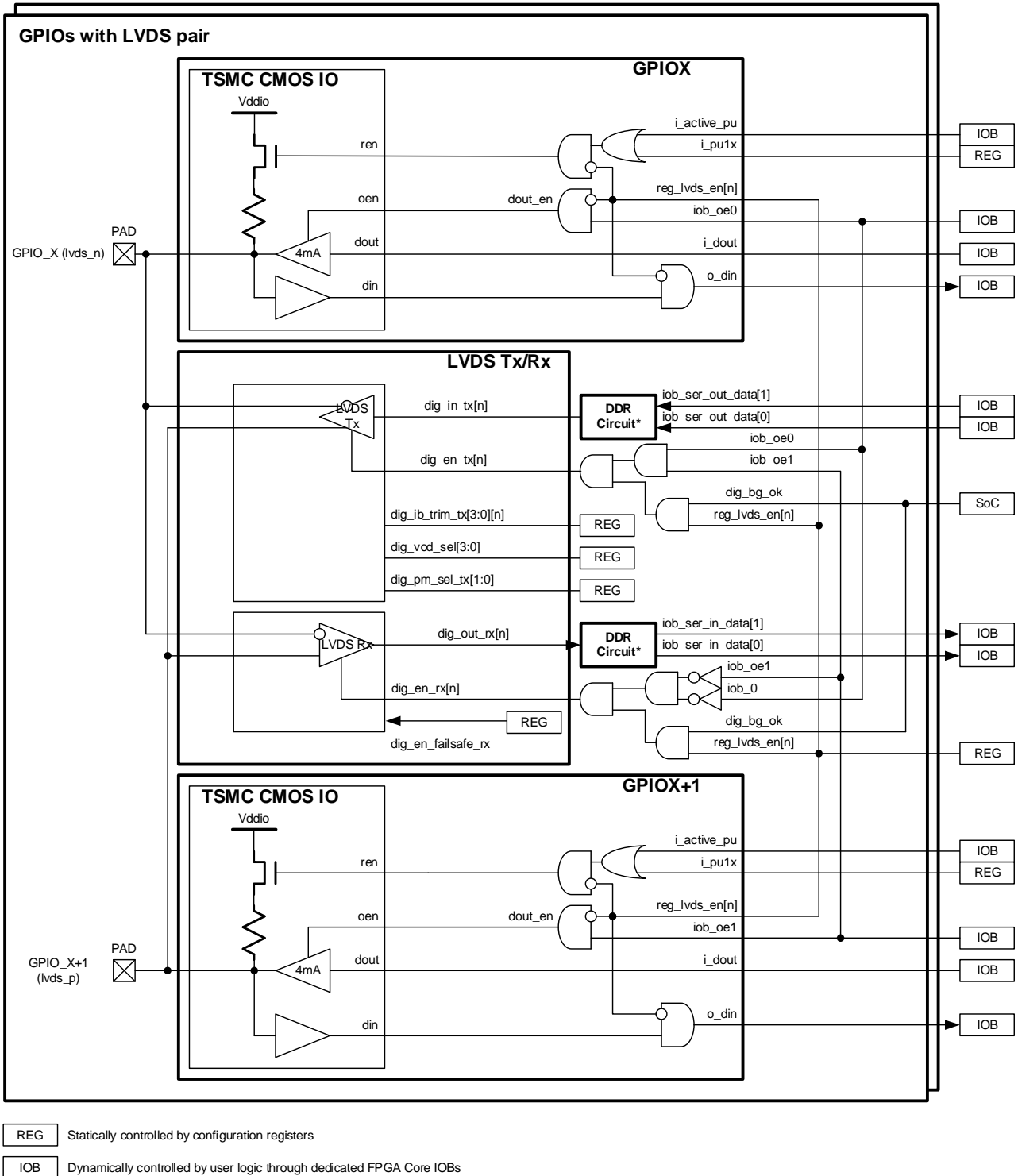
Figure 8. GPIOs Pair with LVDS Capability
