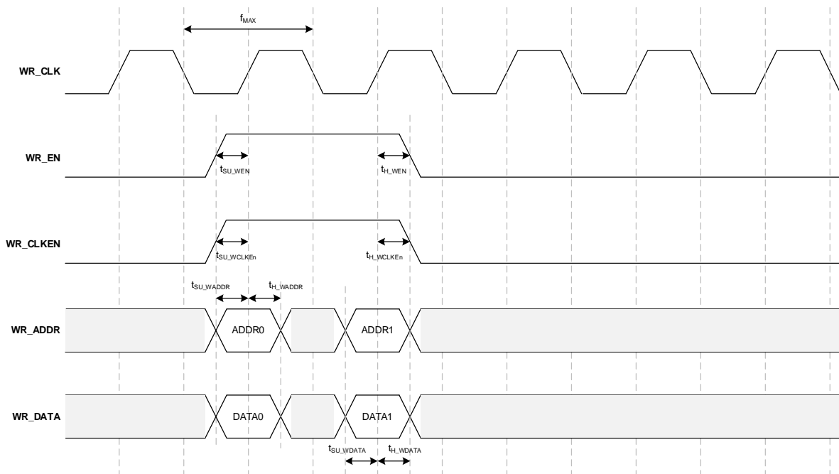
Figure 44. BRAM Write Timing Diagram
