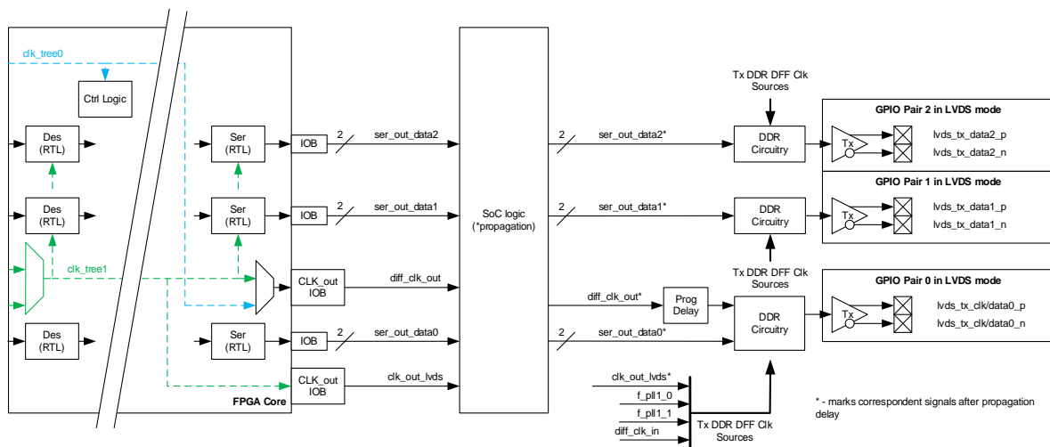
Figure 40. LVDS Output Paths
