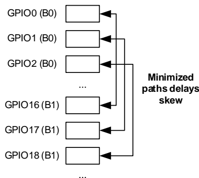
Figure 15. GPIOs Fast Routes Routing Topology
