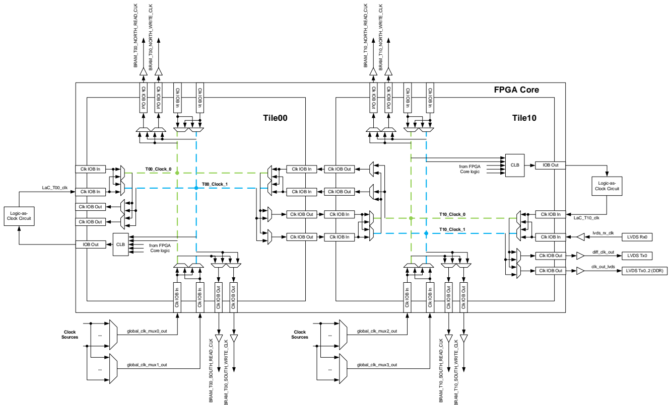
Figure 26. FPGA Core Clock IOBs Connection
