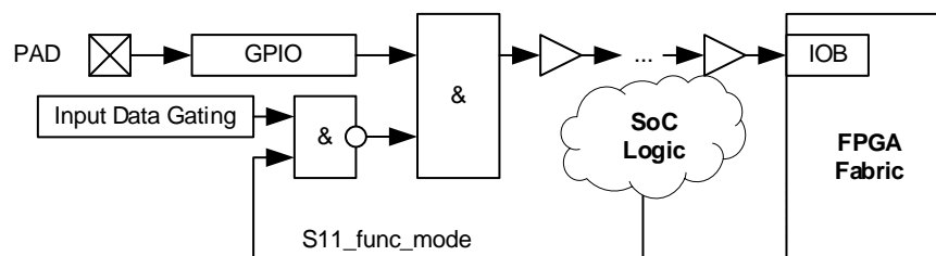
Figure 13. Input Path Optional Gating
