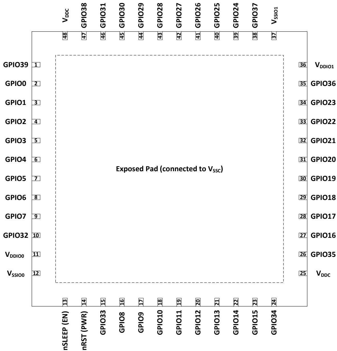
Figure 3. Pin Assignments for 48-pin LQFN Package
