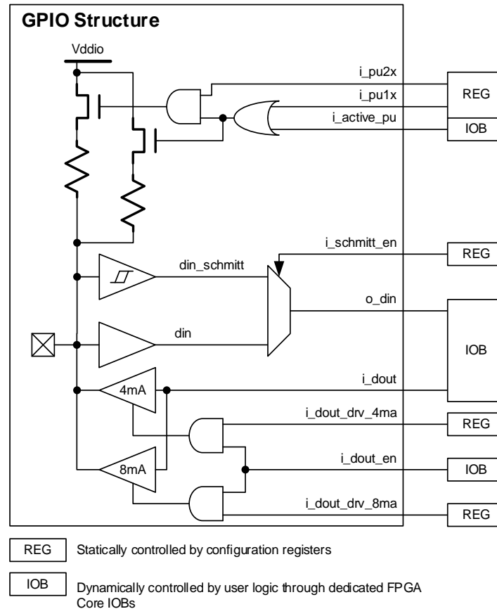
Figure 7. GPIO Buffers
