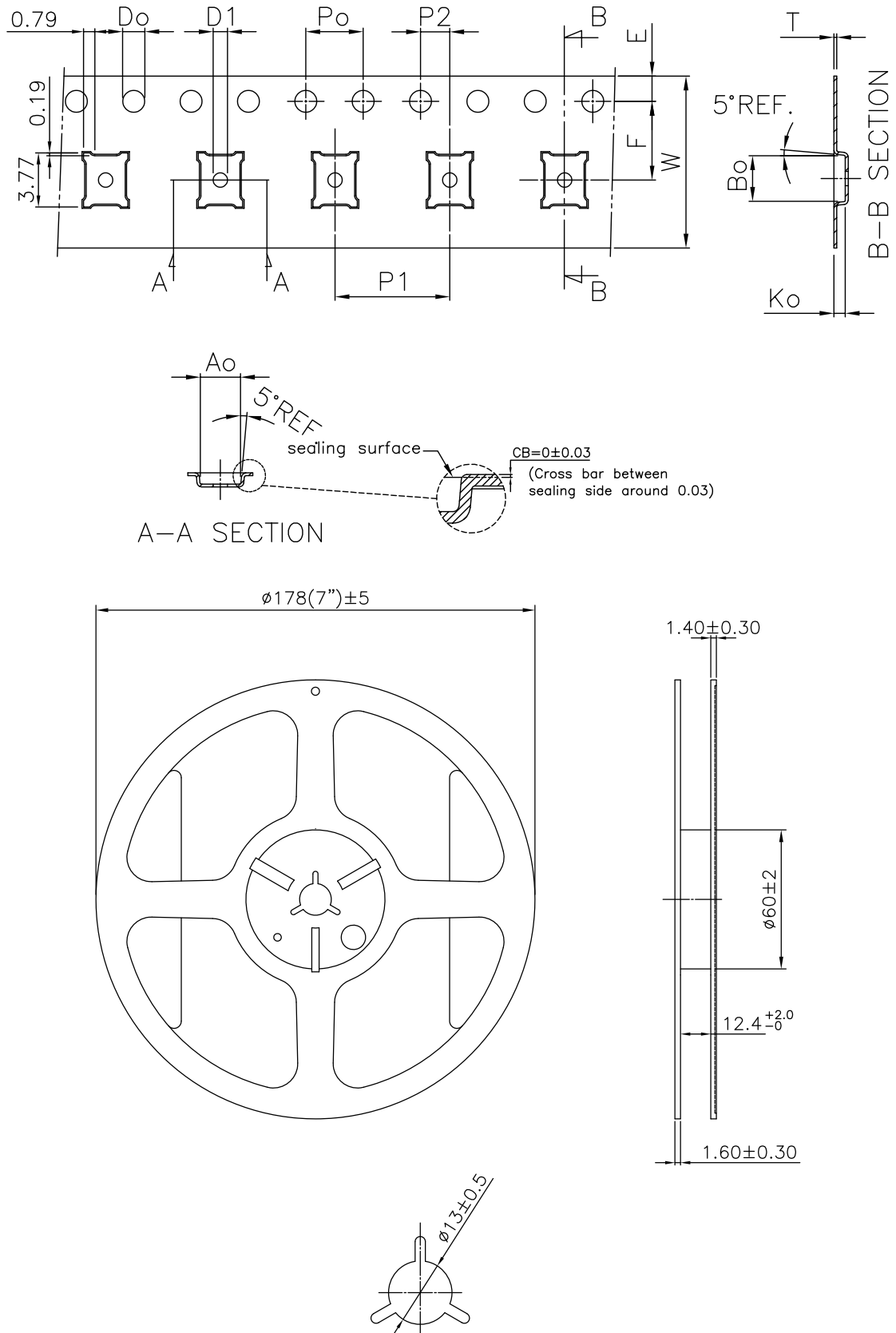
Figure 56. Tape and Reel Drawing for WLCSP-48
