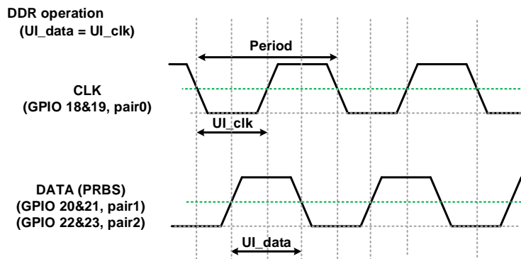
Figure 6. DDR Data and Clock Rates
