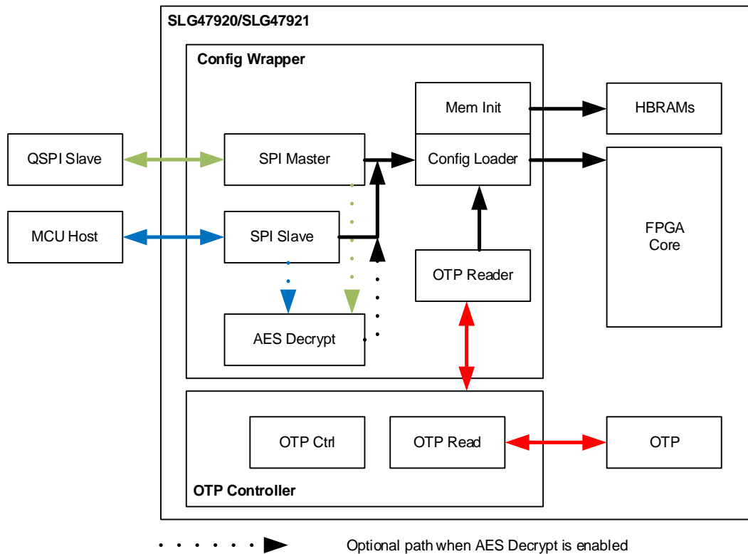
Figure 46. FPGA Core Configuration Paths
