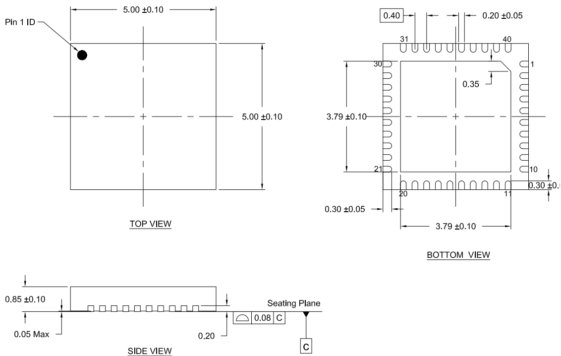
Figure 47. Package Outline Drawing LQFN-40
