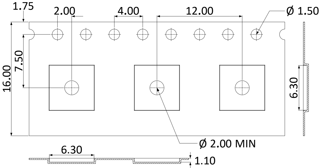
Figure 58. Tape Drawing for LQFN-40
