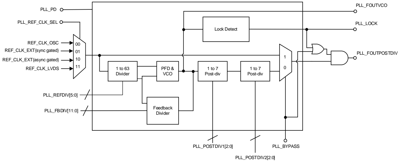
Figure 30. Phase-Locked Loop Block Diagram
