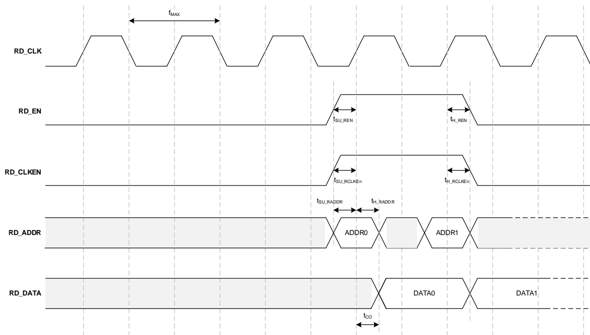
Figure 45. BRAM Read Timing Diagram
