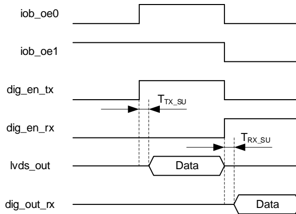
Figure 10. LVDS Bi-Directional Operation
