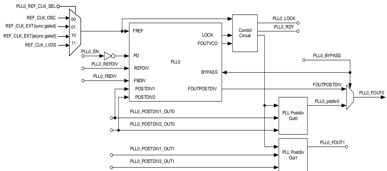
Figure 31. PLL0 with External Post Dividers
