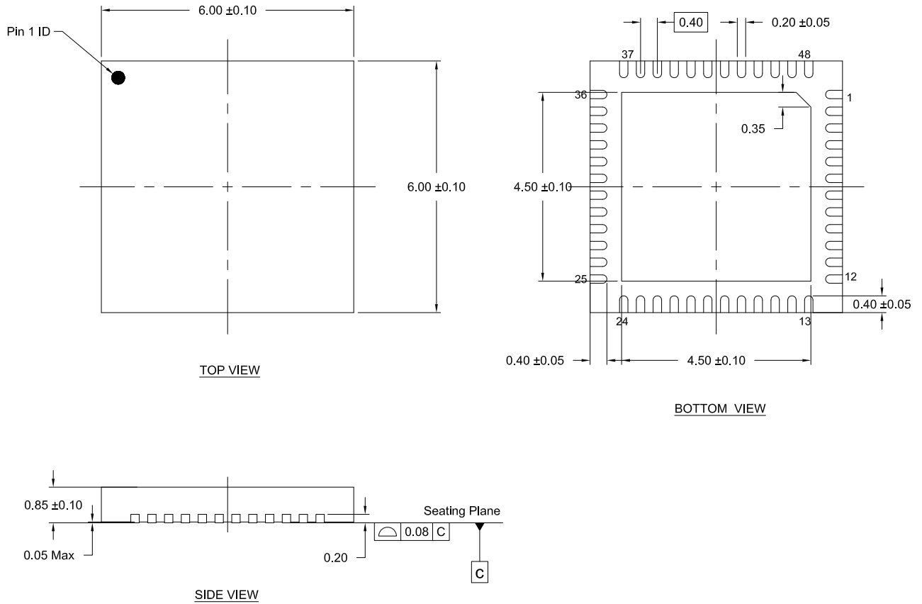
Figure 48. Package Outline Drawing LQFN-48
