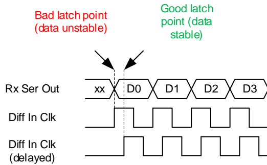
Figure 39. Delayed Input Differential Clock Usage
