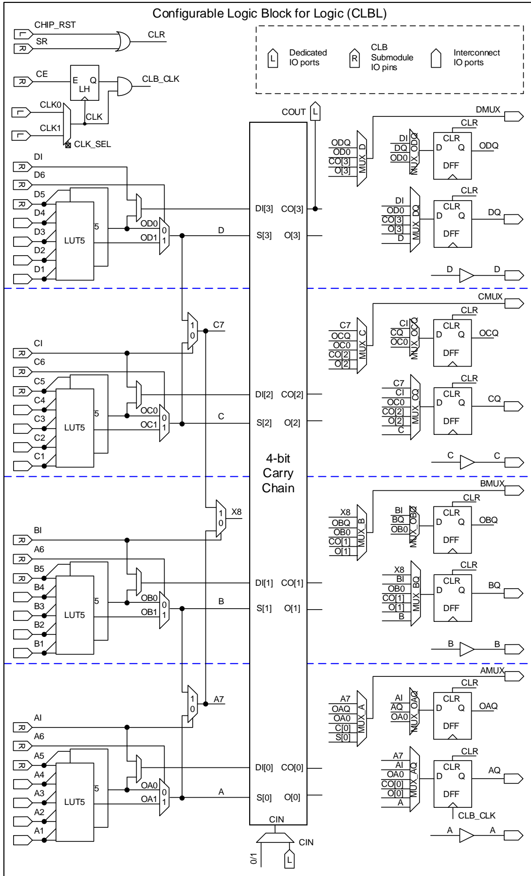
Figure 19. Configurable Logic Blocks for Logic (Part 2)
