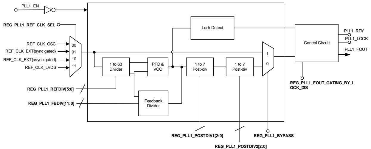
Figure 33. PLL1
