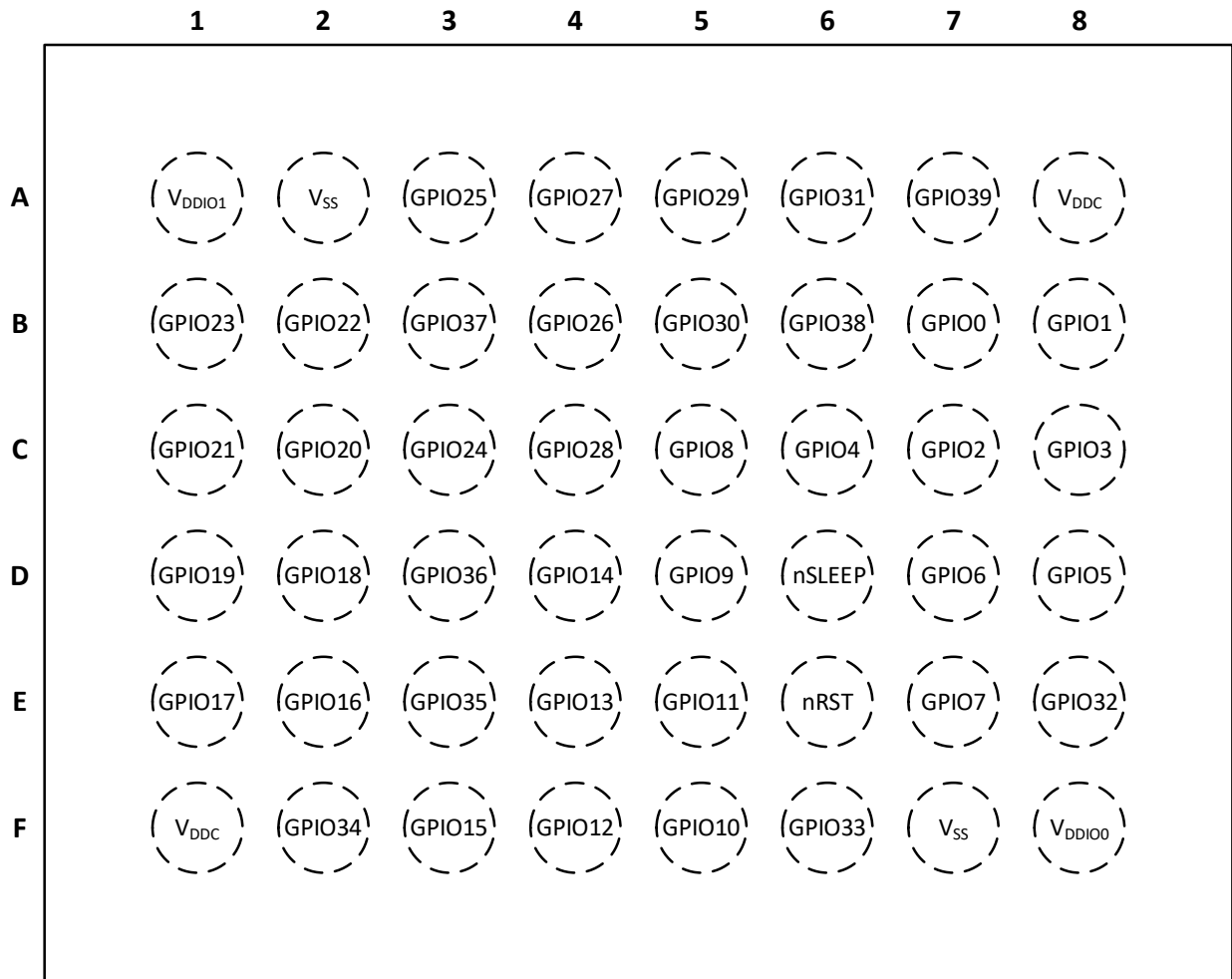
Figure 4. Pin Assignments for 48-pin WLCSP Package (Top View)
