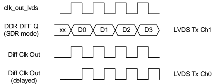
Figure 41. Delayed Output Differential Clock Usage
