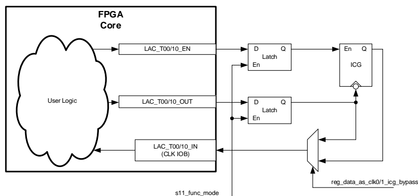
Figure 34. Logic-As-Clock Usage
