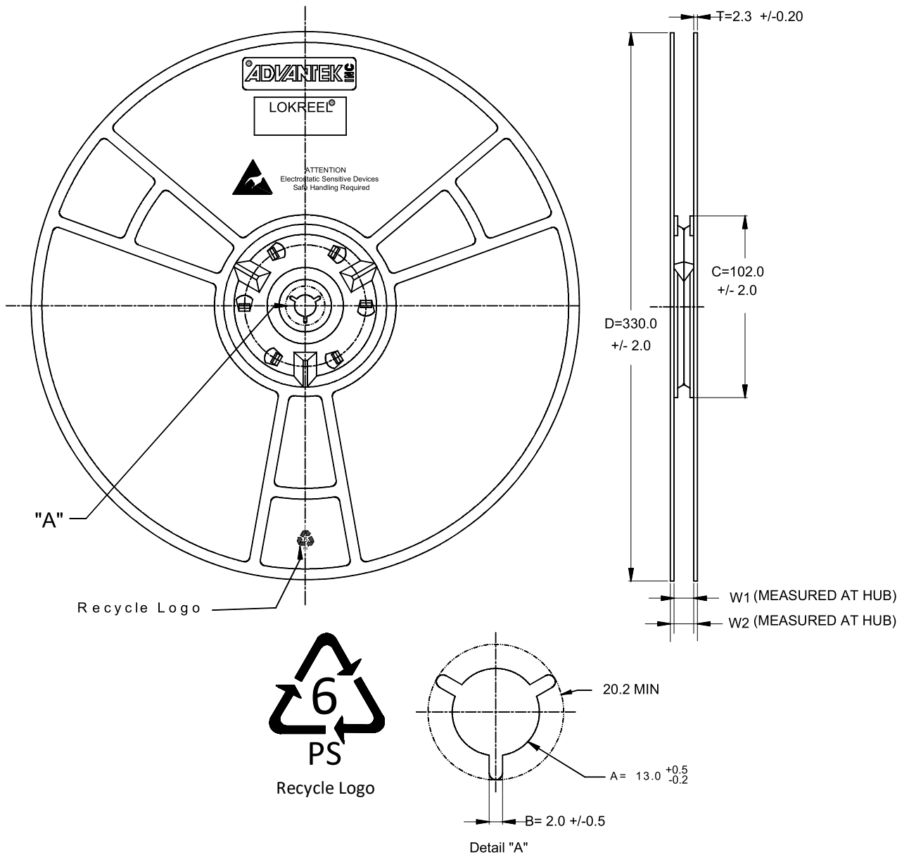
Figure 57. Reel Drawing for LQFN-40 and LQFN-48
