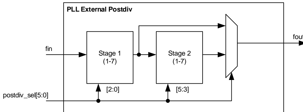
Figure 32. External POSTDIV Architecture
