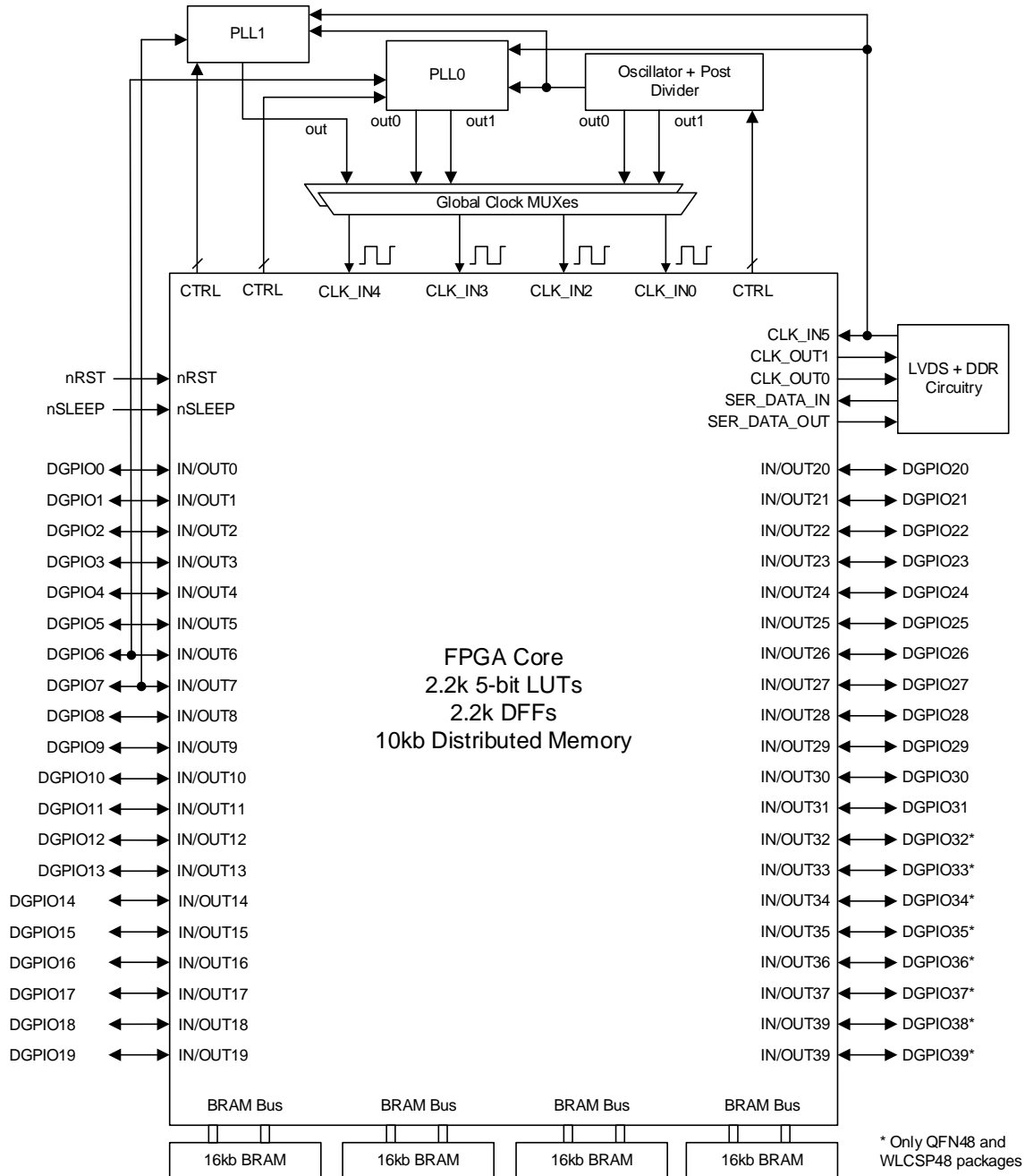
Figure 16. Peripheral Connections to FPGA Core
