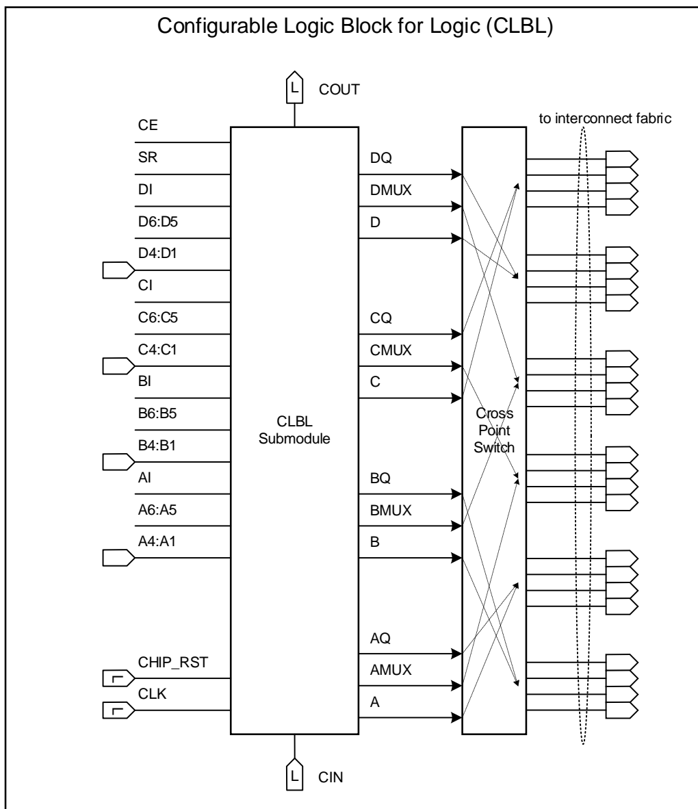
Figure 18. Configurable Logic Blocks for Logic (Part 1)
