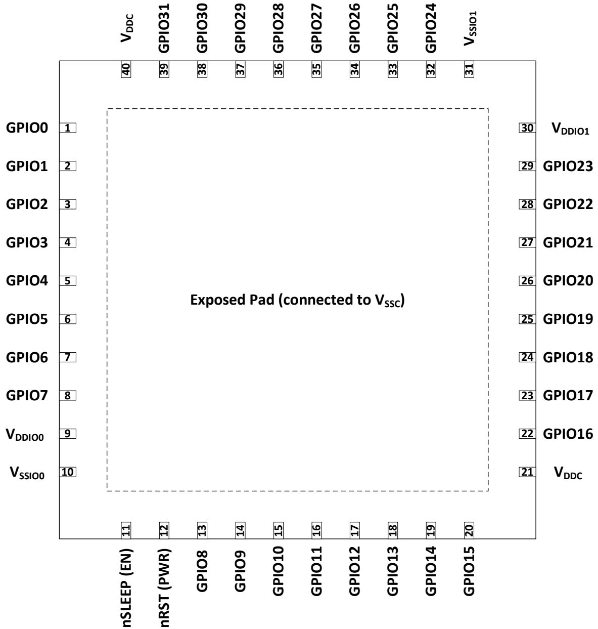
Figure 2. Pin Assignments for 40-pin LQFN Package
