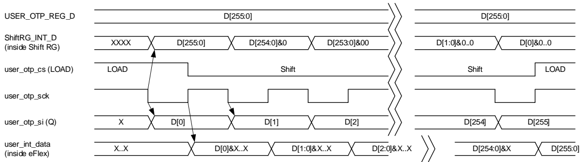
Figure 25. Serial Interface for User Accesses to OTP (Timing Diagram)
