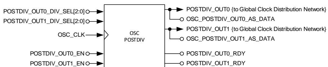
Figure 29. Oscillator Post Divider
