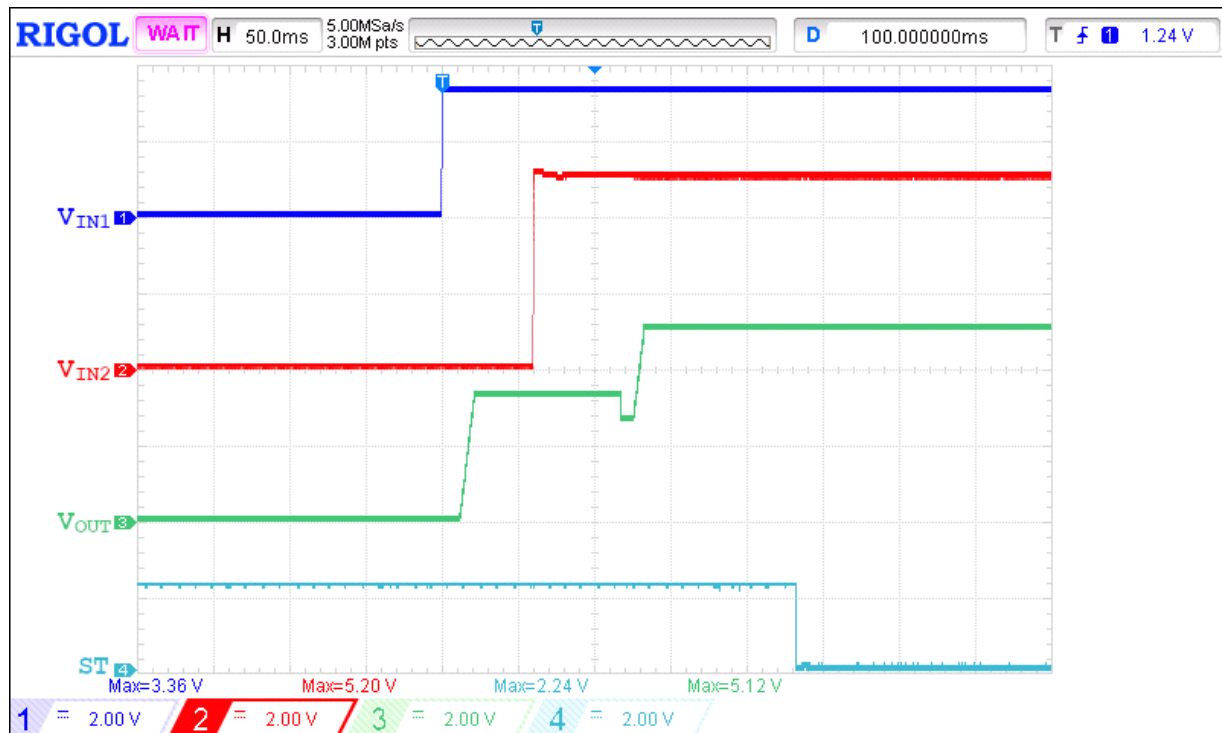
Figure 11. Higher voltage level priority operation waveform for V_{IN1} = 3.3\text{ V} , V_{IN2} = 5\text{ V} , SEL = 0\text{ V} , PR = 0\text{ V} , C_{SS} = 220\text{ nF} , R_{LOAD} = 100\text{ }\Omega , C_{LOAD} = 2\text{ }\mu\text{F}
