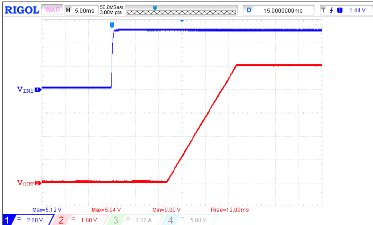
Figure 1. Typical Turn ON operation waveform for V_{IN1} = 5\text{ V} , C_{SS} = 220\text{ nF} , R_{LOAD} = 100\text{ }\Omega , C_{LOAD} = 2\text{ }\mu\text{F}
