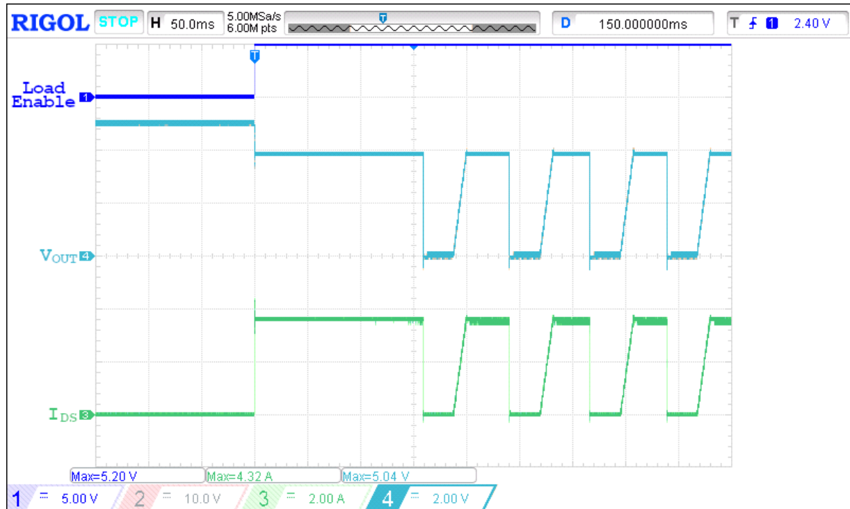
Figure 17. Active Current Limit operation waveform for V_{IN[1,2]} = 5\text{ V} , C_{SS} = 220\text{ nF} , R_{ILIM} = 31.6\text{ k}\Omega , R_{LOAD} = 1.1\text{ }\Omega , C_{LOAD} = 2\text{ }\mu\text{F}
