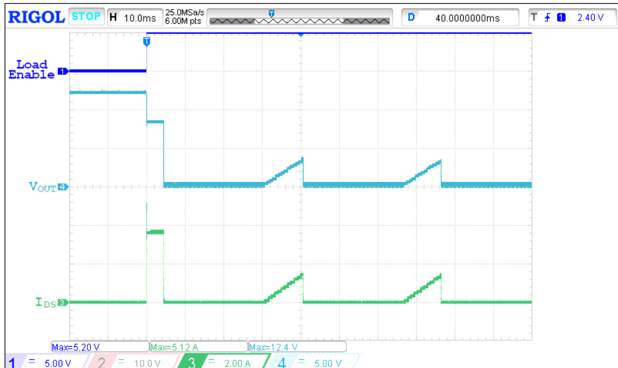
Figure 18. Active Current Limit operation waveform for V_{IN[1,2]} = 12\text{ V} , C_{SS} = 220\text{ nF} , R_{ILIM} = 31.6\text{ k}\Omega , R_{LOAD} = 2.2\text{ }\Omega , C_{LOAD} = 2\text{ }\mu\text{F}
