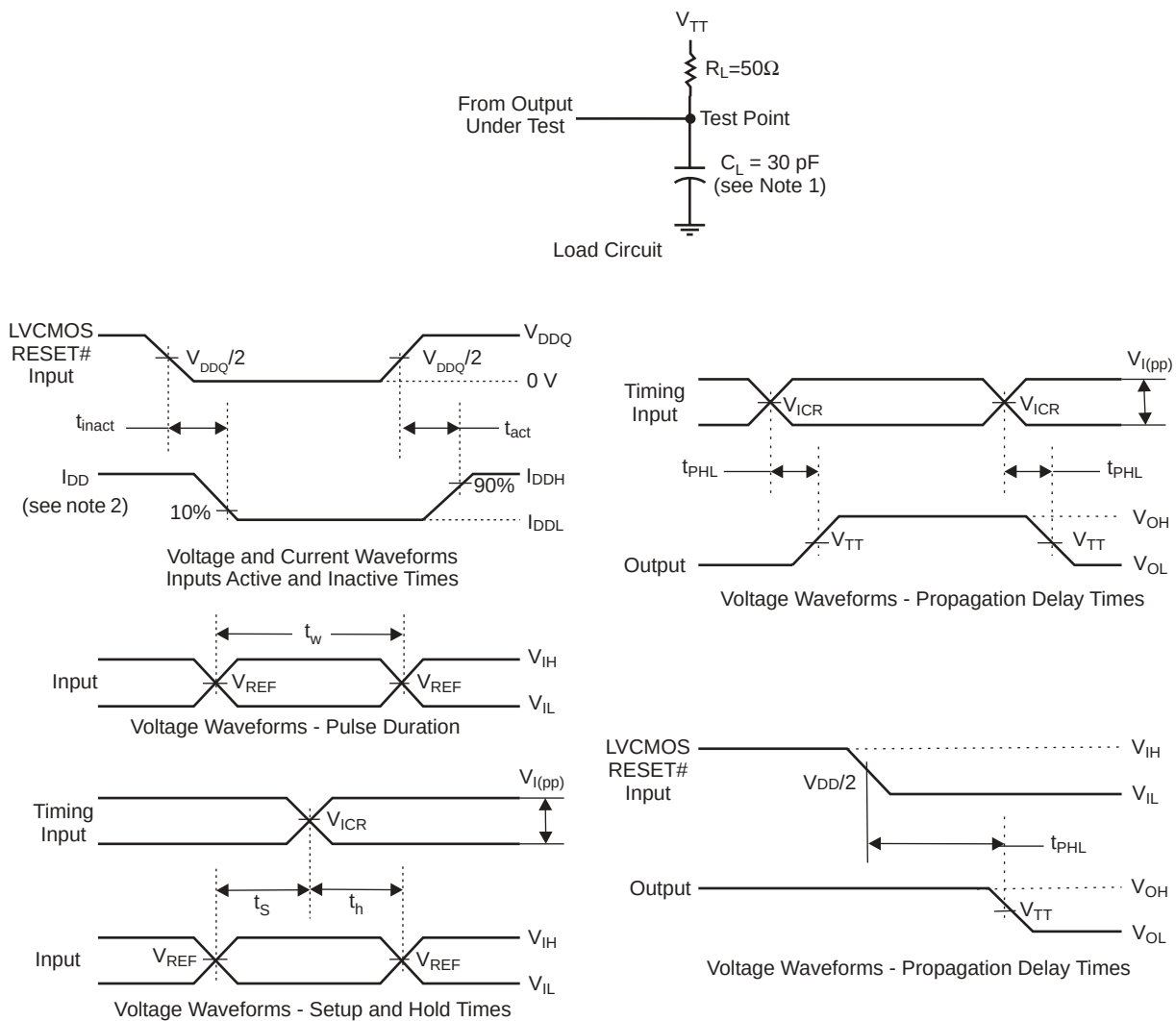
Figure 1 - Parameter Measurement Information ( V_{DDQ} = 2.5\text{V} \pm 0.2\text{V} )
