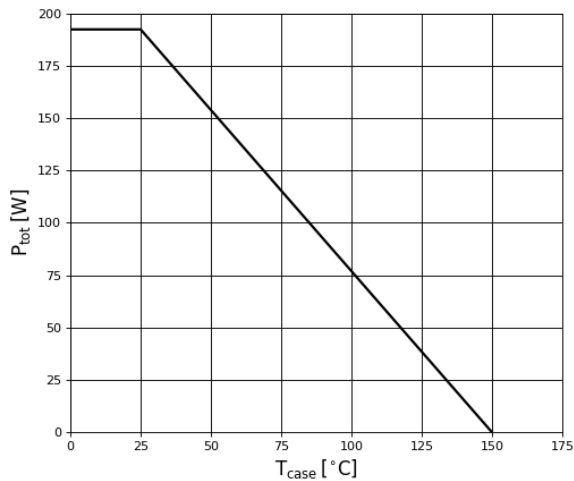
Figure 10. Power Dissipation
