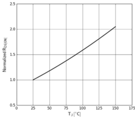
Figure 5. Normalized On-resistance I_D = 30\text{A} , V_{GS} = 12\text{V}
