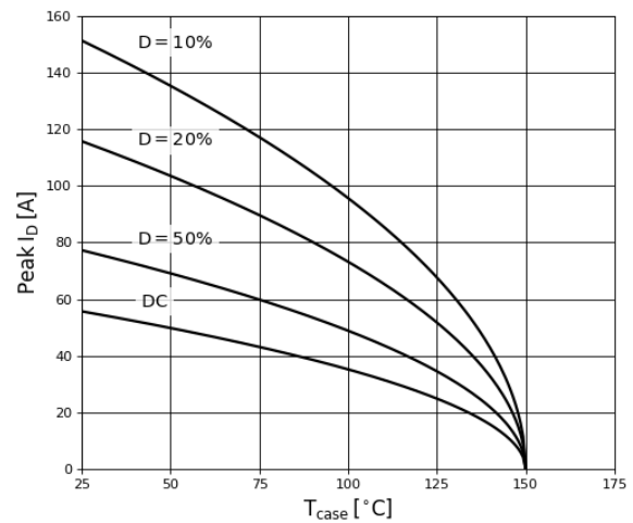
Figure 11. Current Derating
