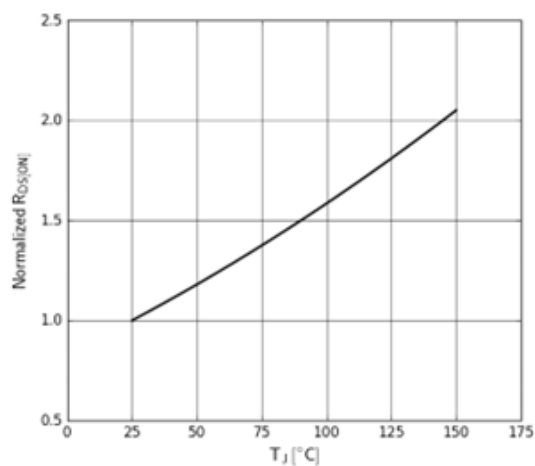
Figure 5. Normalized On-resistance
