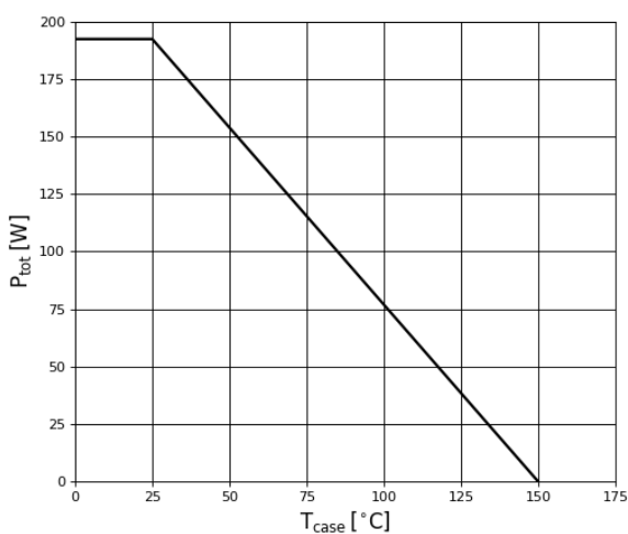
Figure 10. Power Dissipation
