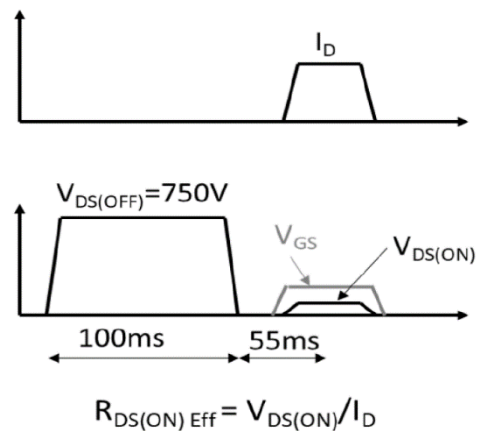
Figure 21. Dynamic R_{DS(on)eff} Waveform
