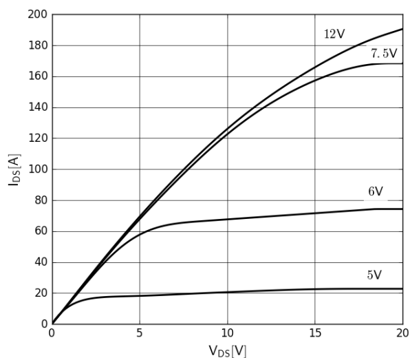
Figure 2. Typical Output Characteristics T_J=175^\circ\text{C} Parameter: V_{GS}
