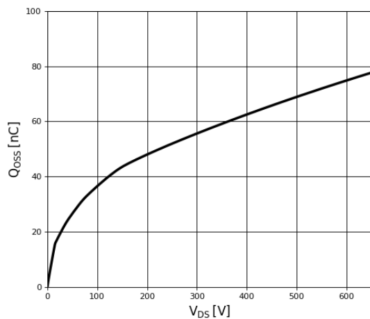
Figure 8. Typical Q_{oss}
