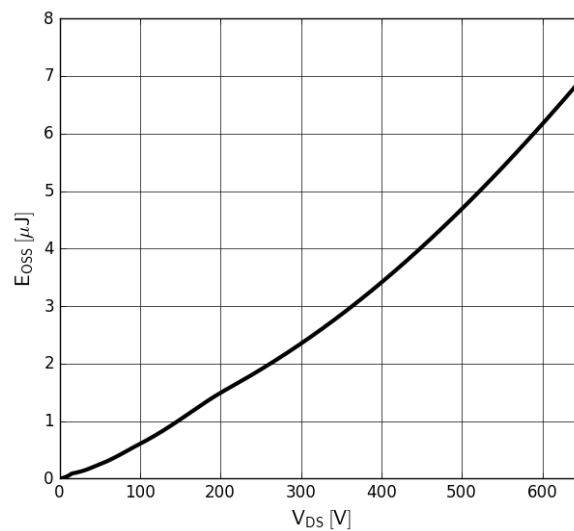
Figure 7. Typical C_{OSS} Stored Energy
