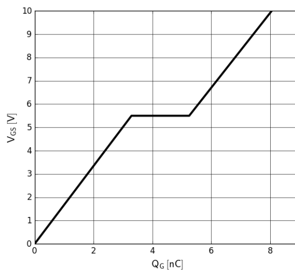
Figure 9. Typical Gate Charge
