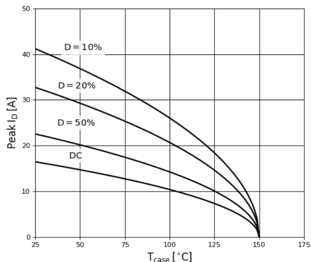
Figure 11. Current Derating
