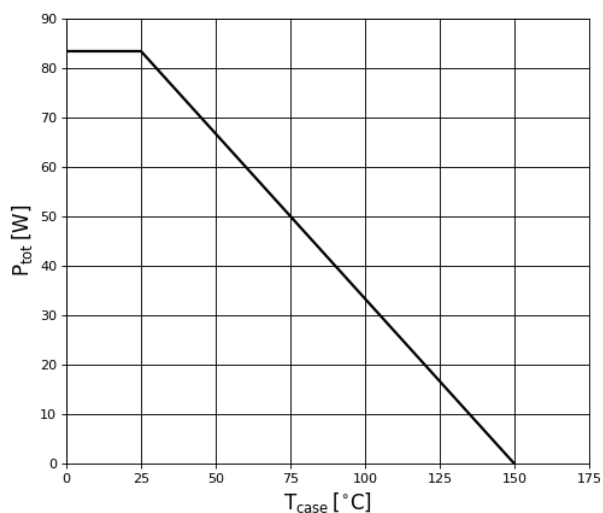
Figure 10. Power Dissipation
