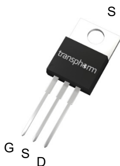
Figure 1. Pin Assignments
