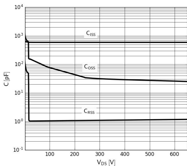
Figure 6. Typical Capacitance
