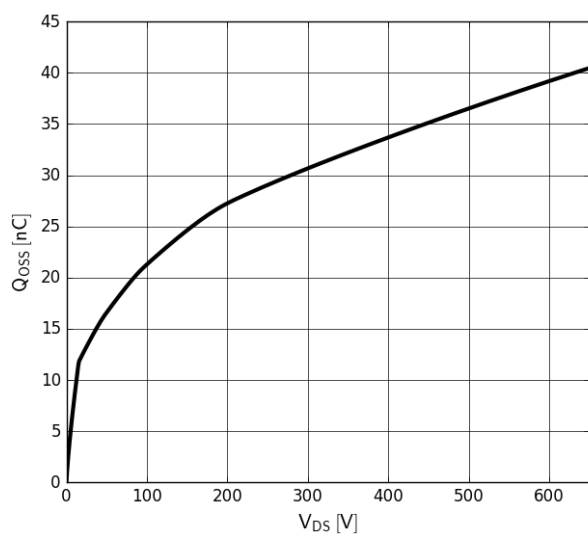
Figure 8. Typical Q_{OSS}
