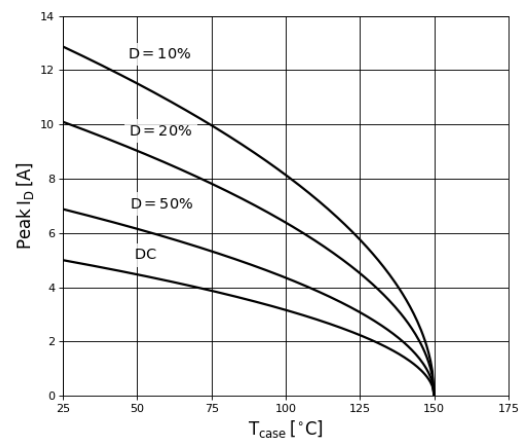
Figure 11. Current Derating
