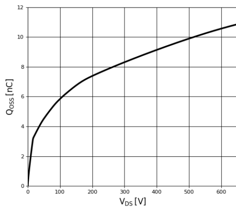
Figure 8. Typical Q_{oss}
