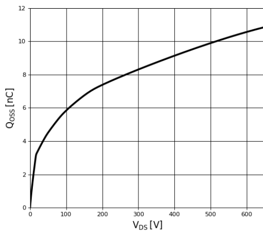
Figure 8. Typical Q_{oss}
