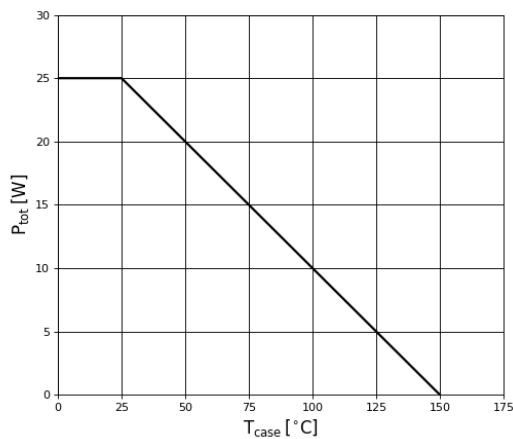
Figure 10. Power Dissipation
