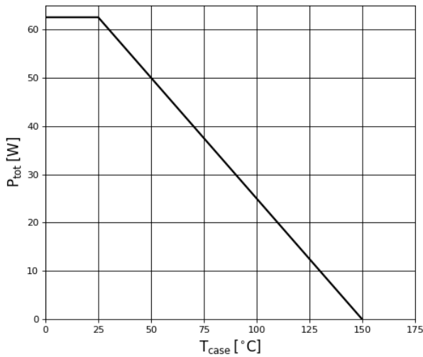
Figure 10. Power Dissipation
