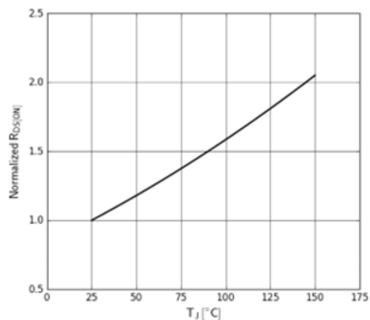
Figure 5. Normalized On-resistance I_D = 10\text{A} , V_{GS} = 10\text{V}
