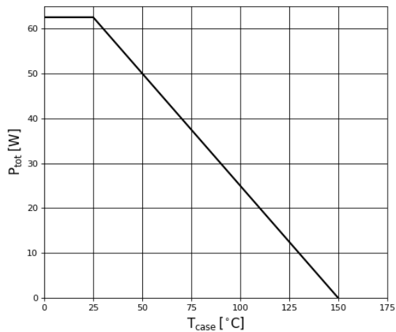
Figure 10. Power Dissipation
