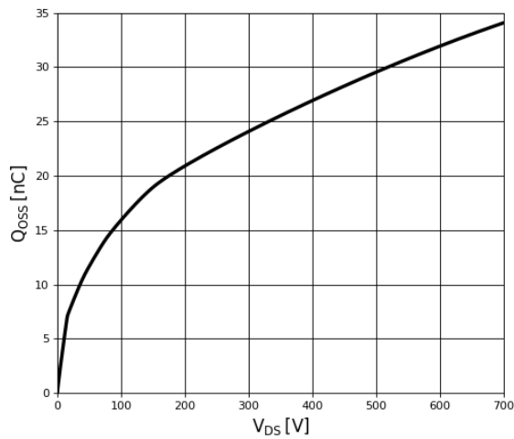
Figure 8. Typical Q_{oss}
