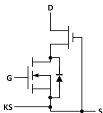
Cascode Device Structure
