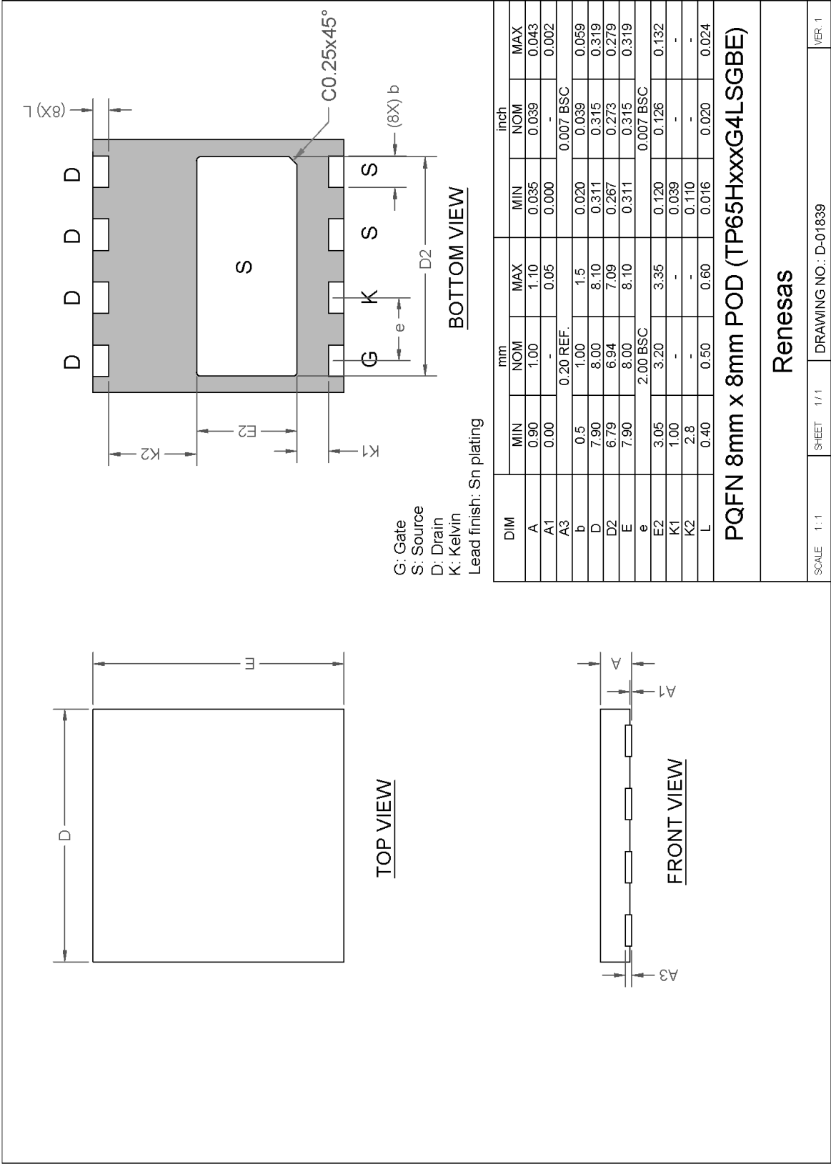
Figure 19. 8 x 8 mm PQFN Package Outline Drawing
