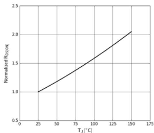
Figure 5. Normalized On-resistance
