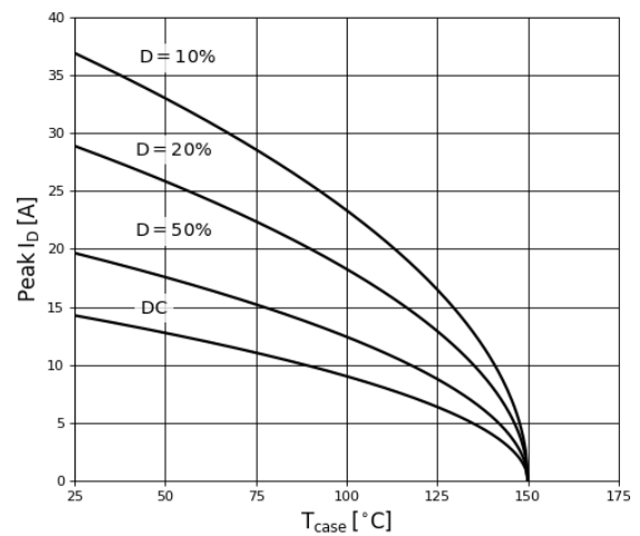
Figure 11. Current Derating
