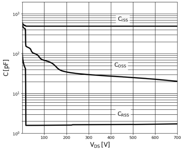
Figure 6. Typical Capacitance
