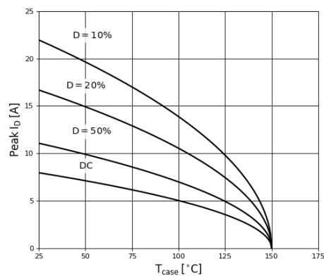
Figure 11. Current Derating
