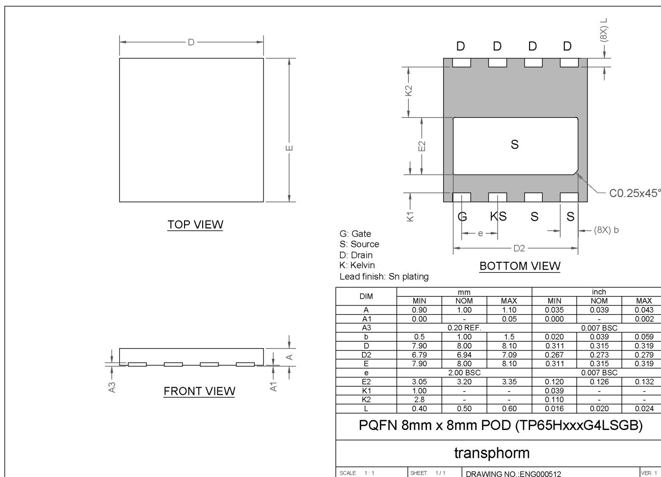
Figure 19. Package Outline Drawing – 8 × 8 PQFN
