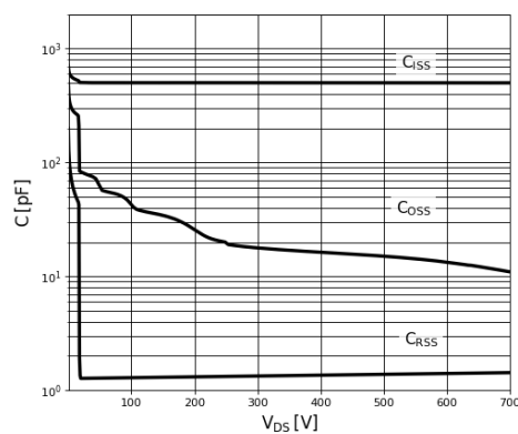
Figure 6. Typical Capacitance
