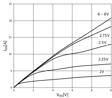
Figure 3. Typical Output Characteristics, T_J = 150^\circ\text{C}
