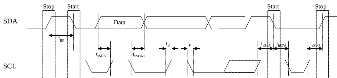
Fig21 Serial Host Interface Timing
