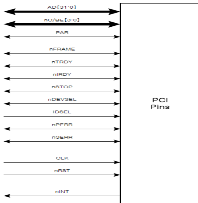
FIGURE 17. PCI PINS INTERFACE
