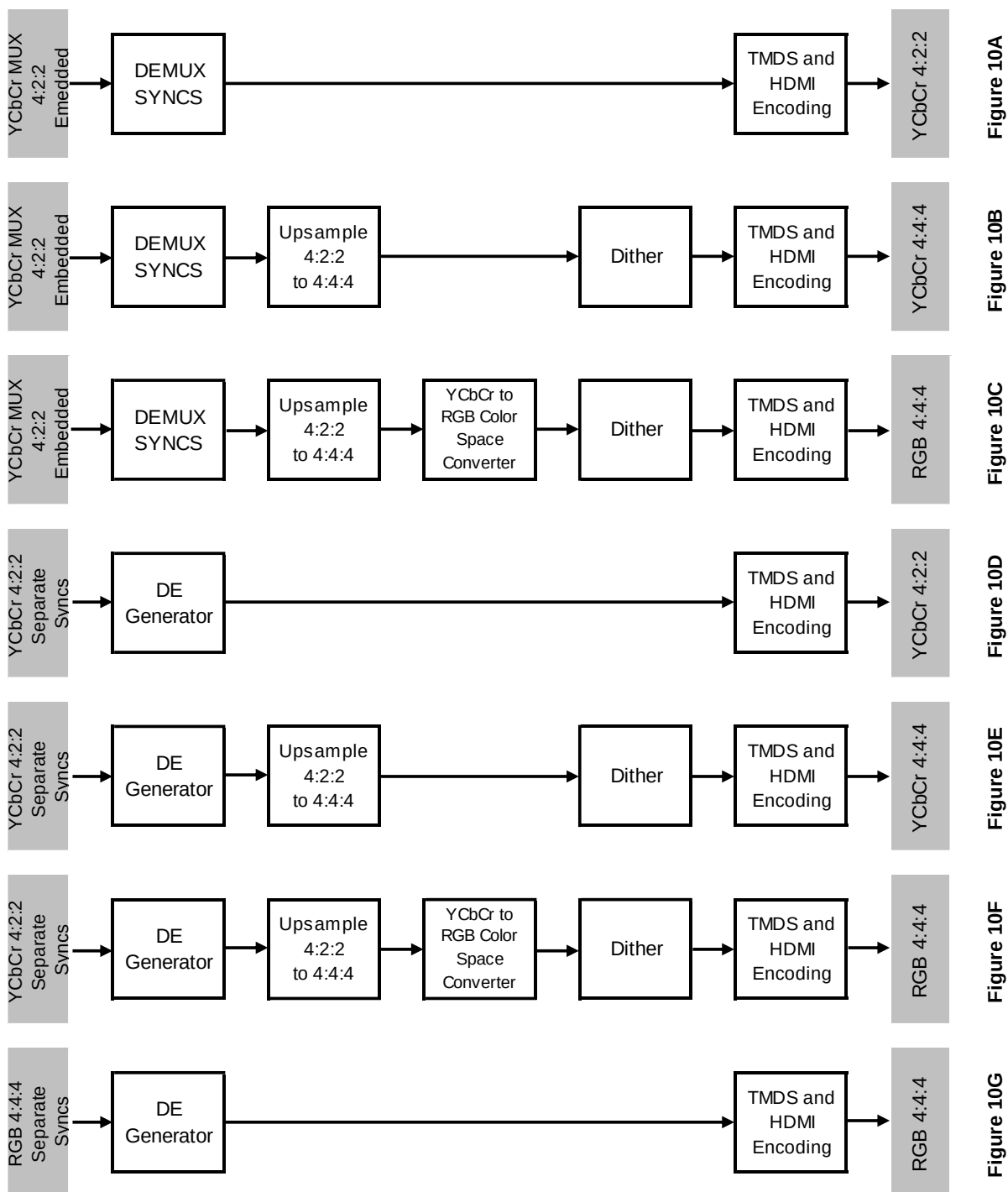
Figure 8-12 Video Input to Video Output Data Flow
