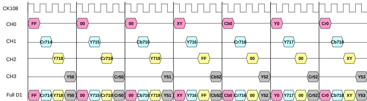
Four Channel Input with 1 Port for Full D1
