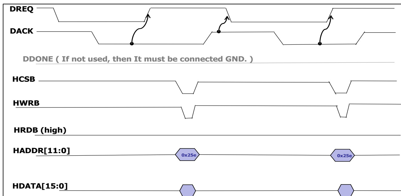
Single service in Handshake Mode with Single Transfer Size
