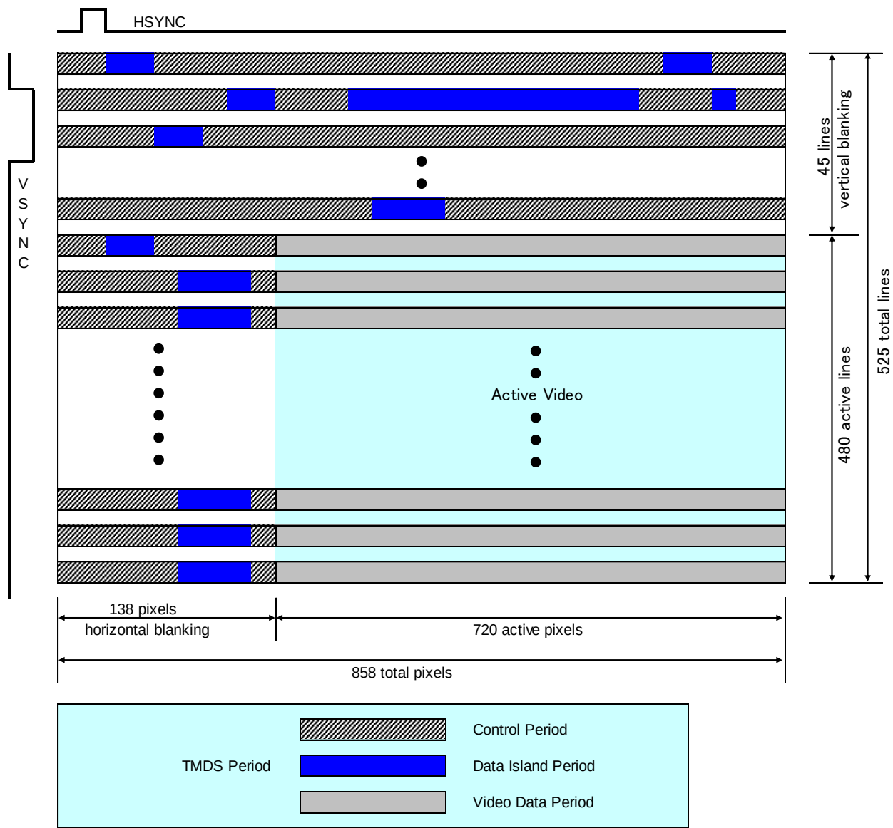
Figure 8-6 Overview of HDMI Operating Modes in 480p Stream
