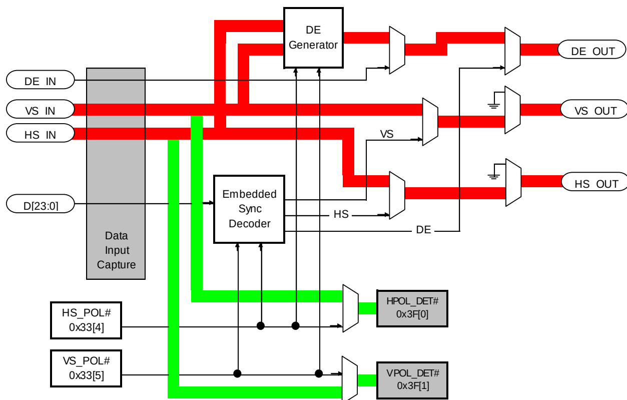
Figure 8-10 Transmitter Video Data with DE Generator from VS, HS
