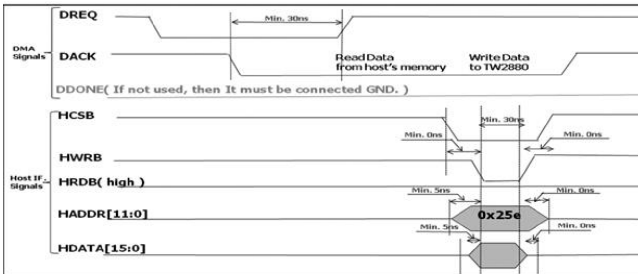
Basic DMA Timing Diagram
