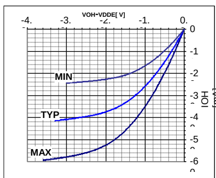
3.3V CMOS Output I/O, M-type V-I Characteristics
