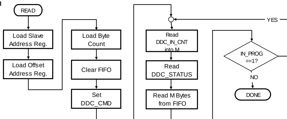
Figure 8-15 Master I 2 C Read Command Flowchart #2
