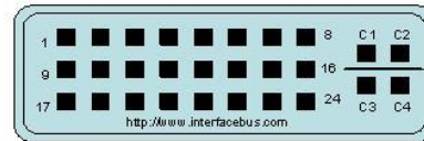
29 pin DVI Connector PinOut and Signal Names
