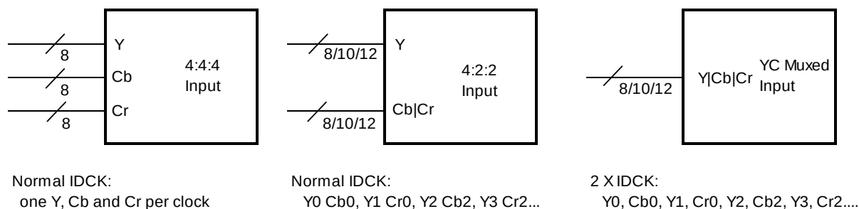
Figure 8-4 Input Bus Diagram for Different Formats
