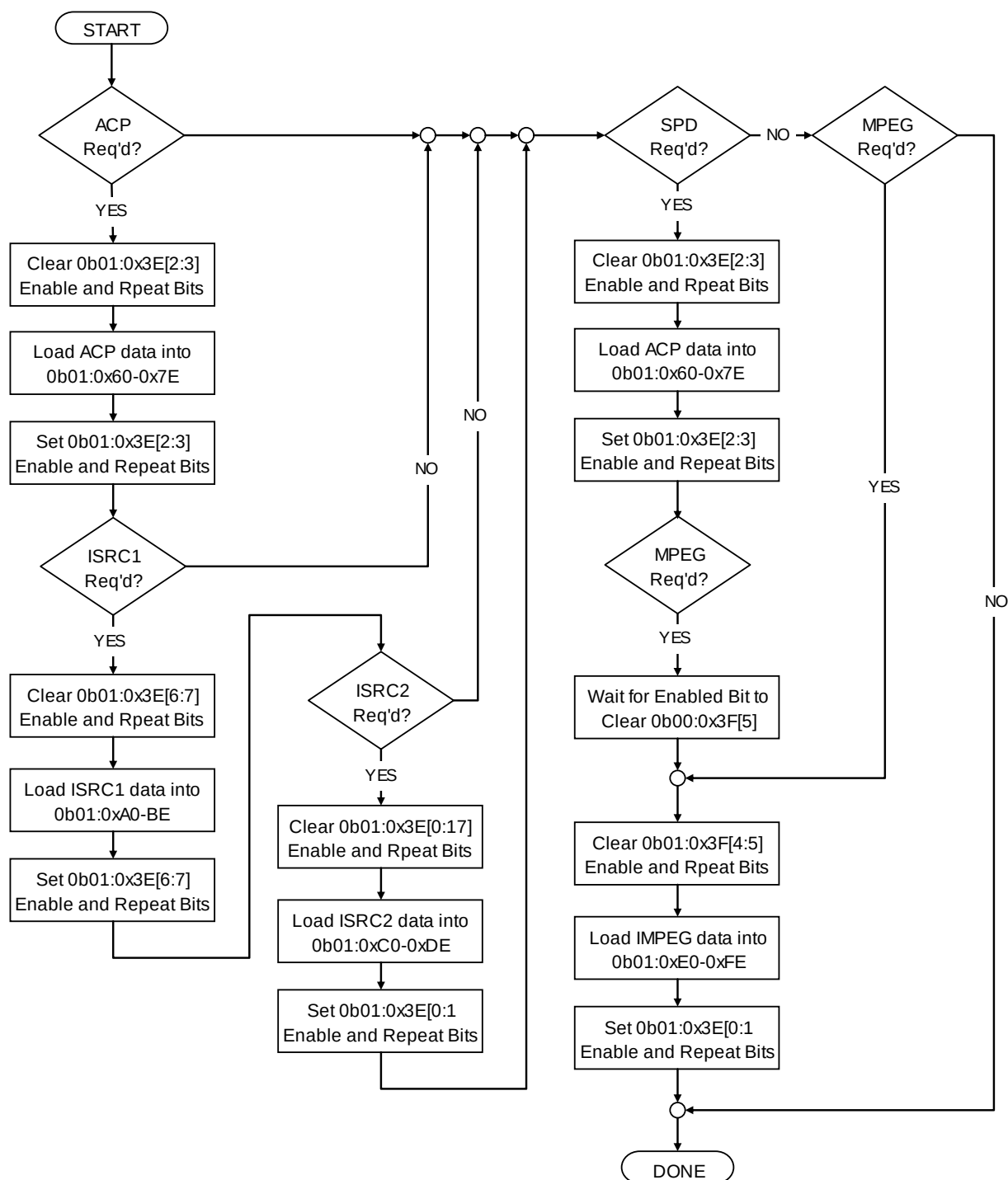
Figure 8-7 ACP Packet Control Flowchart
