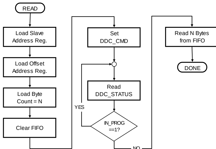
Figure 8-14 Master I 2 C Read Command Flowchart #1
