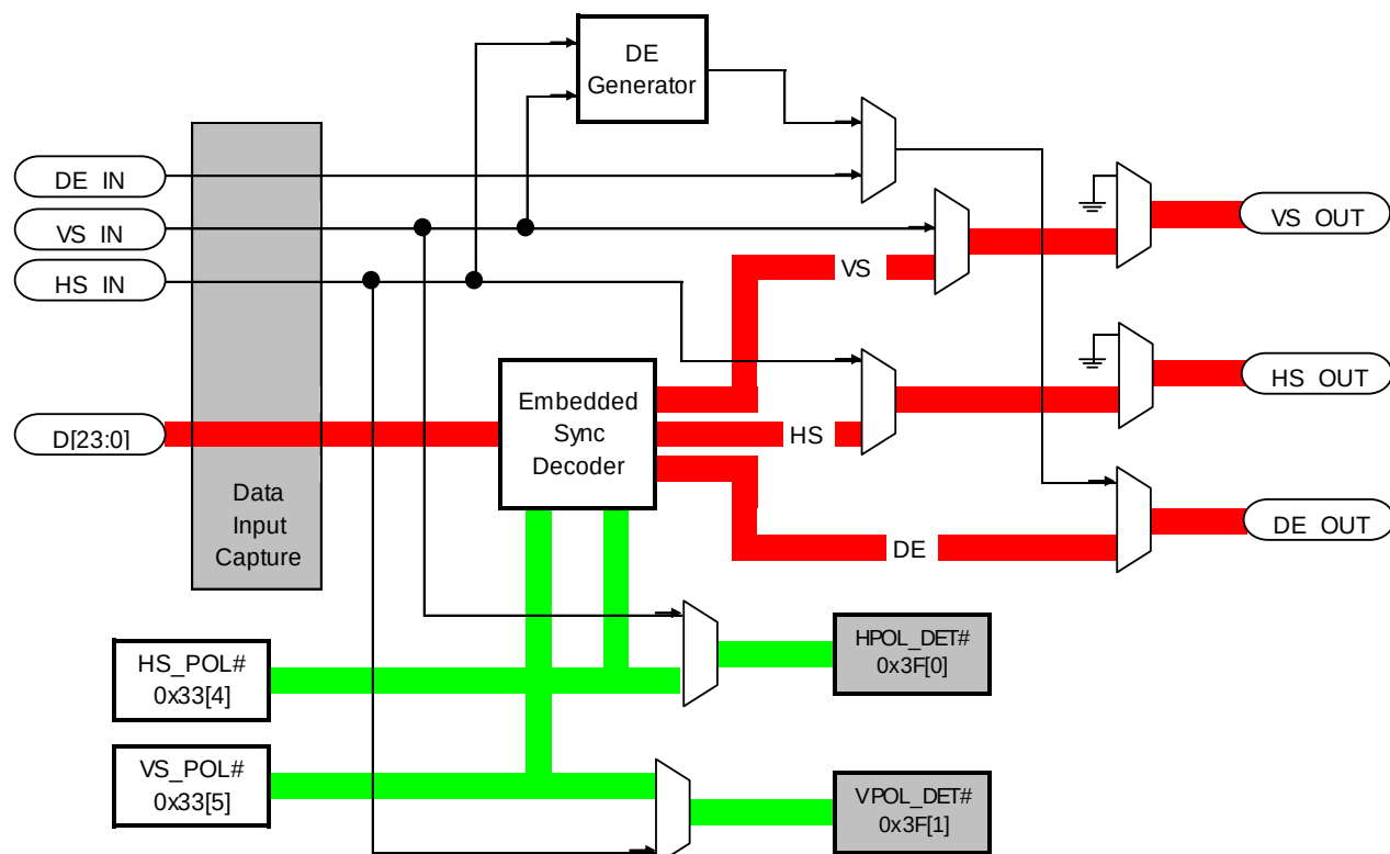
Figure 8-9 Transmitter Video Data with Sync Decoding
