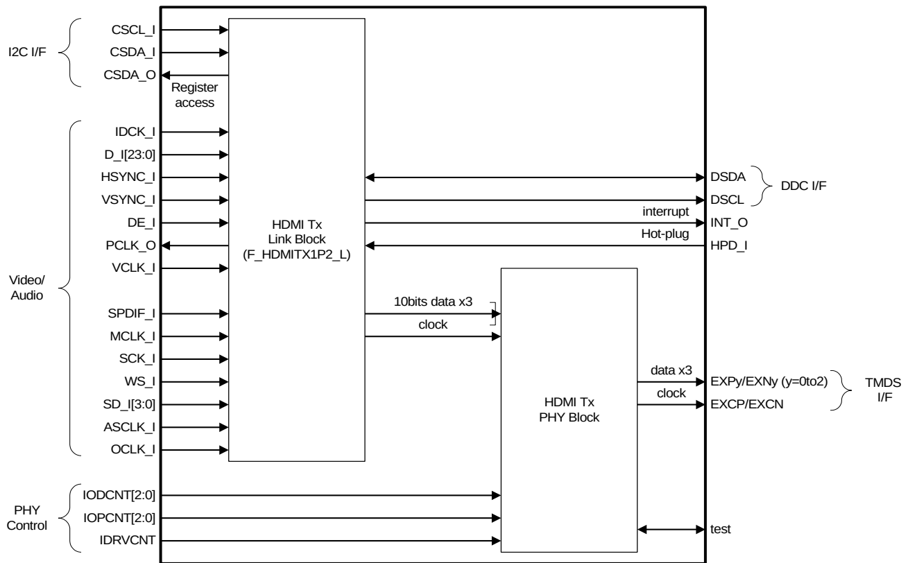
Figure 8-1 HDMI Functional Block Diagram
