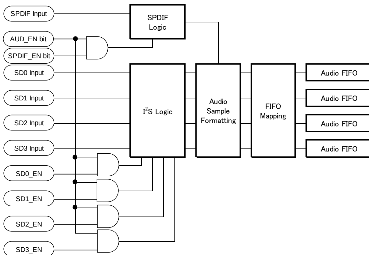
Figure 8-5 Audio Input Control
