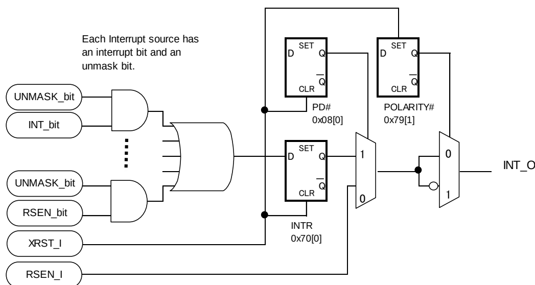
Figure 8-3 Interrupt Pin Control
