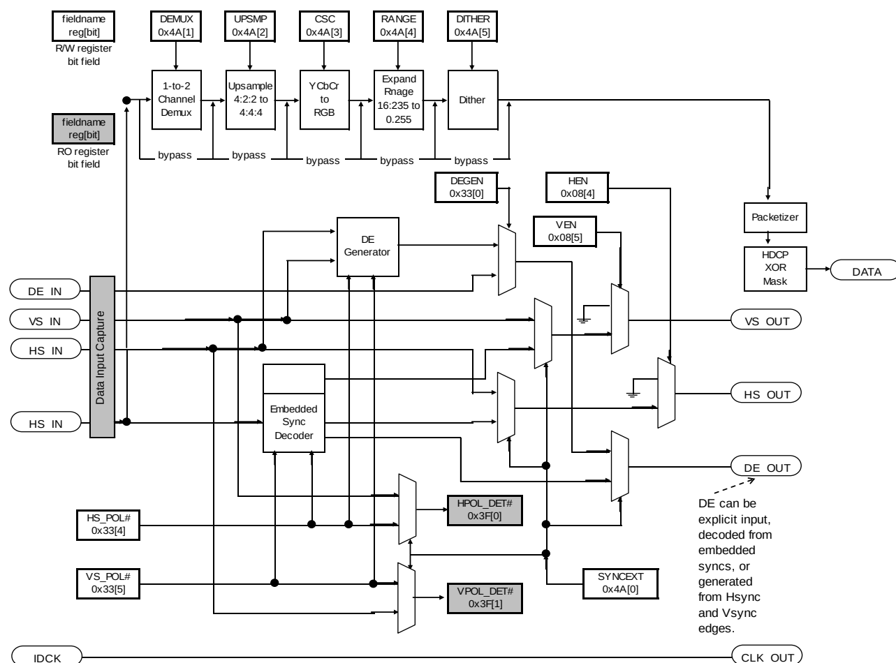
Figure 8-8 Transmitter Video Data Processing Path
