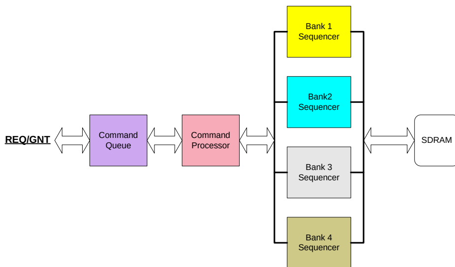
DCU Block Diagram
