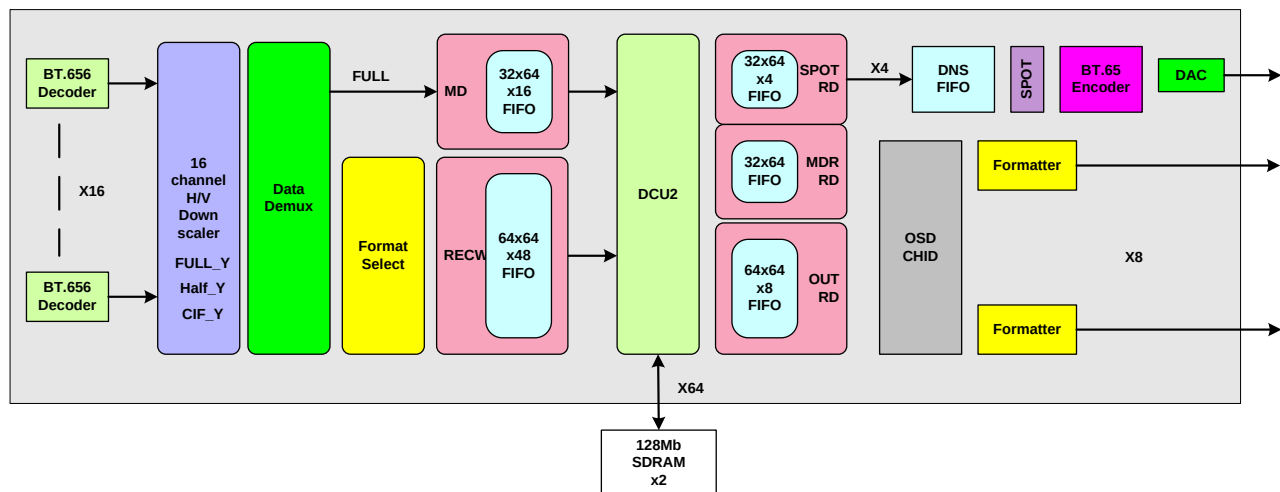
Block Diagram for Record Operation.
