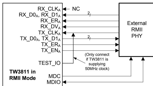
FIGURE 2. OPTIONAL USE OF TEST_IO AS RMII CLOCK SOURCE
