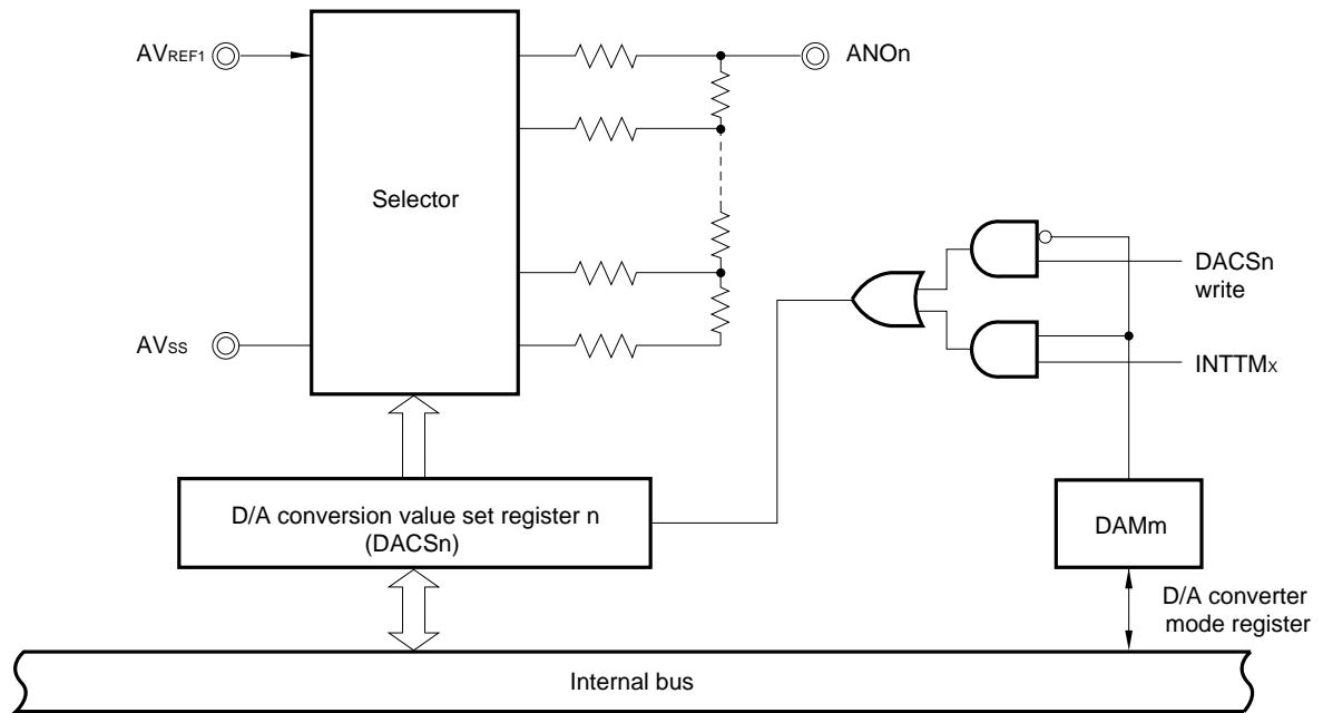
Figure 5-10. D/A Converter Block Diagram
