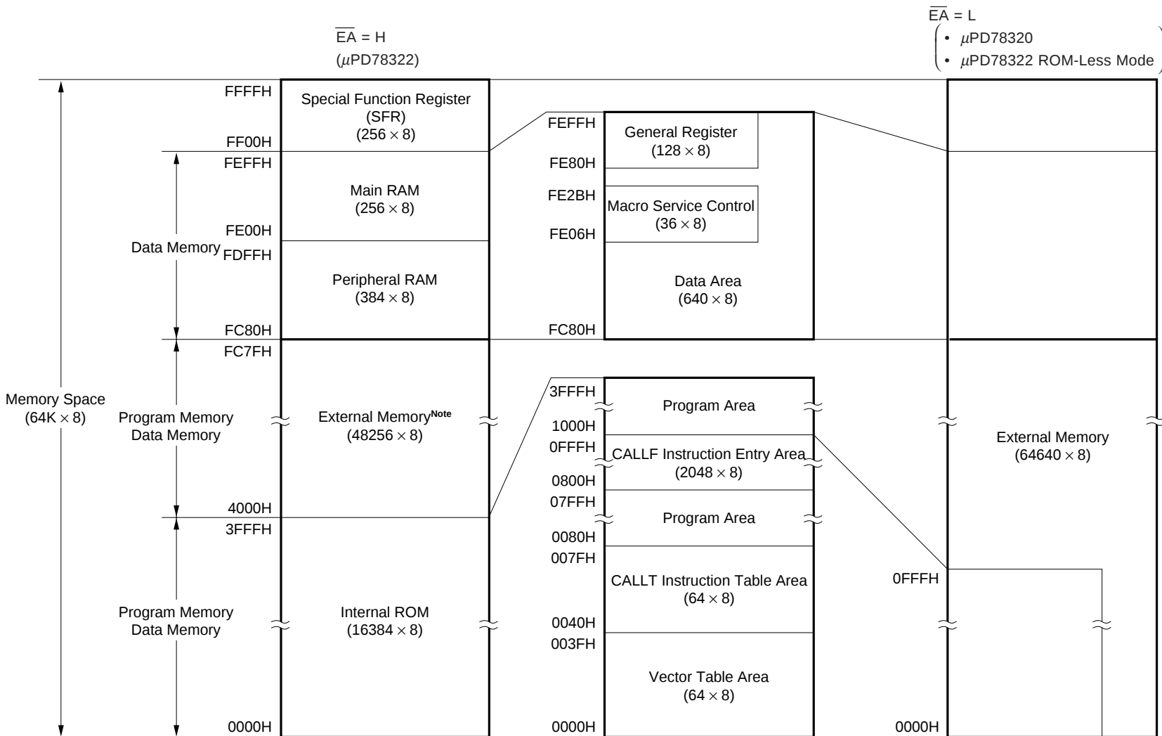
Figure 2-1. Memory Map
