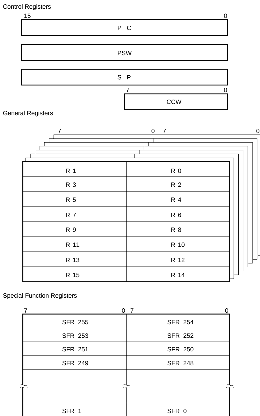
Figure 2-2. Register Configuration
