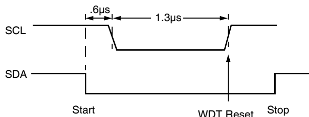
Figure 4. Watchdog Restart
