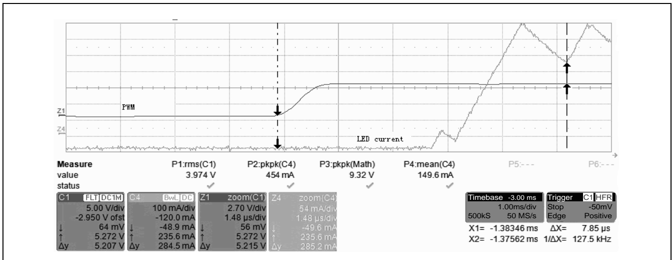
Figure 1.8 Dimming Rate with 100Hz Square Wave Control Signal (PWM) at ADJ Pin (current rise time=7.85 \mu s )
