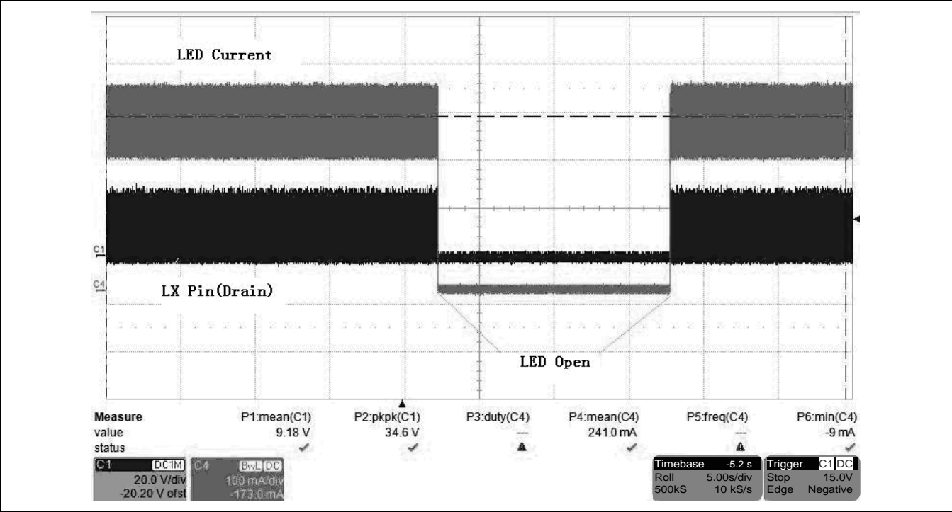
Figure 1.9 LED Open-Circuit Protection ( R_s=0.30\Omega , L1=47\mu H , V_{IN} = 24\text{ V} )
