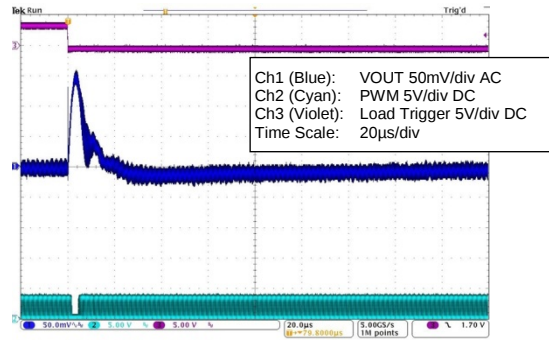
Figure 5.164 ZSPM1509 with Comp0; 8A to 3A Load Step; and Max. Capacitance
