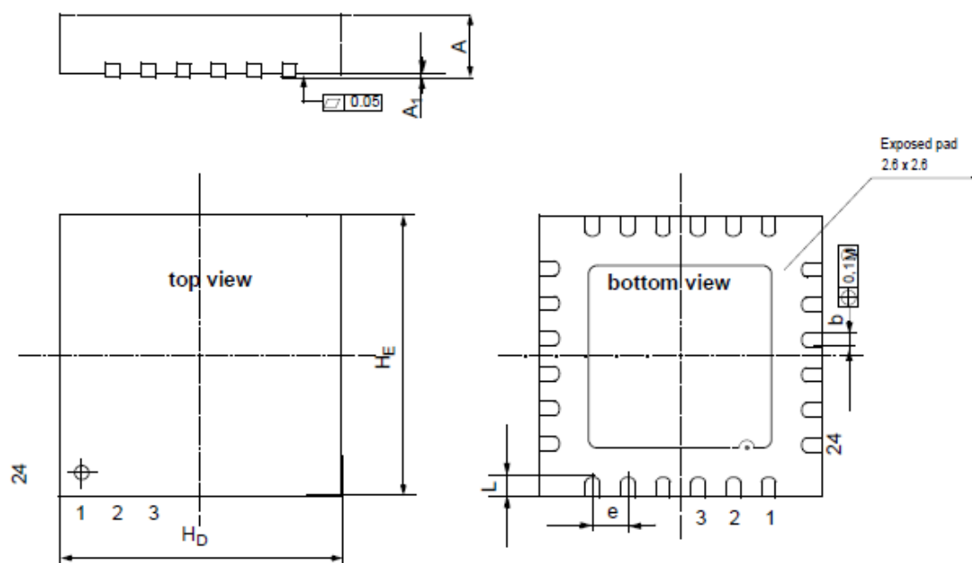
Figure 6.1 24-Pin QFN Package Drawing
