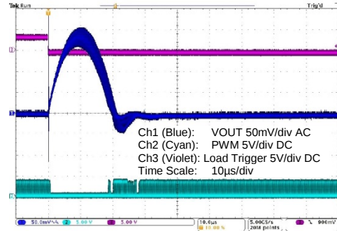
Figure 5.189 ZSPM1511 with Comp1; 15A to 5A Load Step; and Max. Capacitance
