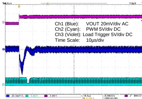
Figure 5.191 ZSPM1511 with Comp2; 5A to 15A Load Step; and Min. Capacitance
