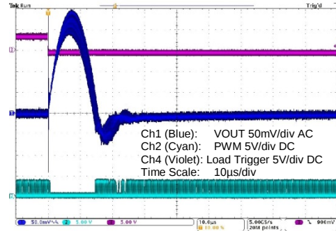
Figure 5.184 ZSPM1511 with Comp0; 15A to 5A Load Step; and Max. Capacitance
