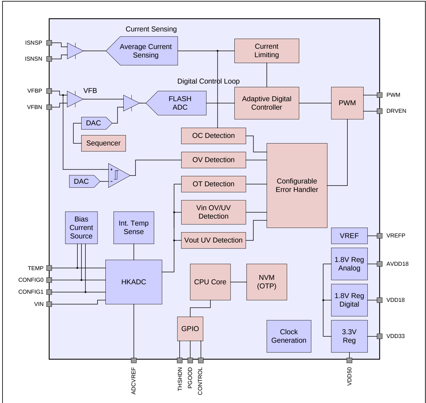
Figure 2.2 Block Diagram
