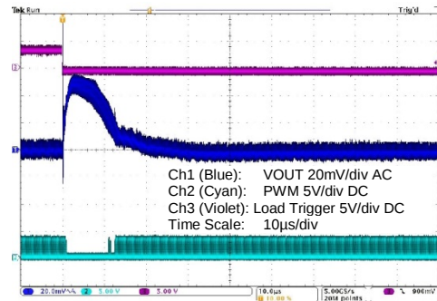
Figure 5.192 ZSPM1511 with Comp2; 15A to 5A Load Step; and Min. Capacitance
